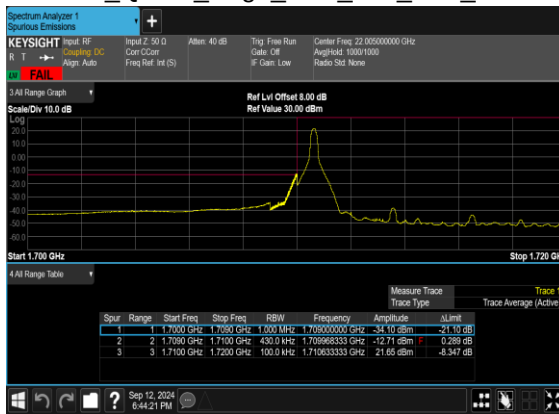
N66(40M)_DFT-s- OFDM_QPSK_Edge_1RB_Left_Low_CH
