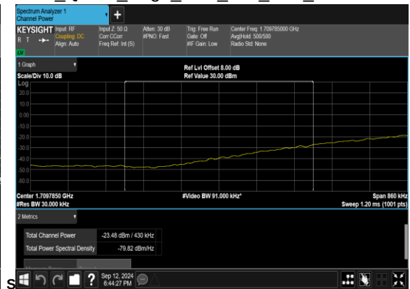
N66(40M)_DFT-s- OFDM_QPSK_Edge_1RB_Left_Low_CH_CHP_PAS
