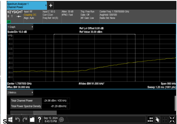
N66(40M)_DFT-s- OFDM_BPSK_Edge_1RB_Left_Low_CH_CHP_PAS
