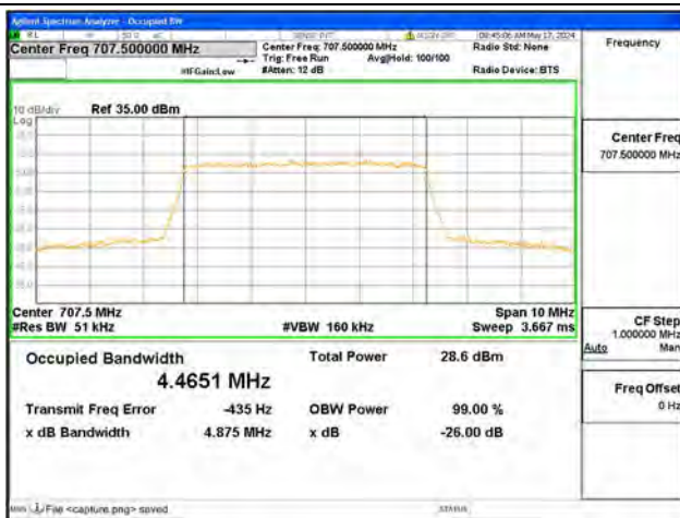
B12 / 5MHz / 64QAM/ Mid CH
