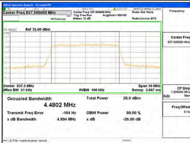
B19 / 5MHz / 64QAM/ Mid CH
