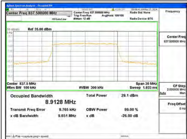
B19 / 10MHz / 16QAM/ Mid CH
