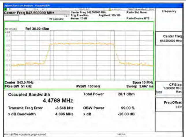
B19 / 5MHz / 64QAM/ High CH
