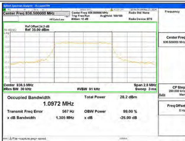
B26 Part22 / 1.4MHz / 64QAM/ Mid CH
