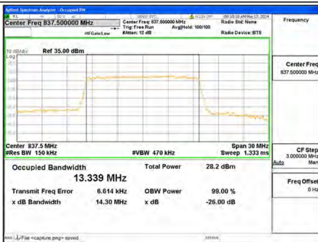
B19 / 15MHz / 64QAM/ Mid CH
