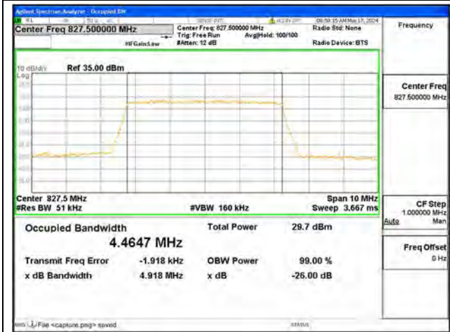
B18 part22 / 5MHz / QPSK/ High CH
