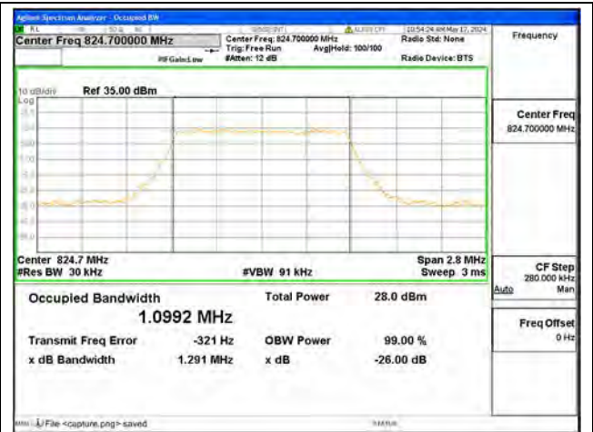
B26 Part22 / 1.4MHz / 64QAM/ Low CH
