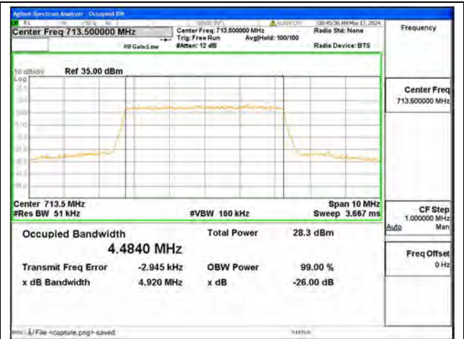
B12 / 5MHz / 64QAM/ High CH
