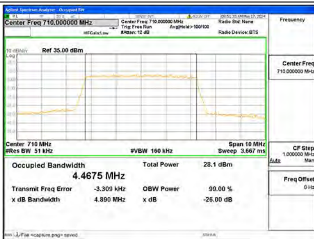
B17 / 5MHz / 64QAM/ Mid CH
