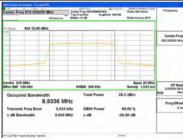
B19 / 10MHz / 64QAM/ Low CH
