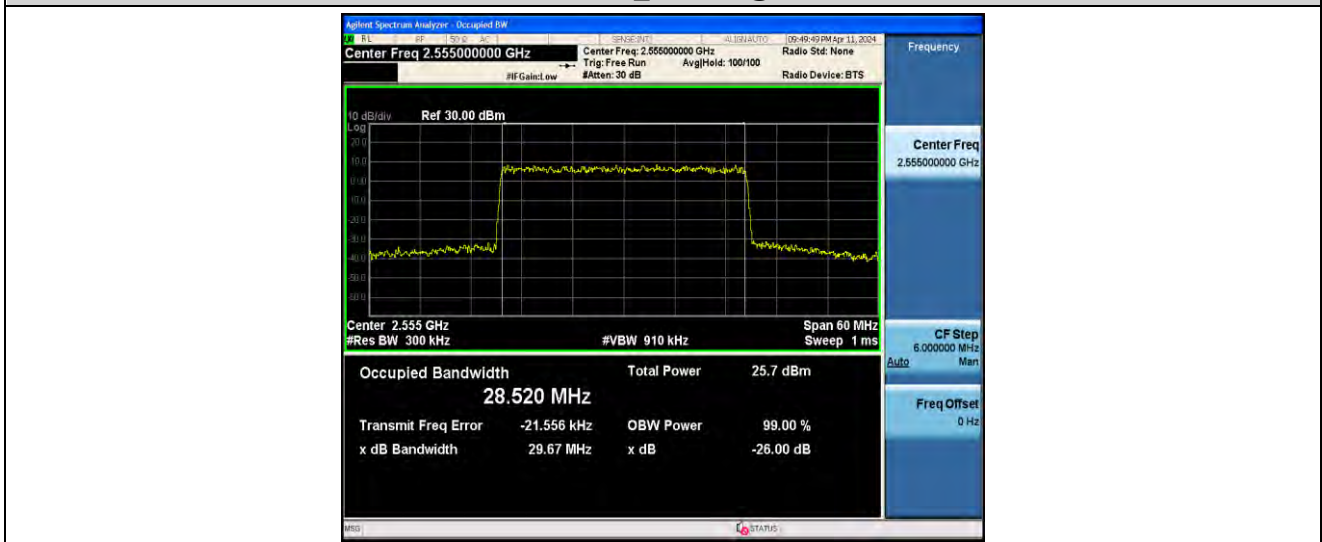
1-N7-PC3-15-30-H-9-CP-256QAM-Outer_Full-160@0-ANT0-28.520-29.67-≤30-PASS
