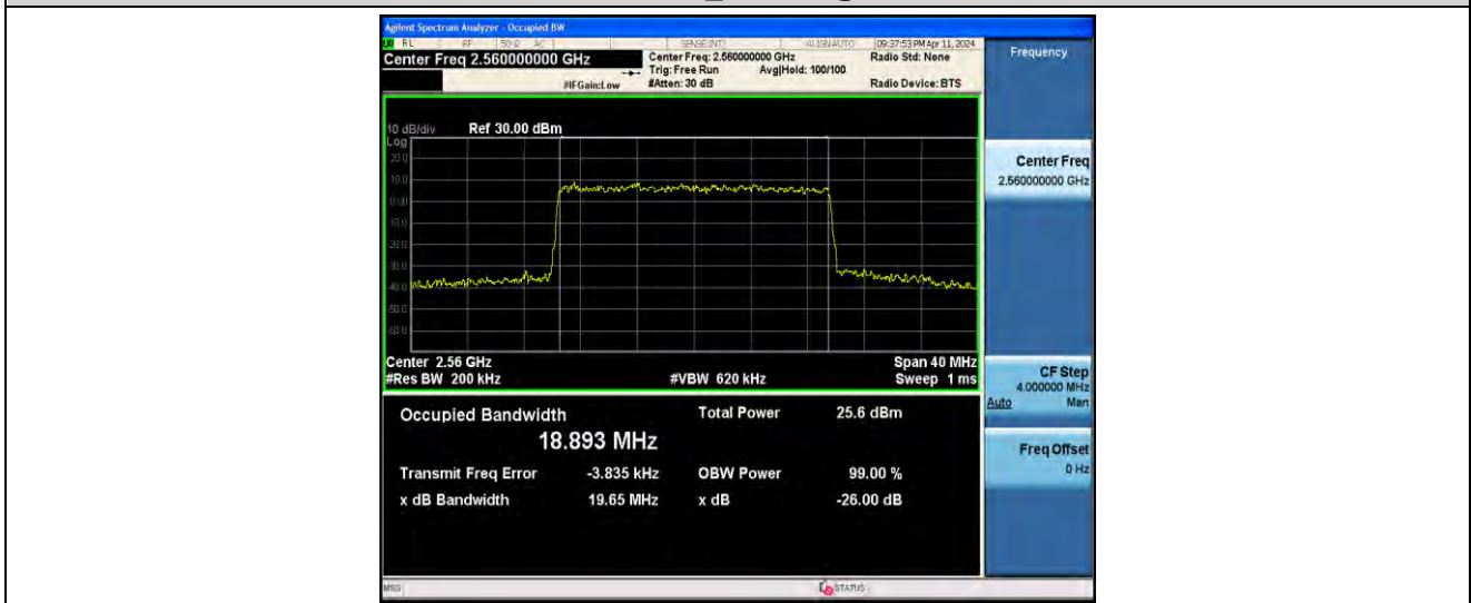
1-N7-PC3-15-20-H-9-CP-256QAM-Outer_Full-106@0-ANT0-18.893-19.65-≤20-PASS
