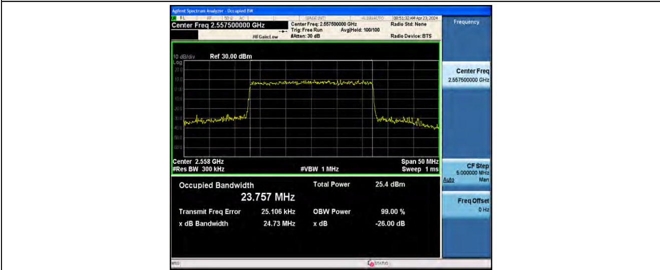
1-N7-PC3-15-25-H-9-CP-256QAM-Outer_Full-133@0-ANT0-23.757-24.73-<=25-PASS
