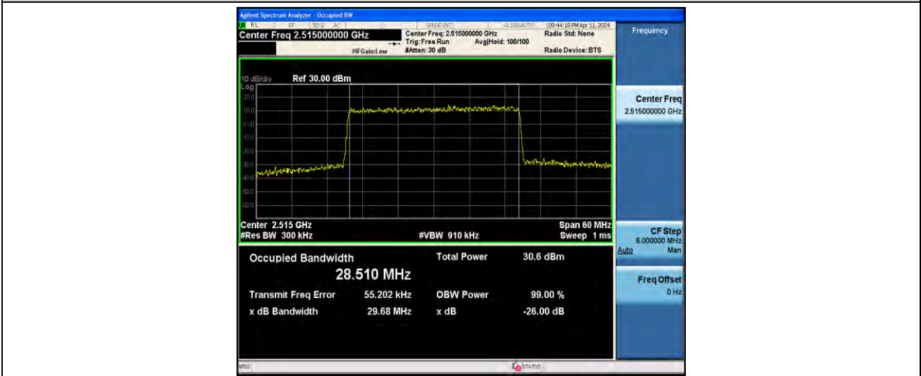
1-N7-PC3-15-30-L-3-DFT-16QAM-Outer_Full-160@0-ANT0-28.510-29.68-≤30-PASS
