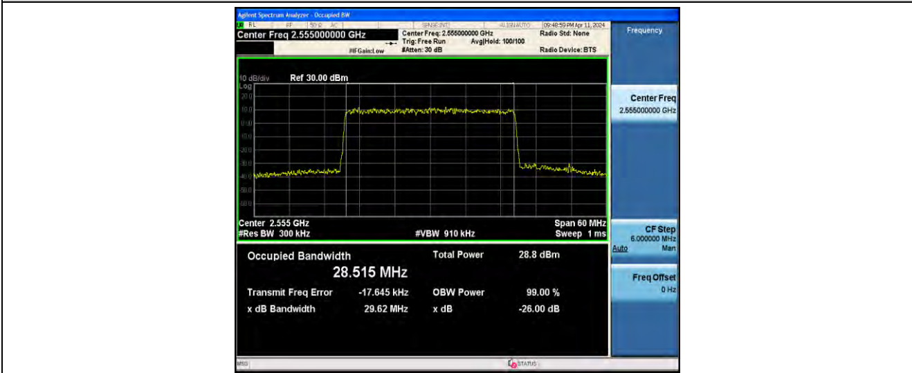
1-N7-PC3-15-30-H-5-DFT-256QAM-Outer_Full-160@0-ANT0-28.515-29.62-≤30-PASS
