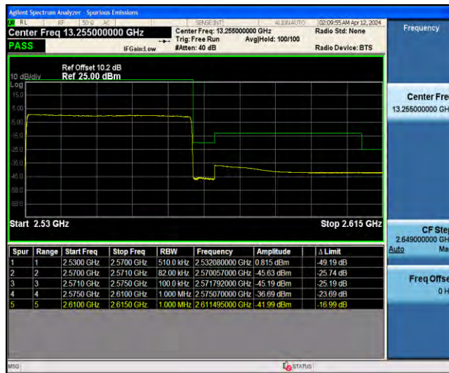
1-N7-PC3-15-40-H-6-CP-QPSK-Outer_Full-216@0-ANT0-2611.50-16.99--41.99-PASS
