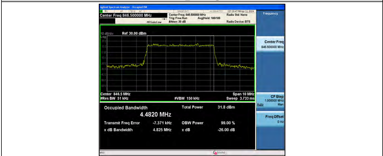
1-N5-PC3-15-5-H-3-DFT-16QAM-Outer_Full-25@0-ANT1-4.4820-4.825-≤5-PASS
