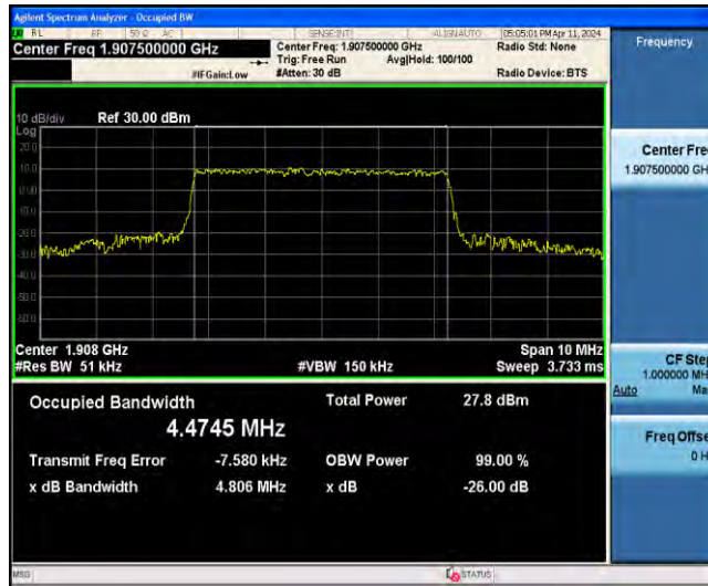
1-N2-PC3-15-5-H-6-CP-QPSK-Outer_Full-25@0-ANT0-4.4745-4.806-≤5-PASS
