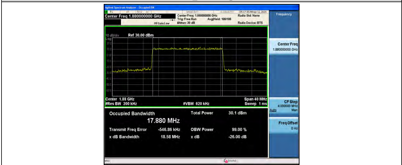
1-N2-PC3-15-20-M-3-DFT-16QAM-Outer_Full-100@0-ANT0-17.880-18.58-≤20-PASS
