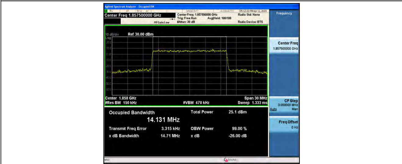
1-N2-PC3-15-15-L-9-CP-256QAM-Outer_Full-79@0-ANT0-14.131-14.71-≤15-PASS
