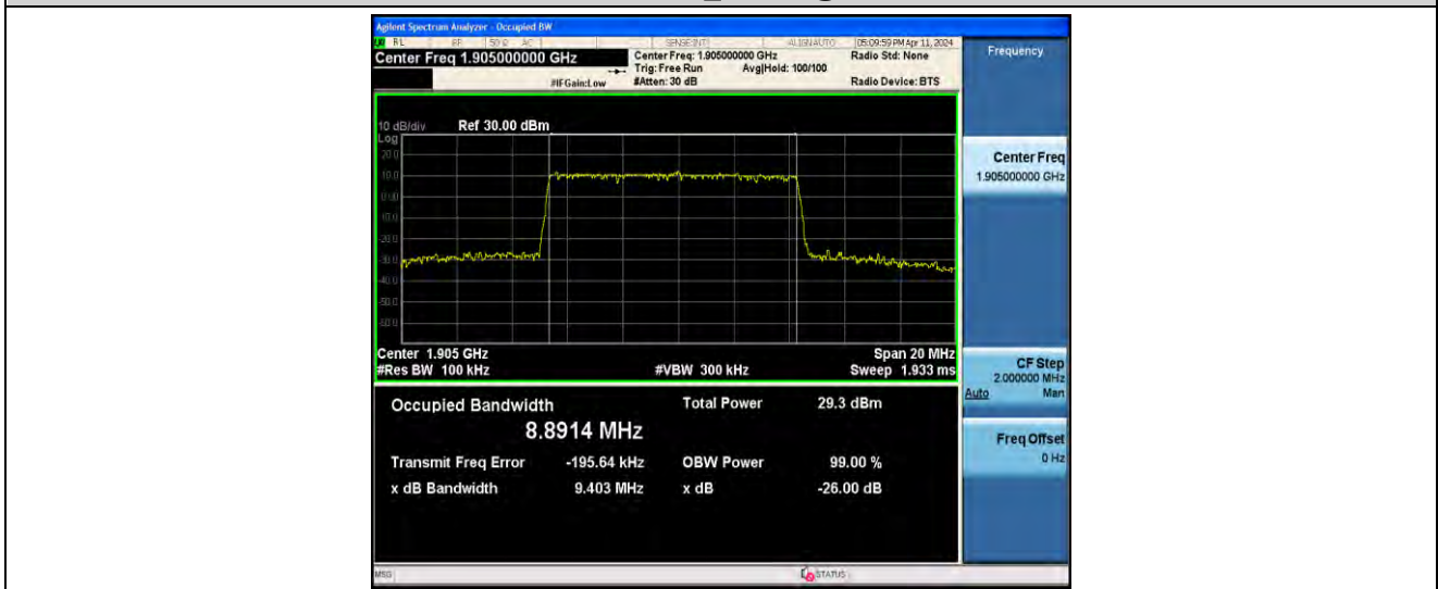
1-N2-PC3-15-10-H-5-DFT-256QAM-Outer_Full-50@0-ANT0-8.8914-9.403-≤10-PASS
