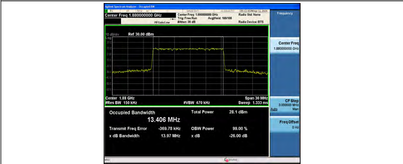
1-N2-PC3-15-15-M-5-DFT-256QAM-Outer_Full-75@0-ANT0-13.406-13.97-≤15-PASS
