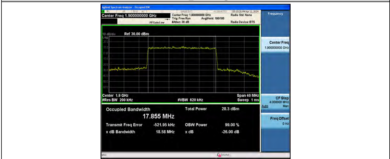
1-N2-PC3-15-20-H-5-DFT-256QAM-Outer_Full-100@0-ANT0-17.855-18.58-≤20-PASS
