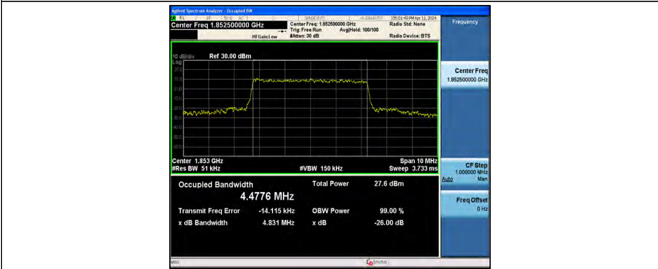
1-N2-PC3-15-5-L-7-CP-16QAM-Outer_Full-25@0-ANT0-4.4776-4.831-≤5-PASS
