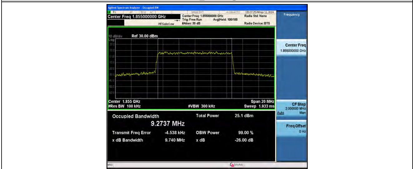
1-N2-PC3-15-10-L-9-CP-256QAM-Outer_Full-52@0-ANT0-9.2737-9.740-≤10-PASS
