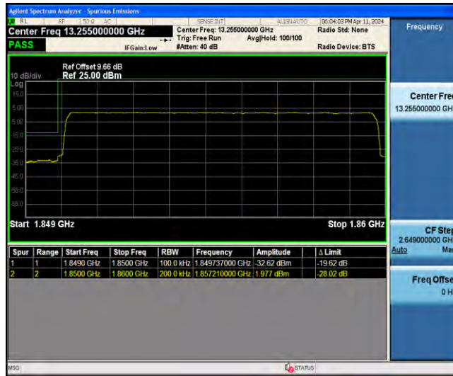
1-N2-PC3-15-10-L-6-CP-QPSK-Outer_Full-52@0-ANT0-1849.74-19.62--32.62-PASS
