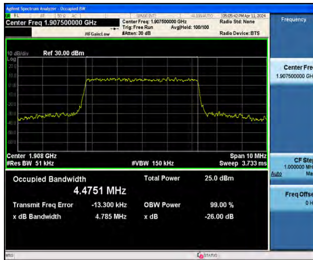
1-N2-PC3-15-5-H-9-CP-256QAM-Outer_Full-25@0-ANT0-4.4751-4.785-≤5-PASS
