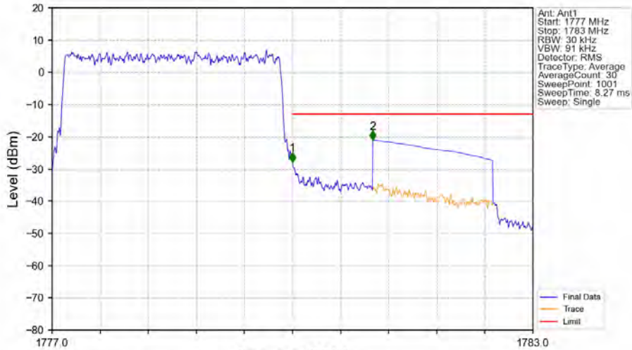
Band66_3MHz_QPSK_HCH_1778.5MHz_RB_15_0_NTNV
