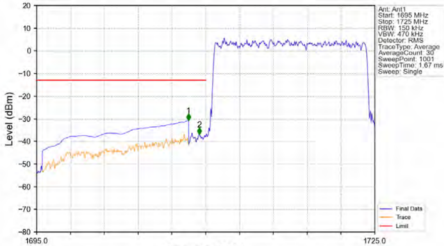
Band66_15MHz_64QAM_LCH_1717.5MHz_RB_75_0_NTNV
