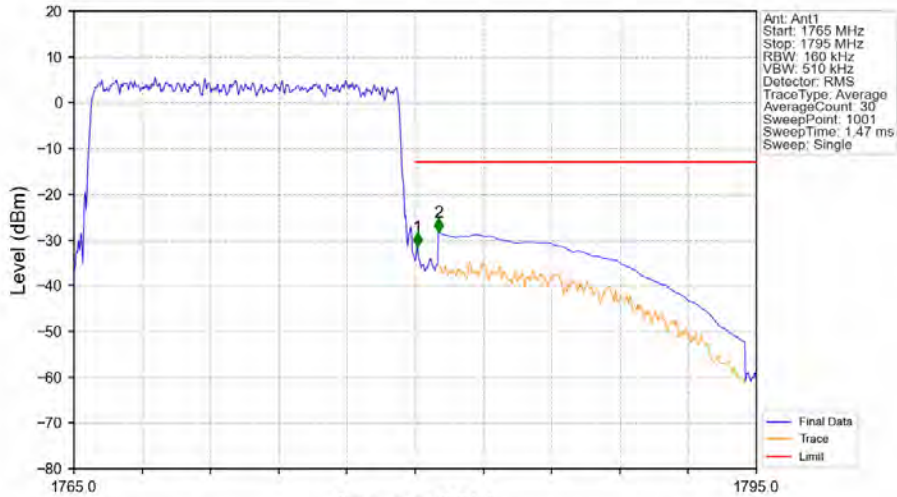
Band66_15MHz_16QAM_HCH_1772.5MHz_RB_75_0_NTNV
