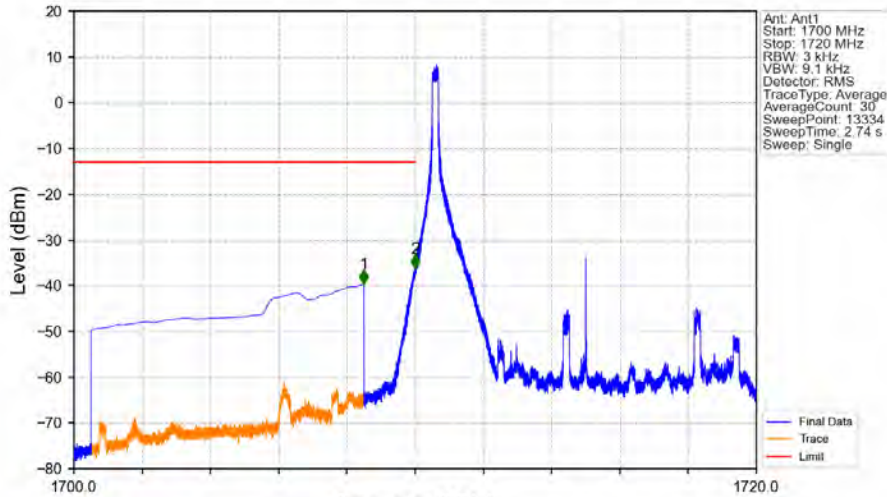
Band66_10MHz_16QAM_LCH_1715MHz_RB_1_0_NTNV
