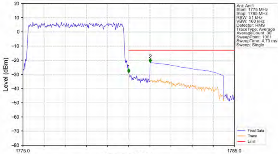
Band66_5MHz_QPSK_HCH_1777.5MHz_RB_25_0_NTNV
