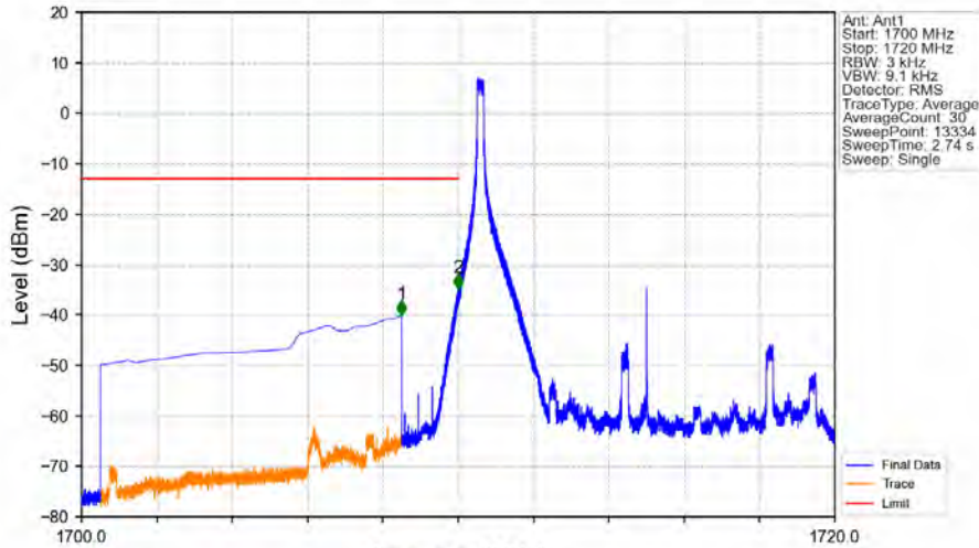
Band66_10MHz_64QAM_LCH_1715MHz_RB_1_0_NTNV
