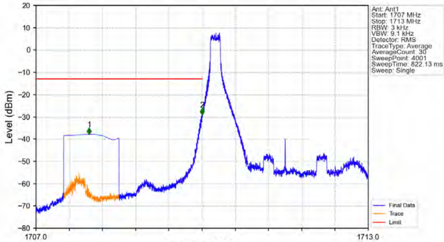
Band66_3MHz_64QAM_LCH_1711.5MHz_RB_1_0_NTNV
