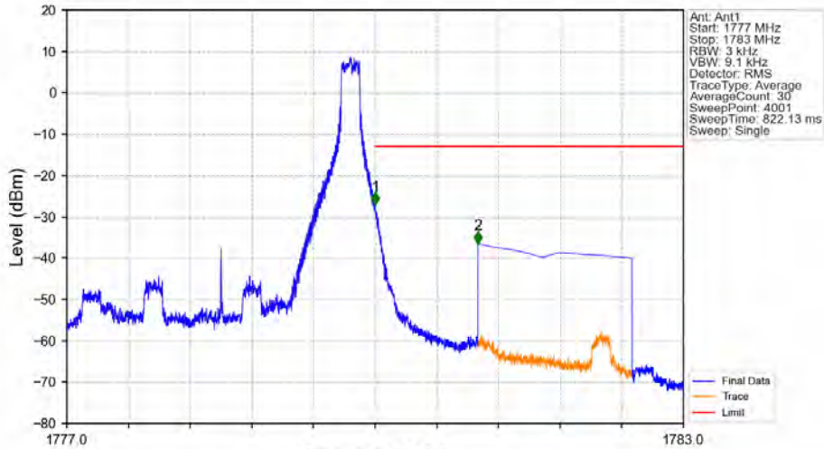
Band66_3MHz_QPSK_HCH_1778.5MHz_RB_1_14_NTNV
