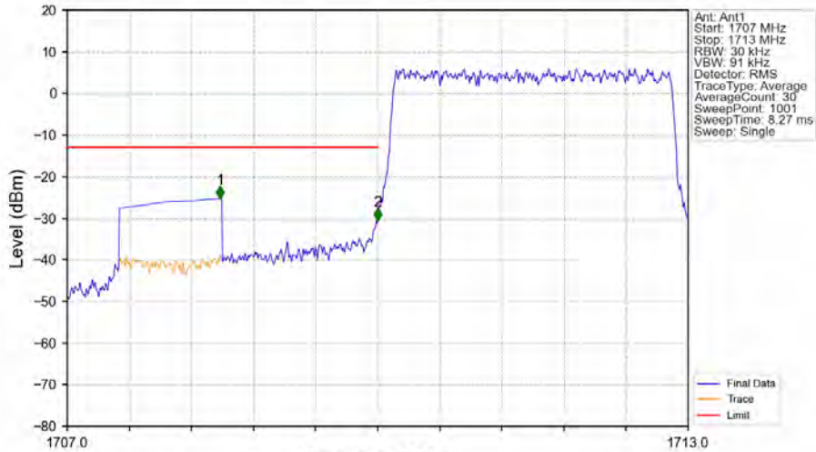
Band66_3MHz_QPSK_LCH_1711.5MHz_RB_15_0_NTNV
