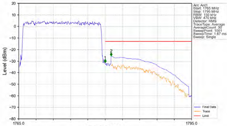
Band66_15MHz_64QAM_HCH_1772.5MHz_RB_75_0_NTNV
