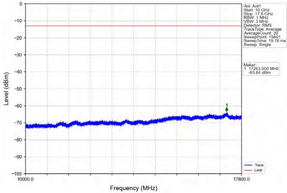
Band66_10MHz_64QAM_HCH_1775MHz_RB_1_0_NTNV
