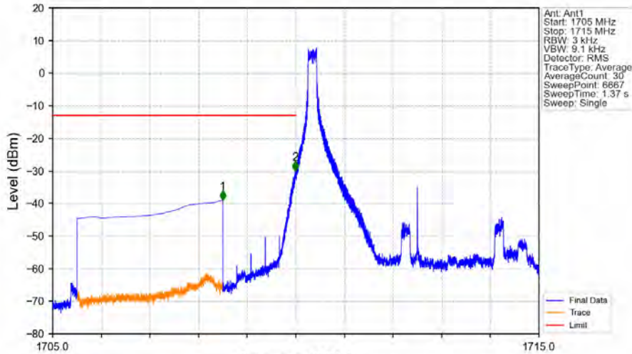
Band66_5MHz_64QAM_LCH_1712.5MHz_RB_1_0_NTNV
