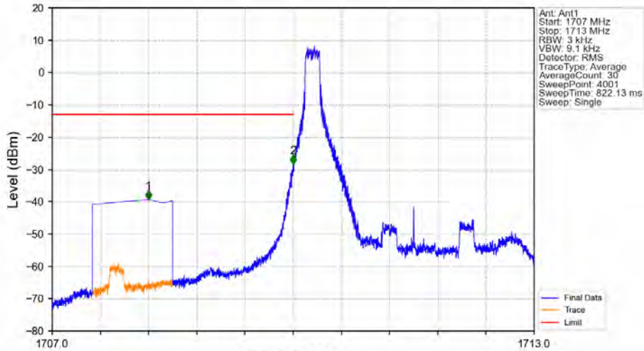
Band66_3MHz_16QAM_LCH_1711.5MHz_RB_1_0_NTV
