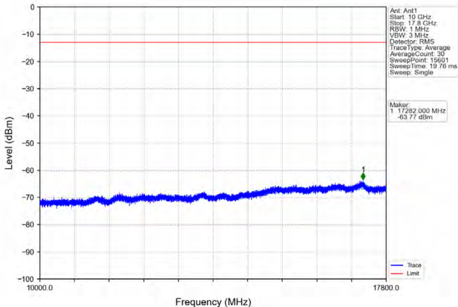
Band66_10MHz_QPSK_HCH_1775MHz_RB_1_0_NTNV
