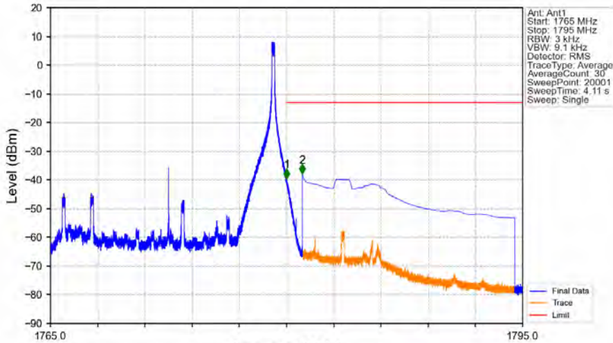
Band66_15MHz_64QAM_HCH_1772.5MHz_RB_1_74_NTNV
