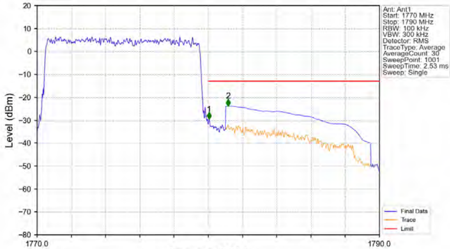
Band66_10MHz_QPSK_HCH_1775MHz_RB_50_0_NTNV
