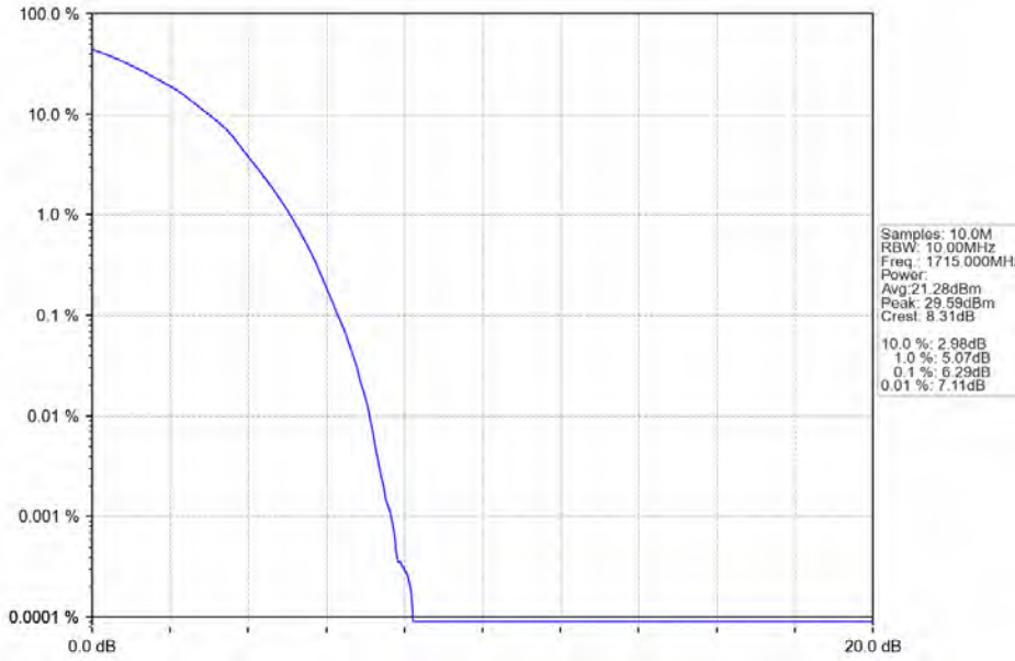
Band66_10MHz_64QAM_LCH_1715MHz_RB_50_0_NTNV
