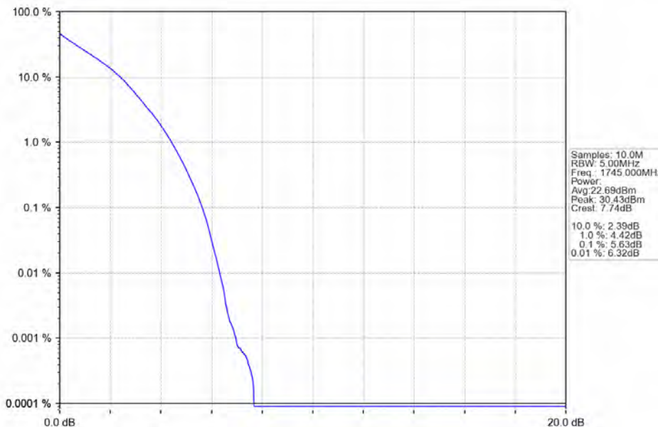
Band66_5MHz_QPSK_MCH_1745MHz_RB_25_0_NTNV
