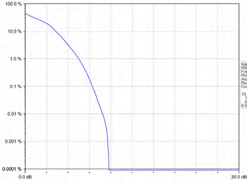
Band66_10MHz_16QAM_LCH_1715MHz_RB_50_0_NTNV
