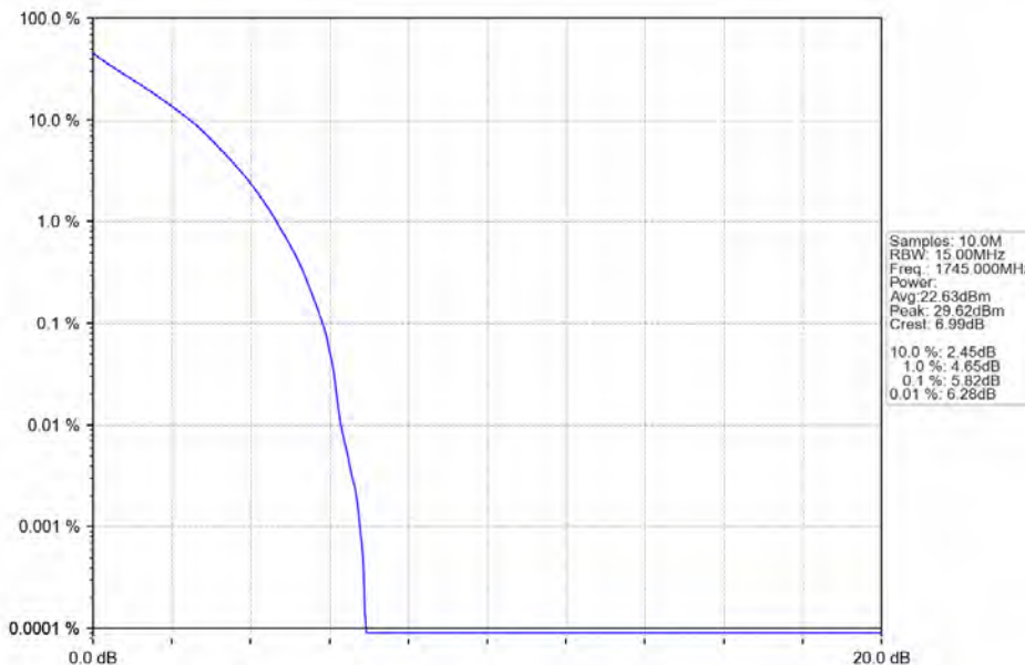
Band66_15MHz_QPSK_MCH_1745MHz_RB_75_0_NTNV
