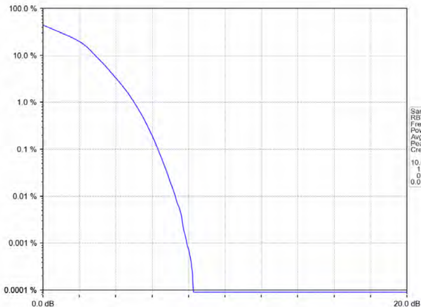
Band66_20MHz_16QAM_MCH_1745MHz_RB_100_0_NTNV
