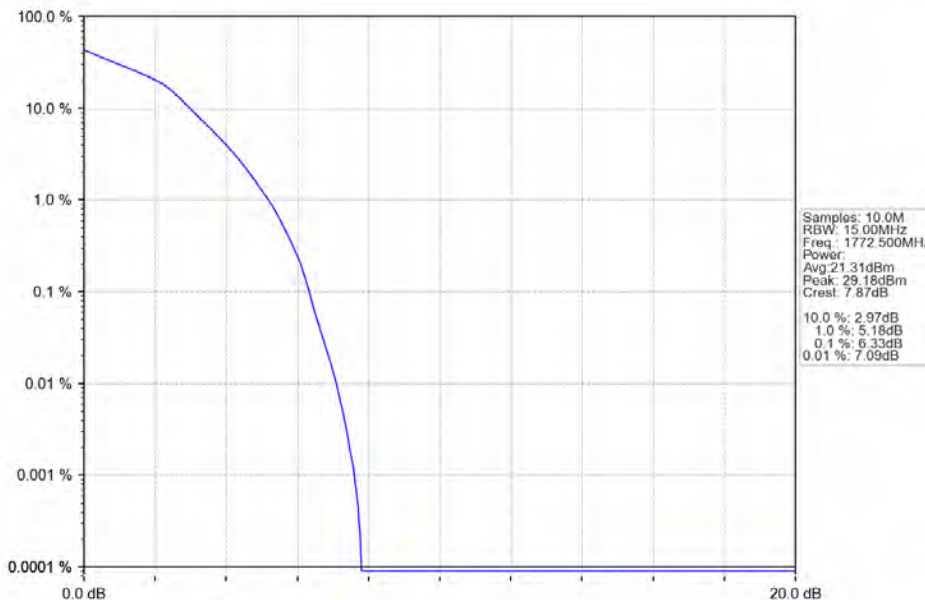
Band66_15MHz_16QAM_HCH_1772.5MHz_RB_75_0_NTNV
