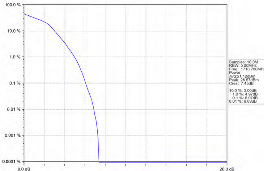
Band66_1.4MHz_16QAM_LCH_1710.7MHz_RB_6_0_NTNV
