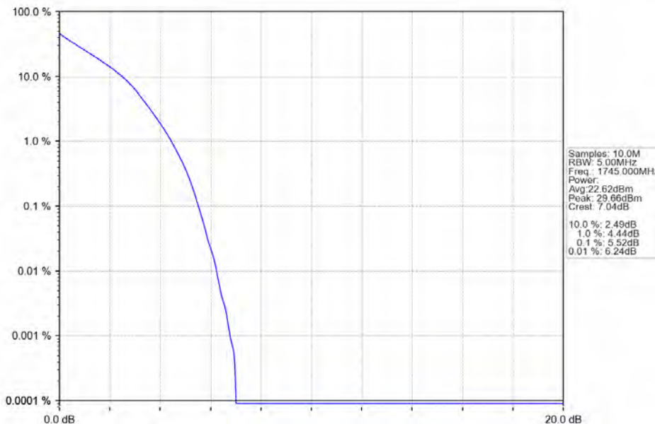
Band66_3MHz_QPSK_MCH_1745MHz_RB_15_0_NTNV
