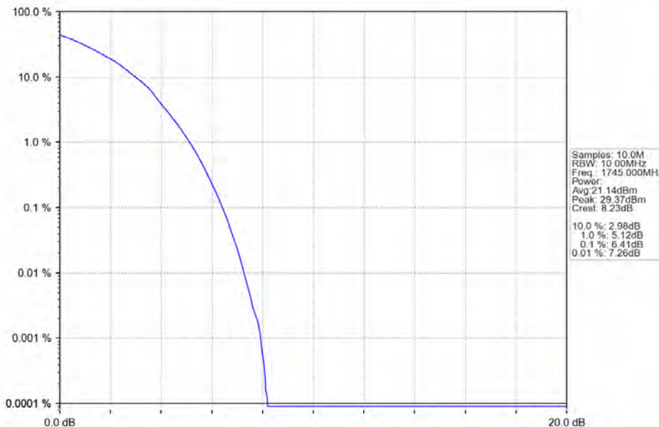
Band66_10MHz_64QAM_MCH_1745MHz_RB_50_0_NTNV
