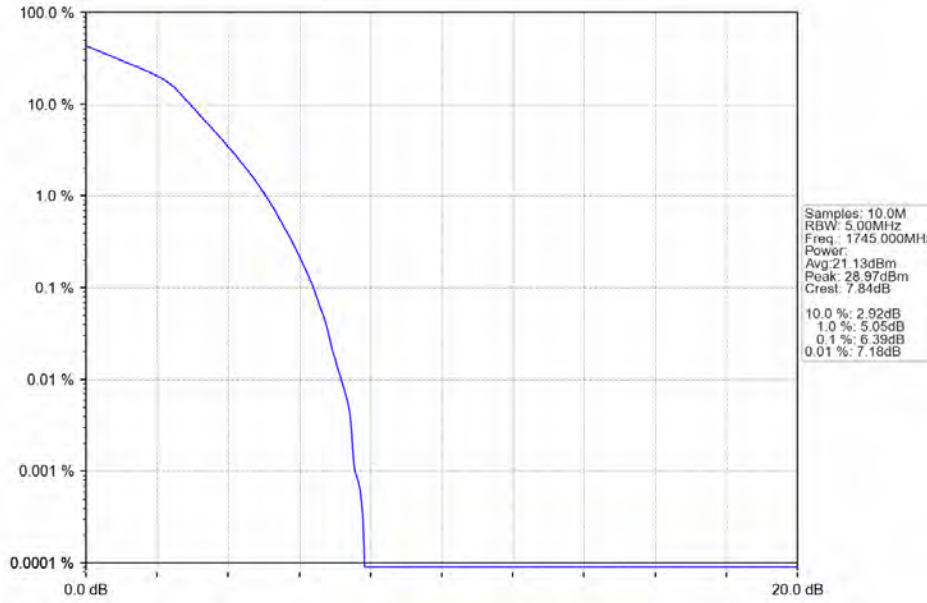
Band66_3MHz_16QAM_MCH_1745MHz_RB_15_0_NTNV
