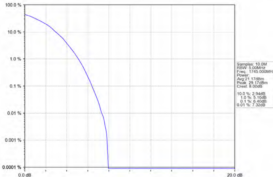
Band66_5MHz_64QAM_MCH_1745MHz_RB_25_0_NTNV
