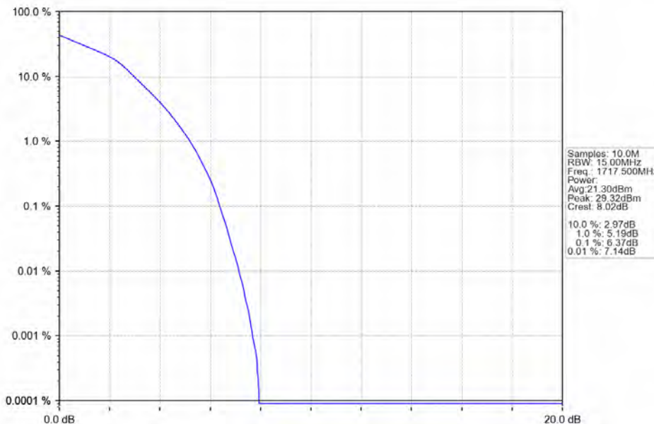
Band66_15MHz_16QAM_LCH_1717.5MHz_RB_75_0_NTNV
