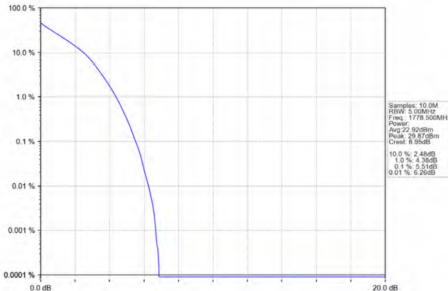
Band66_3MHz_QPSK_HCH_1778.5MHz_RB_15_0_NTNV
