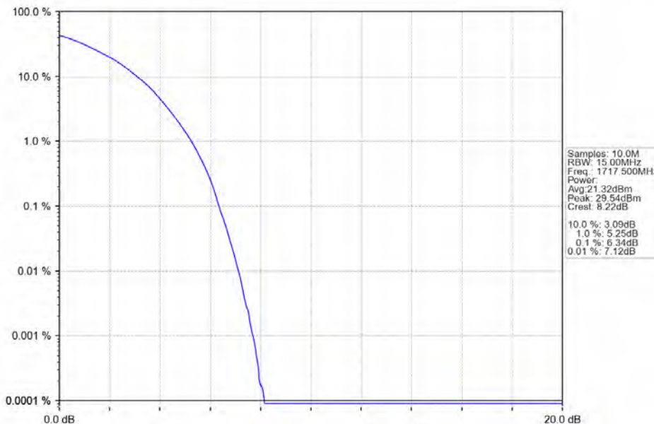
Band66_15MHz_64QAM_LCH_1717.5MHz_RB_75_0_NTNV
