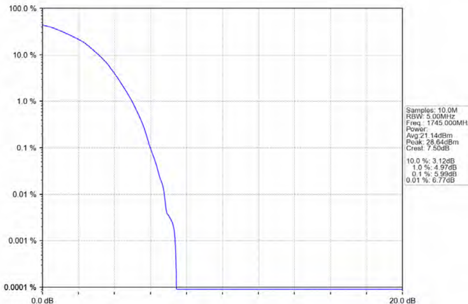
Band66_1.4MHz_64QAM_MCH_1745MHz_RB_6_0_NTNV
