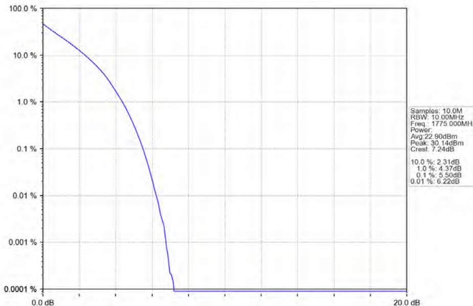
Band66_10MHz_QPSK_HCH_1775MHz_RB_50_0_NTNV
