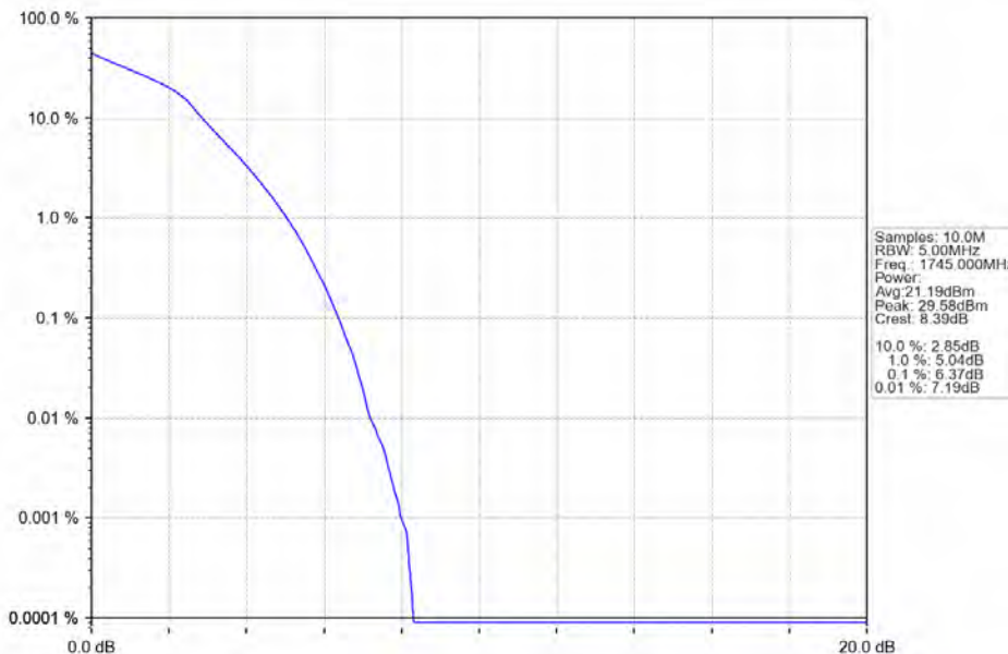
Band66_5MHz_16QAM_MCH_1745MHz_RB_25_0_NTNV
