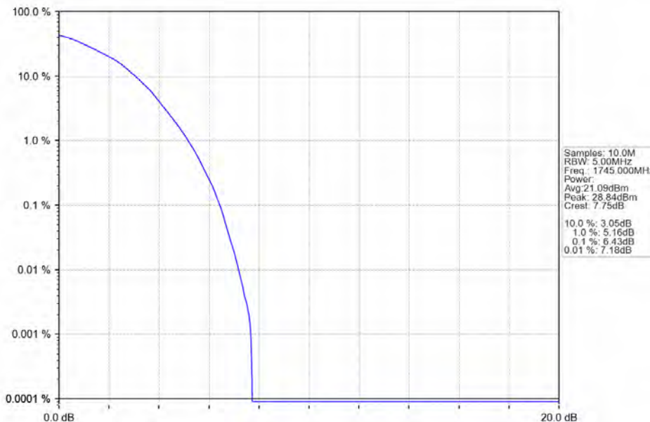
Band66_3MHz_64QAM_MCH_1745MHz_RB_15_0_NTNV
