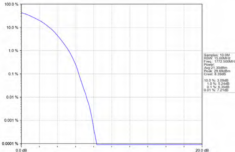
Band66_15MHz_64QAM_HCH_1772.5MHz_RB_75_0_NTNV
