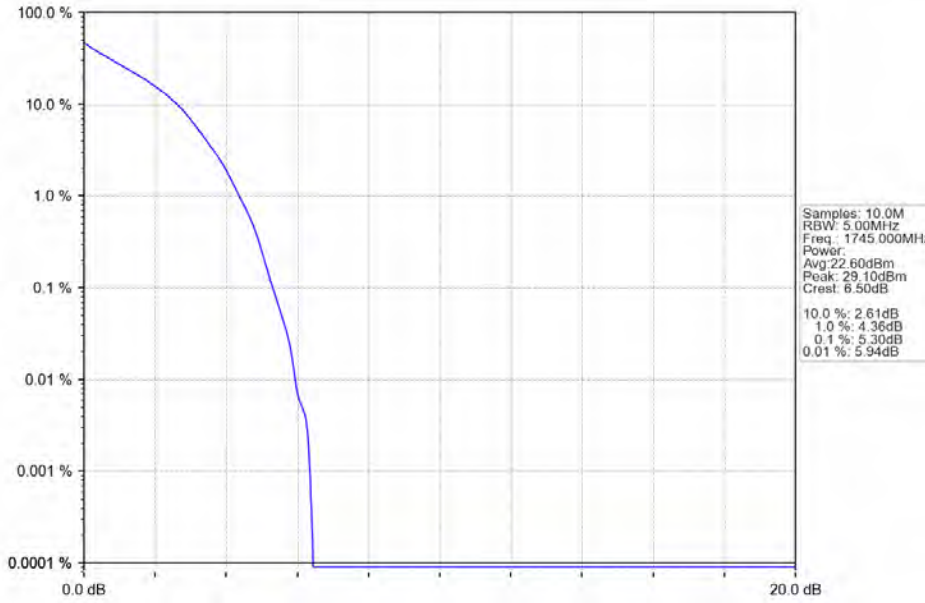
Band66_1.4MHz_QPSK_MCH_1745MHz_RB_6_0_NTNV
