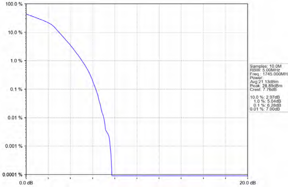
Band66_1.4MHz_16QAM_MCH_1745MHz_RB_6_0_NTNV
