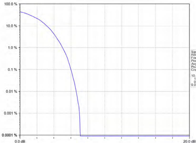
Band66_1.4MHz_64QAM_LCH_1710.7MHz_RB_6_0_NTNV
