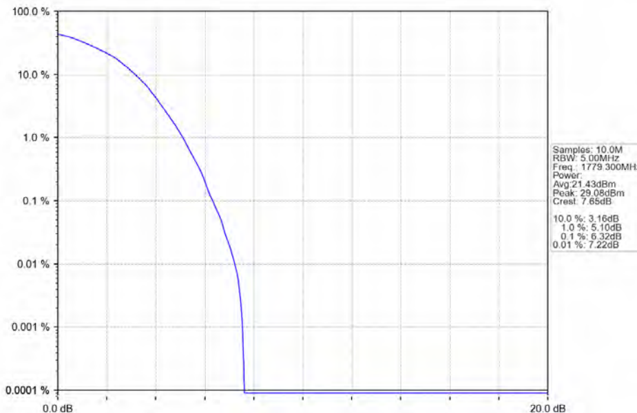
Band66_1.4MHz_64QAM_HCH_1779.3MHz_RB_6_0_NTNV
