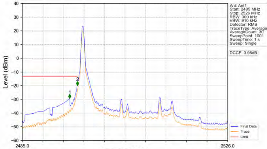
Band41_20MHz_16QAM_LCH_2506MHz_RB_1_0_NTNV
