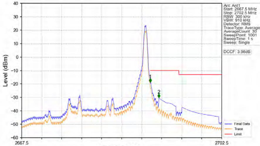
Band41_15MHz_16QAM_HCH_2682.5MHz_RB_1_74_NTNV
