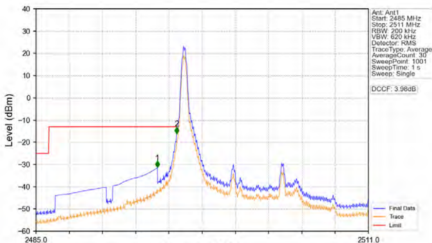
Band41_10MHz_64QAM_LCH_2501MHz_RB_1_0_NTNV
