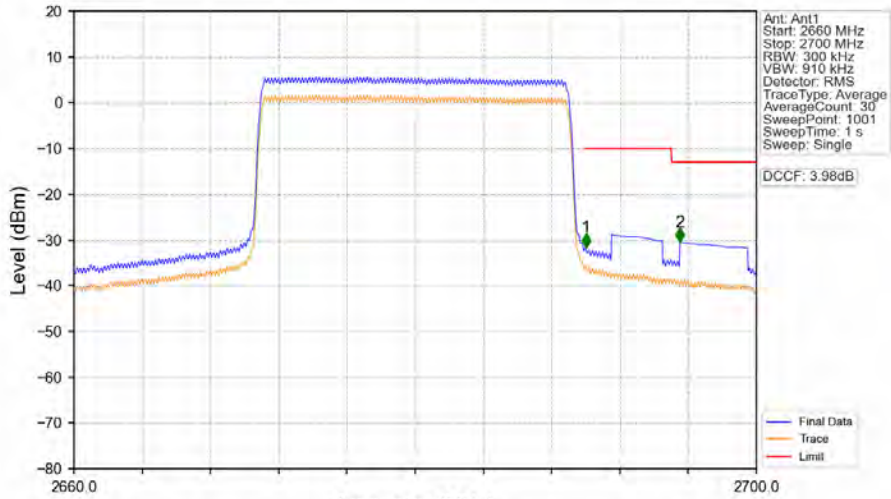
Band41_20MHz_64QAM_HCH_2680MHz_RB_100_0_NTNV
