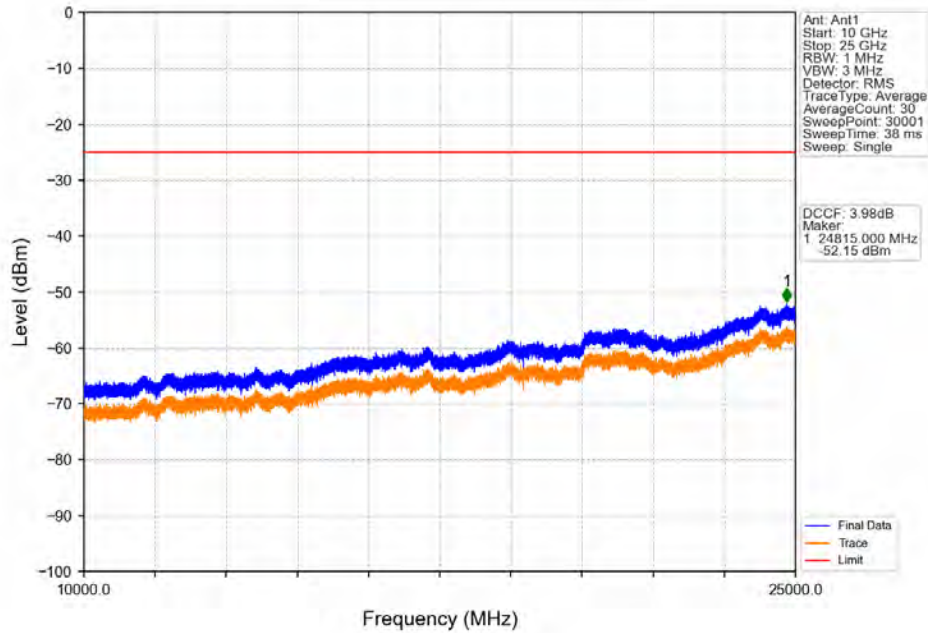
Band41_10MHz_64QAM_MCH_2593MHz_RB_1_0_NTNV
