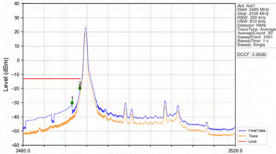
Band41_20MHz_64QAM_LCH_2506MHz_RB_1_0_NTNV
