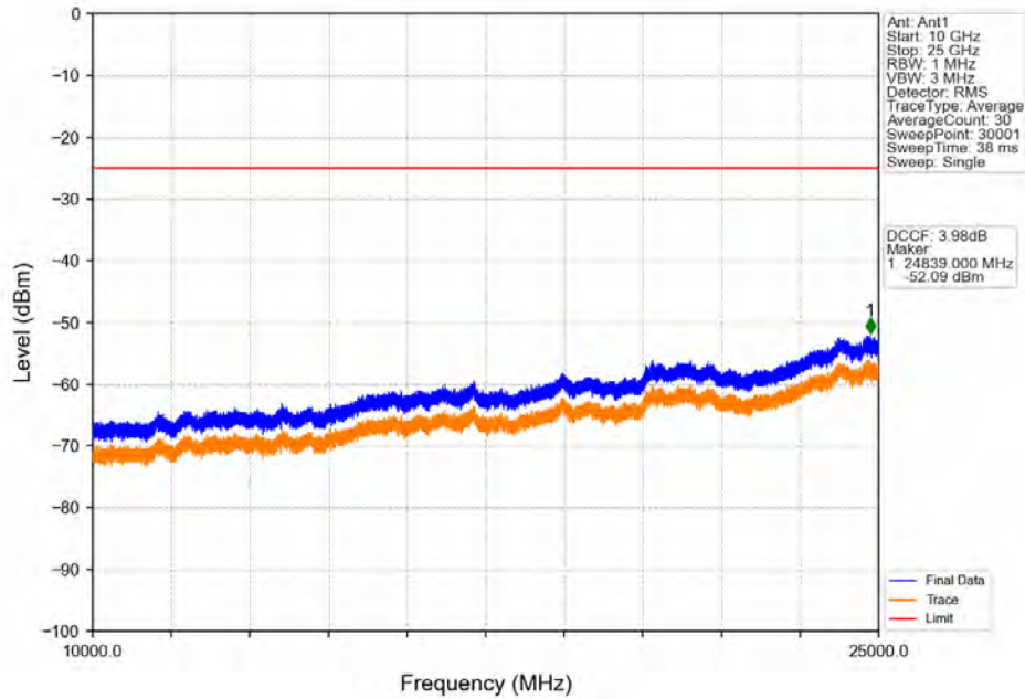
Band41_10MHz_64QAM_HCH_2685MHz_RB_1_0_NTNV
