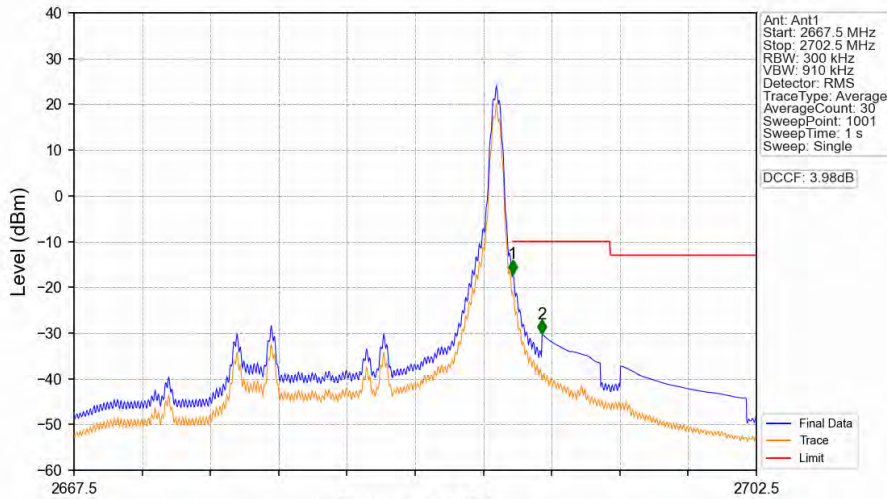
Band41_15MHz_64QAM_HCH_2682.5MHz_RB_1_74_NTNV
