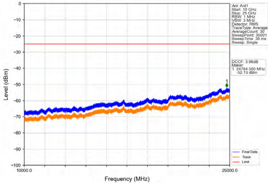
Band41_20MHz_64QAM_HCH_2680MHz_RB_1_0_NTNV
