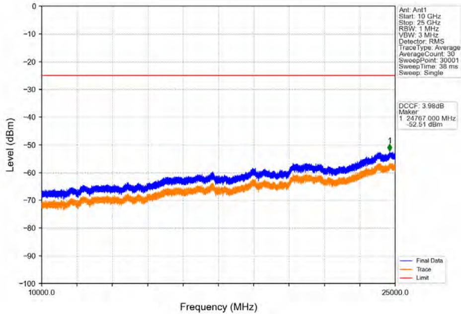
Band41_15MHz_64QAM_MCH_2593MHz_RB_1_0_NTNV
