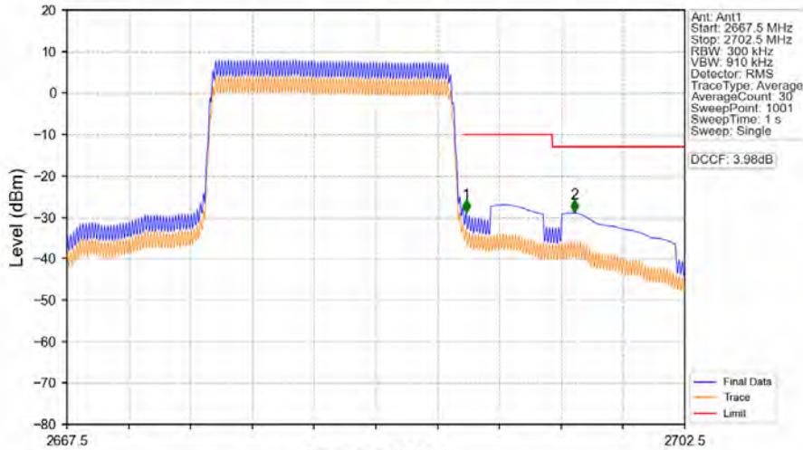
Band41_15MHz_16QAM_HCH_2682.5MHz_RB_75_0_NTNV
