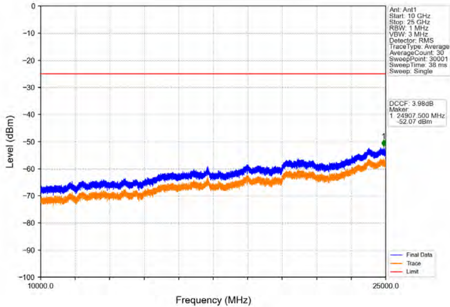
Band41_20MHz_64QAM_LCH_2506MHz_RB_1_0_NTNV
