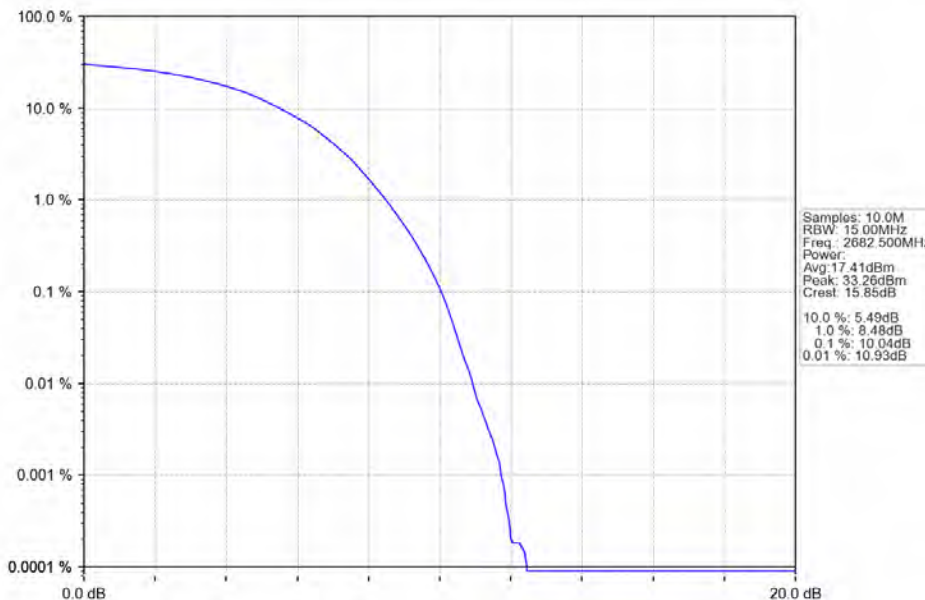
Band41_15MHz_64QAM_HCH_2682.5MHz_RB_75_0_NTNV
