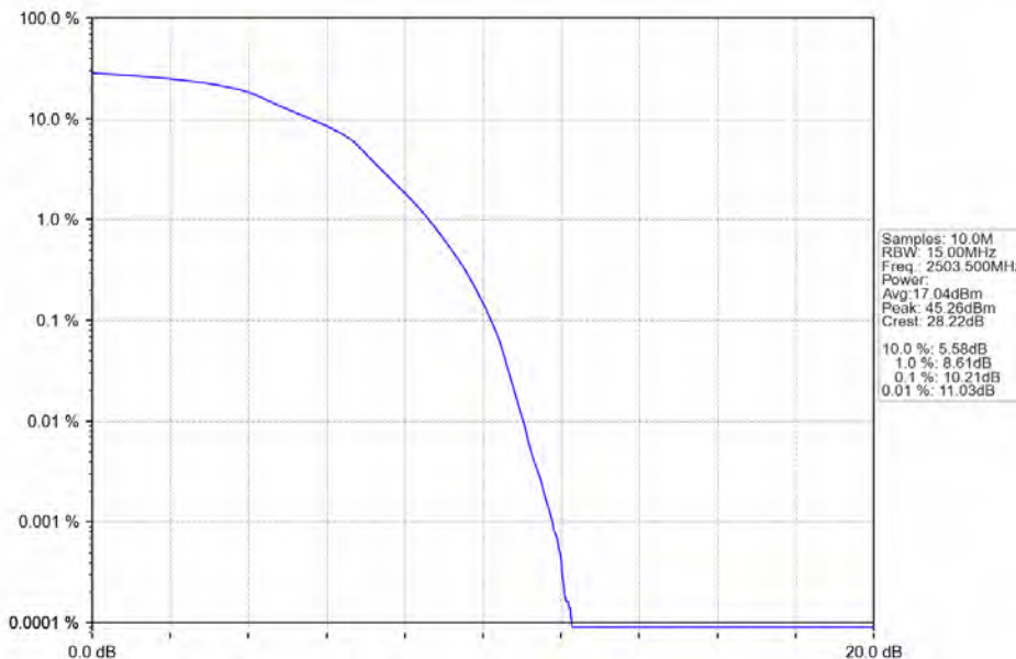
Band41_15MHz_16QAM_LCH_2503.5MHz_RB_75_0_NTNV
