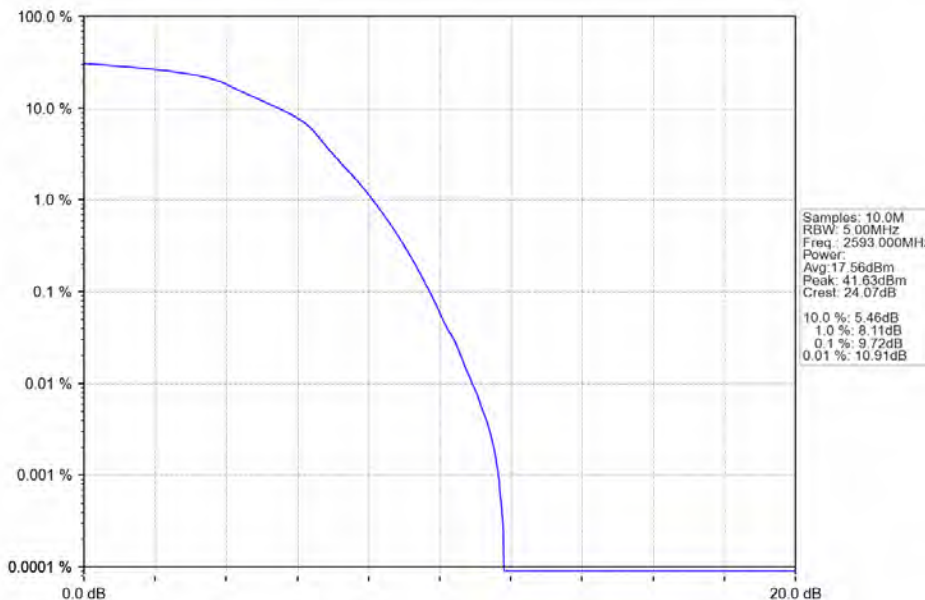
Band41_5MHz_16QAM_MCH_2593MHz_RB_25_0_NTNV
