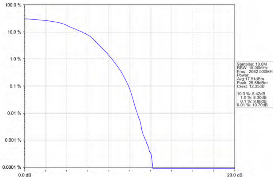
Band41_15MHz_16QAM_HCH_2682.5MHz_RB_75_0_NTNV
