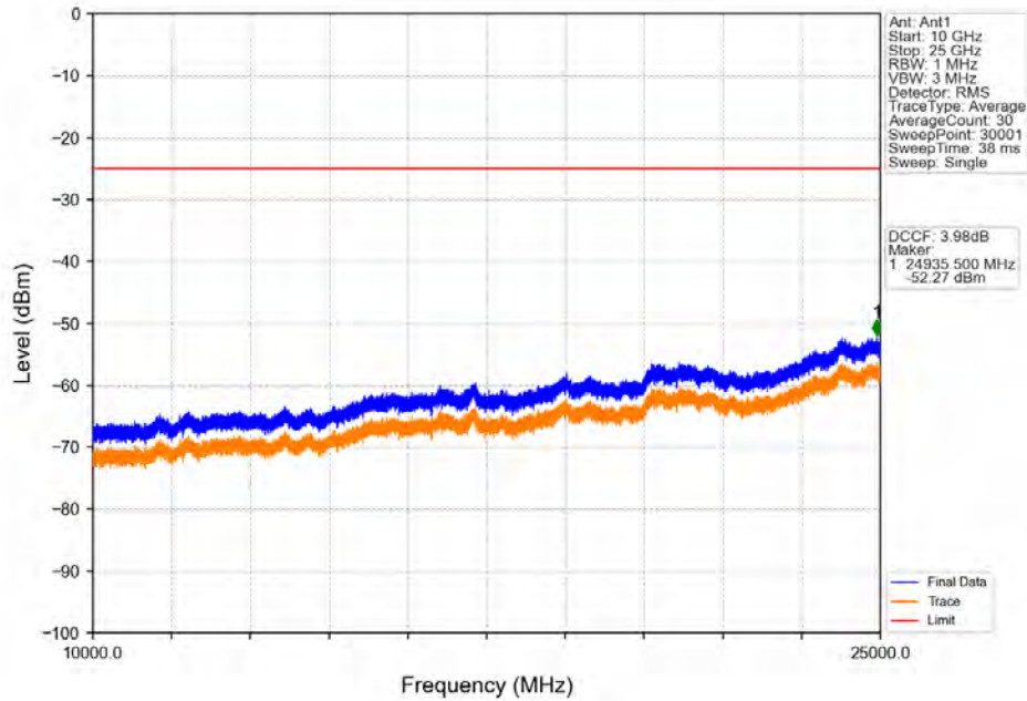
Band41_5MHz_64QAM_MCH_2593MHz_RB_1_0_NTNV
