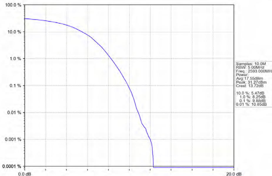
Band41_5MHz_64QAM_MCH_2593MHz_RB_25_0_NTNV
