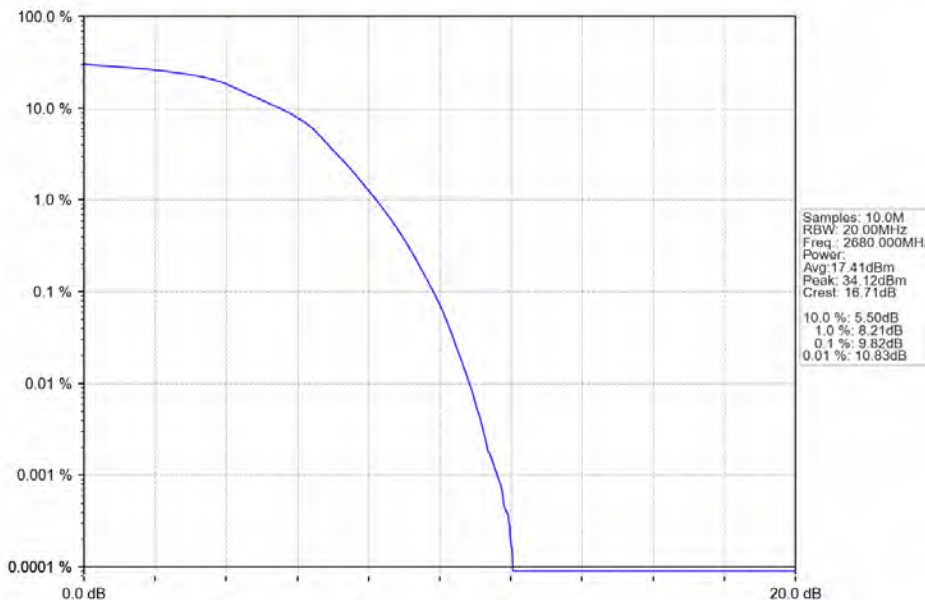
Band41_20MHz_16QAM_HCH_2680MHz_RB_100_0_NTNV
