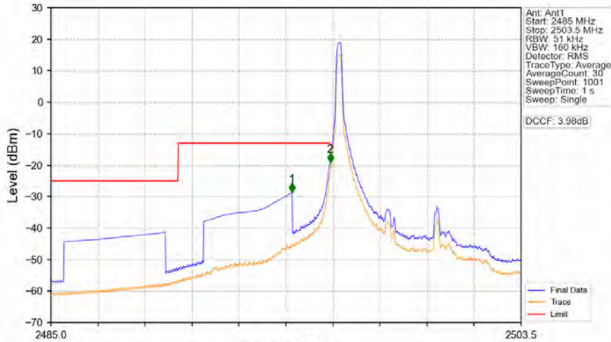
Band41_5MHz_16QAM_LCH_2498.5MHz_RB_1_0_NTNV
