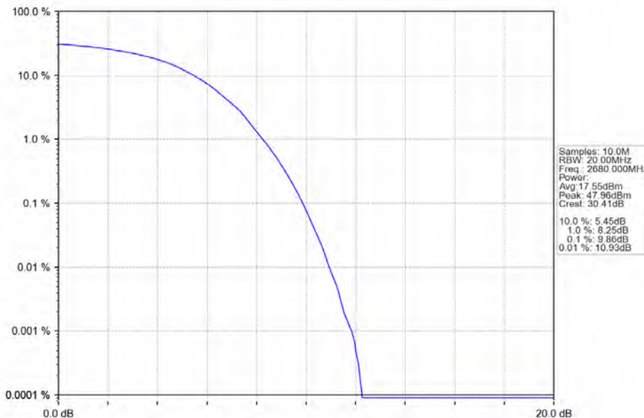
Band41_20MHz_64QAM_HCH_2680MHz_RB_100_0_NTNV
