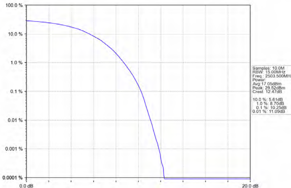
Band41_15MHz_64QAM_LCH_2503.5MHz_RB_75_0_NTNV
