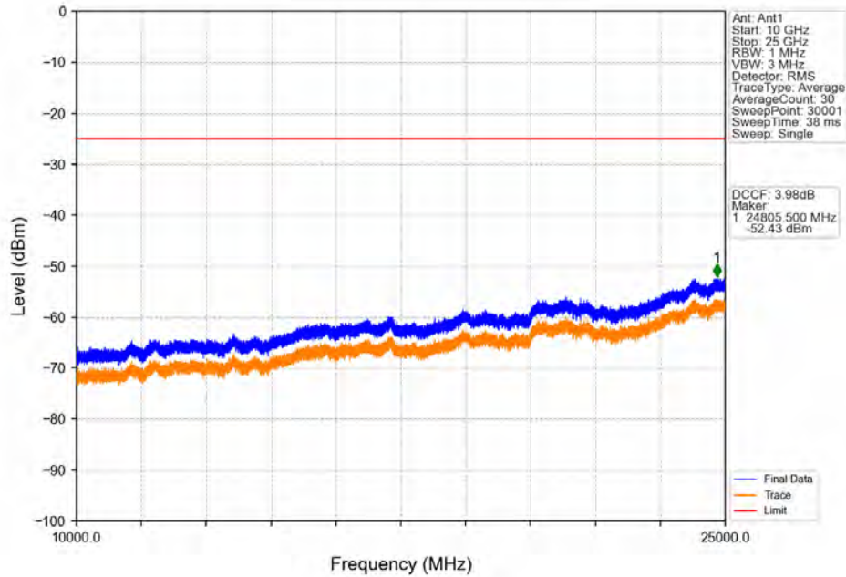
Band41_5MHz_16QAM_MCH_2593MHz_RB_1_0_NTNV
