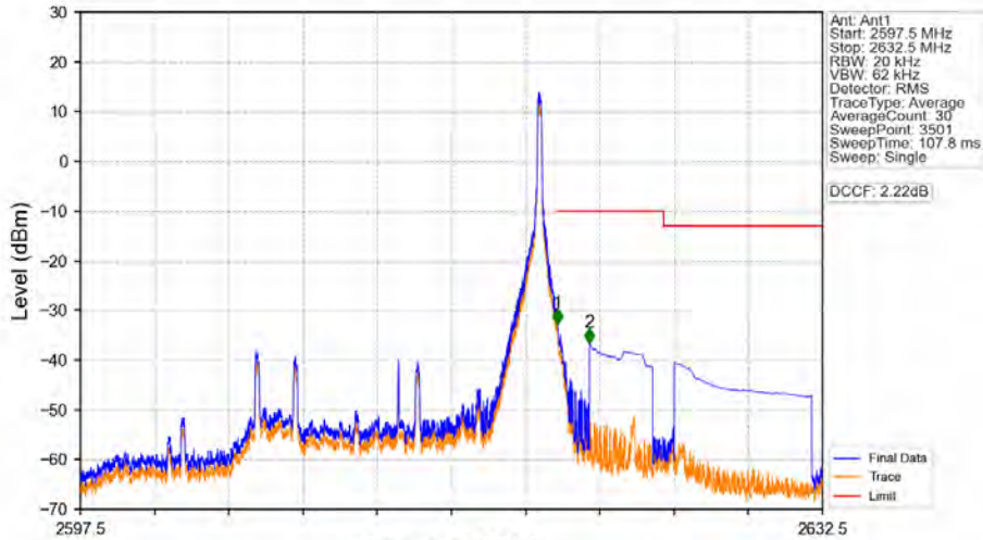
Band38_15MHz_64QAM_HCH_2612.5MHz_RB_1_74_NTNV
