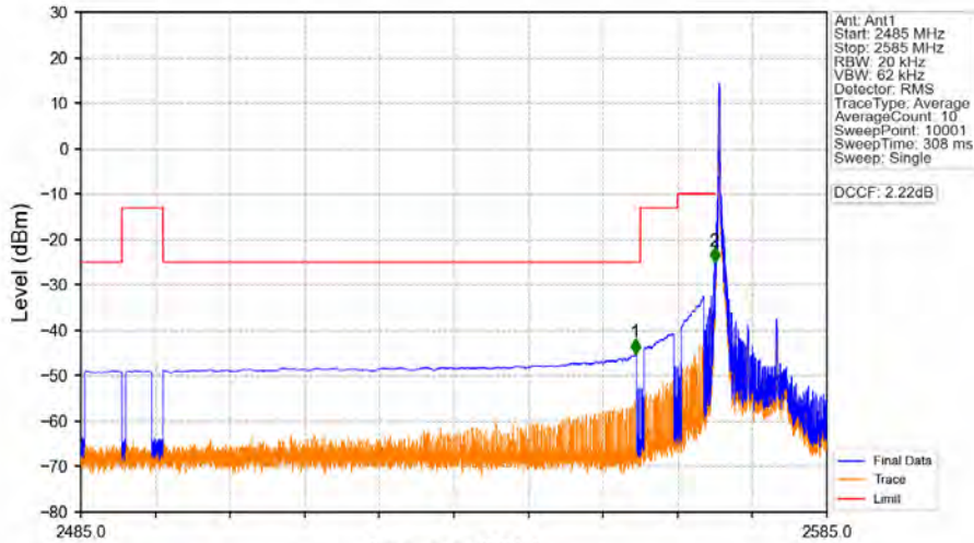
Band38_10MHz_64QAM_LCH_2575MHz_RB_1_0_NTNV
