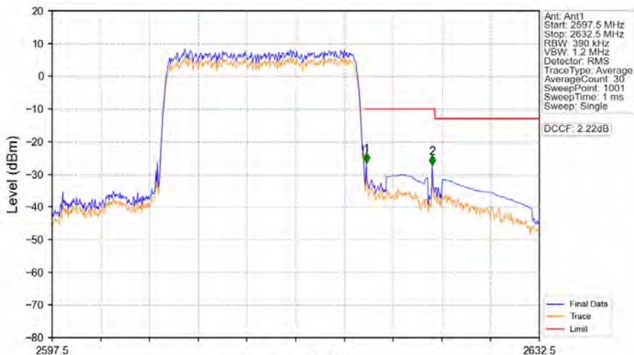
Band38_15MHz_16QAM_HCH_2612.5MHz_RB_75_0_NTNV
