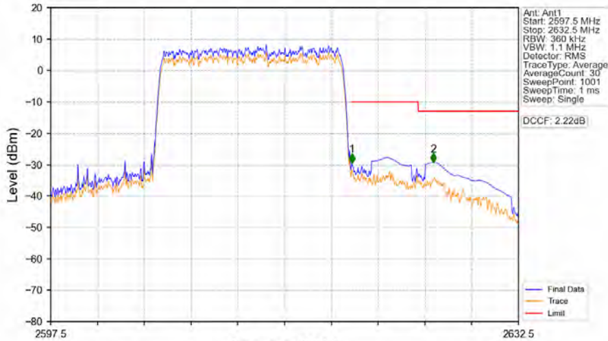
Band38_15MHz_64QAM_HCH_2612.5MHz_RB_75_0_NTNV
