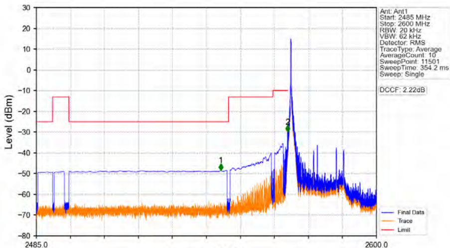
Band38_20MHz_64QAM_LCH_2580MHz_RB_1_0_NTNV
