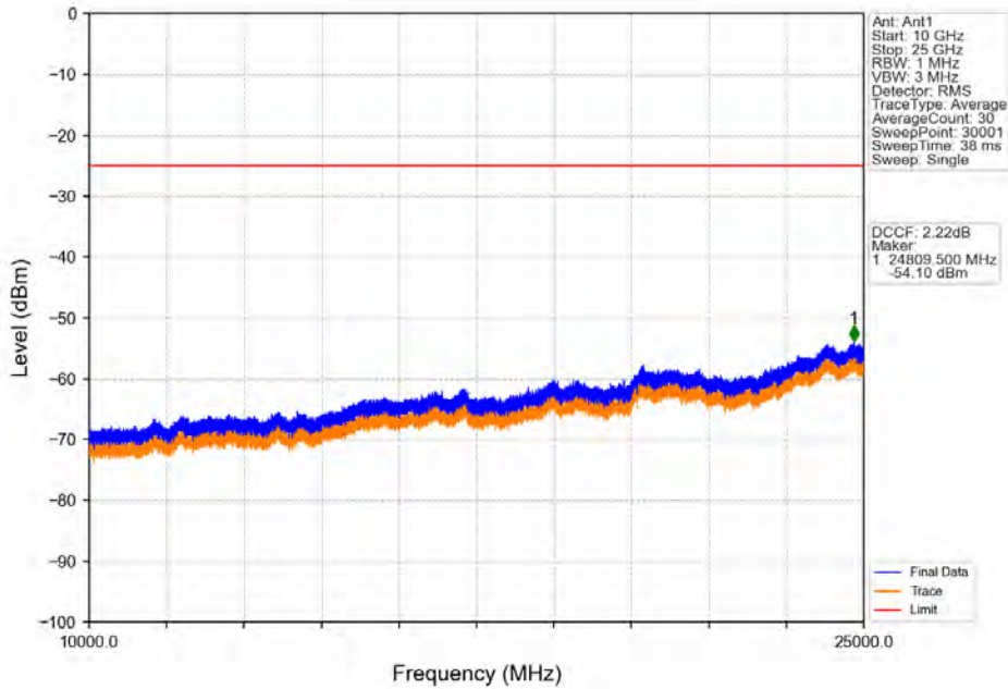
Band38_10MHz_64QAM_HCH_2615MHz_RB_1_0_NTNV
