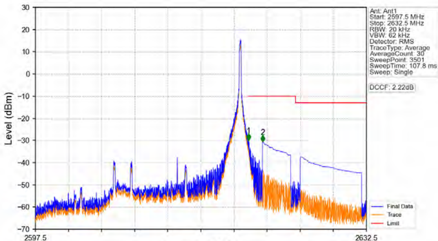
Band38_15MHz_16QAM_HCH_2612.5MHz_RB_1_74_NTNV
