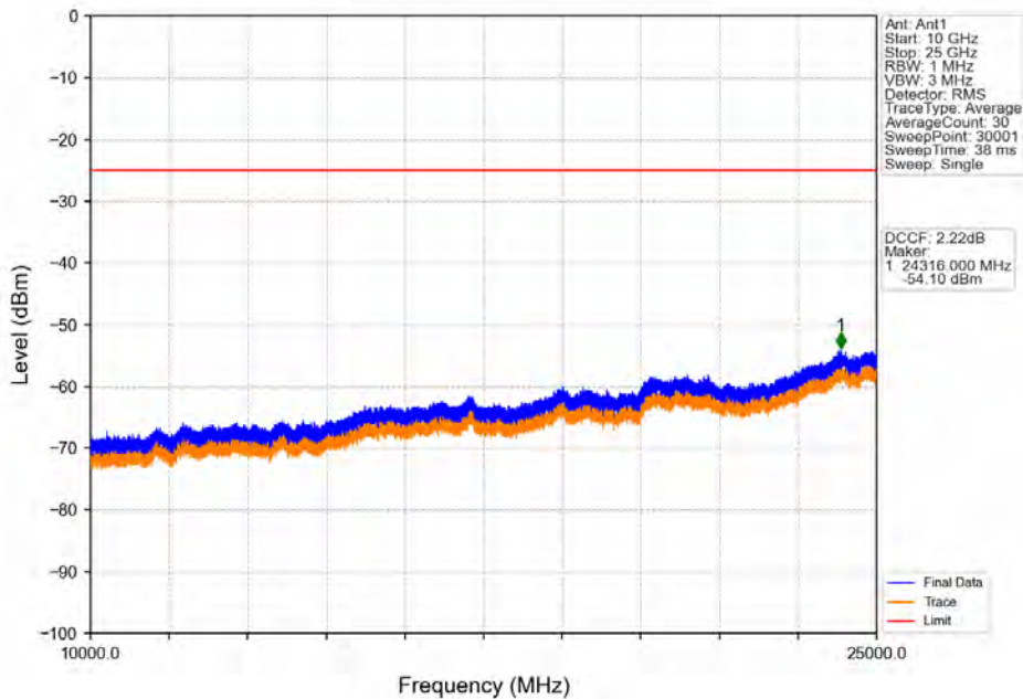
Band38_20MHz_64QAM_MCH_2595MHz_RB_1_0_NTNV
