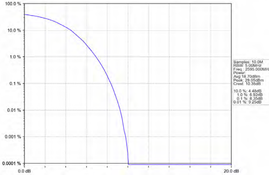
Band38_5MHz_64QAM_MCH_2595MHz_RB_25_0_NTNV
