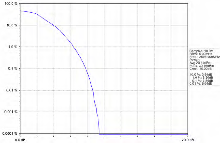
Band38_5MHz_QPSK_MCH_2595MHz_RB_25_0_NTNV
