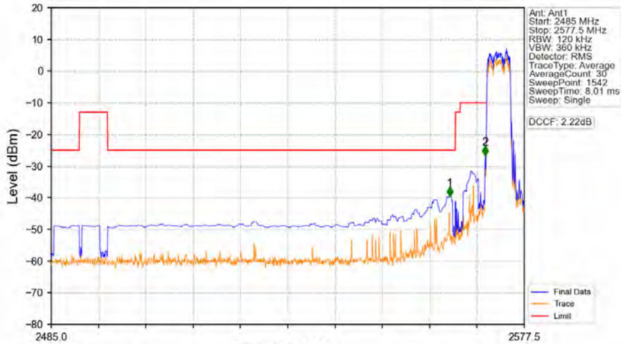
Band38_5MHz_QPSK_LCH_2572.5MHz_RB_25_0_NTNV
