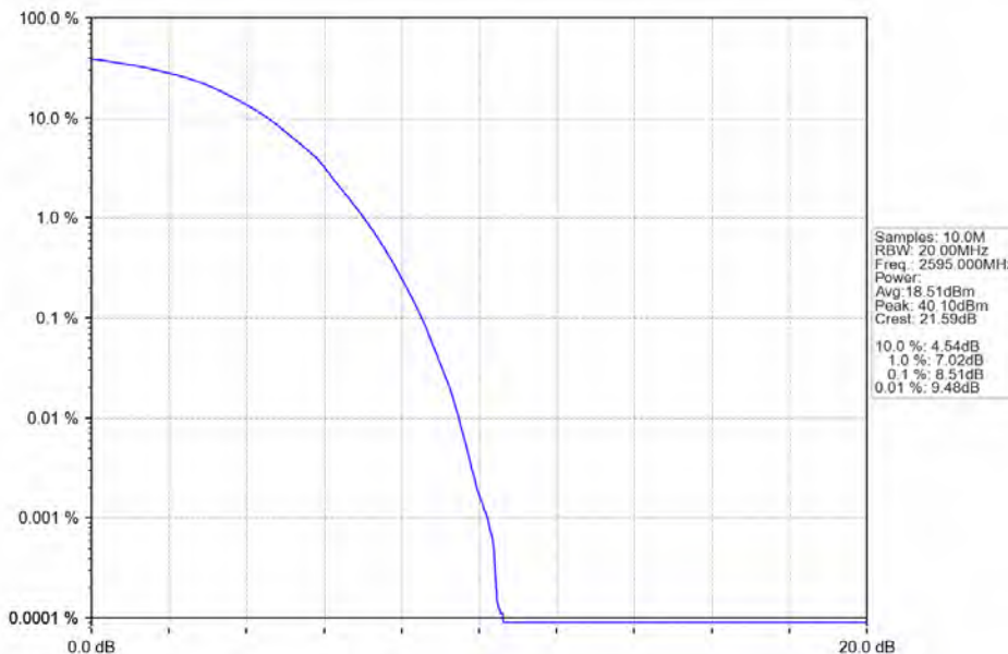
Band38_20MHz_64QAM_MCH_2595MHz_RB_100_0_NTNV
