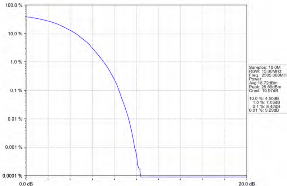
Band38_15MHz_64QAM_MCH_2595MHz_RB_75_0_NTNV
