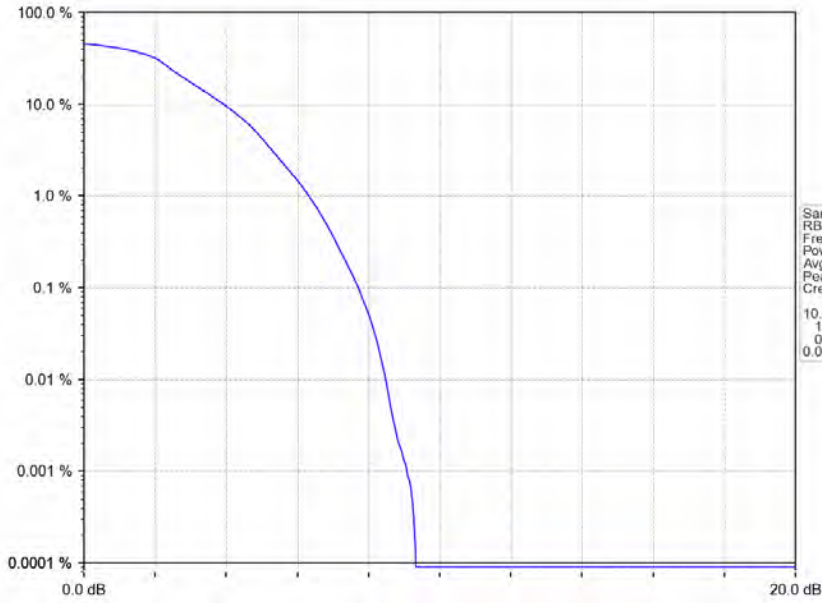
Band38_5MHz_QPSK_HCH_2617.5MHz_RB_25_0_NTNV
