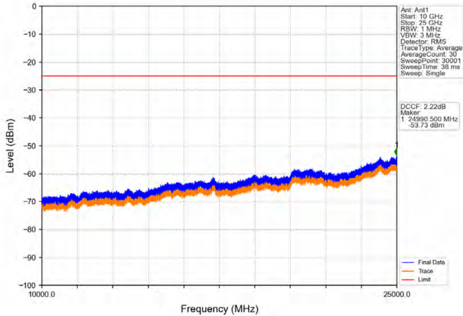
Band38_5MHz_16QAM_LCH_2572.5MHz_RB_1_0_NTNV
