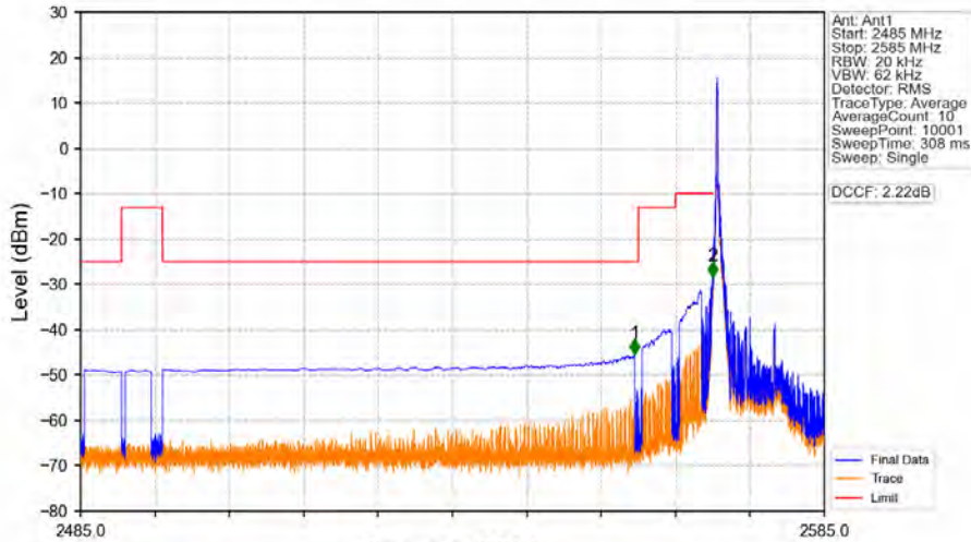
Band38_10MHz_16QAM_LCH_2575MHz_RB_1_0_NTNV
