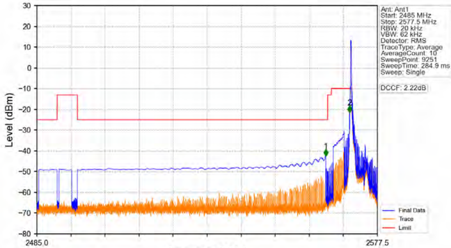
Band38_5MHz_16QAM_LCH_2572.5MHz_RB_1_0_NTNV
