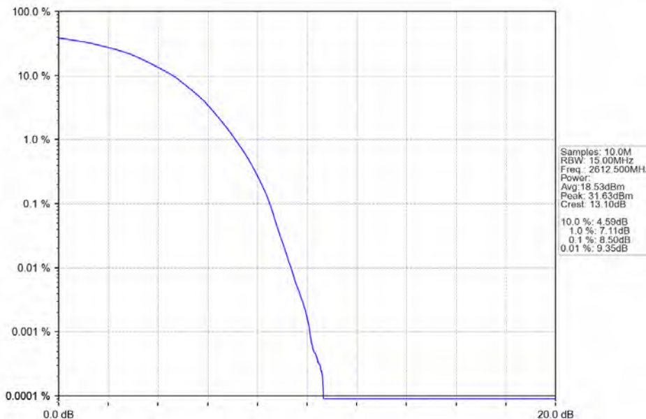
Band38_15MHz_64QAM_HCH_2612.5MHz_RB_75_0_NTNV
