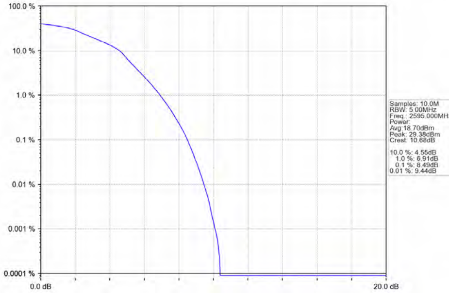
Band38_5MHz_16QAM_MCH_2595MHz_RB_25_0_NTNV
