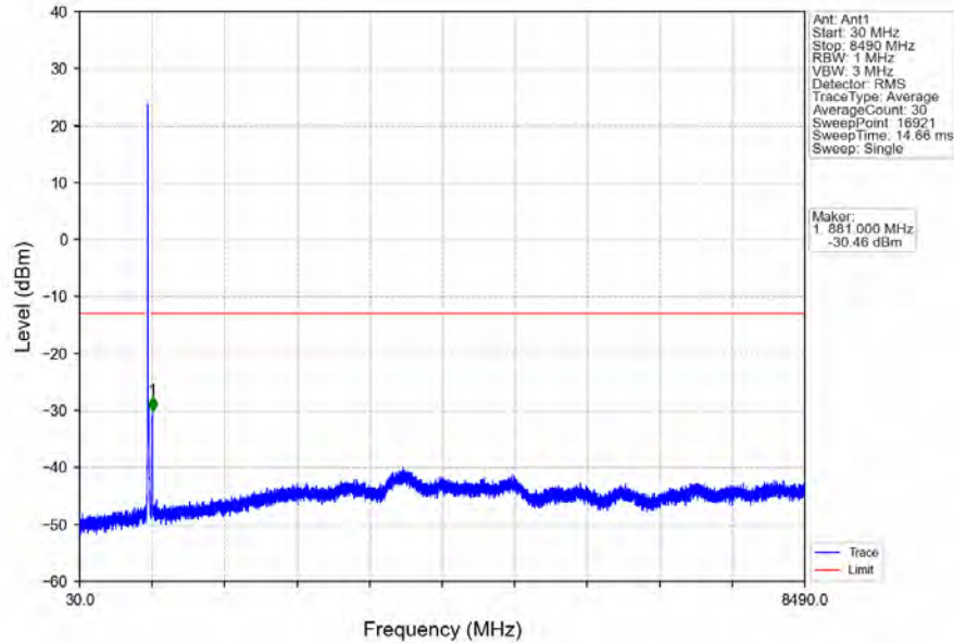
Band26b_15MHz_16QAM_LCH_831.5MHz_RB_75_0_NTNV
