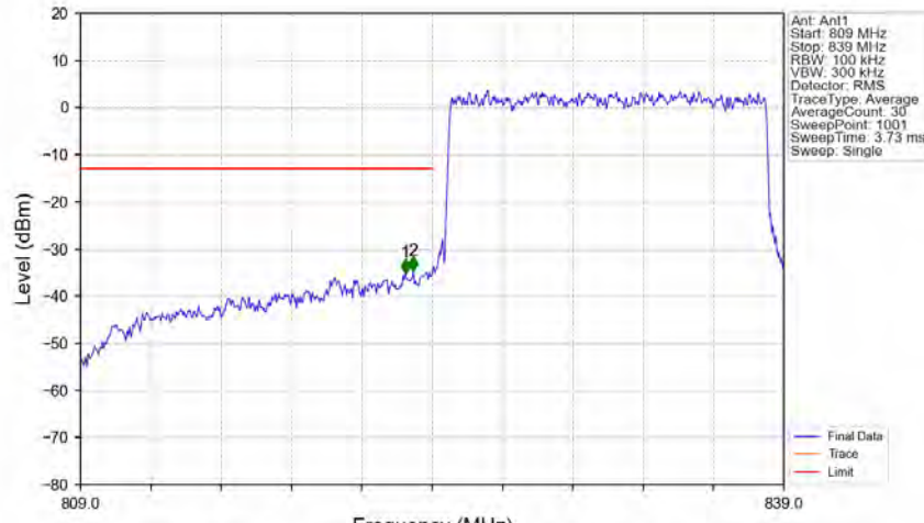
Band26b_15MHz_64QAM_LCH_831.5MHz_RB_75_0_NTNV
