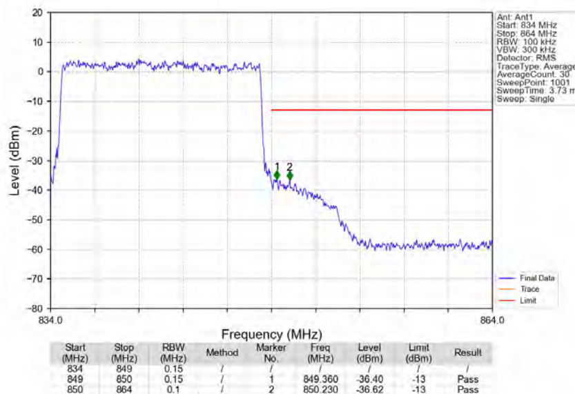
Band26b_15MHz_16QAM_HCH_841.5MHz_RB_75_0_NTNV
