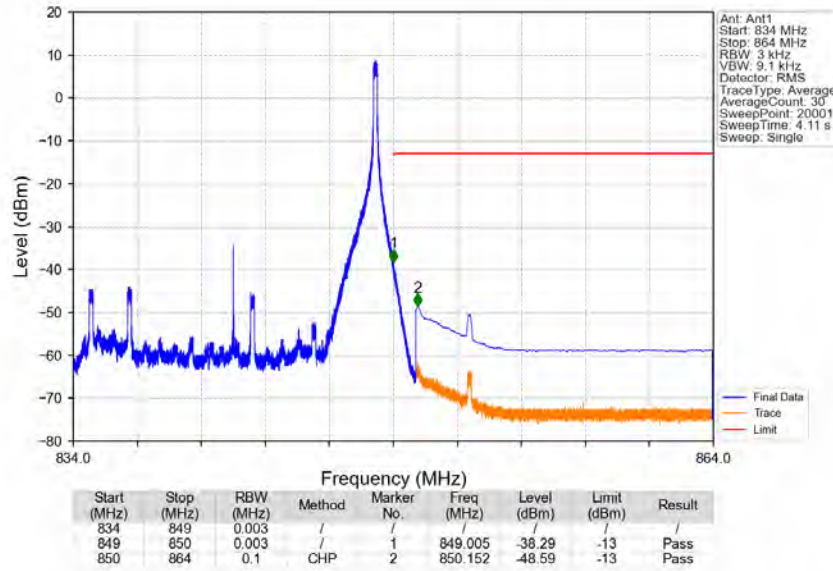
Band26b_15MHz_16QAM_HCH_841.5MHz_RB_1_74_NTNV
