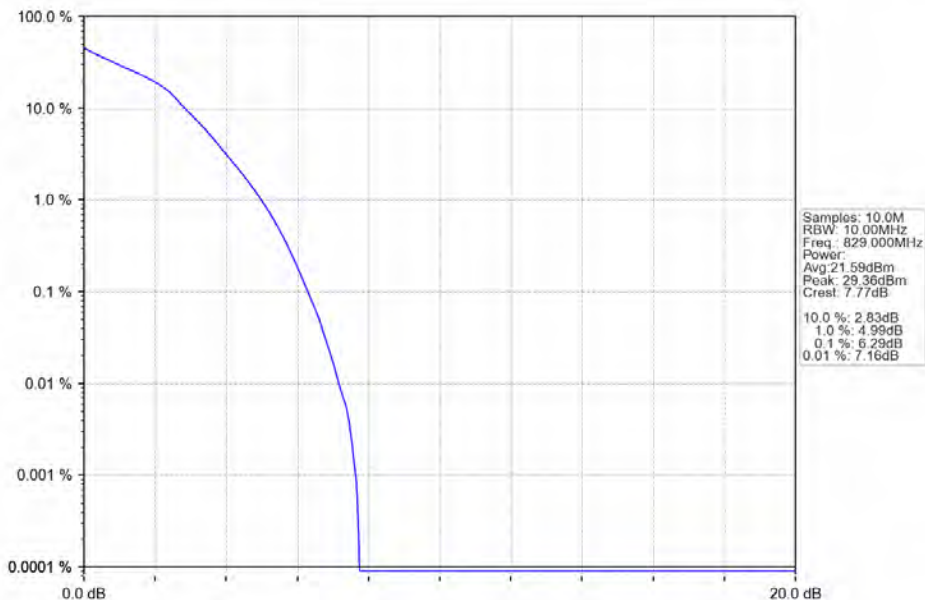
Band26b_10MHz_16QAM_LCH_829MHz_RB_50_0_NTNV
