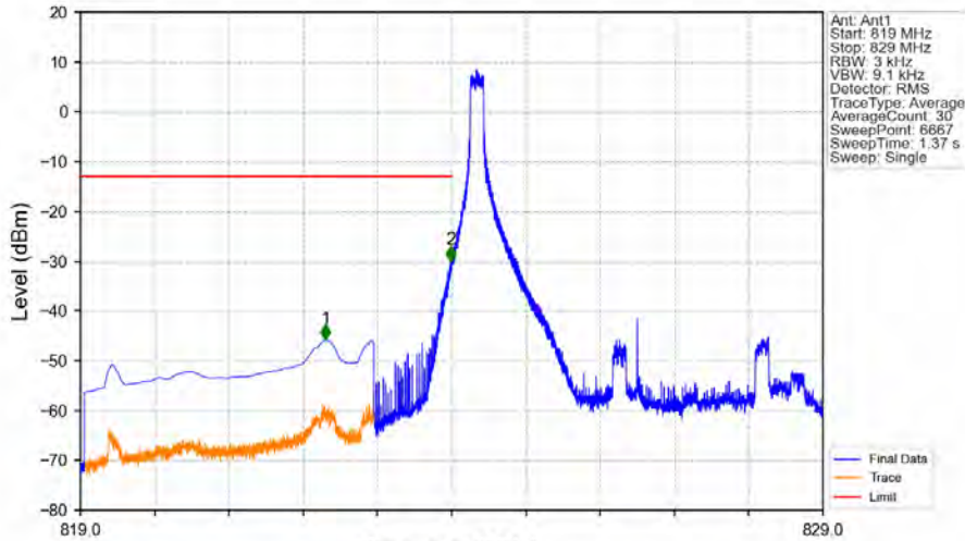
Band26b_5MHz_16QAM_LCH_826.5MHz_RB_1_0_NTNV
