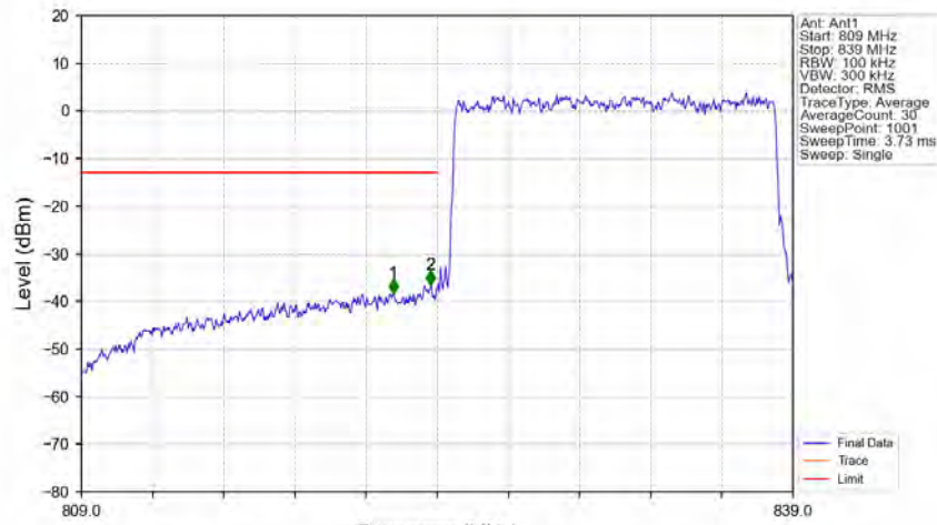
Band26b_15MHz_16QAM_LCH_831.5MHz_RB_75_0_NTNV
