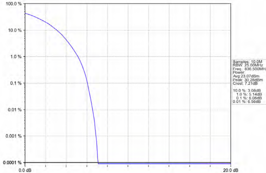
Band26b_15MHz_64QAM_MCH_836.5MHz_RB_75_0_NTNV
