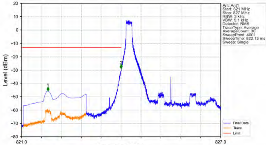
Band26b_3MHz_64QAM_LCH_825.5MHz_RB_1_0_NTNV
