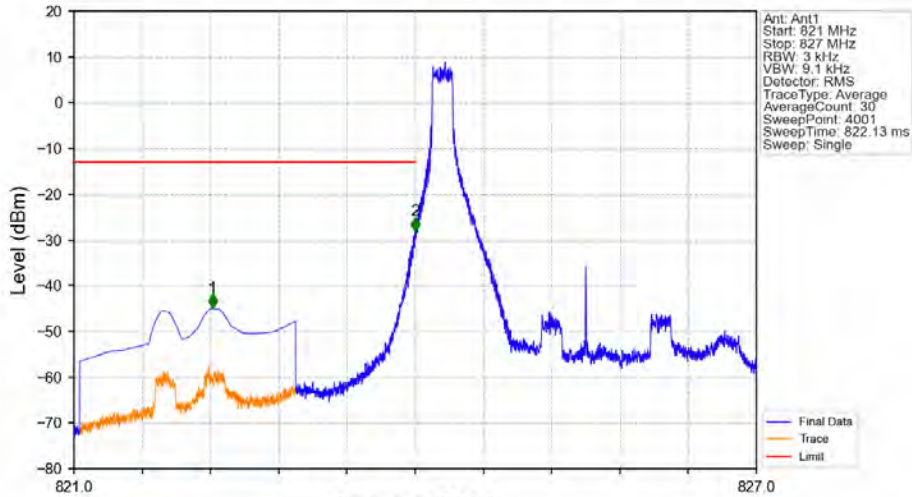
Band26b_3MHz_16QAM_LCH_825.5MHz_RB_1_0_NTNV
