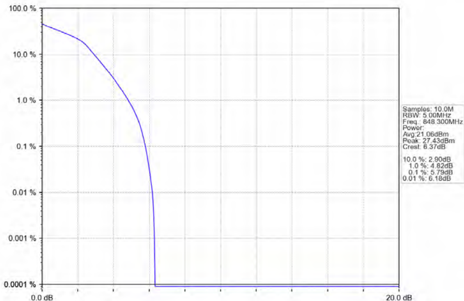
Band26b_1.4MHz_16QAM_HCH_848.3MHz_RB_6_0_NTNV
