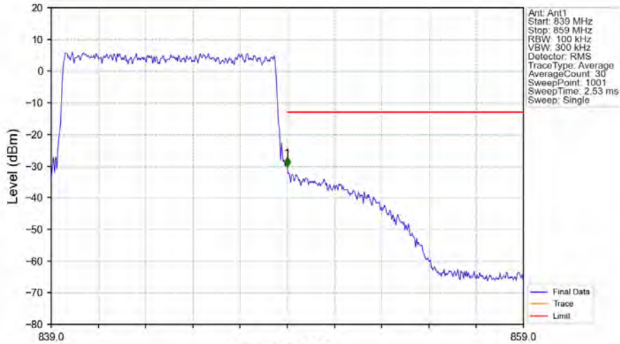
Band26b_10MHz_QPSK_HCH_844MHz_RB_50_0_NTNV
