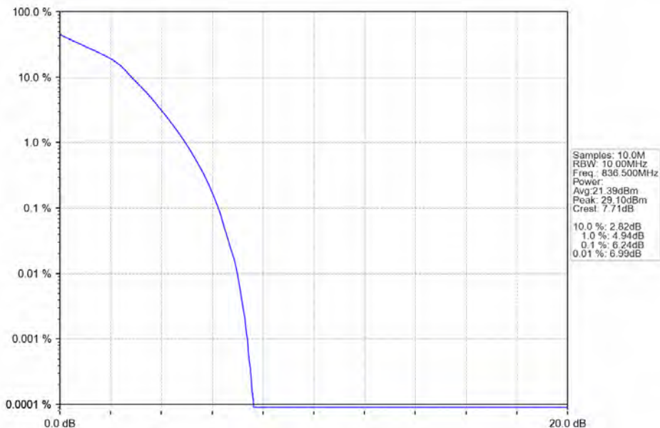
Band26b_10MHz_16QAM_MCH_836.5MHz_RB_50_0_NTNV
