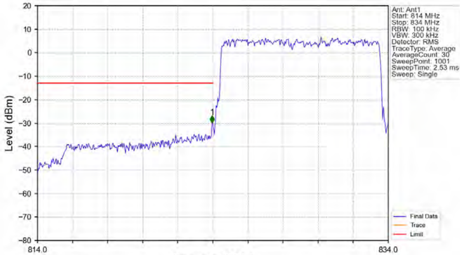
Band26b_10MHz_QPSK_LCH_829MHz_RB_50_0_NTNV
