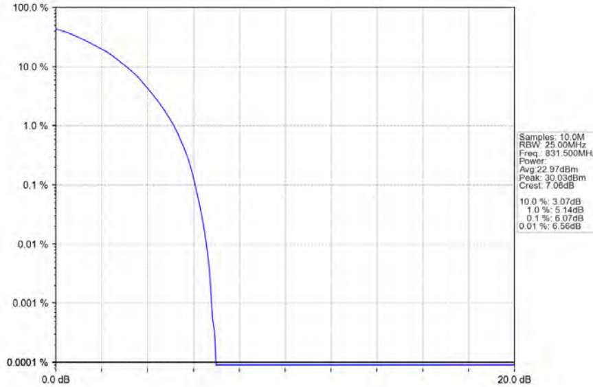
Band26b_15MHz_64QAM_LCH_831.5MHz_RB_75_0_NTNV
