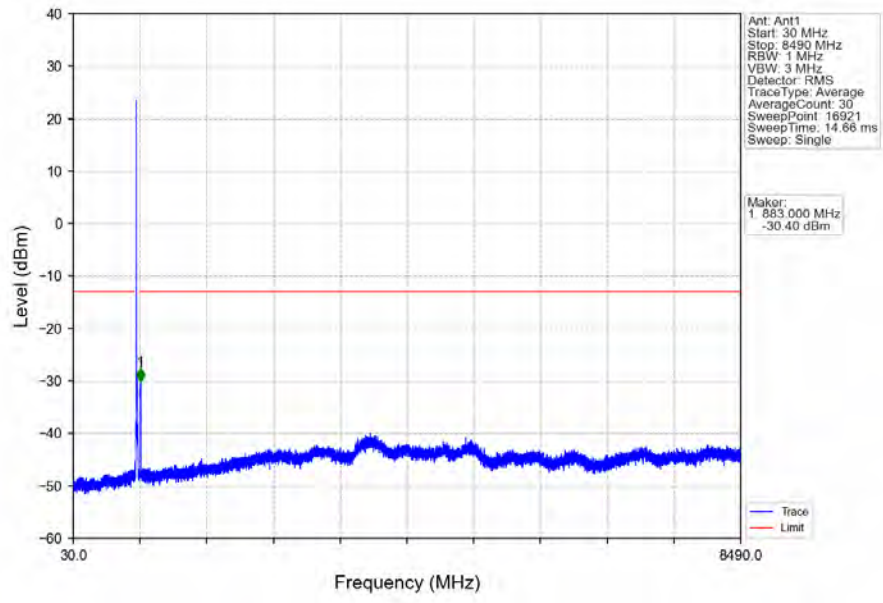
Band26b_15MHz_64QAM_MCH_836.5MHz_RB_1_0_NTNV
