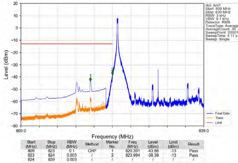
Band26b_15MHz_64QAM_LCH_831.5MHz_RB_1_0_NTNV
