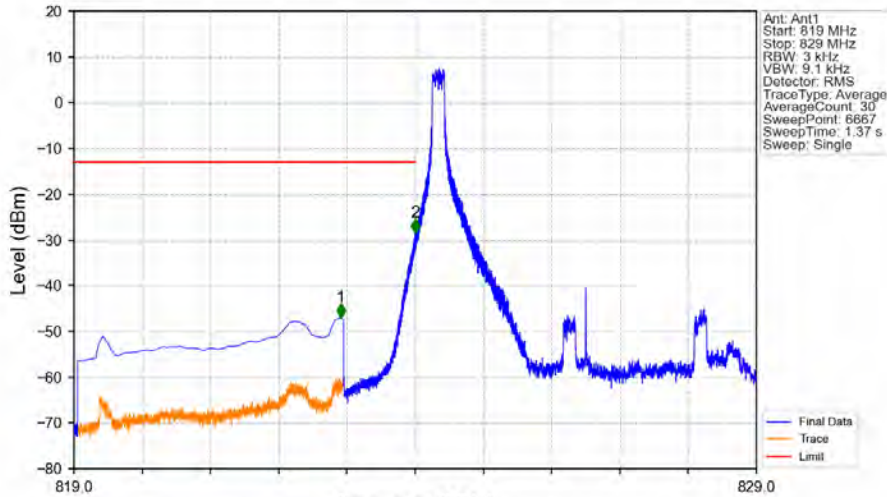
Band26b_5MHz_64QAM_LCH_826.5MHz_RB_1_0_NTNV
