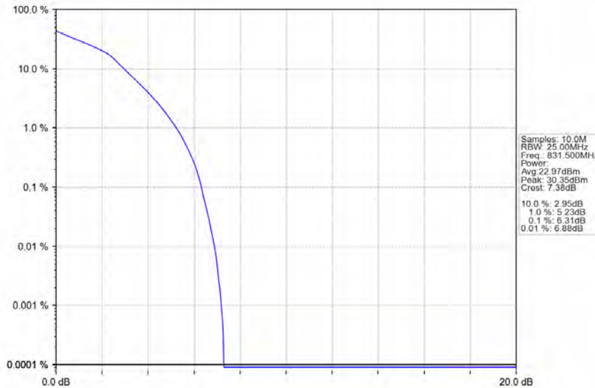
Band26b_15MHz_16QAM_LCH_831.5MHz_RB_75_0_NTNV
