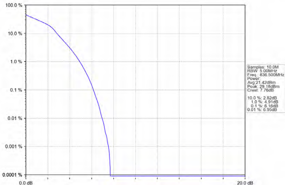
Band26b_5MHz_16QAM_MCH_836.5MHz_RB_25_0_NTNV
