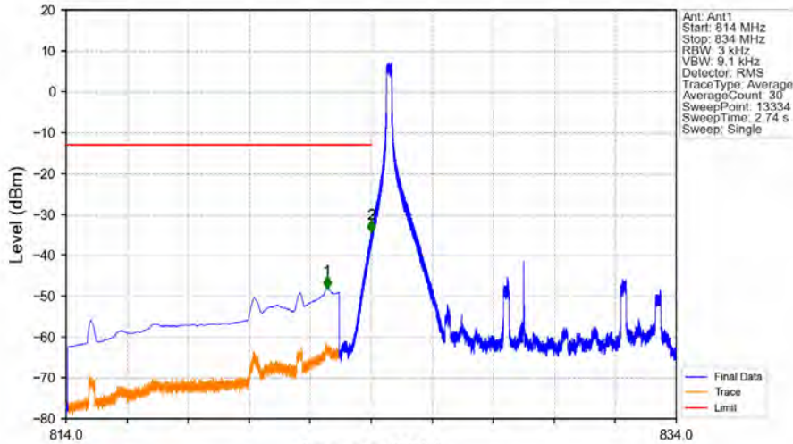
Band26b_10MHz_64QAM_LCH_829MHz_RB_1_0_NTNV
