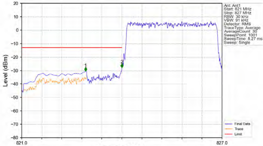
Band26b_3MHz_QPSK_LCH_825.5MHz_RB_15_0_NTNV
