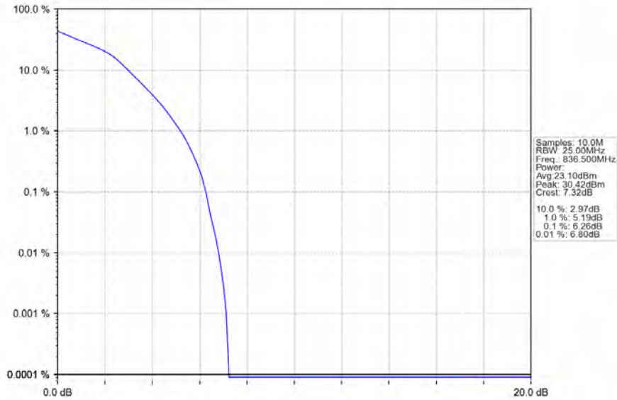
Band26b_15MHz_16QAM_MCH_836.5MHz_RB_75_0_NTNV
