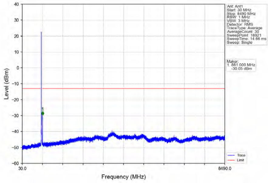
Band26b_15MHz_64QAM_LCH_831.5MHz_RB_1_0_NTNV
