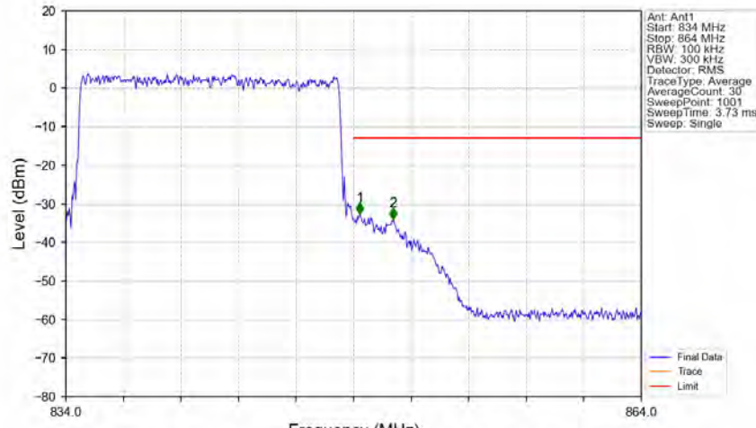
Band26b_15MHz_64QAM_HCH_841.5MHz_RB_75_0_NTNV
