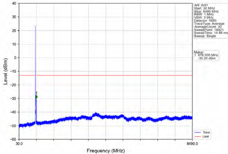
Band26b_15MHz_16QAM_HCH_841.5MHz_RB_1_0_NTNV
