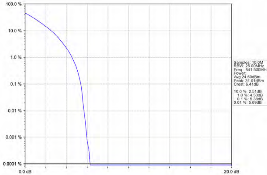
Band26b_15MHz_QPSK_HCH_841.5MHz_RB_75_0_NTNV
