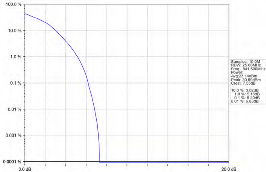
Band26b_15MHz_16QAM_HCH_841.5MHz_RB_75_0_NTNV
