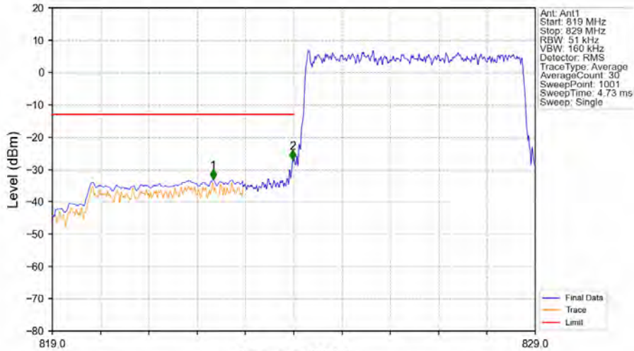
Band26b_5MHz_QPSK_LCH_826.5MHz_RB_25_0_NTNV
