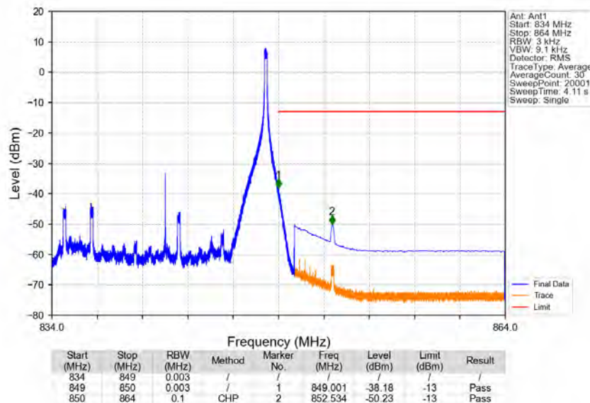
Band26b_15MHz_64QAM_HCH_841.5MHz_RB_1_74_NTNV
