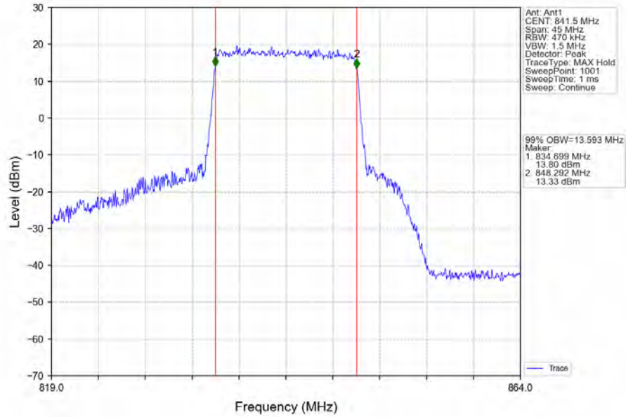
Band26b_15MHz_64QAM_HCH_841.5MHz_RB_75_0_NTNV
