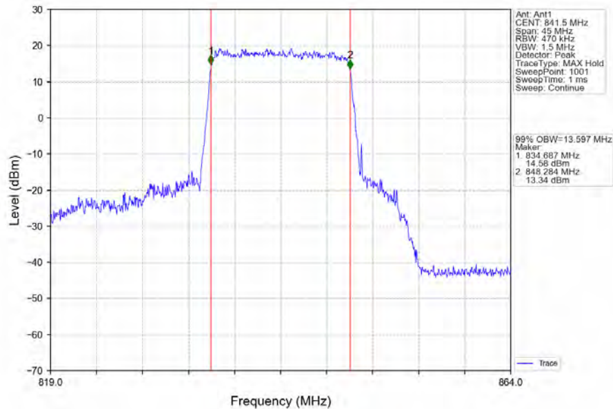
Band26b_15MHz_16QAM_HCH_841.5MHz_RB_75_0_NTNV
