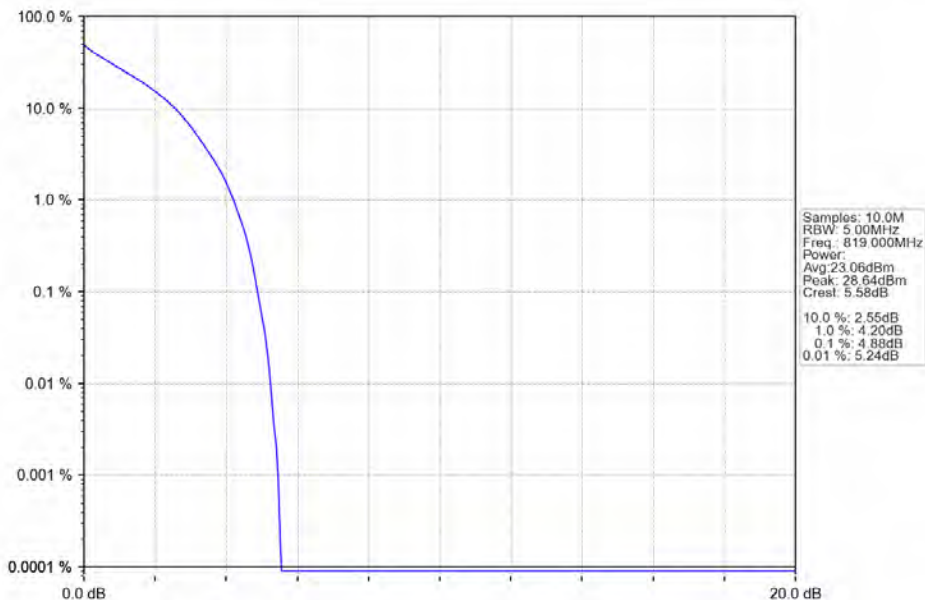
Band26a_1.4MHz_QPSK_MCH_819MHz_RB_6_0_NTNV
