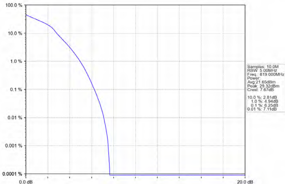
Band26a_5MHz_16QAM_MCH_819MHz_RB_25_0_NTNV
