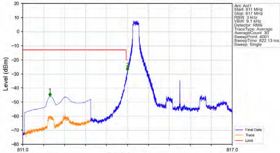
Band26a_3MHz_16QAM_LCH_815.5MHz_RB_1_0_NTV
