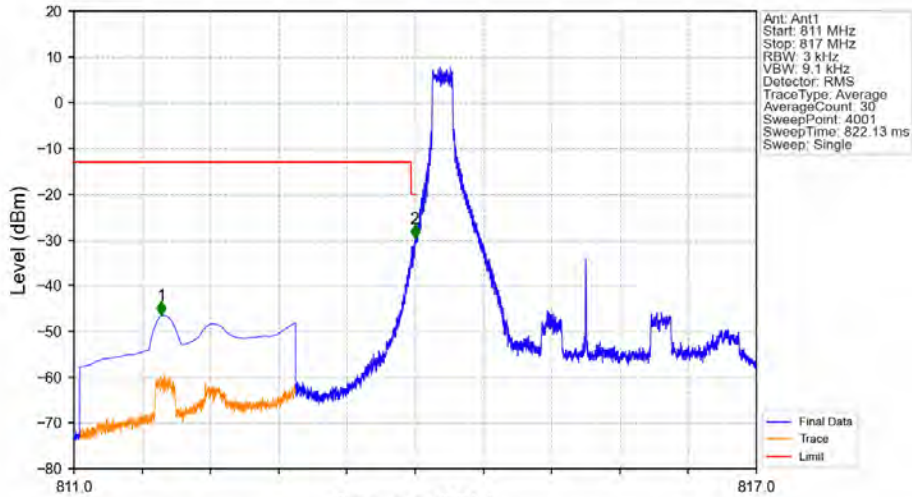
Band26a_3MHz_64QAM_LCH_815.5MHz_RB_1_0_NTV
