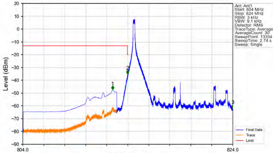
Band26a_10MHz_16QAM_LCH_819MHz_RB_1_0_NTNV
