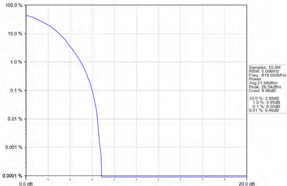
Band26a_3MHz_64QAM_MCH_819MHz_RB_15_0_NTNV
