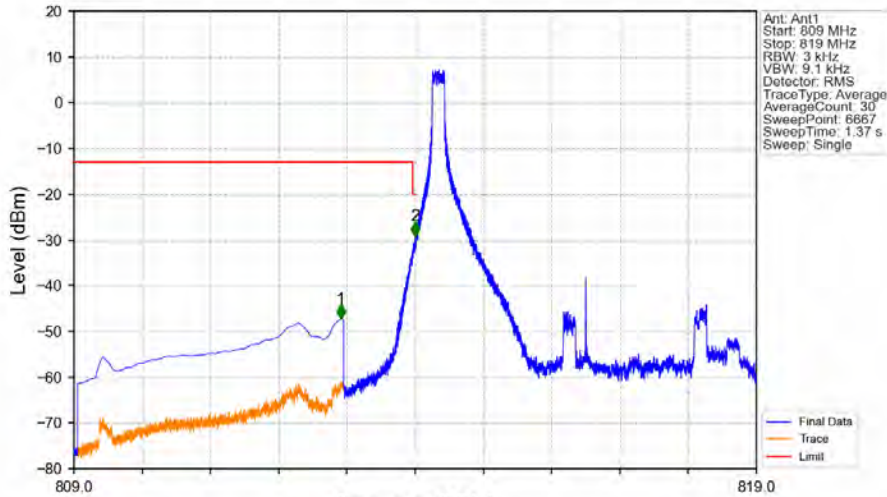
Band26a_5MHz_64QAM_LCH_816.5MHz_RB_1_0_NTV
