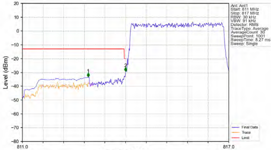
Band26a_3MHz_QPSK_LCH_815.5MHz_RB_15_0_NTV
