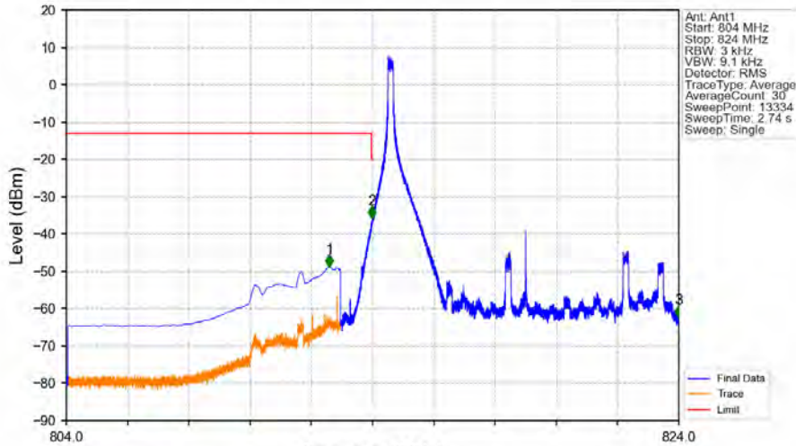
Band26a_10MHz_64QAM_LCH_819MHz_RB_1_0_NTNV
