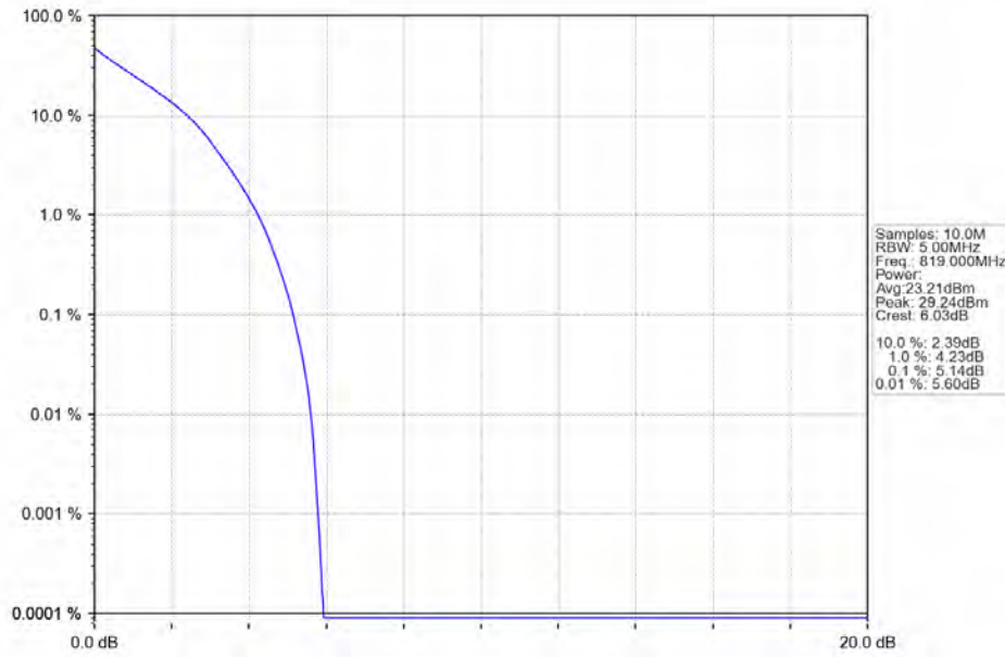
Band26a_3MHz_QPSK_MCH_819MHz_RB_15_0_NTNV
