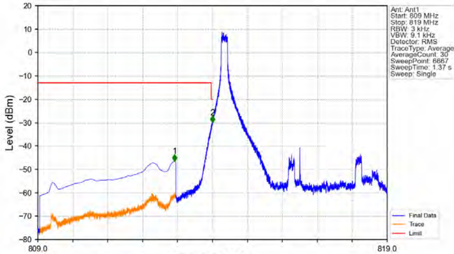
Band26a_5MHz_16QAM_LCH_816.5MHz_RB_1_0_NTV
