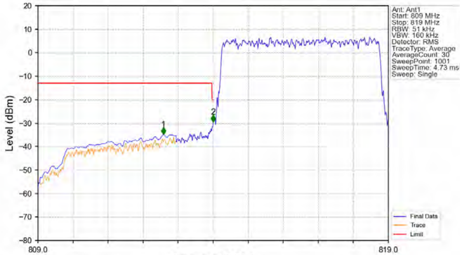
Band26a_5MHz_QPSK_LCH_816.5MHz_RB_25_0_NTNV
