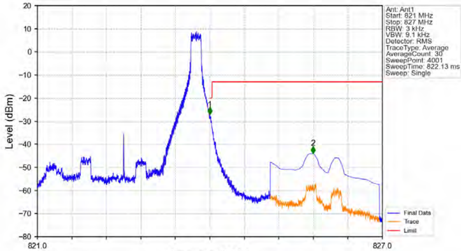
Band26a_3MHz_QPSK_HCH_822.5MHz_RB_1_14_NTNV
