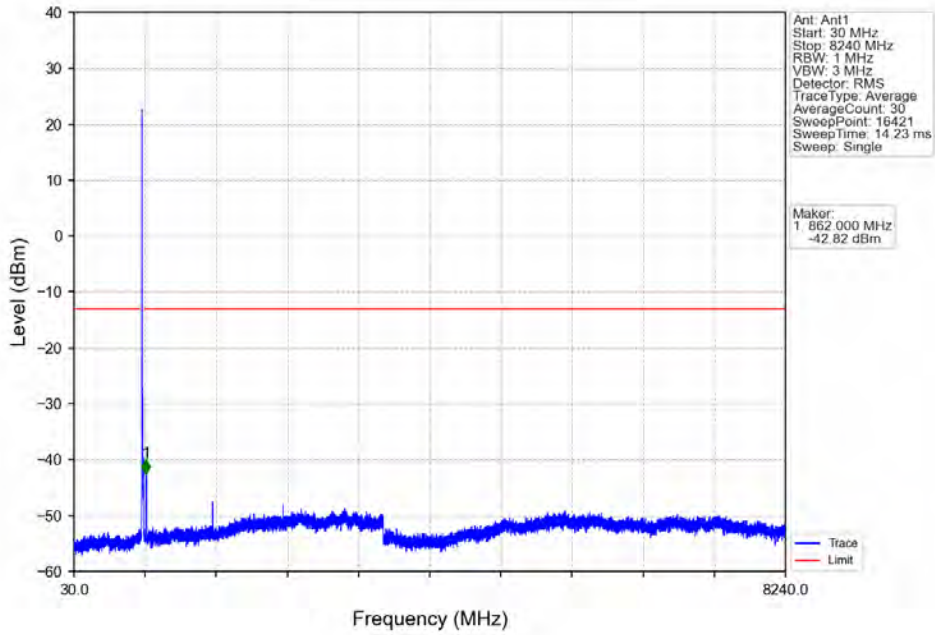
Band26a_10MHz_64QAM_LCH_819MHz_RB_1_0_NTNV
