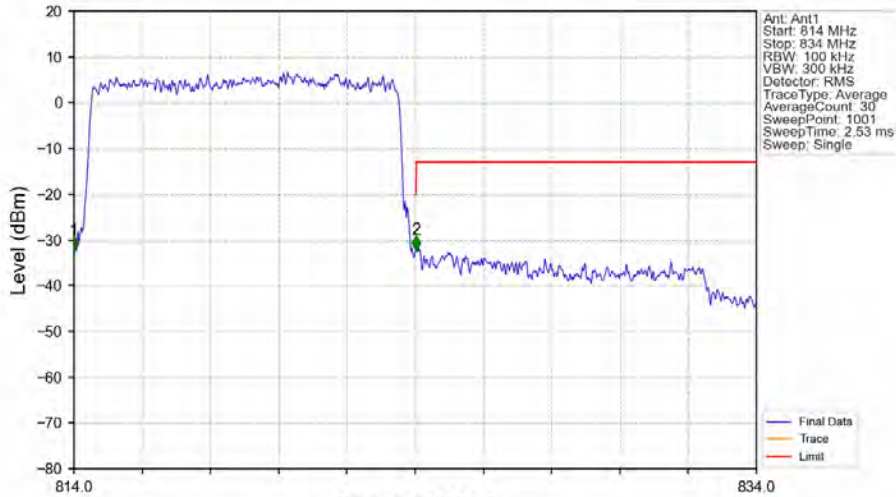
Band26a_10MHz_QPSK_HCH_819MHz_RB_50_0_NTNV
