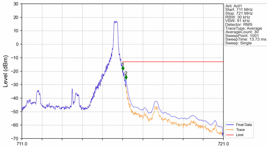
Band17_5MHz_QPSK_HCH_713.5MHz_RB_1_24_NTNV
