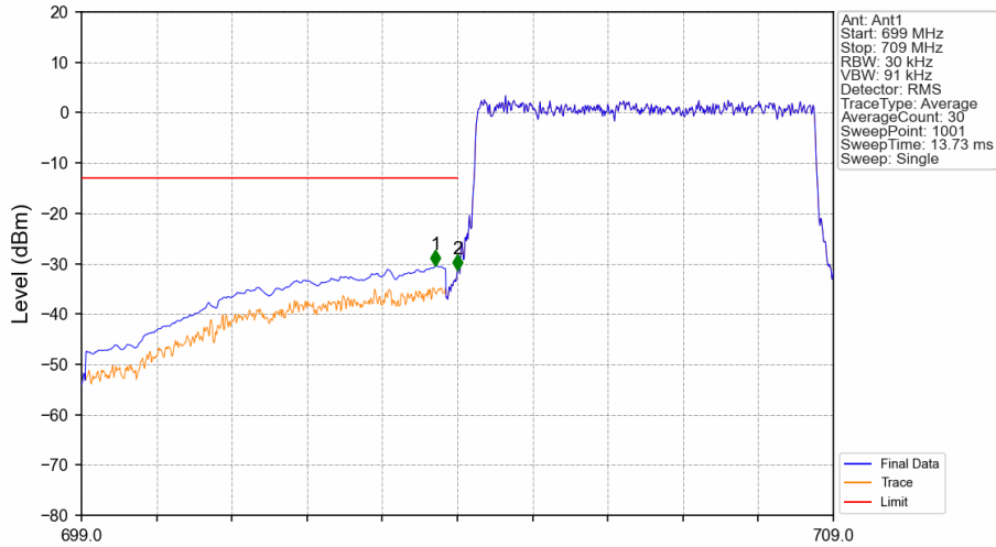
Band17_5MHz_64QAM_LCH_706.5MHz_RB_25_0_NTNV
