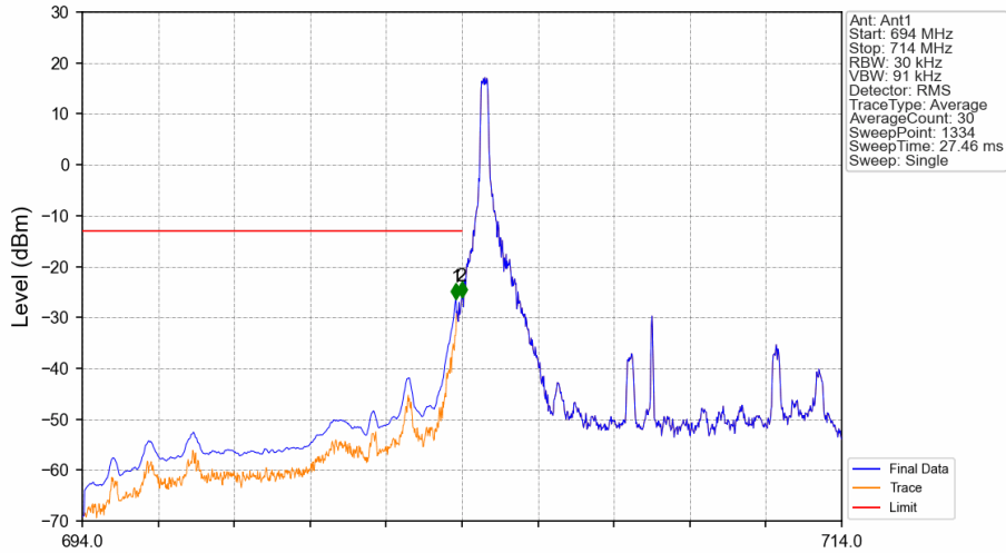
Band17_10MHz_16QAM_LCH_709MHz_RB_1_0_NTNV
