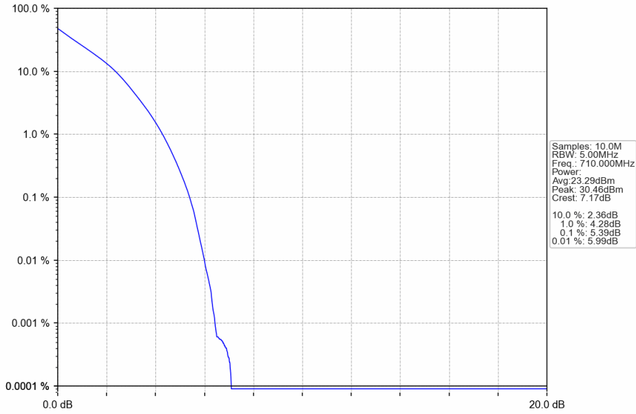
Band17_5MHz_QPSK_MCH_710MHz_RB_25_0_NTNV
