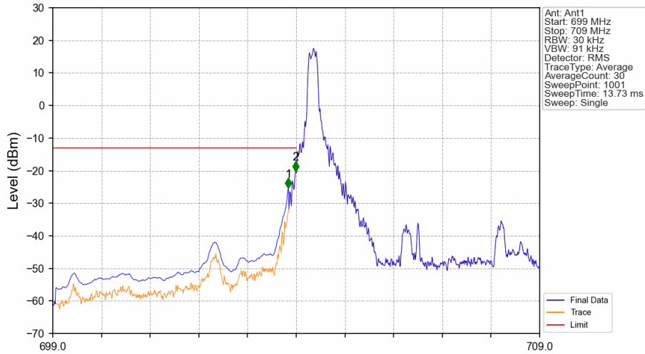
Band17_5MHz_16QAM_LCH_706.5MHz_RB_1_0_NTNV
