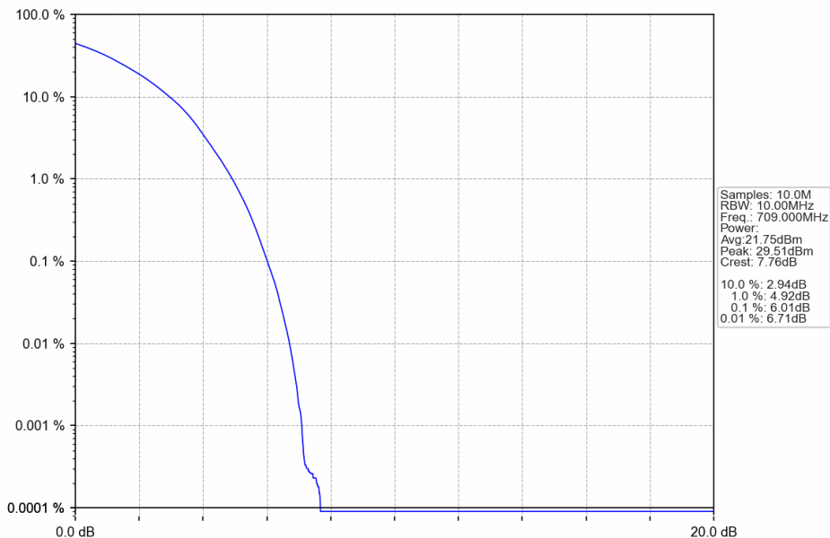
Band17_10MHz_64QAM_LCH_709MHz_RB_50_0_NTNV
