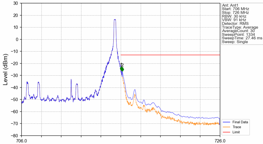
Band17_10MHz_16QAM_HCH_711MHz_RB_1_49_NTNV
