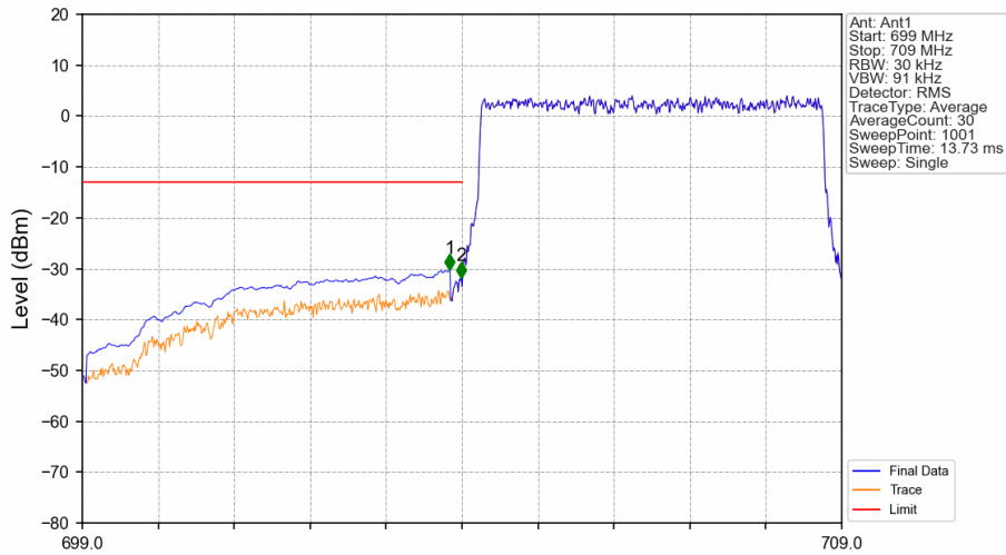
Band17_5MHz_QPSK_LCH_706.5MHz_RB_25_0_NTNV
