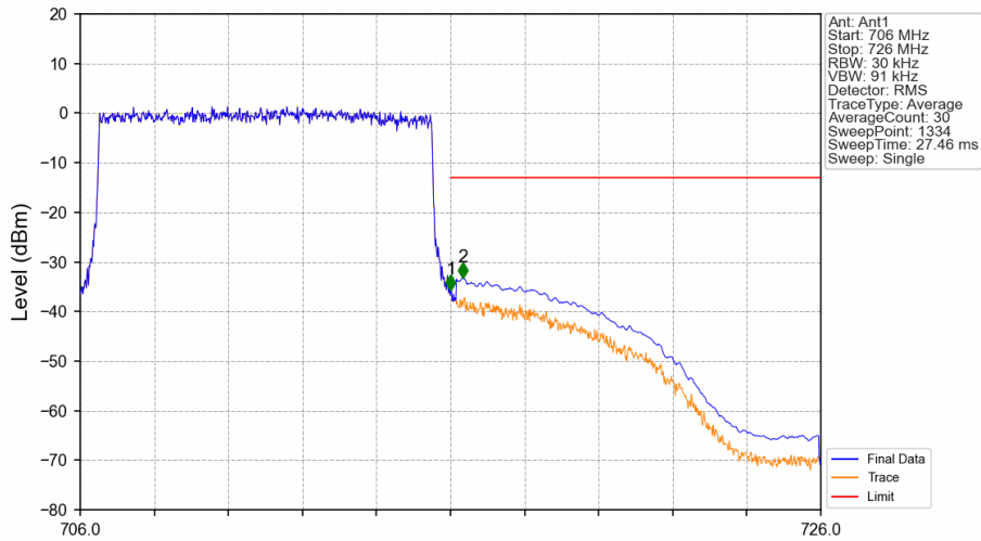
Band17_10MHz_QPSK_HCH_711MHz_RB_50_0_NTNV
