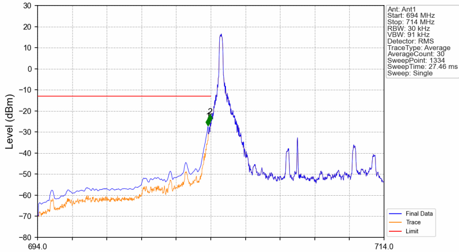
Band17_10MHz_64QAM_LCH_709MHz_RB_1_0_NTNV
