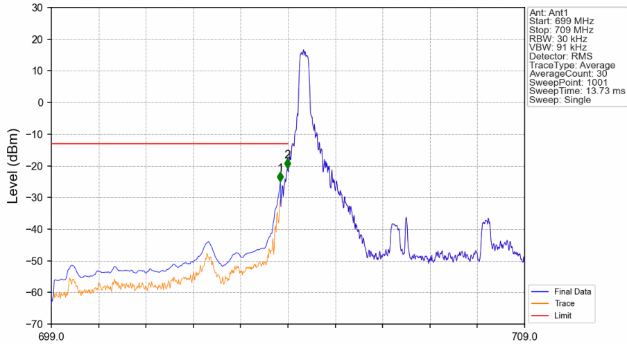
Band17_5MHz_64QAM_LCH_706.5MHz_RB_1_0_NTNV
