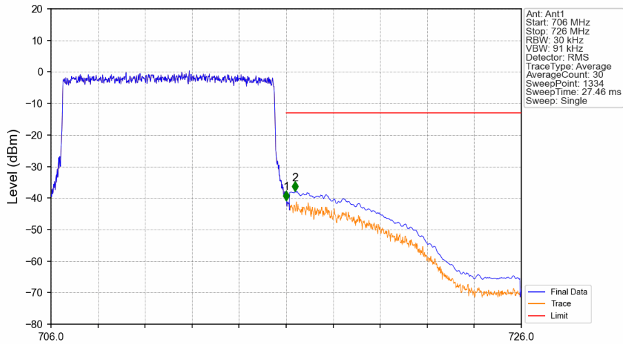
Band17_10MHz_16QAM_HCH_711MHz_RB_50_0_NTNV
