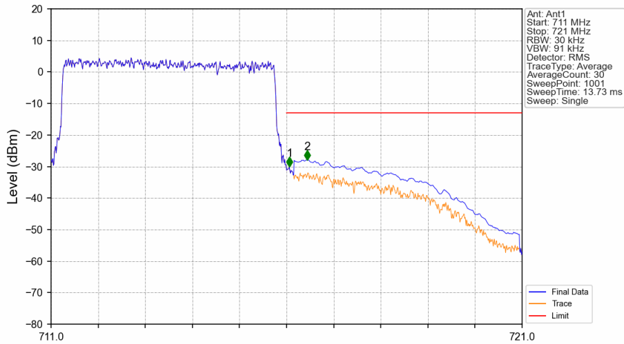
Band17_5MHz_QPSK_HCH_713.5MHz_RB_25_0_NTNV
