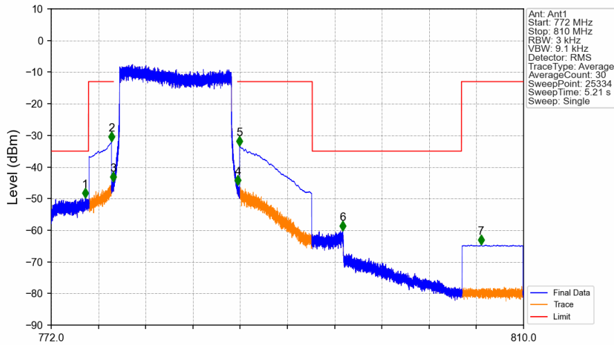
Band13_10MHz_QPSK_HCH_782MHz_RB_50_0_NTNV
