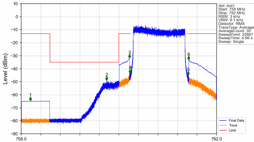
Band13_10MHz_QPSK_LCH_782MHz_RB_50_0_NTNV
