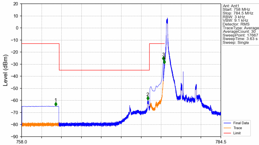
Band13_5MHz_16QAM_LCH_779.5MHz_RB_1_0_NTNV
