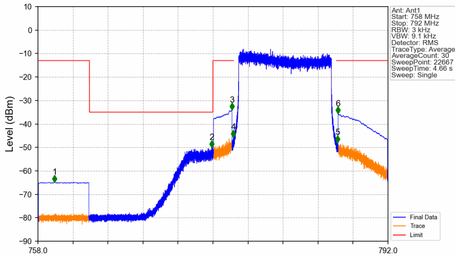
Band13_10MHz_64QAM_LCH_782MHz_RB_50_0_NTNV
