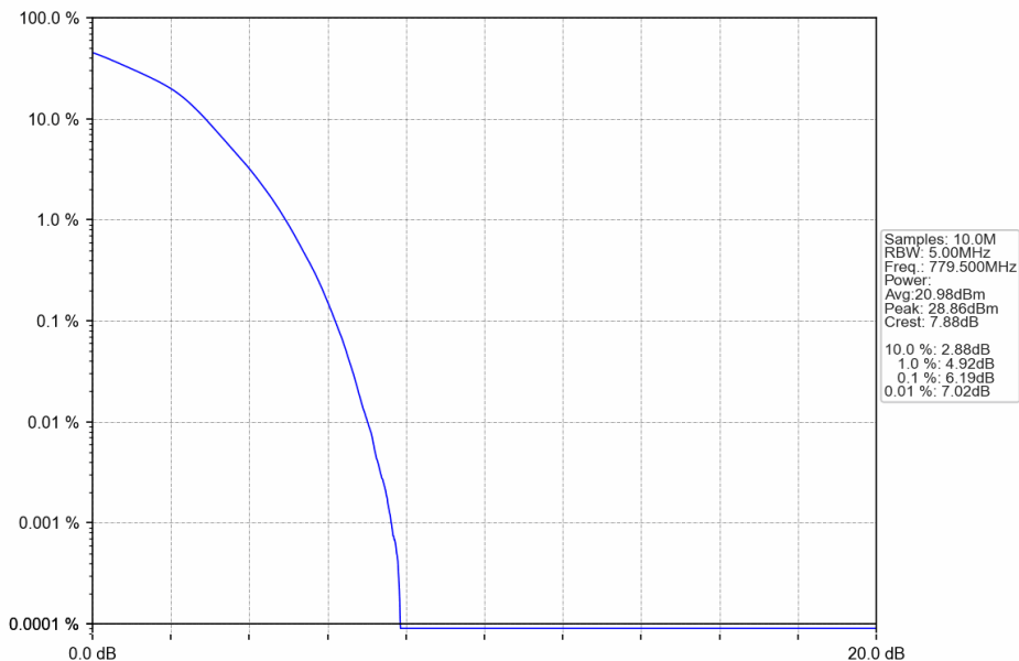
Band13_5MHz_16QAM_LCH_779.5MHz_RB_25_0_NTNV
