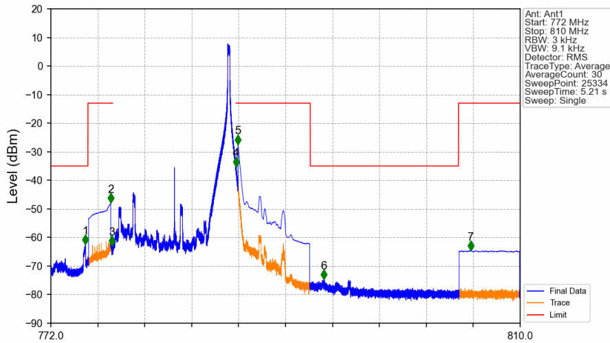
Band13_10MHz_QPSK_HCH_782MHz_RB_1_49_NTNV
