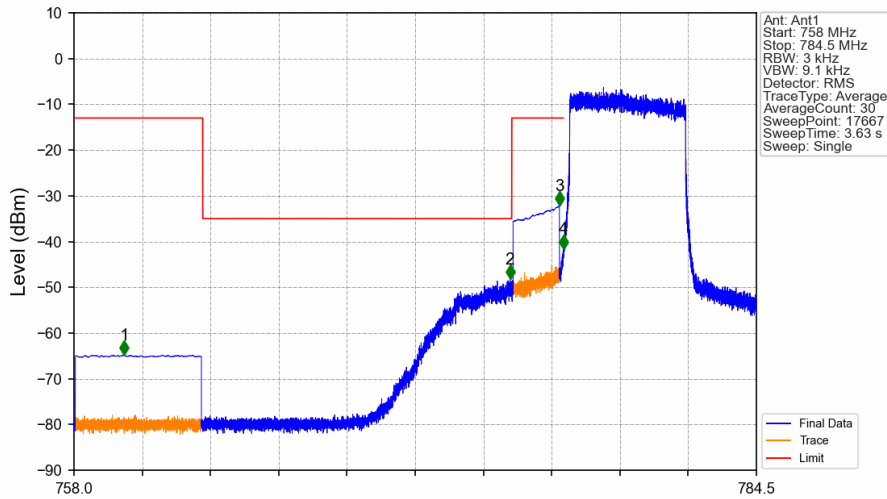
Band13_5MHz_64QAM_LCH_779.5MHz_RB_25_0_NTNV
