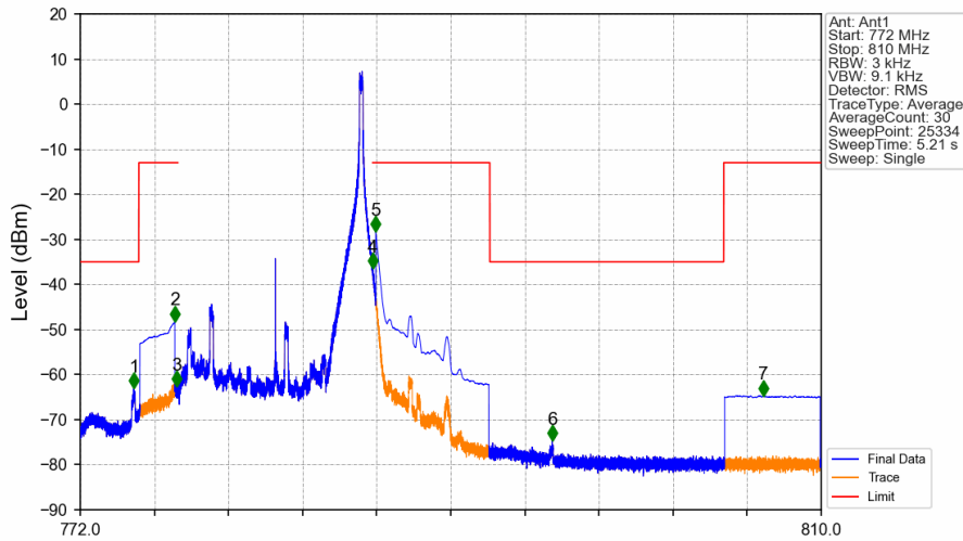
Band13_10MHz_64QAM_HCH_782MHz_RB_1_49_NTNV
