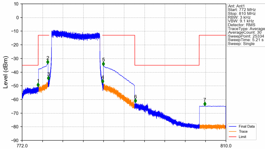
Band13_10MHz_64QAM_HCH_782MHz_RB_50_0_NTNV
