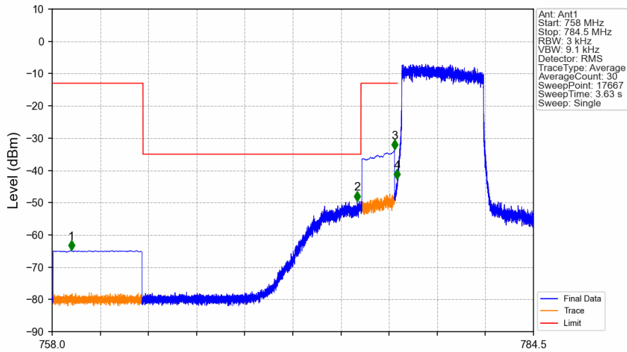
Band13_5MHz_16QAM_LCH_779.5MHz_RB_25_0_NTNV
