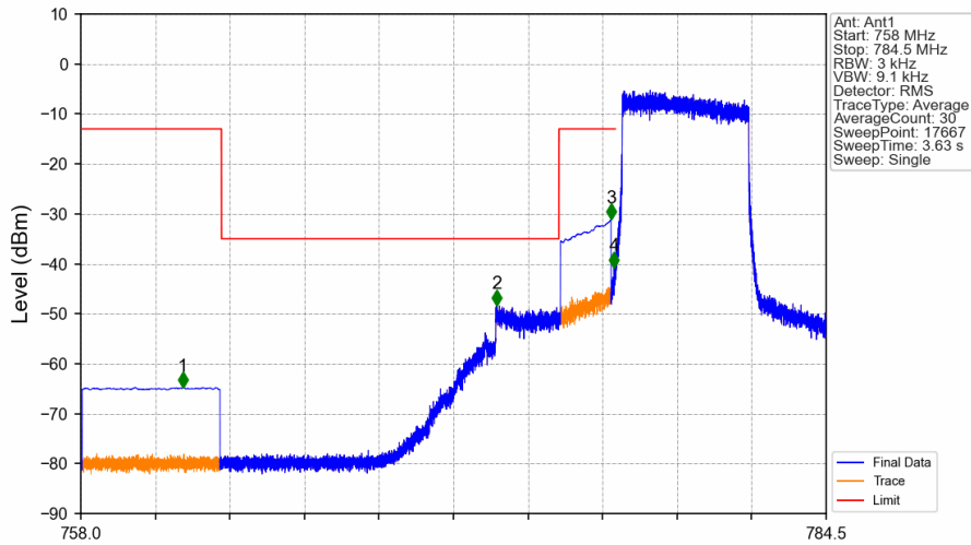
Band13_5MHz_QPSK_LCH_779.5MHz_RB_25_0_NTNV
