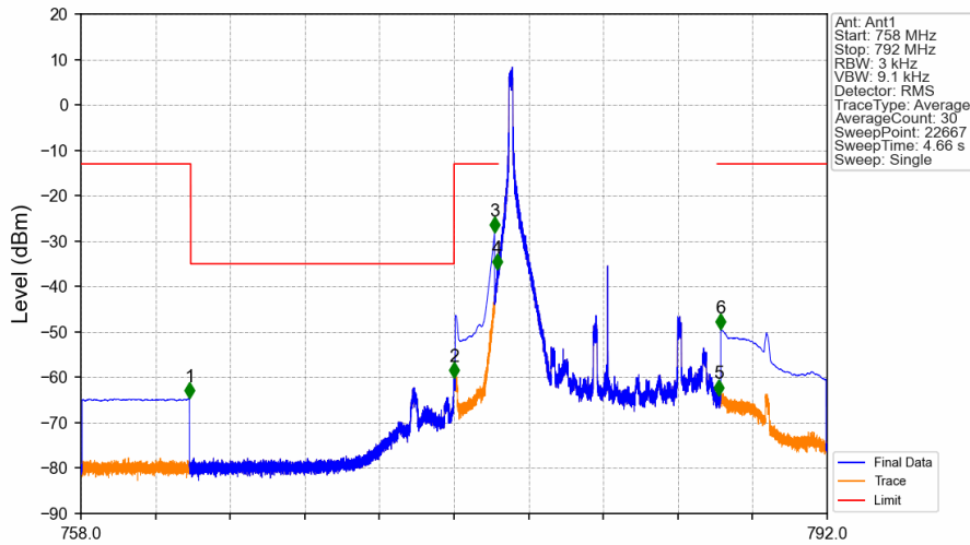
Band13_10MHz_16QAM_LCH_782MHz_RB_1_0_NTNV
