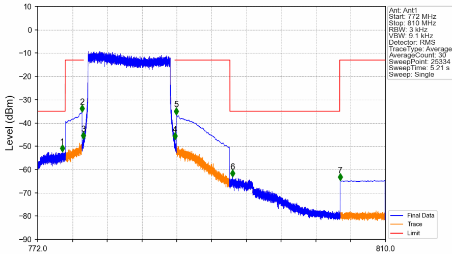
Band13_10MHz_16QAM_HCH_782MHz_RB_50_0_NTNV
