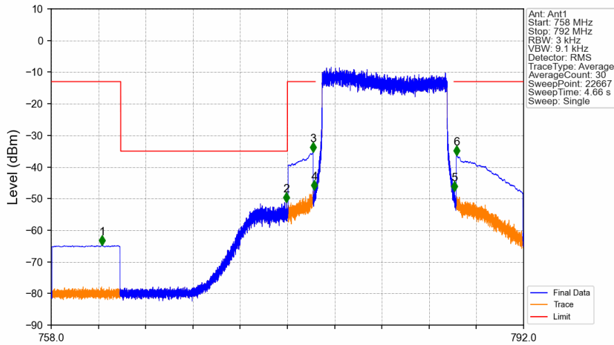
Band13_10MHz_16QAM_LCH_782MHz_RB_50_0_NTNV
