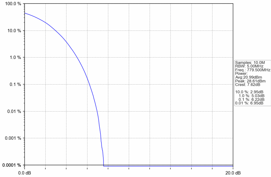
Band13_5MHz_64QAM_LCH_779.5MHz_RB_25_0_NTNV
