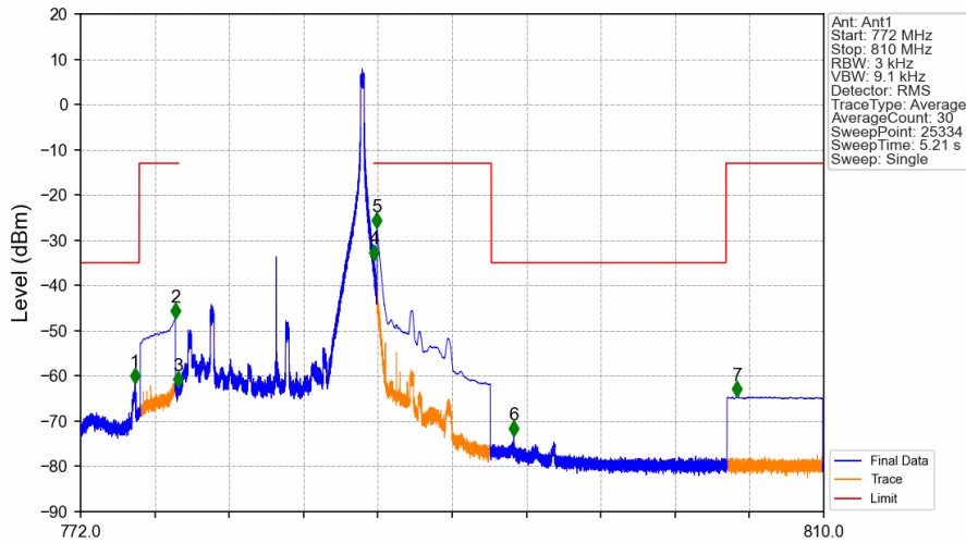
Band13_10MHz_16QAM_HCH_782MHz_RB_1_49_NTNV
