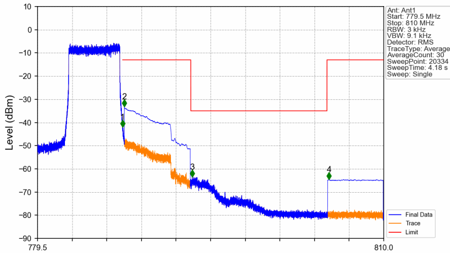
Band13_5MHz_QPSK_HCH_784.5MHz_RB_25_0_NTNV
