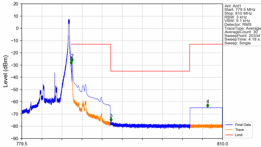
Band13_5MHz_QPSK_HCH_784.5MHz_RB_1_24_NTNV
