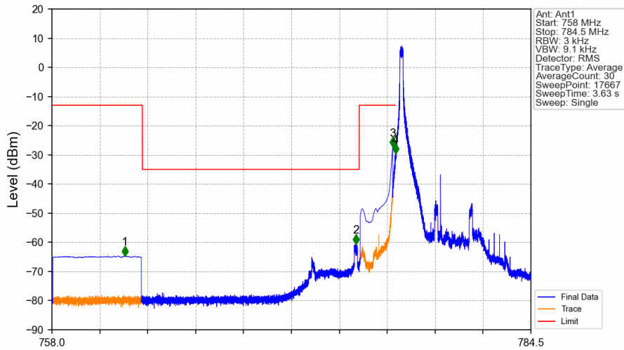
Band13_5MHz_64QAM_LCH_779.5MHz_RB_1_0_NTNV
