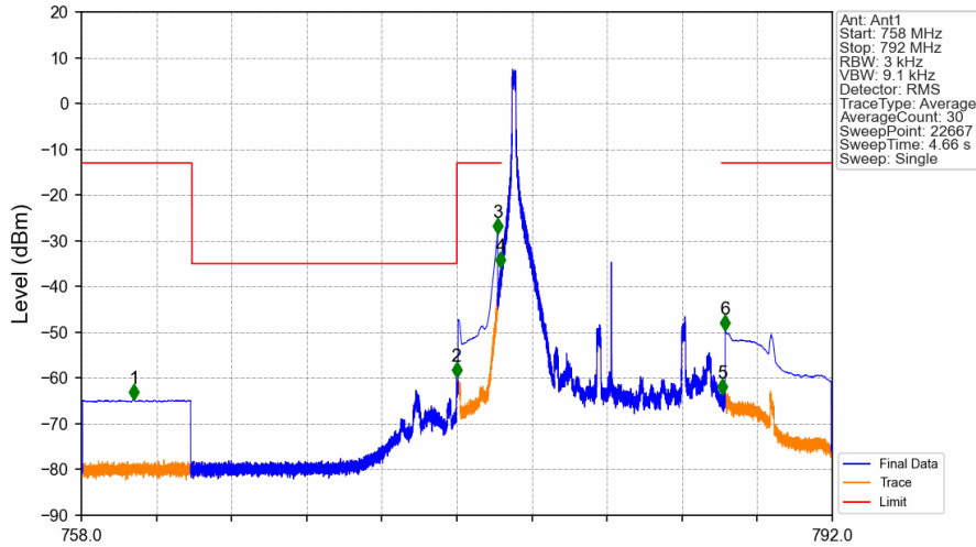
Band13_10MHz_64QAM_LCH_782MHz_RB_1_0_NTNV
