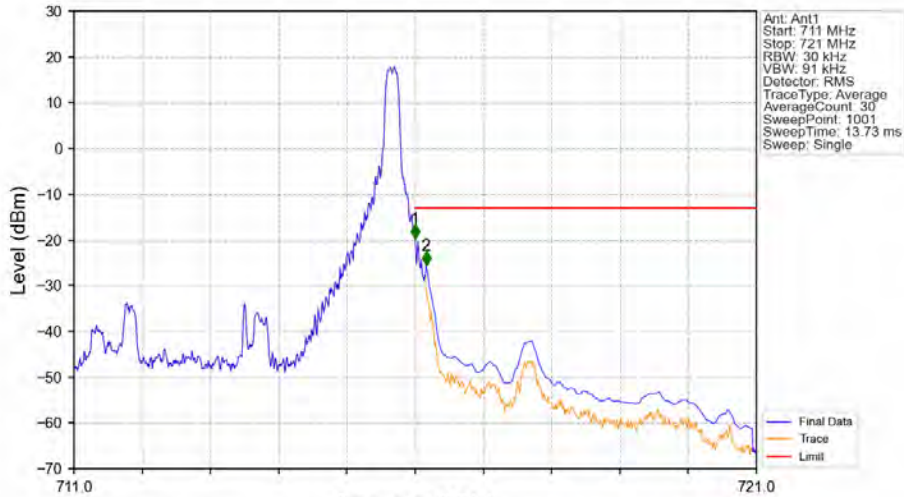
Band12_5MHz_QPSK_HCH_713.5MHz_RB_1_24_NTNV
