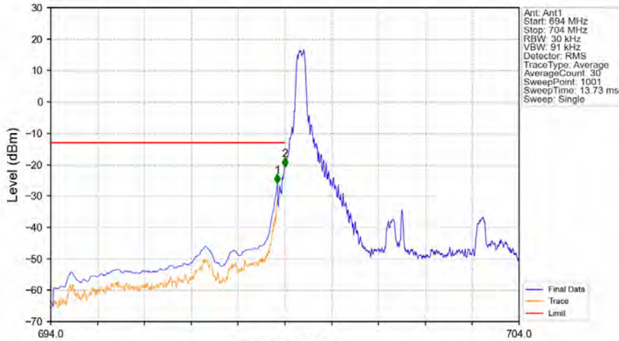
Band12_5MHz_64QAM_LCH_701.5MHz_RB_1_0_NTNV
