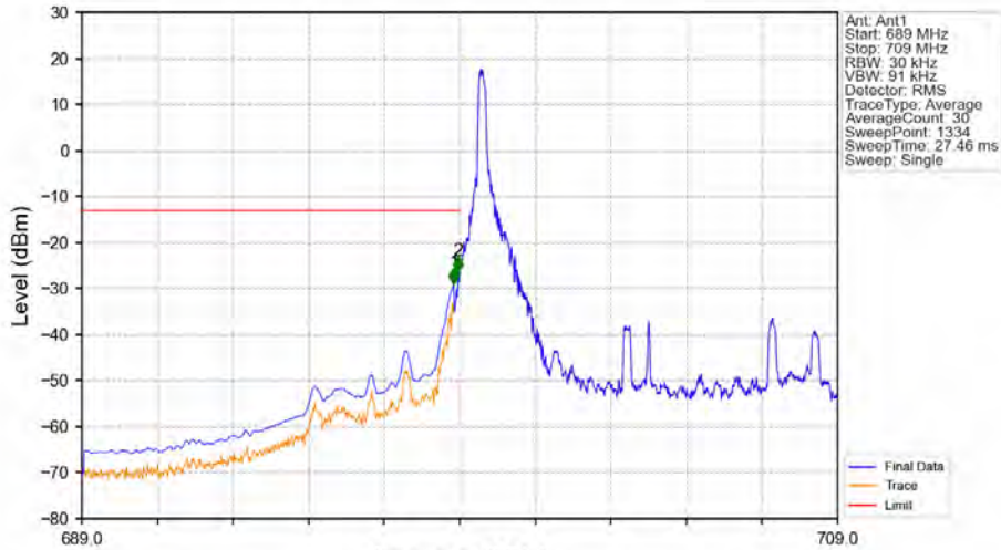
Band12_10MHz_16QAM_LCH_704MHz_RB_1_0_NTNV
