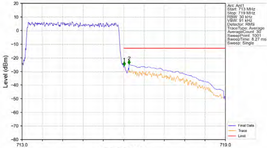
Band12_3MHz_QPSK_HCH_714.5MHz_RB_15_0_NTNV
