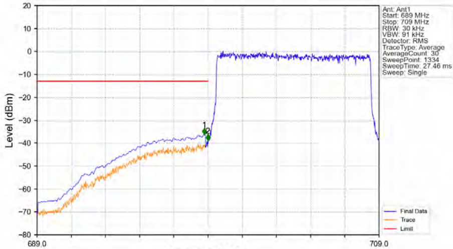
Band12_10MHz_16QAM_LCH_704MHz_RB_50_0_NTNV
