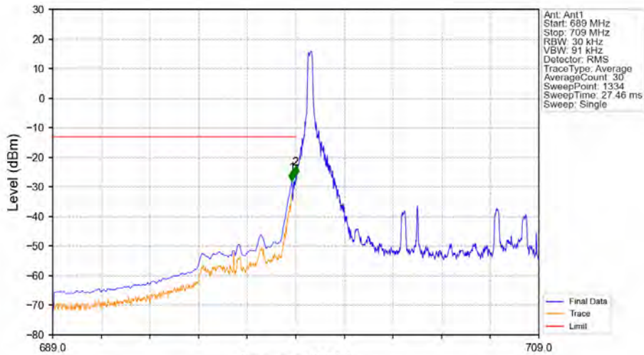
Band12_10MHz_64QAM_LCH_704MHz_RB_1_0_NTNV
