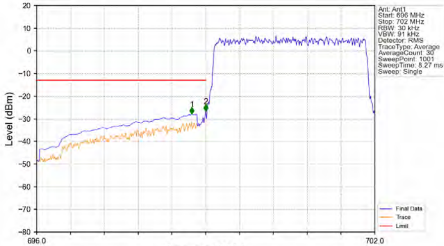
Band12_3MHz_QPSK_LCH_700.5MHz_RB_15_0_NTNV
