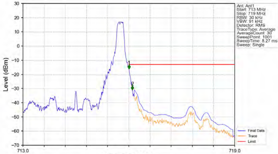
Band12_3MHz_QPSK_HCH_714.5MHz_RB_1_14_NTNV
