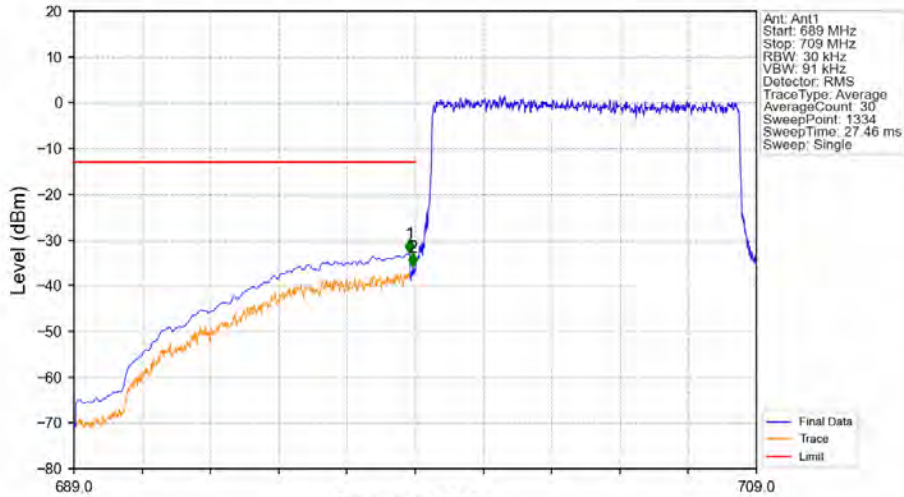
Band12_10MHz_QPSK_LCH_704MHz_RB_50_0_NTNV
