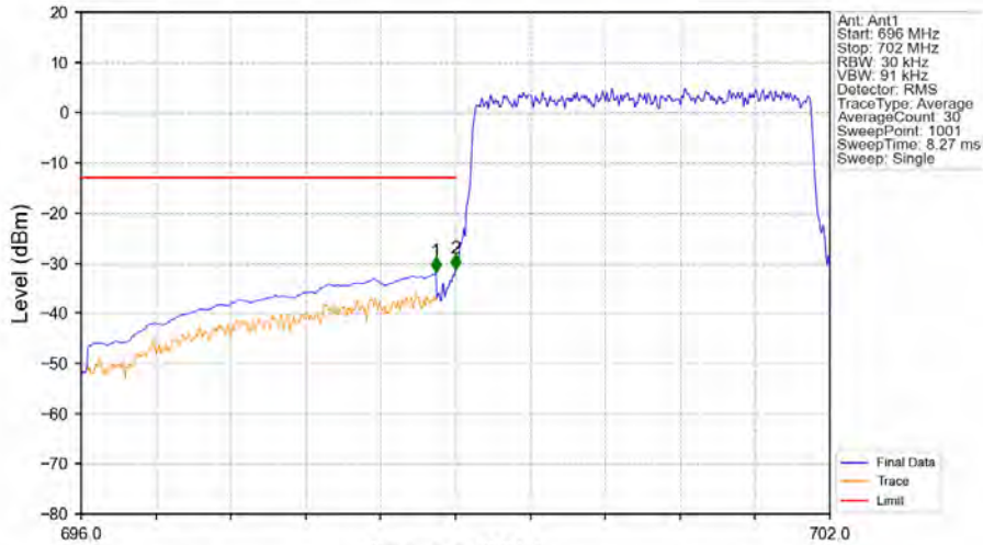
Band12_3MHz_16QAM_LCH_700.5MHz_RB_15_0_NTV
