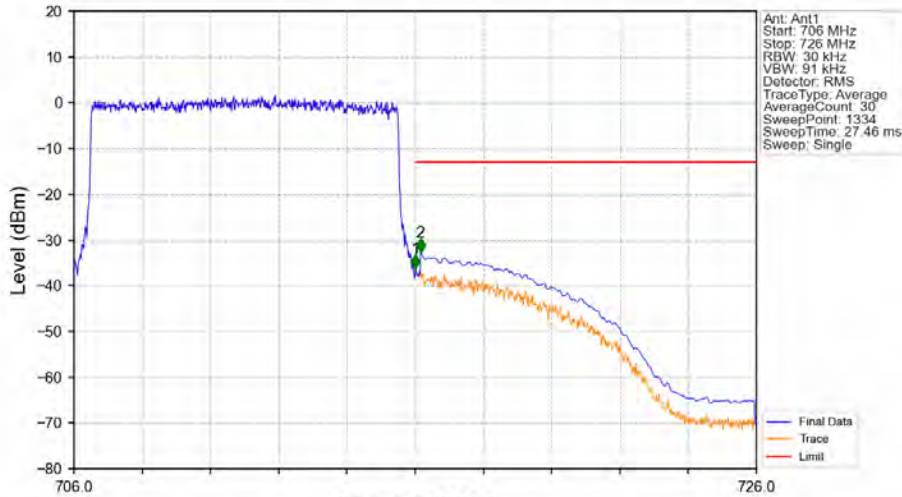
Band12_10MHz_QPSK_HCH_711MHz_RB_50_0_NTNV
