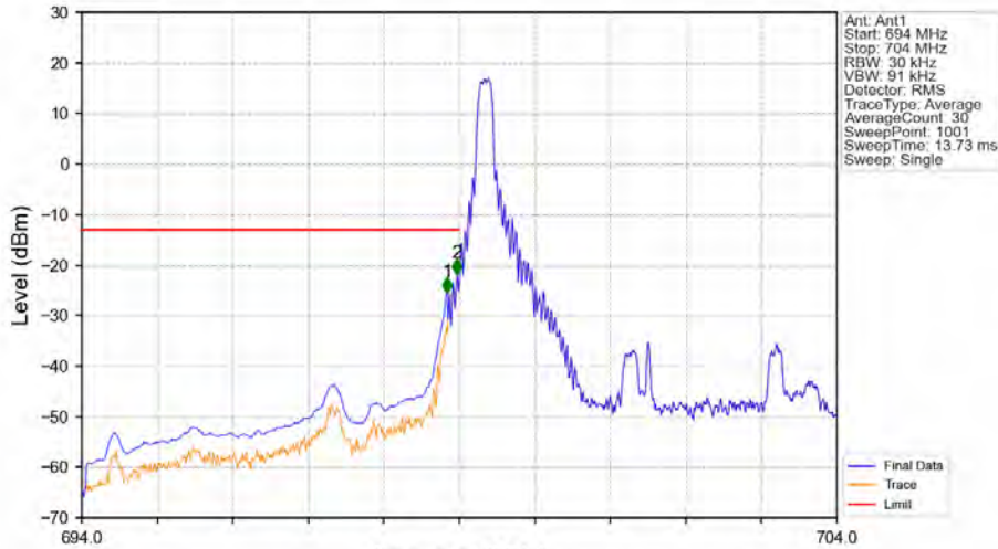
Band12_5MHz_16QAM_LCH_701.5MHz_RB_1_0_NTNV
