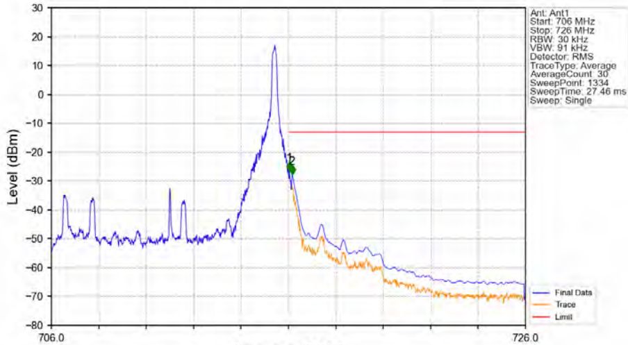
Band12_10MHz_64QAM_HCH_711MHz_RB_1_49_NTNV
