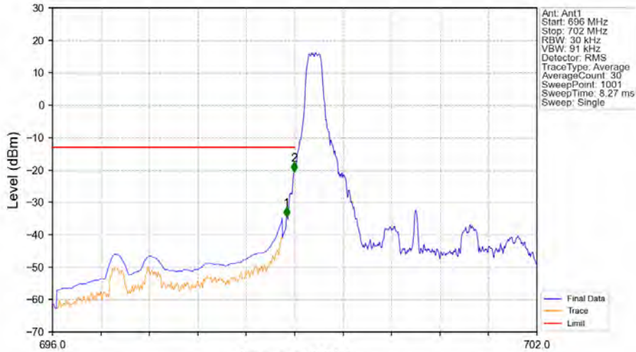
Band12_3MHz_64QAM_LCH_700.5MHz_RB_1_0_NTNV
