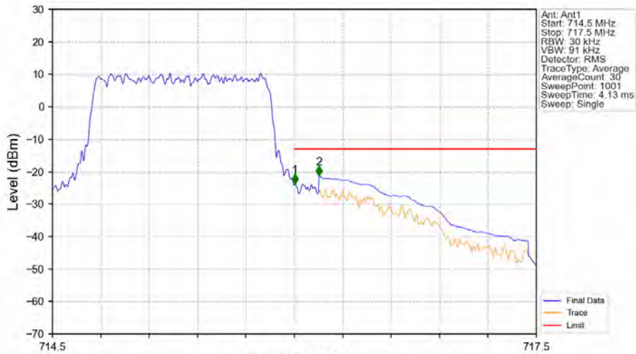
Band12_1.4MHz_QPSK_HCH_715.3MHz_RB_6_0_NTNV
