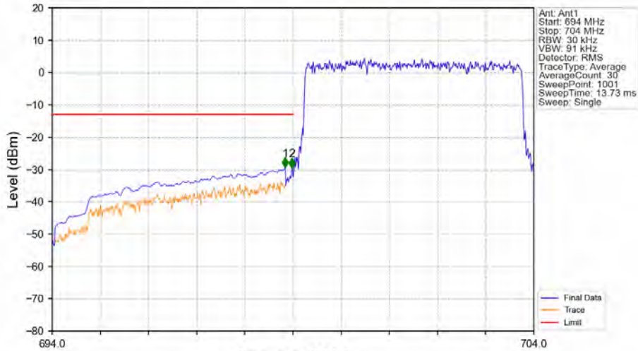
Band12_5MHz_QPSK_LCH_701.5MHz_RB_25_0_NTNV
