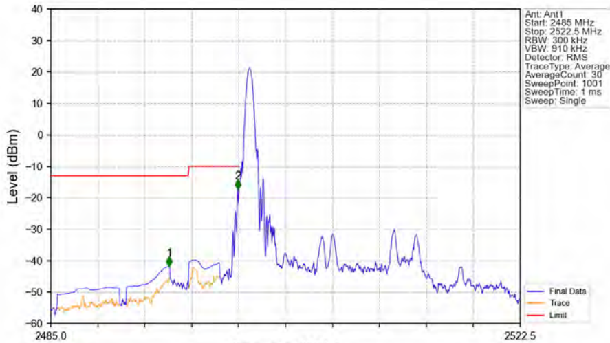
Band7_15MHz_64QAM_LCH_2507.5MHz_RB_1_0_NTV
