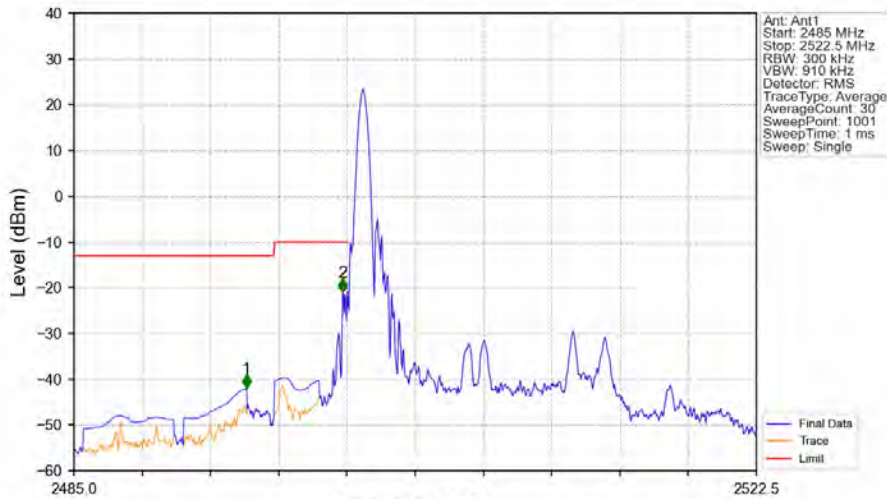
Band7_15MHz_16QAM_LCH_2507.5MHz_RB_1_0_NTV
