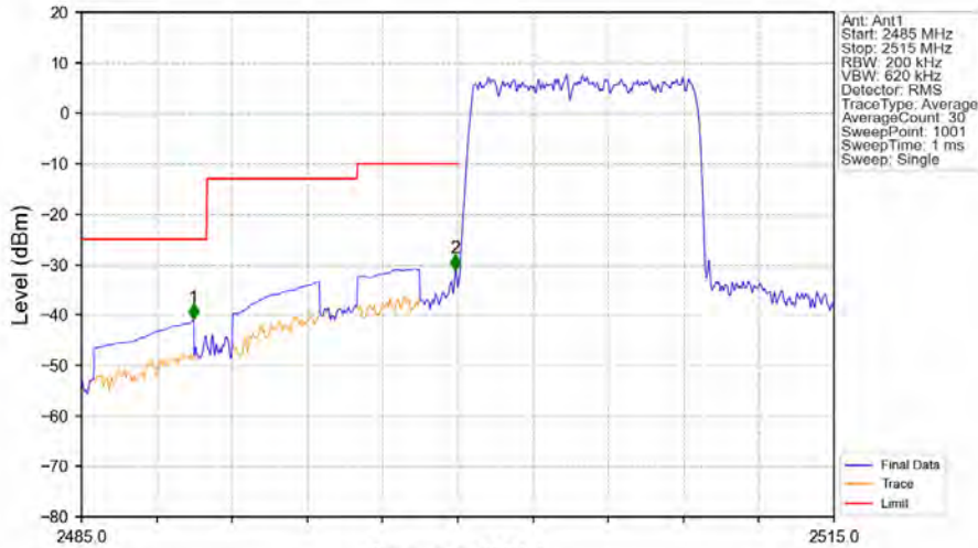
Band7_10MHz_16QAM_LCH_2505MHz_RB_50_0_NTNV
