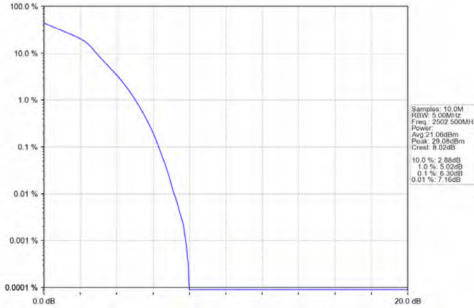
Band7_5MHz_16QAM_LCH_2502.5MHz_RB_25_0_NTNV
