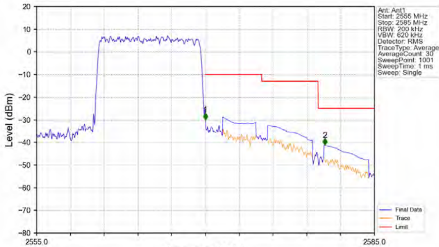
Band7_10MHz_64QAM_HCH_2565MHz_RB_50_0_NTNV
