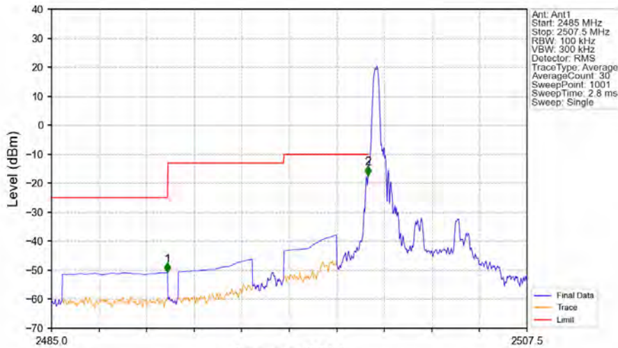
Band7_5MHz_16QAM_LCH_2502.5MHz_RB_1_0_NTNV
