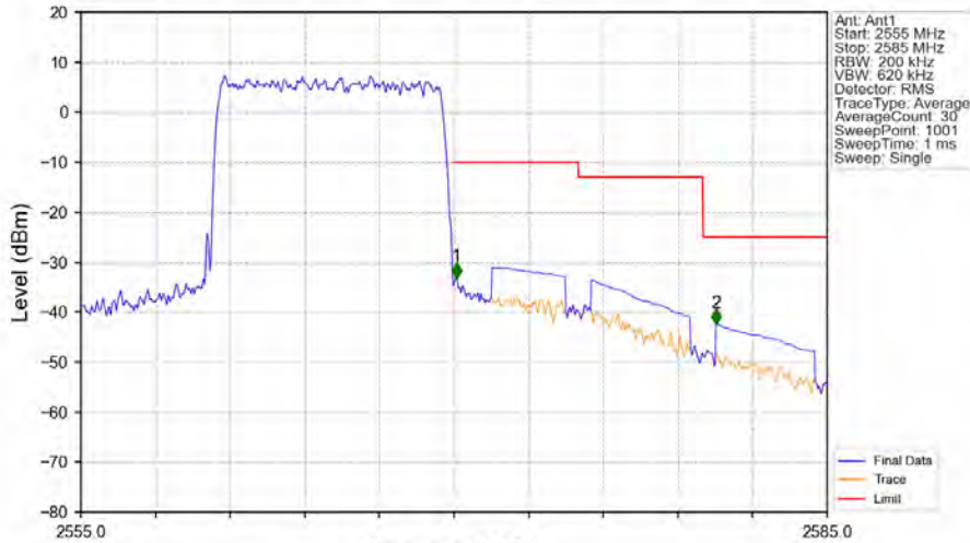
Band7_10MHz_16QAM_HCH_2565MHz_RB_50_0_NTNV
