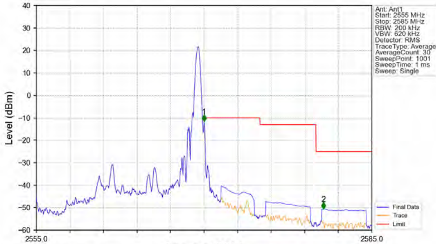
Band7_10MHz_64QAM_HCH_2565MHz_RB_1_49_NTNV
