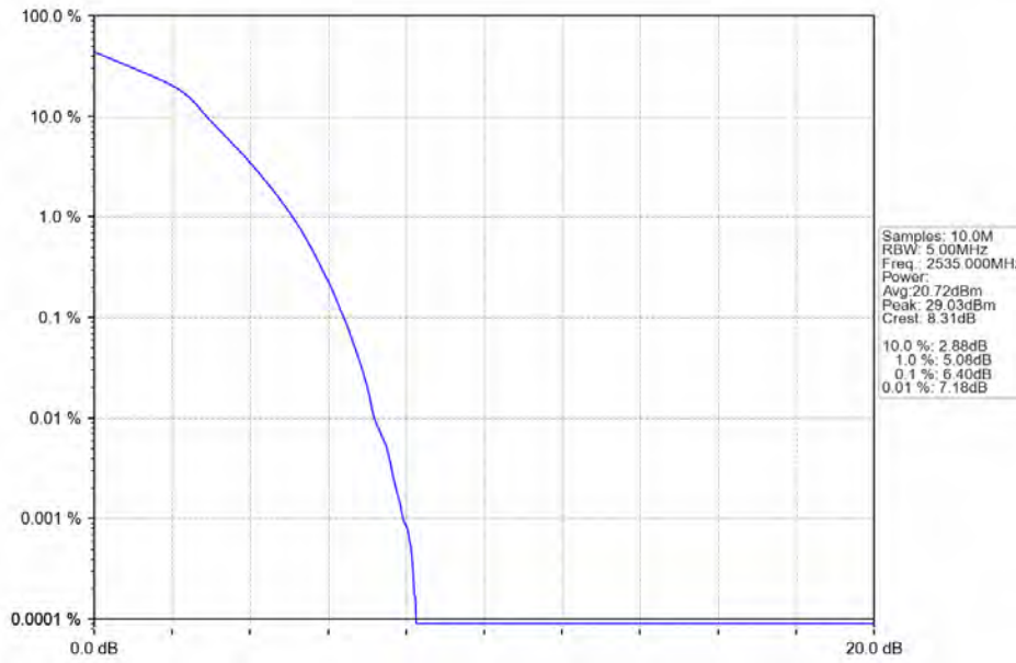
Band7_5MHz_16QAM_MCH_2535MHz_RB_25_0_NTNV
