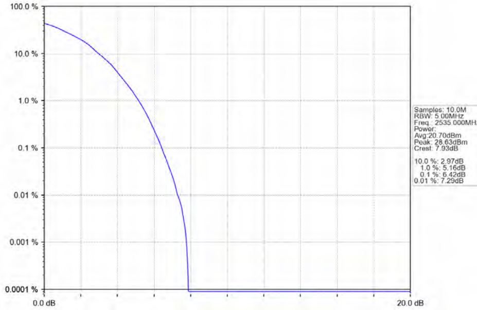
Band7_5MHz_64QAM_MCH_2535MHz_RB_25_0_NTNV
