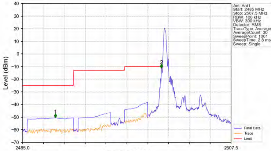
Band7_5MHz_64QAM_LCH_2502.5MHz_RB_1_0_NTNV
