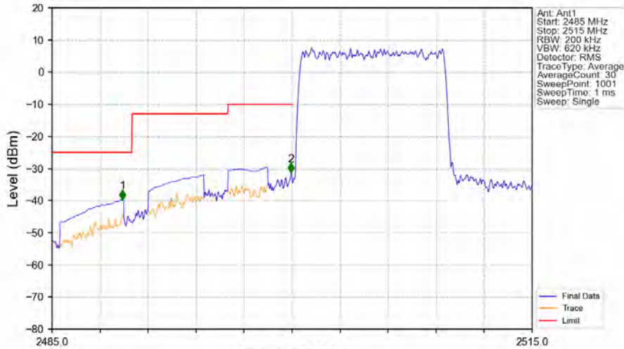
Band7_10MHz_64QAM_LCH_2505MHz_RB_50_0_NTNV
