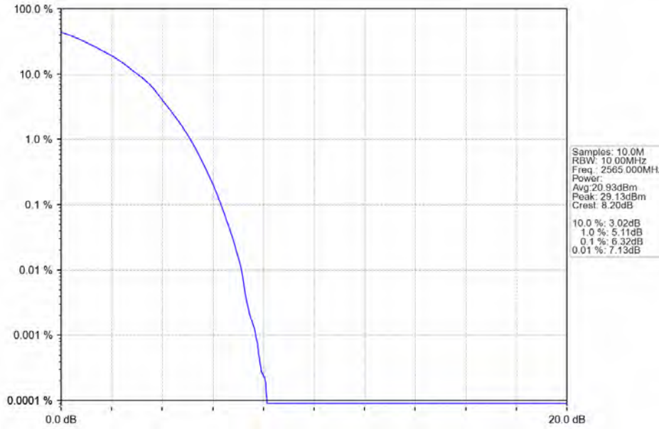
Band7_10MHz_64QAM_HCH_2565MHz_RB_50_0_NTNV
