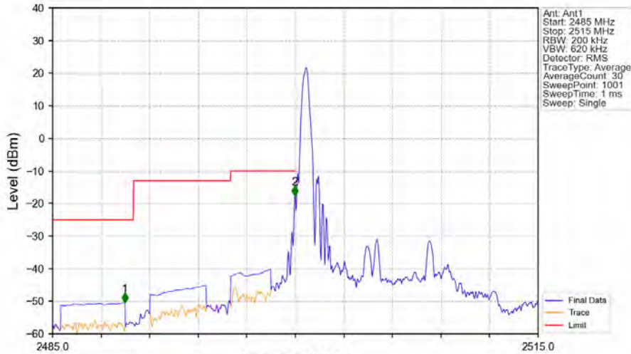
Band7_10MHz_64QAM_LCH_2505MHz_RB_1_0_NTNV
