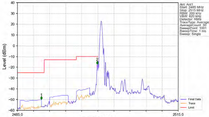
Band7_10MHz_16QAM_LCH_2505MHz_RB_1_0_NTNV
