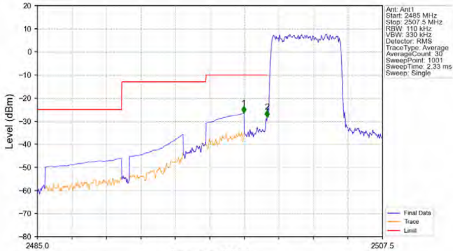
Band7_5MHz_64QAM_LCH_2502.5MHz_RB_25_0_NTV
