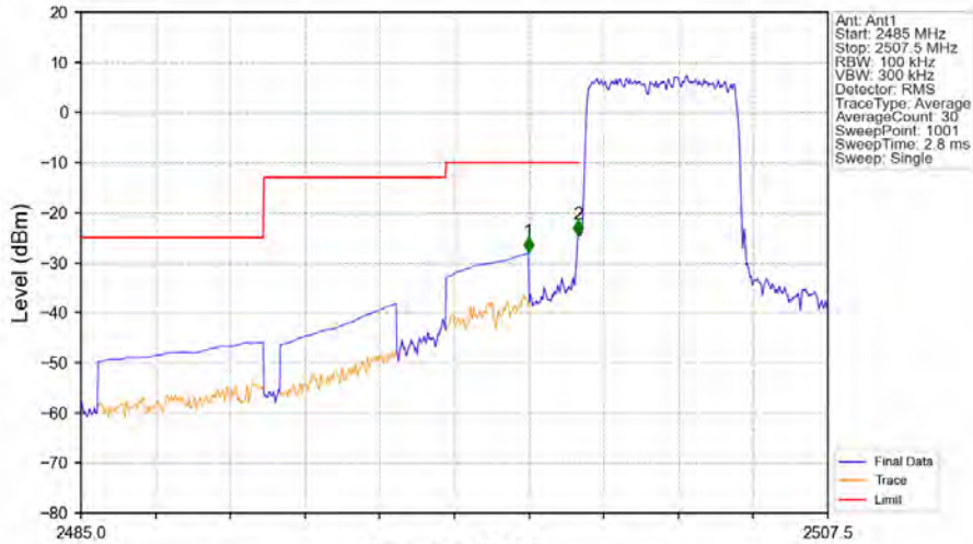
Band7_5MHz_16QAM_LCH_2502.5MHz_RB_25_0_NTV
