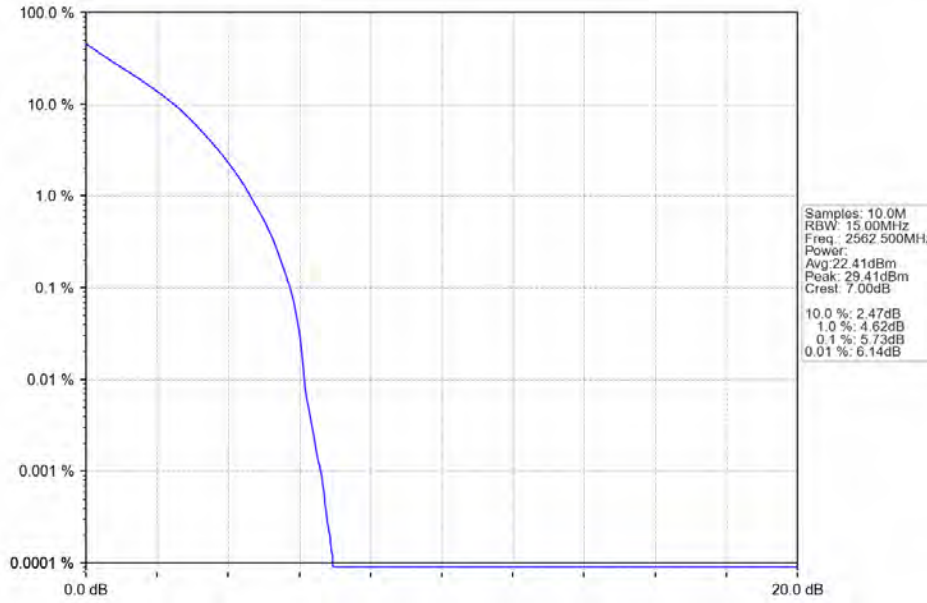
Band7_15MHz_QPSK_HCH_2562.5MHz_RB_75_0_NTNV
