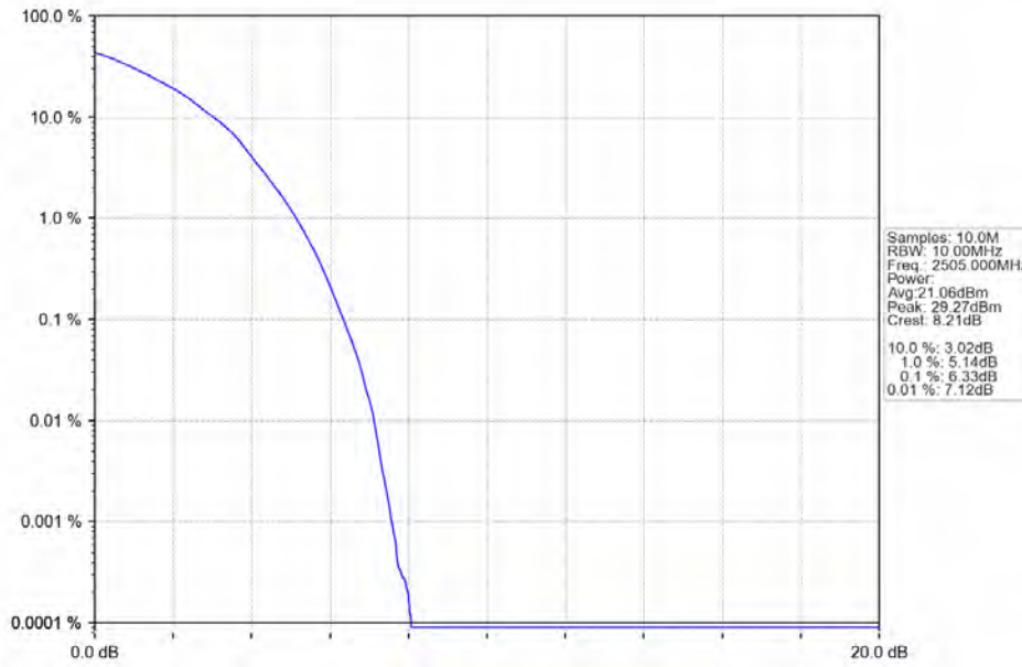
Band7_10MHz_64QAM_LCH_2505MHz_RB_50_0_NTNV
