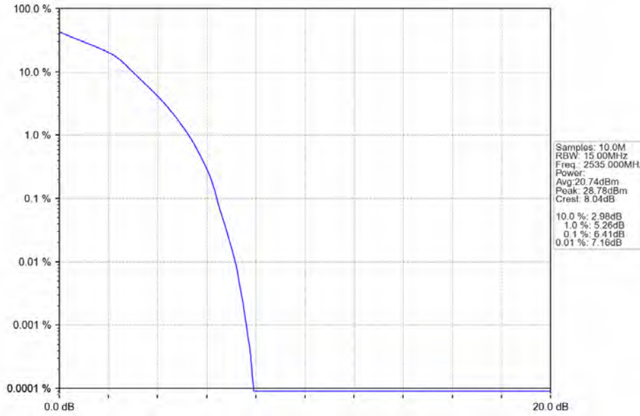
Band7_15MHz_16QAM_MCH_2535MHz_RB_75_0_NTNV
