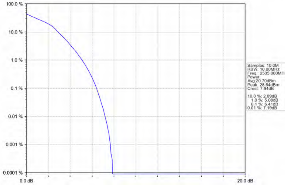
Band7_10MHz_16QAM_MCH_2535MHz_RB_50_0_NTNV
