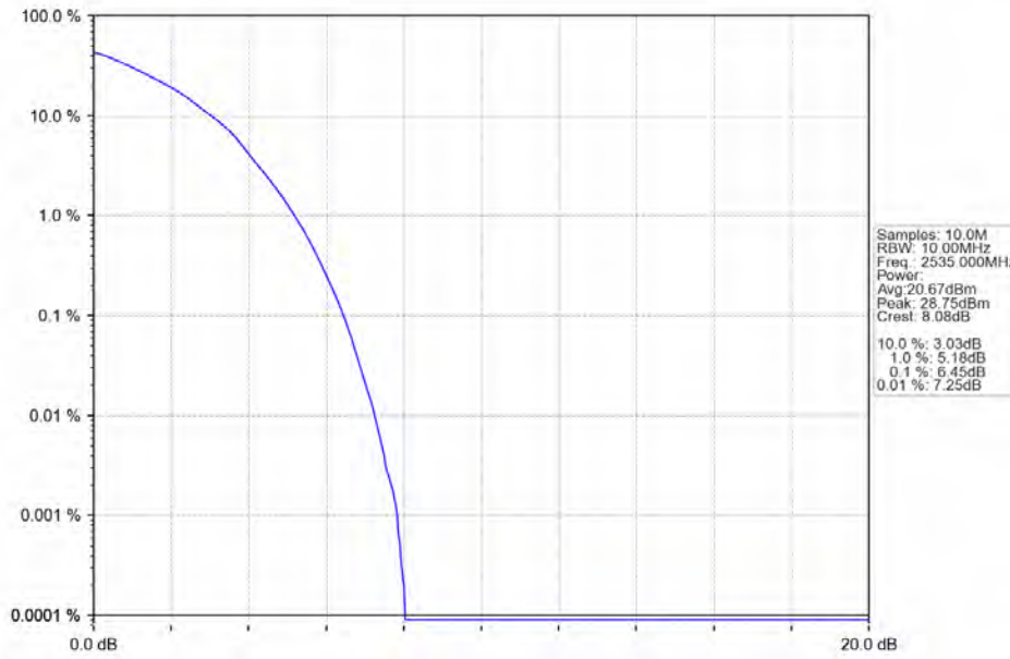
Band7_10MHz_64QAM_MCH_2535MHz_RB_50_0_NTNV
