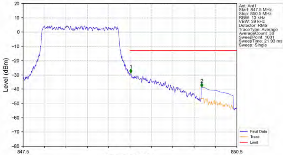
Band5_1.4MHz_64QAM_HCH_848.3MHz_RB_6_0_NTNV
