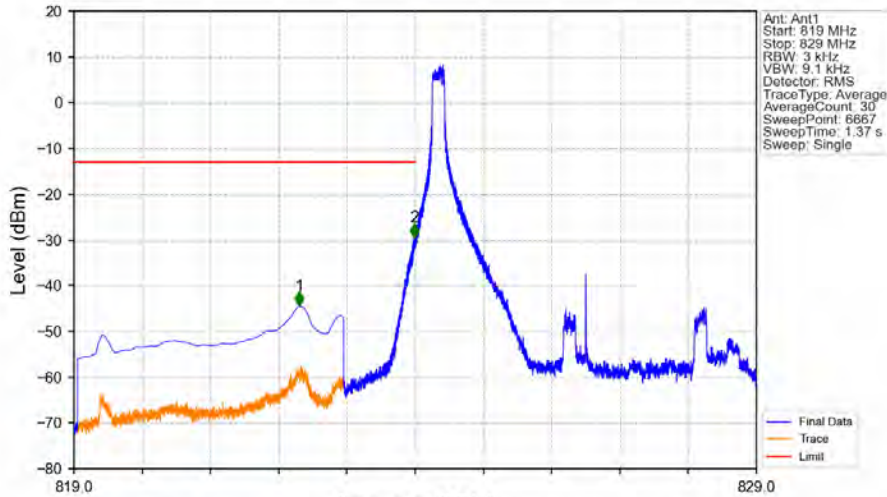
Band5_5MHz_16QAM_LCH_826.5MHz_RB_1_0_NTNV
