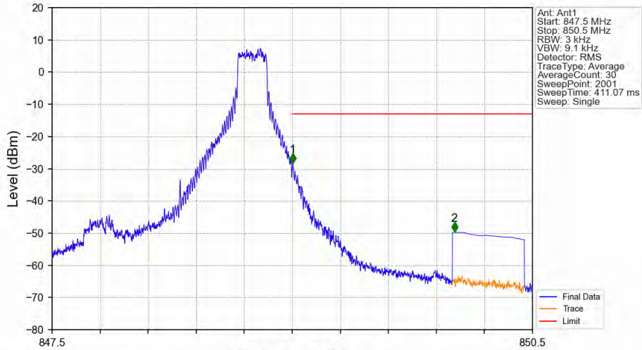
Band5_1.4MHz_64QAM_HCH_848.3MHz_RB_1_5_NTNV
