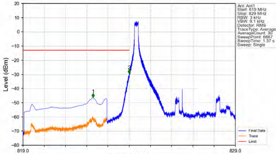
Band5_5MHz_64QAM_LCH_826.5MHz_RB_1_0_NTNV
