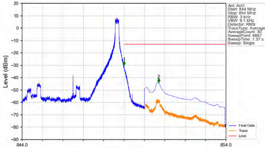
Band5_5MHz_16QAM_HCH_846.5MHz_RB_1_24_NTNV
