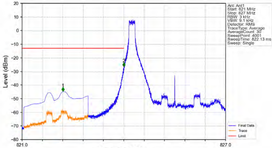
Band5_3MHz_16QAM_LCH_825.5MHz_RB_1_0_NTNV
