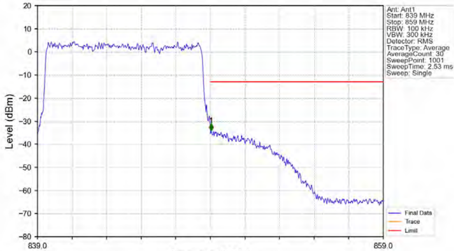
Band5_10MHz_64QAM_HCH_844MHz_RB_50_0_NTNV
