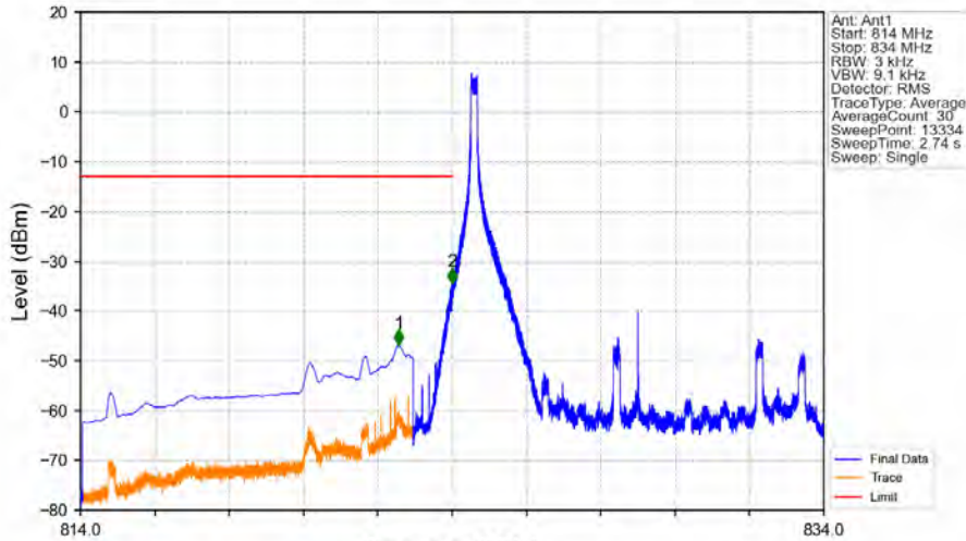
Band5_10MHz_64QAM_LCH_829MHz_RB_1_0_NTNV
