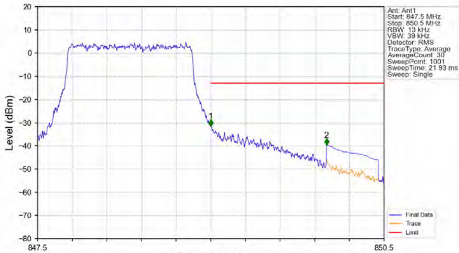
Band5_1.4MHz_16QAM_HCH_848.3MHz_RB_6_0_NTNV
