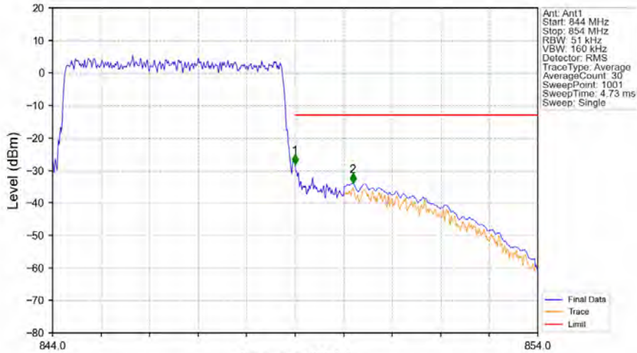
Band5_5MHz_64QAM_HCH_846.5MHz_RB_25_0_NTNV
