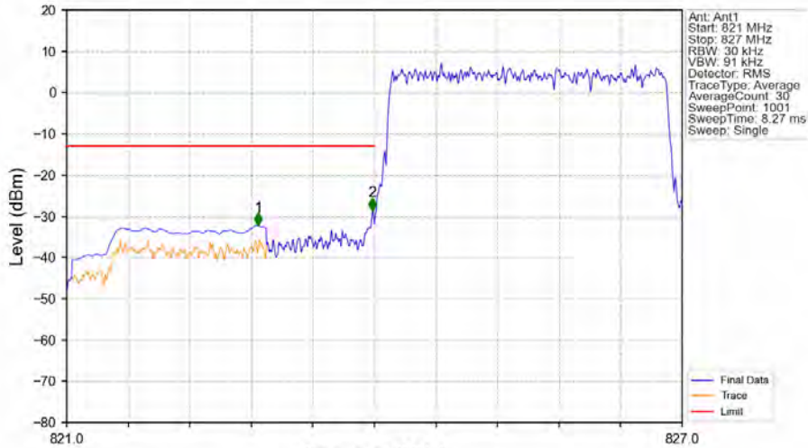
Band5_3MHz_QPSK_LCH_825.5MHz_RB_15_0_NTNV
