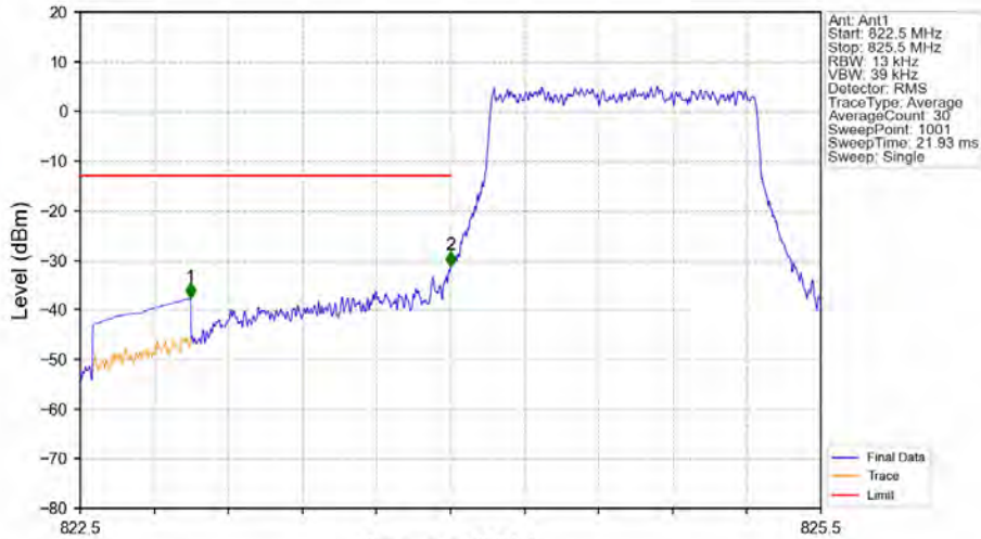
Band5_1.4MHz_16QAM_LCH_824.7MHz_RB_6_0_NTNV
