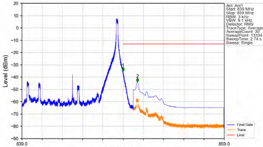
Band5_10MHz_16QAM_HCH_844MHz_RB_1_49_NTNV
