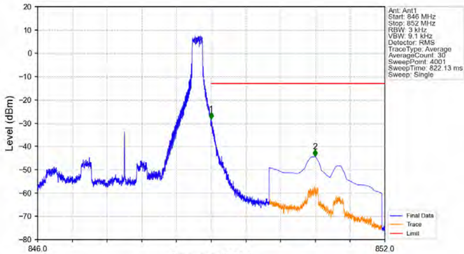
Band5_3MHz_16QAM_HCH_847.5MHz_RB_1_14_NTNV
