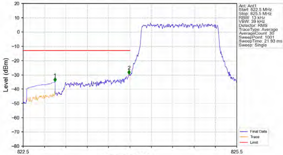
Band5_1.4MHz_QPSK_LCH_824.7MHz_RB_6_0_NTNV
