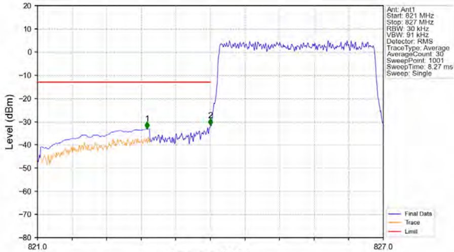
Band5_3MHz_64QAM_LCH_825.5MHz_RB_15_0_NTNV
