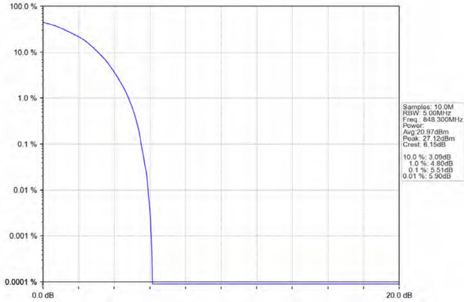
Band5_1.4MHz_64QAM_HCH_848.3MHz_RB_6_0_NTNV
