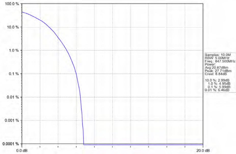
Band5_3MHz_64QAM_HCH_847.5MHz_RB_15_0_NTNV
