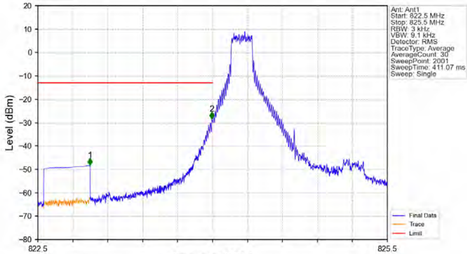
Band5_1.4MHz_16QAM_LCH_824.7MHz_RB_1_0_NTNV
