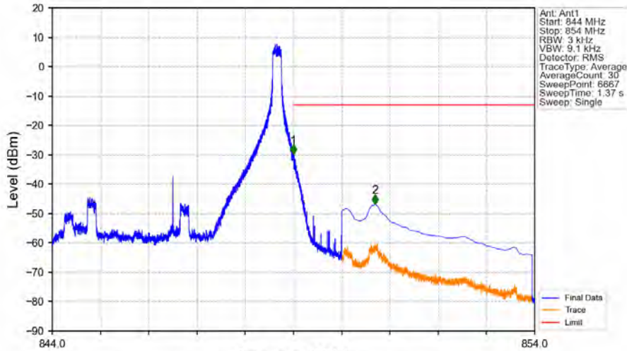
Band5_5MHz_64QAM_HCH_846.5MHz_RB_1_24_NTNV
