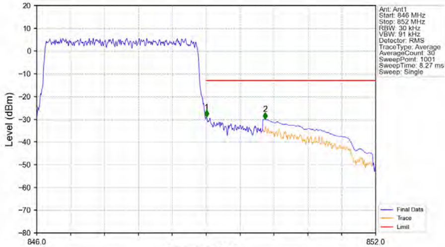
Band5_3MHz_QPSK_HCH_847.5MHz_RB_15_0_NTNV
