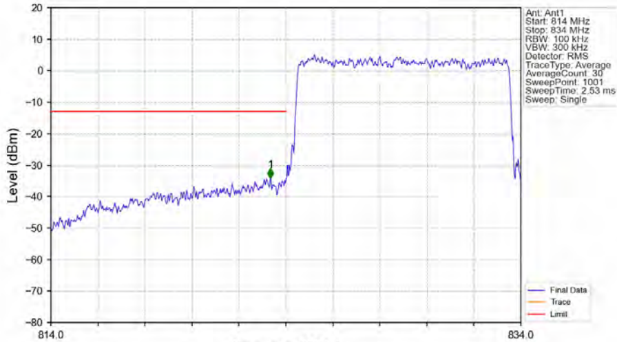
Band5_10MHz_64QAM_LCH_829MHz_RB_50_0_NTNV
