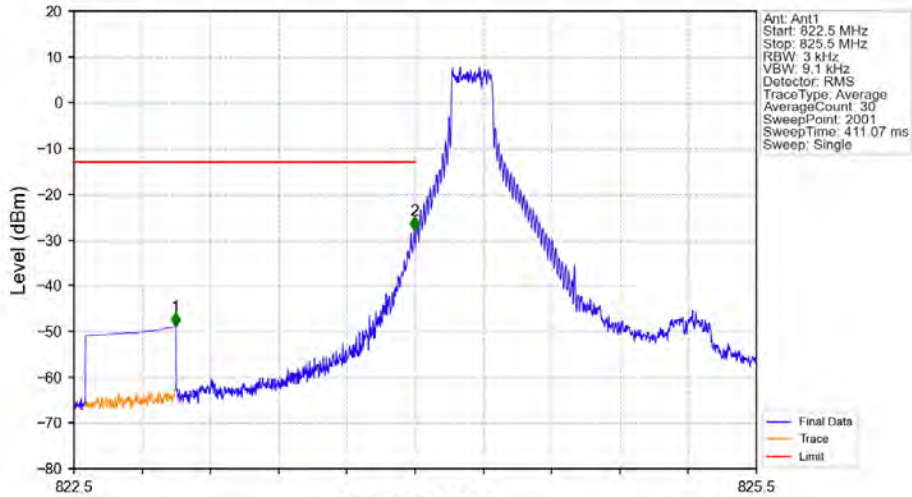
Band5_1.4MHz_64QAM_LCH_824.7MHz_RB_1_0_NTNV
