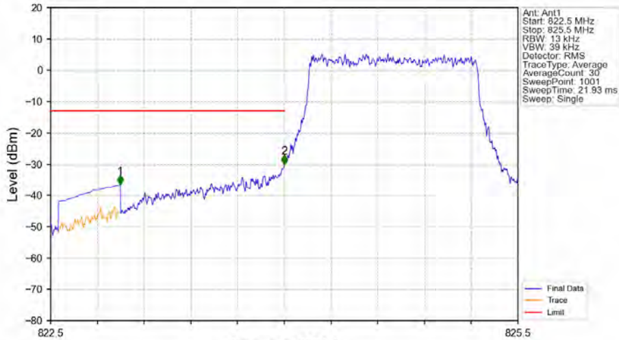
Band5_1.4MHz_64QAM_LCH_824.7MHz_RB_6_0_NTNV
