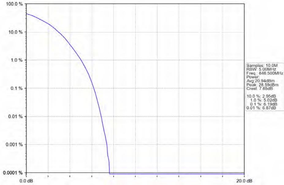
Band5_5MHz_64QAM_HCH_846.5MHz_RB_25_0_NTNV
