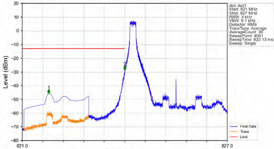
Band5_3MHz_64QAM_LCH_825.5MHz_RB_1_0_NTNV
