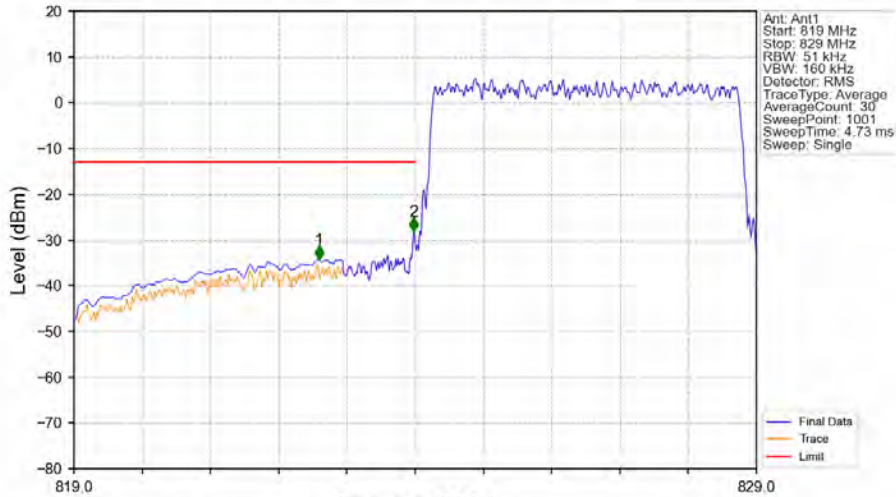
Band5_5MHz_64QAM_LCH_826.5MHz_RB_25_0_NTNV
