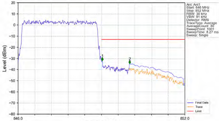
Band5_3MHz_16QAM_HCH_847.5MHz_RB_15_0_NTNV
