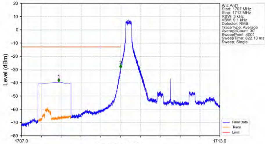
Band4_3MHz_64QAM_LCH_1711.5MHz_RB_1_0_NTNV
