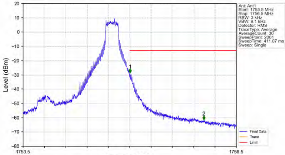
Band4_1.4MHz_QPSK_HCH_1754.3MHz_RB_1_5_NTV
