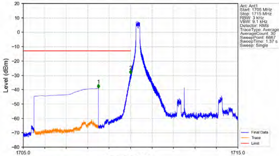
Band4_5MHz_64QAM_LCH_1712.5MHz_RB_1_0_NTNV
