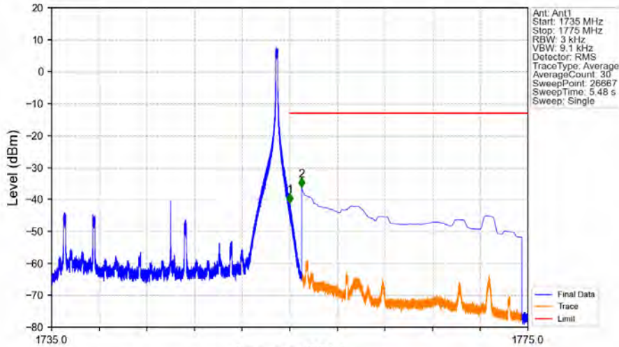
Band4_20MHz_16QAM_HCH_1745MHz_RB_1_99_NTNV
