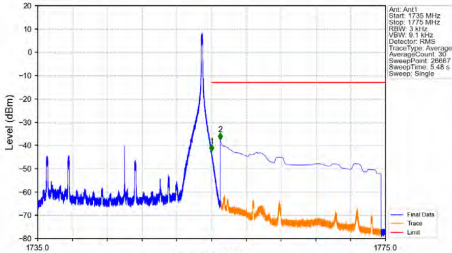
Band4_20MHz_64QAM_HCH_1745MHz_RB_1_99_NTNV
