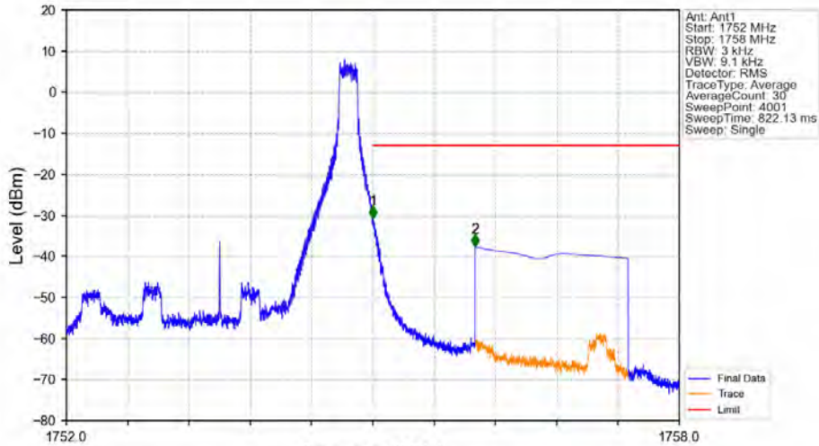
Band4_3MHz_64QAM_HCH_1753.5MHz_RB_1_14_NTNV
