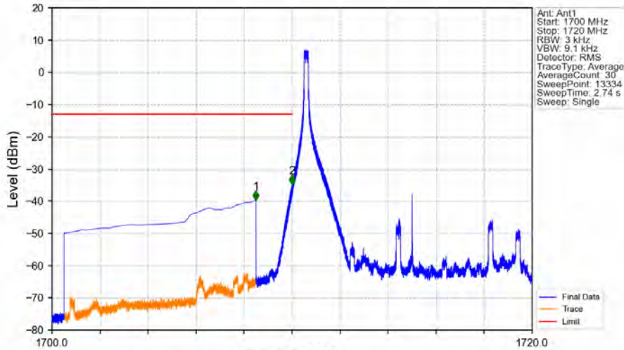
Band4_10MHz_64QAM_LCH_1715MHz_RB_1_0_NTNV
