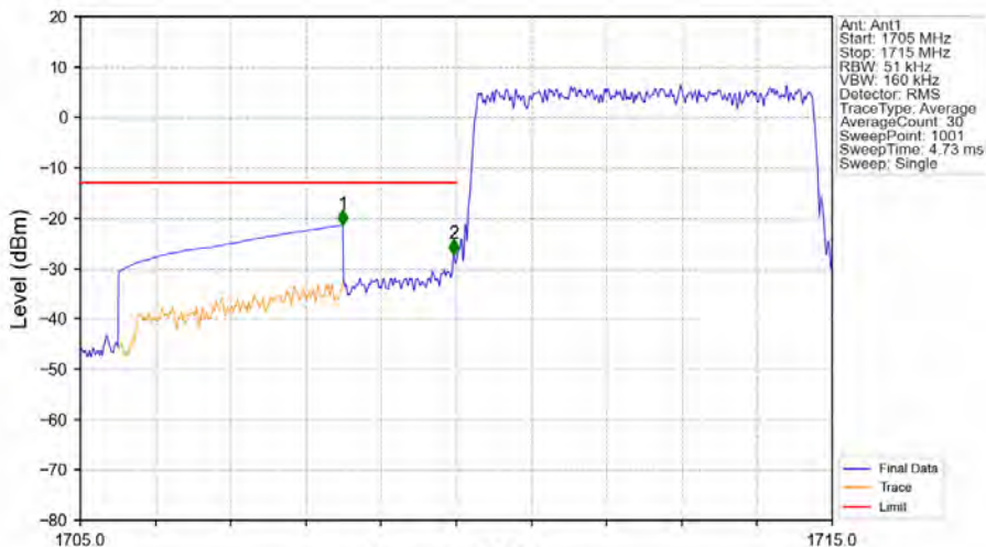
Band4_5MHz_QPSK_LCH_1712.5MHz_RB_25_0_NTNV
