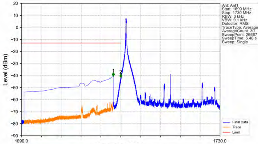
Band4_20MHz_64QAM_LCH_1720MHz_RB_1_0_NTNV
