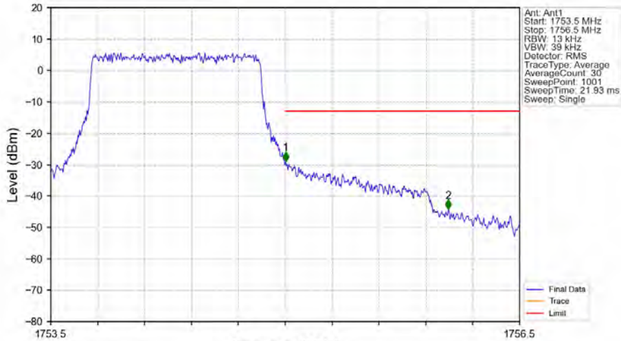
Band4_1.4MHz_QPSK_HCH_1754.3MHz_RB_6_0_NTV
