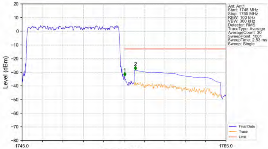
Band4_10MHz_16QAM_HCH_1750MHz_RB_50_0_NTNV
