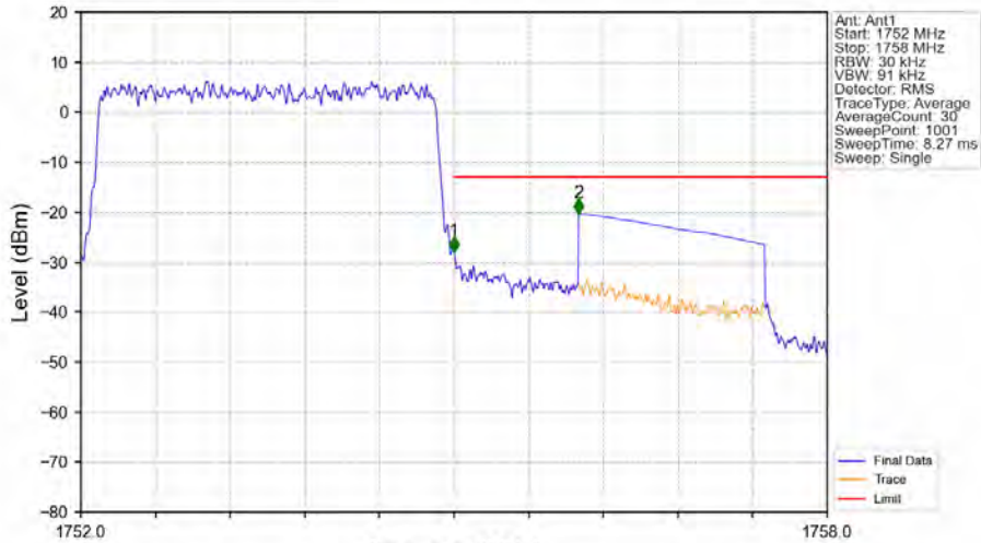
Band4_3MHz_QPSK_HCH_1753.5MHz_RB_15_0_NTNV
