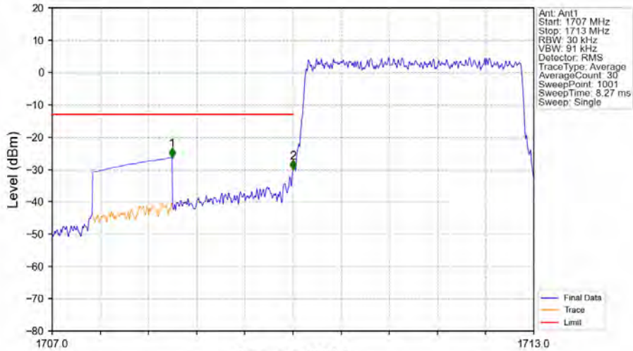
Band4_3MHz_16QAM_LCH_1711.5MHz_RB_15_0_NTV
