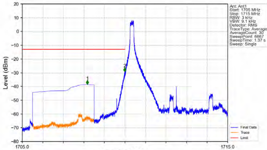
Band4_5MHz_16QAM_LCH_1712.5MHz_RB_1_0_NTNV
