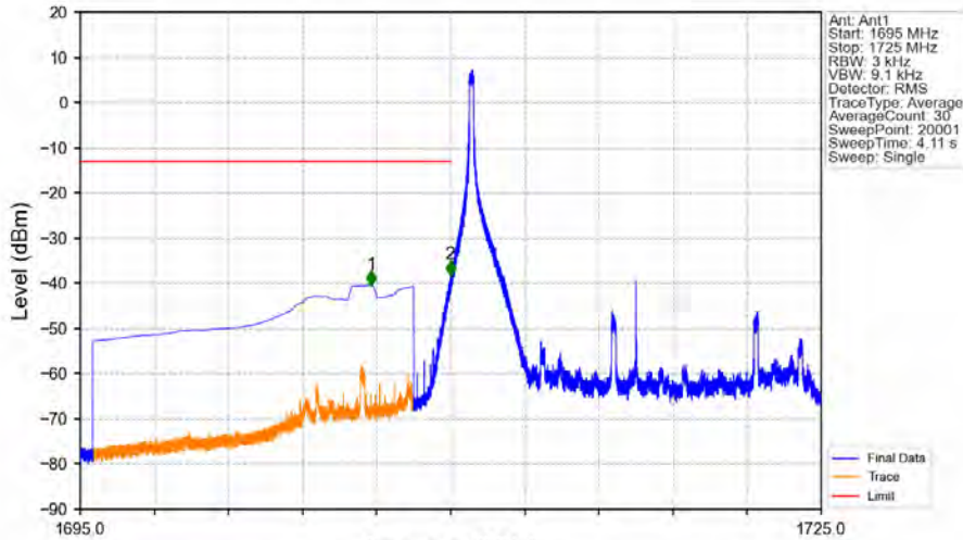
Band4_15MHz_64QAM_LCH_1717.5MHz_RB_1_0_NTV
