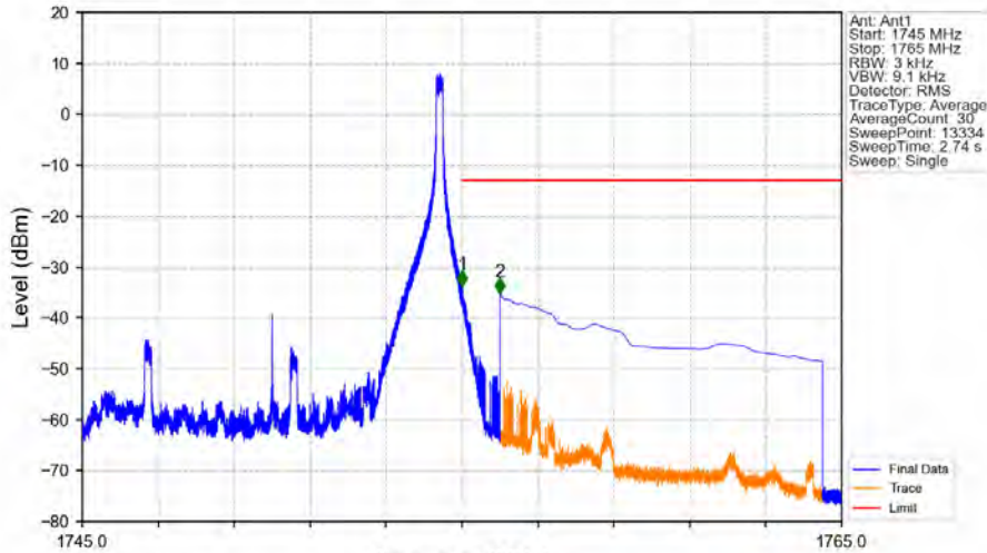
Band4_10MHz_16QAM_HCH_1750MHz_RB_1_49_NTNV
