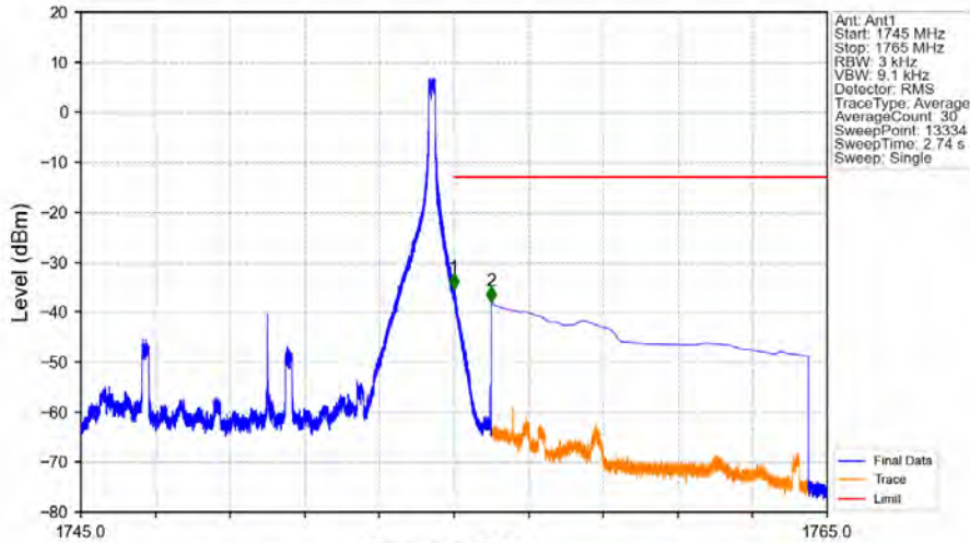
Band4_10MHz_64QAM_HCH_1750MHz_RB_1_49_NTNV
