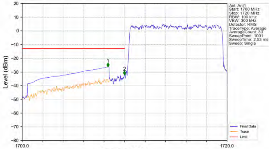
Band4_10MHz_64QAM_LCH_1715MHz_RB_50_0_NTNV
