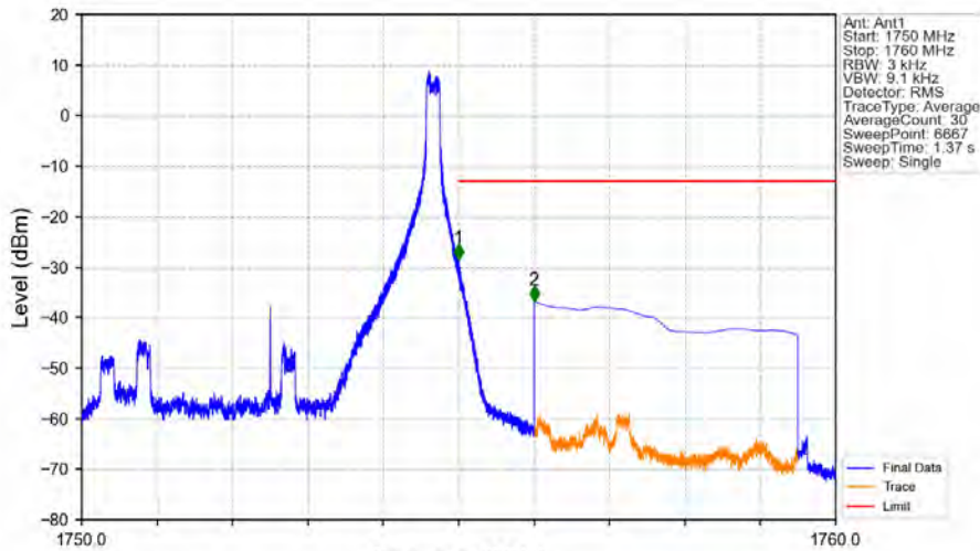
Band4_5MHz_QPSK_HCH_1752.5MHz_RB_1_24_NTNV
