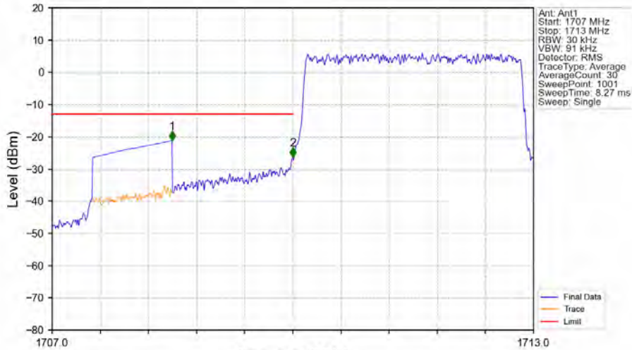
Band4_3MHz_QPSK_LCH_1711.5MHz_RB_15_0_NTNV
