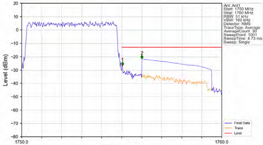
Band4_5MHz_QPSK_HCH_1752.5MHz_RB_25_0_NTNV
