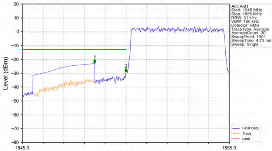
Band2_5MHz_16QAM_LCH_1852.5MHz_RB_25_0_NTV
