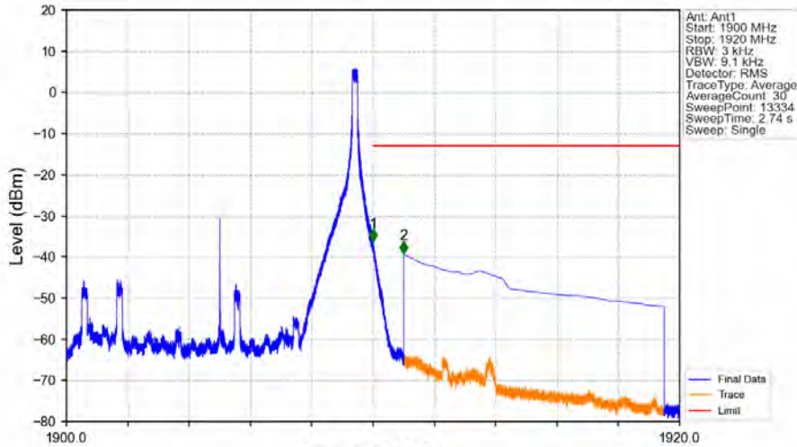
Band2_10MHz_64QAM_HCH_1905MHz_RB_1_49_NTNV
