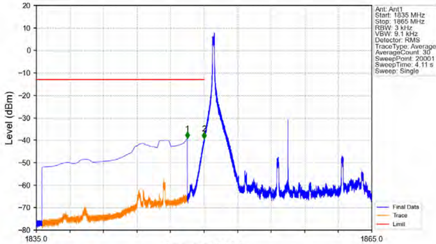
Band2_15MHz_16QAM_LCH_1857.5MHz_RB_1_0_NTV
