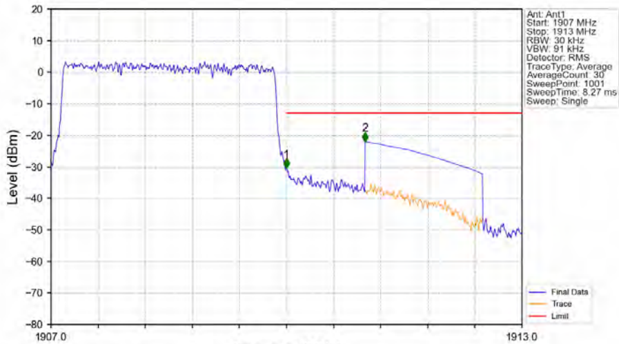
Band2_3MHz_64QAM_HCH_1908.5MHz_RB_15_0_NTNV
