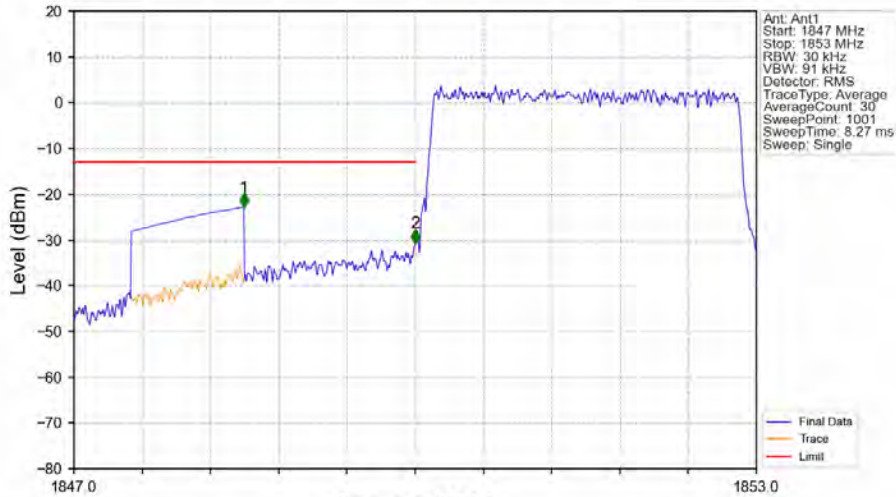
Band2_3MHz_16QAM_LCH_1851.5MHz_RB_15_0_NTV
