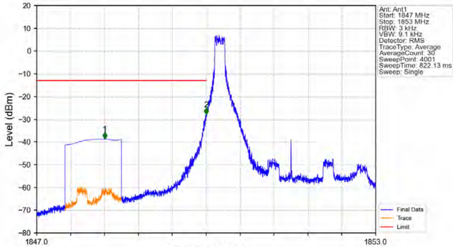
Band2_3MHz_16QAM_LCH_1851.5MHz_RB_1_0_NTNV
