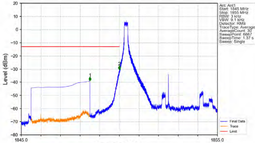
Band2_5MHz_64QAM_LCH_1852.5MHz_RB_1_0_NTNV
