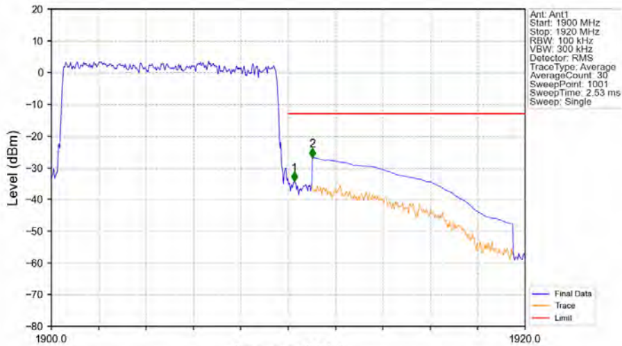
Band2_10MHz_64QAM_HCH_1905MHz_RB_50_0_NTNV
