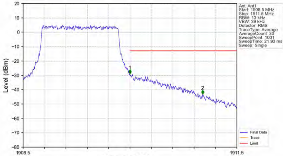
Band2_1.4MHz_QPSK_HCH_1909.3MHz_RB_6_0_NTV
