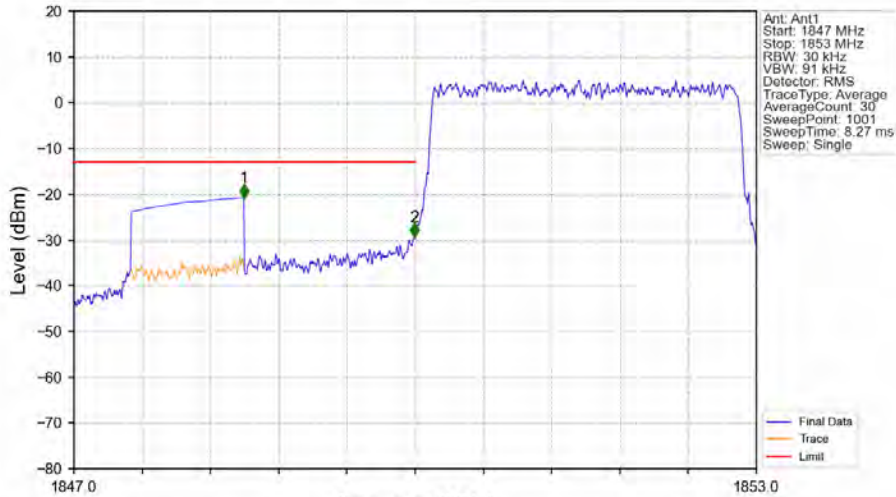
Band2_3MHz_QPSK_LCH_1851.5MHz_RB_15_0_NTNV
