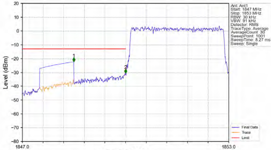
Band2_3MHz_64QAM_LCH_1851.5MHz_RB_15_0_NTV
