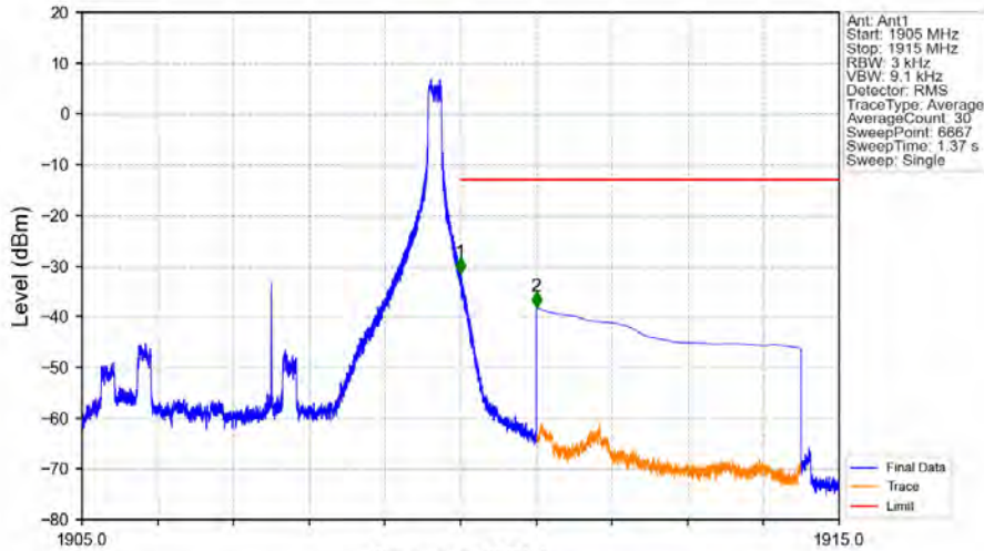
Band2_5MHz_QPSK_HCH_1907.5MHz_RB_1_24_NTNV
