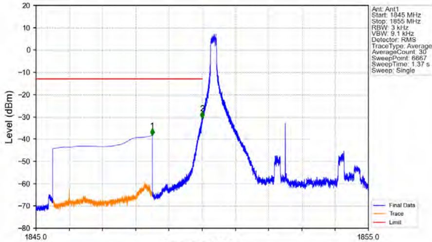
Band2_5MHz_16QAM_LCH_1852.5MHz_RB_1_0_NTNV
