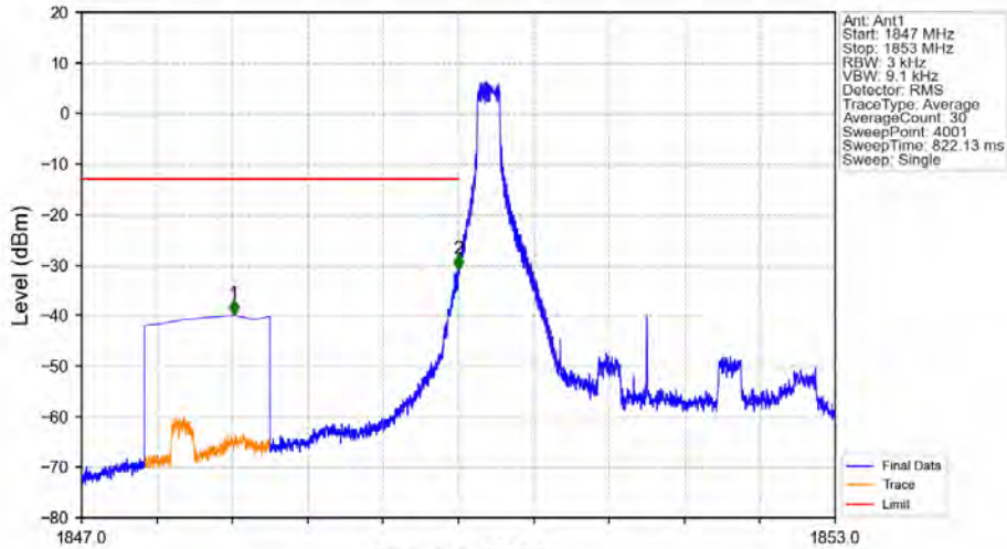
Band2_3MHz_64QAM_LCH_1851.5MHz_RB_1_0_NTNV
