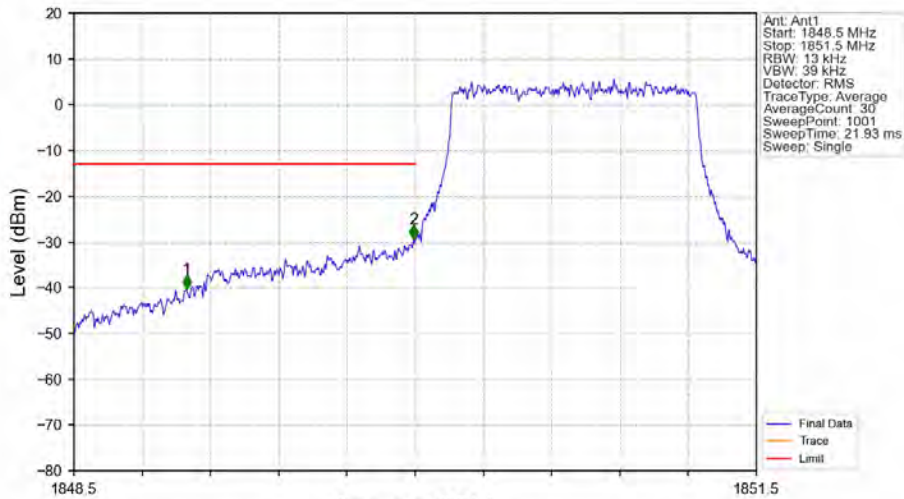
Band2_1.4MHz_QPSK_LCH_1850.7MHz_RB_6_0_NTNV
