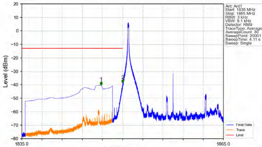
Band2_15MHz_64QAM_LCH_1857.5MHz_RB_1_0_NTV
