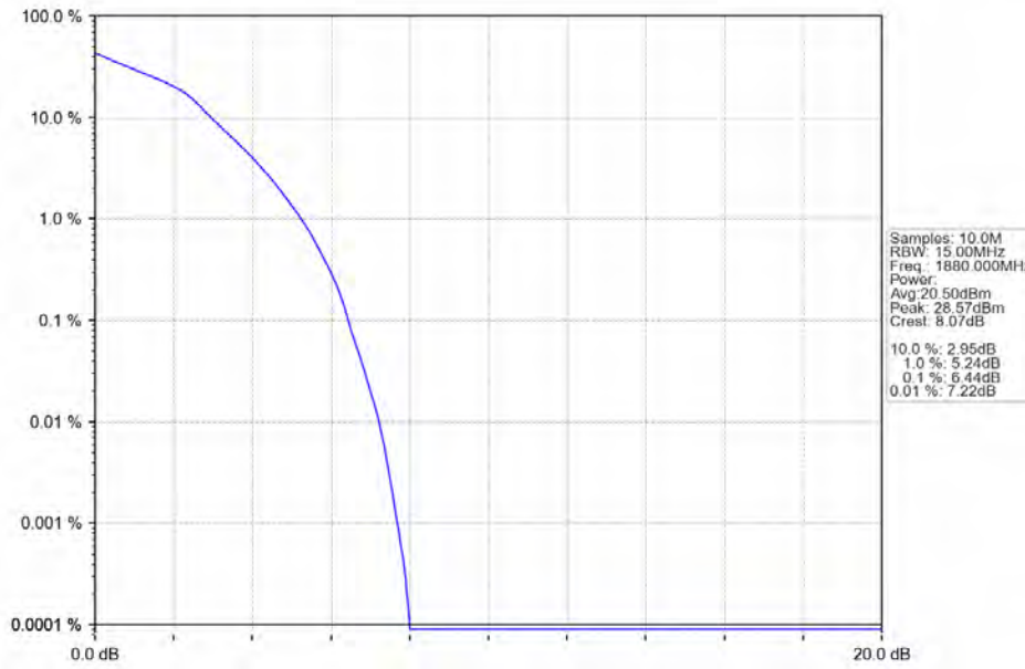
Band2_15MHz_16QAM_MCH_1880MHz_RB_75_0_NTNV
