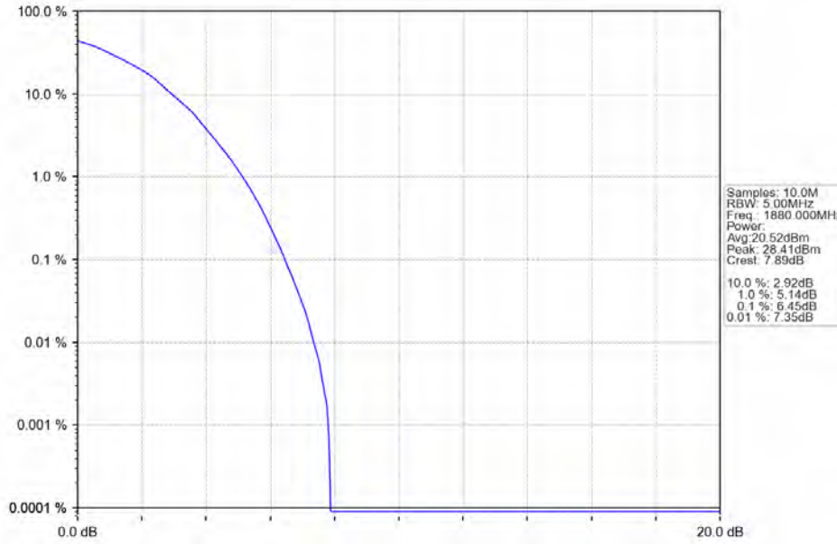
Band2_5MHz_64QAM_MCH_1880MHz_RB_25_0_NTNV
