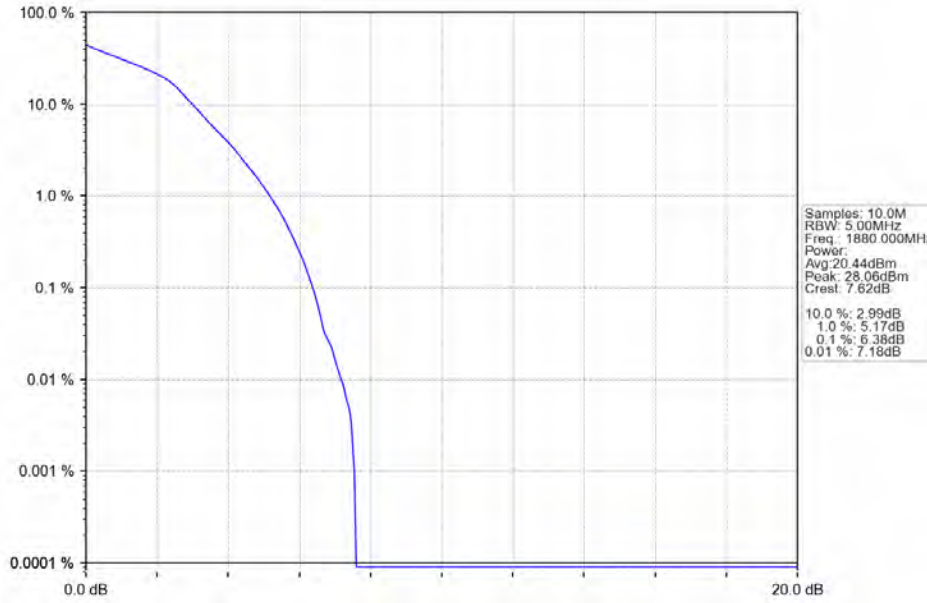
Band2_1.4MHz_16QAM_MCH_1880MHz_RB_6_0_NTNV
