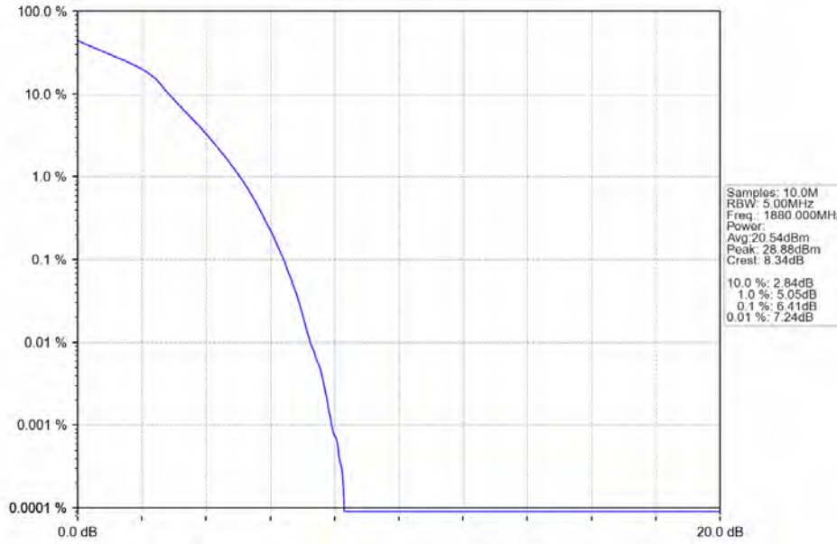
Band2_5MHz_16QAM_MCH_1880MHz_RB_25_0_NTNV
