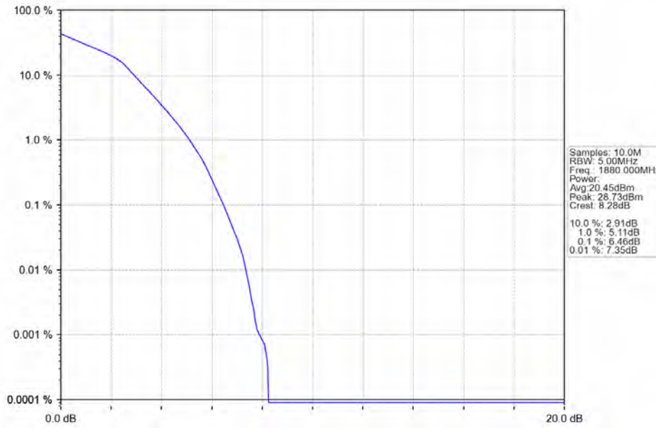
Band2_3MHz_16QAM_MCH_1880MHz_RB_15_0_NTNV
