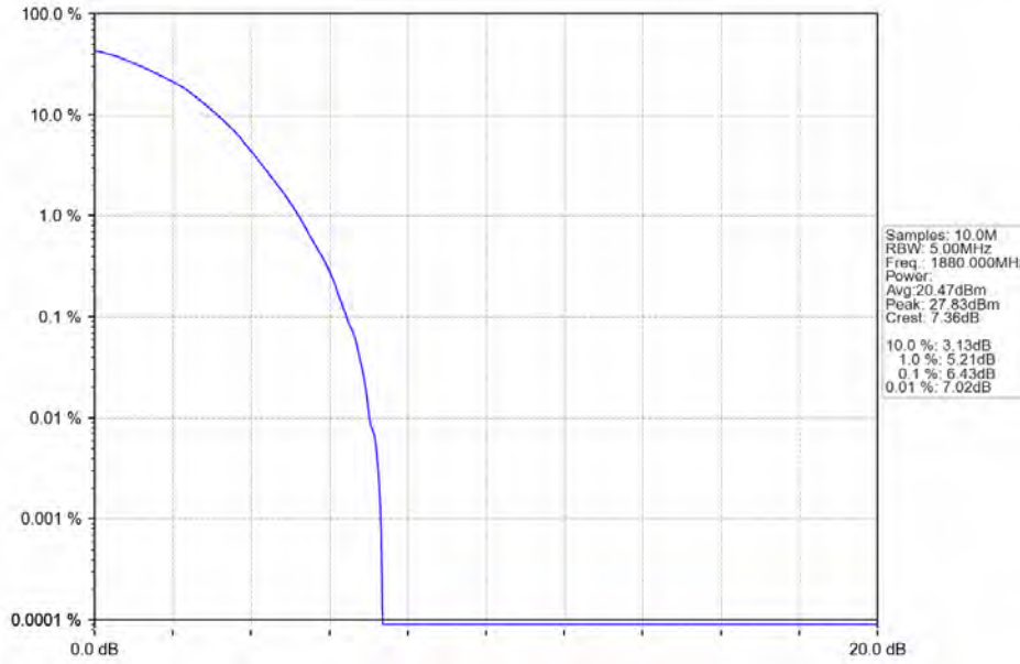
Band2_1.4MHz_64QAM_MCH_1880MHz_RB_6_0_NTNV
