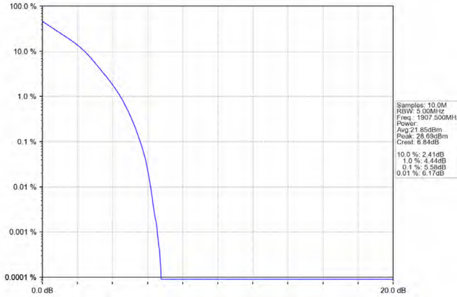
Band2_5MHz_QPSK_HCH_1907.5MHz_RB_25_0_NTNV
