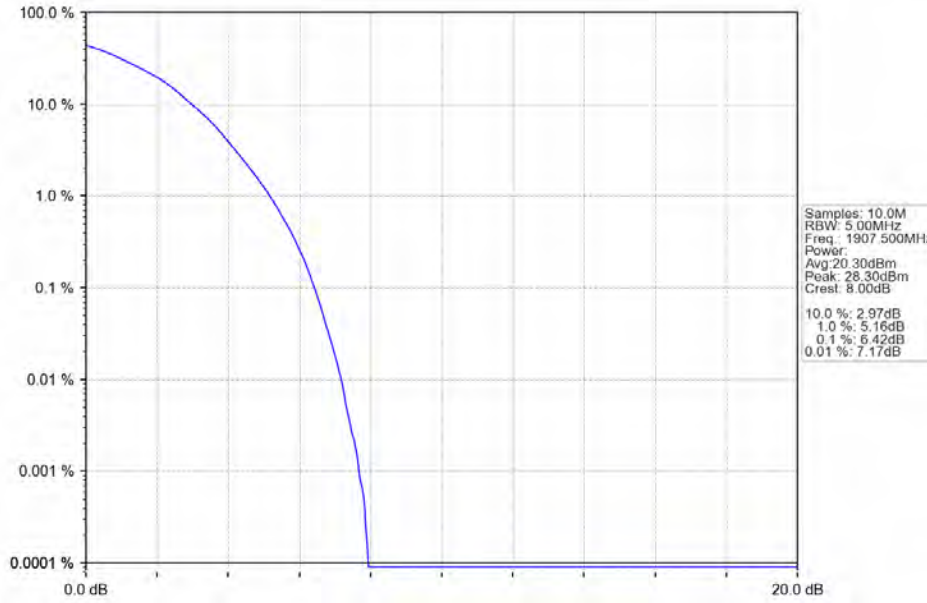
Band2_5MHz_64QAM_HCH_1907.5MHz_RB_25_0_NTNV
