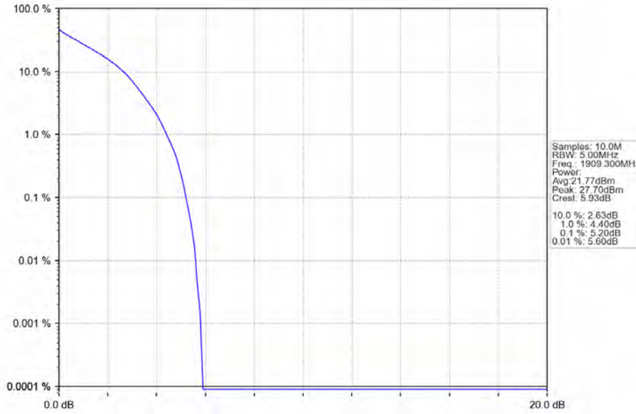
Band2_1.4MHz_QPSK_HCH_1909.3MHz_RB_6_0_NTNV
