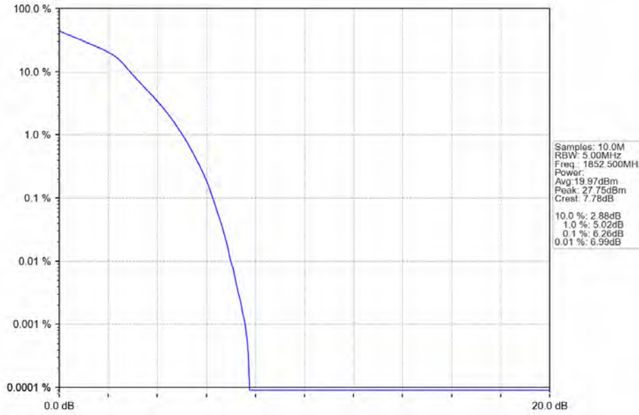
Band2_5MHz_16QAM_LCH_1852.5MHz_RB_25_0_NTNV
