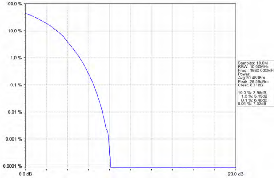
Band2_10MHz_64QAM_MCH_1880MHz_RB_50_0_NTNV
