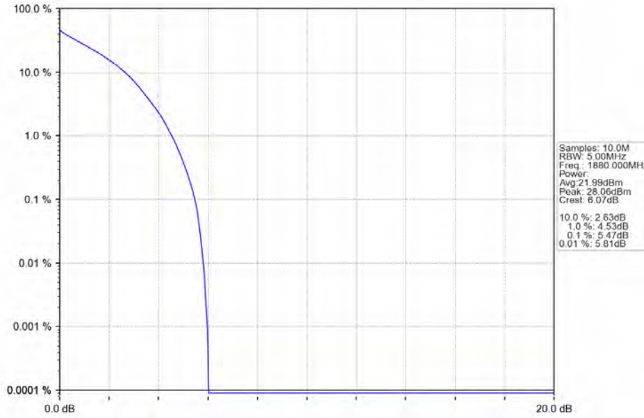
Band2_1.4MHz_QPSK_MCH_1880MHz_RB_6_0_NTNV
