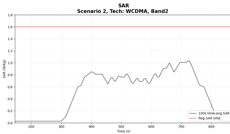
Figure 6-23 Time-averaged SAR for case 2.10(WCDMA B2)
