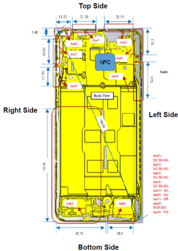
Figure 6-1 Antenna placement of the phone
