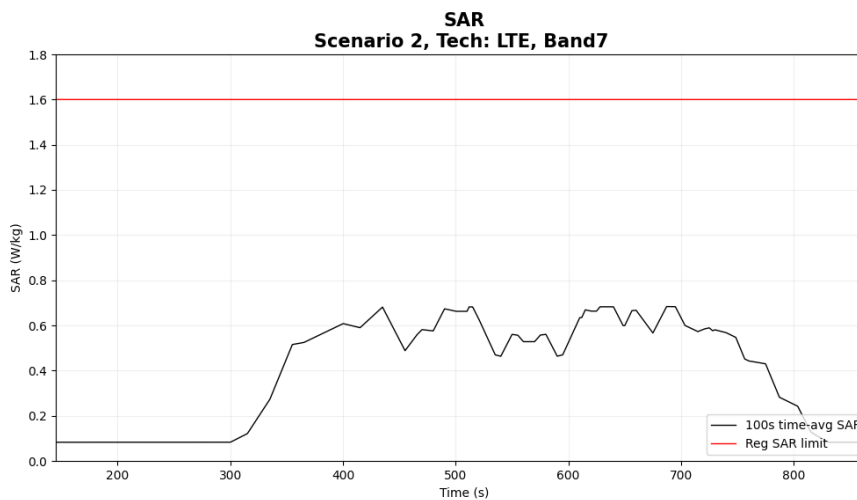
Figure 6-19 Time-averaged SAR for case 2.8(LTE B7)
