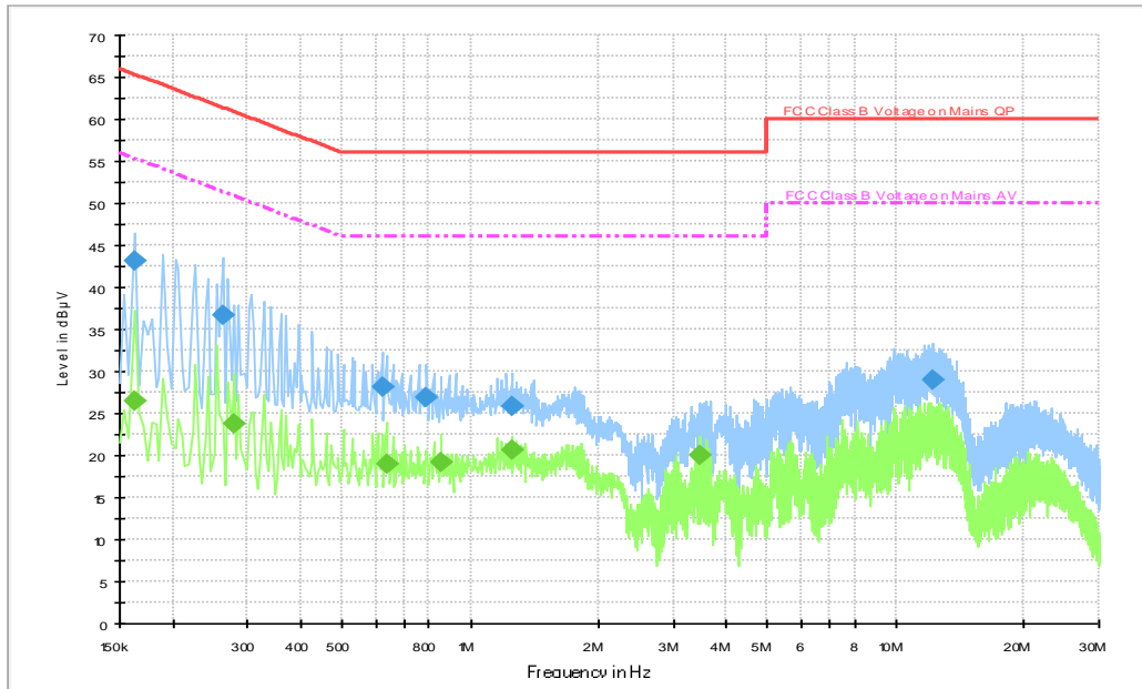
Fig.B.8.3 AC Powerline Conducted Emission-Bluetooth (AE2-2)
