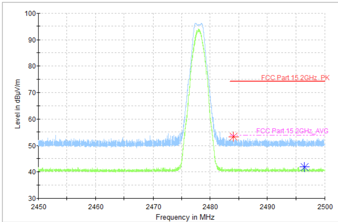
Fig.21. Frequency Band Edges: BLE 5.0, GFSK, 2478 MHz, Hopping Off, 2.45 GHz - 2.50GHz
