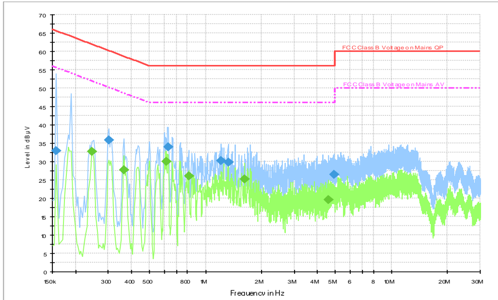
Fig.B.8.1 AC Powerline Conducted Emission-Bluetooth (AE2-1)
