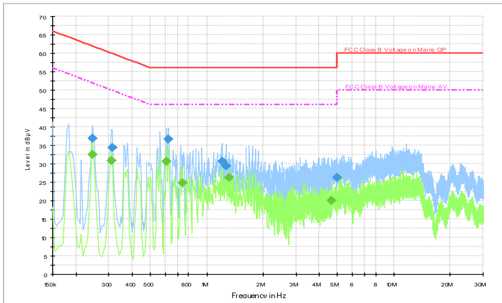
Fig.B.8.2 AC Powerline Conducted Emission-Idle (AE2-1)
