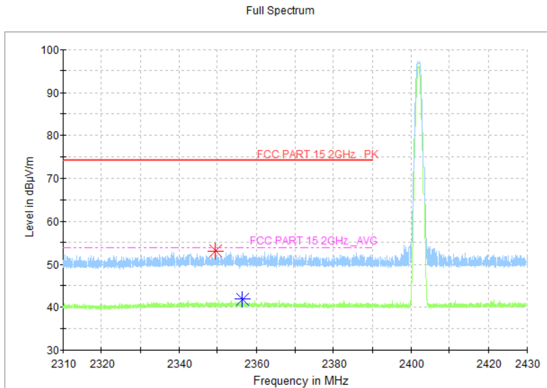
Fig.18. Frequency Band Edges: BLE 4.0, GFSK, 2402 MHz, Hopping Off, 2.31 GHz – 2.43GHz
