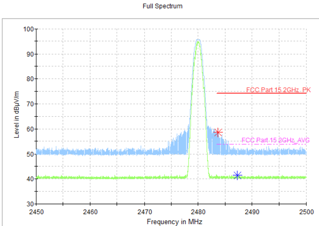
Fig.19. Frequency Band Edges: BLE 4.0, GFSK, 2480 MHz, Hopping Off, 2.45 GHz - 2.50GHz
