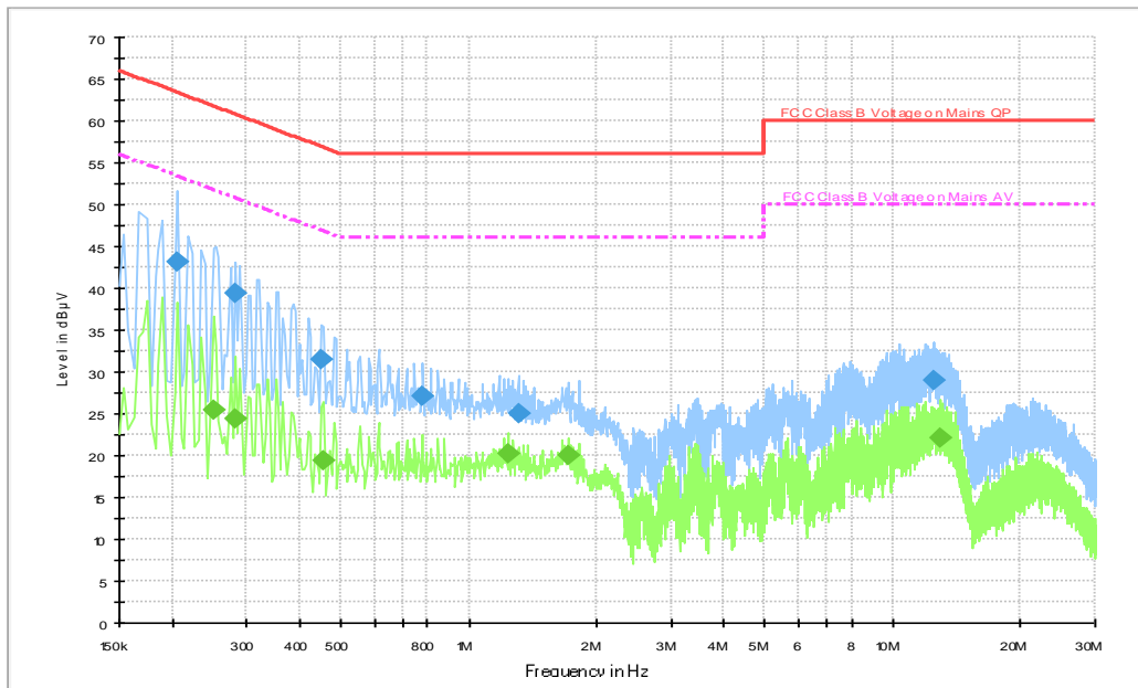
Fig.B.10.3 AC Powerline Conducted Emission-Bluetooth(AE2-2)
