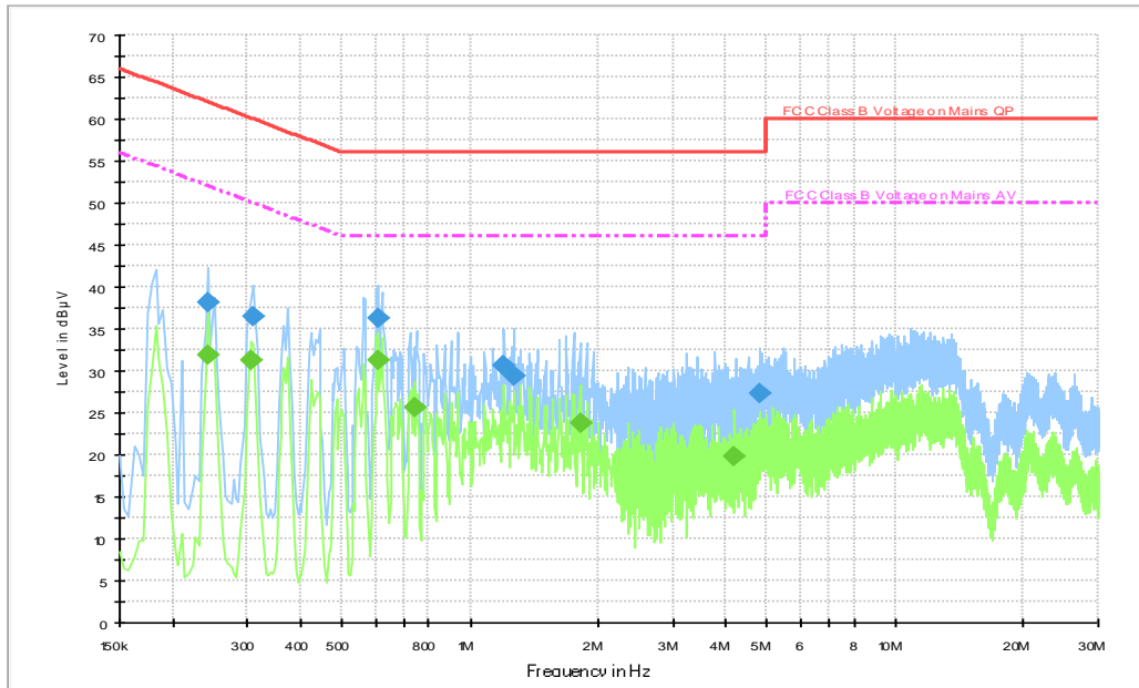
Fig.B.10.1 AC Powerline Conducted Emission-Bluetooth(AE2-1)
