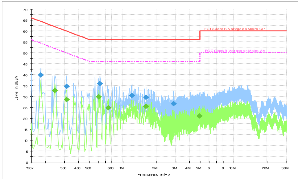
Fig.B.10.2 AC Powerline Conducted Emission-Idle(AE2-1)
