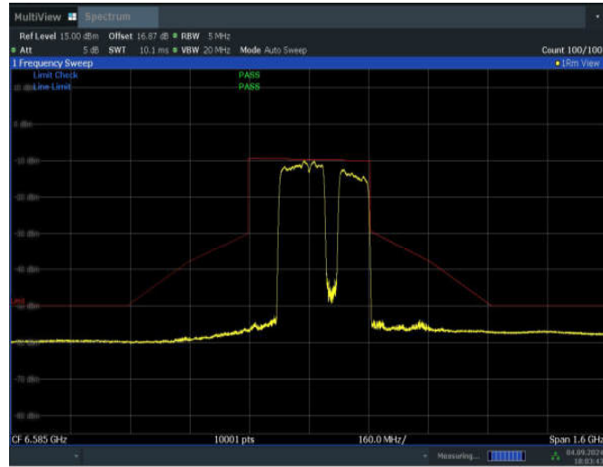
11BE320MIMO_Ant1_6585_2*996+484_Non-OFDMA_10
