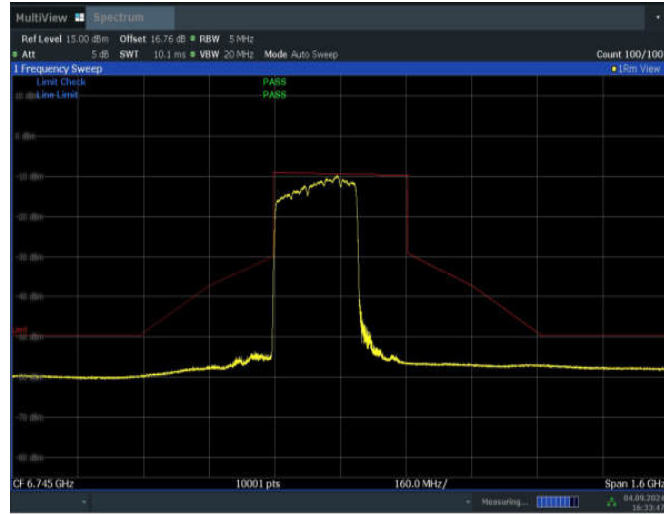
11BE320MIMO_Ant1_6745_2*996+484_Non-OFDMA_6
