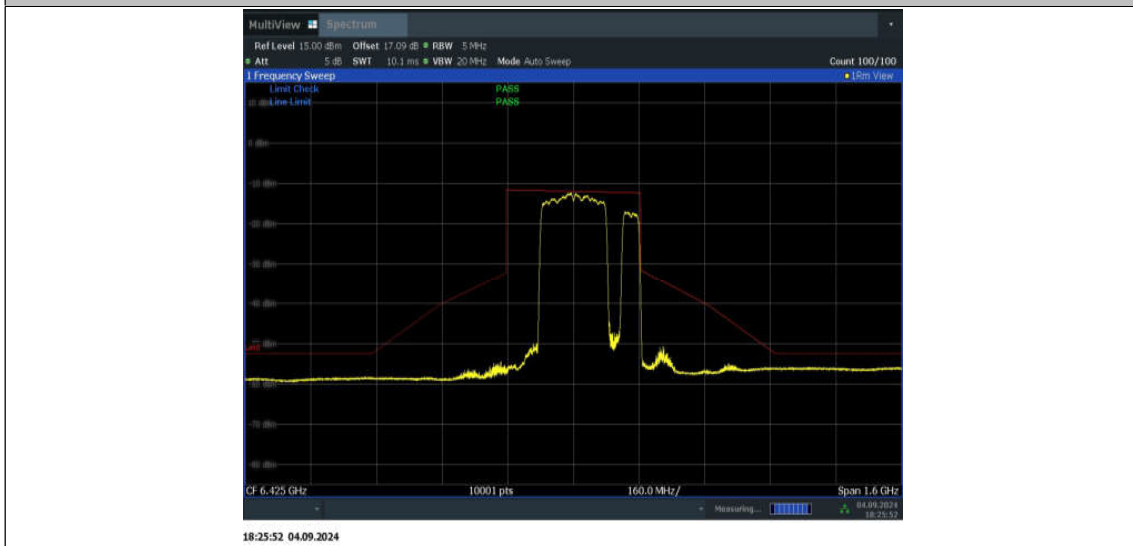
11BE320MIMO_Ant2_6425_2*996+484_Non-OFDMA_12
