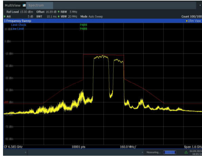
11BE320MIMO_Ant2_6585_2*996+484_Non-OFDMA_10
