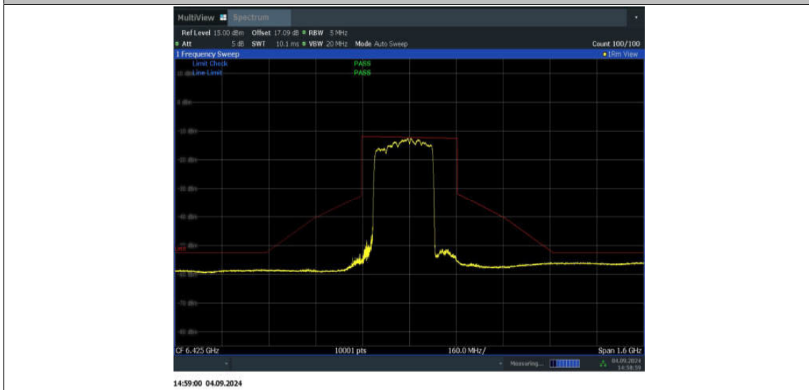
11BE320MIMO_Ant2_6425_2*996+484_Non-OFDMA_2
