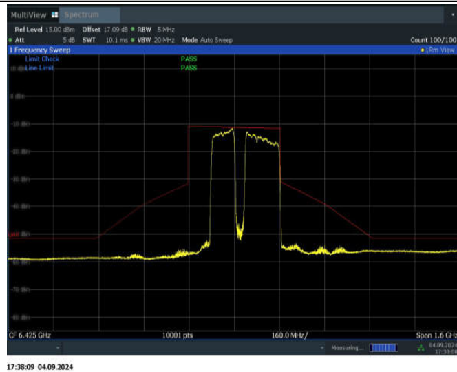
11BE320MIMO_Ant2_6425_2*996+484_Non-OFDMA_10
