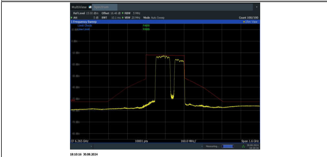
11BE320MIMO_Ant2_6265_2*996+484_Non-OFDMA_10
