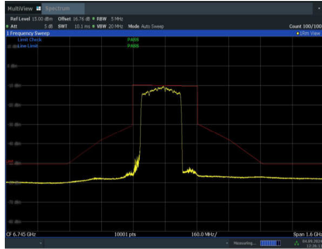
11BE320MIMO_Ant1_6745_2*996+484_Non-OFDMA_1
