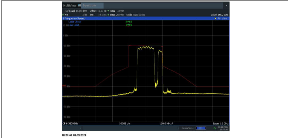
11BE320MIMO_Ant1_6585_2*996+484_Non-OFDMA_12
