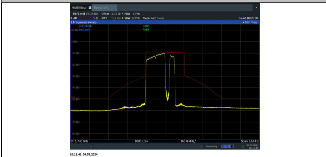
11BE320MIMO_Ant1_6745_2*996+484_Non-OFDMA_5
