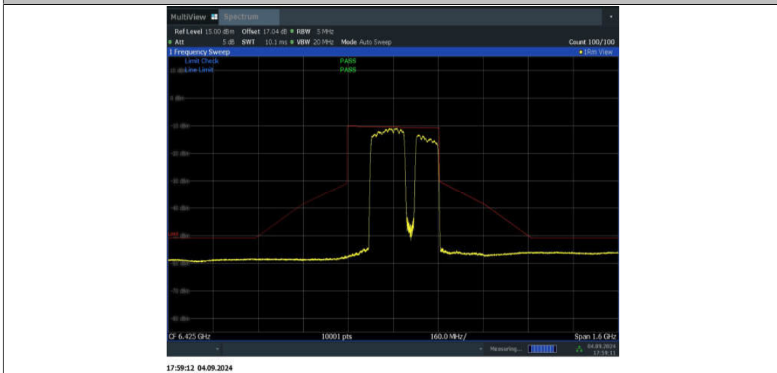
11BE320MIMO_Ant1_6425_2*996+484_Non-OFDMA_11
