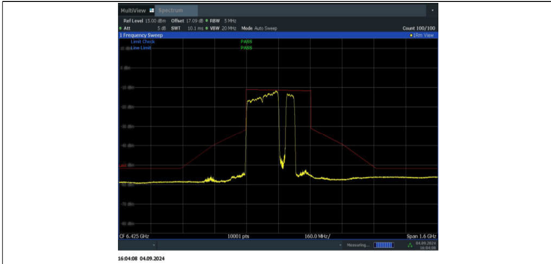
11BE320MIMO_Ant2_6425_2*996+484_Non-OFDMA_6
