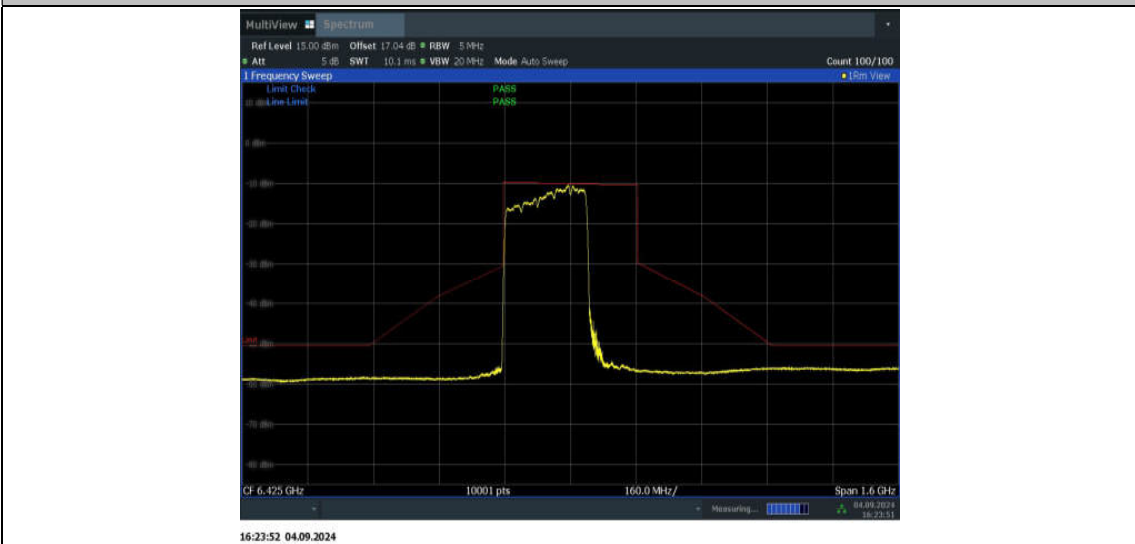
11BE320MIMO_Ant1_6425_2*996+484_Non-OFDMA_6
