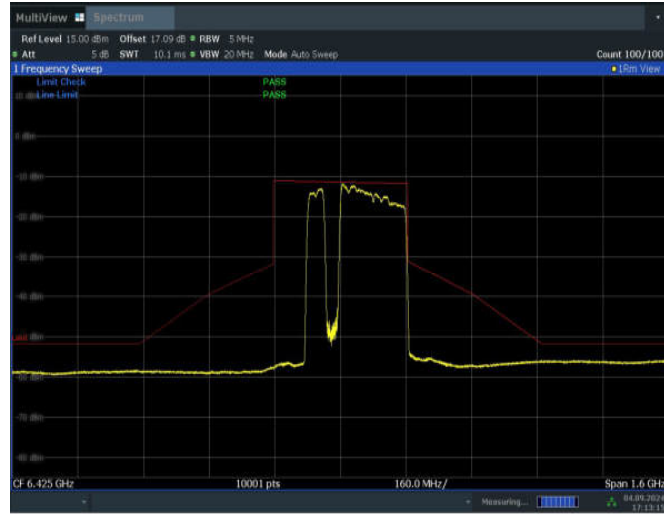
11BE320MIMO_Ant2_6425_2*996+484_Non-OFDMA_8
