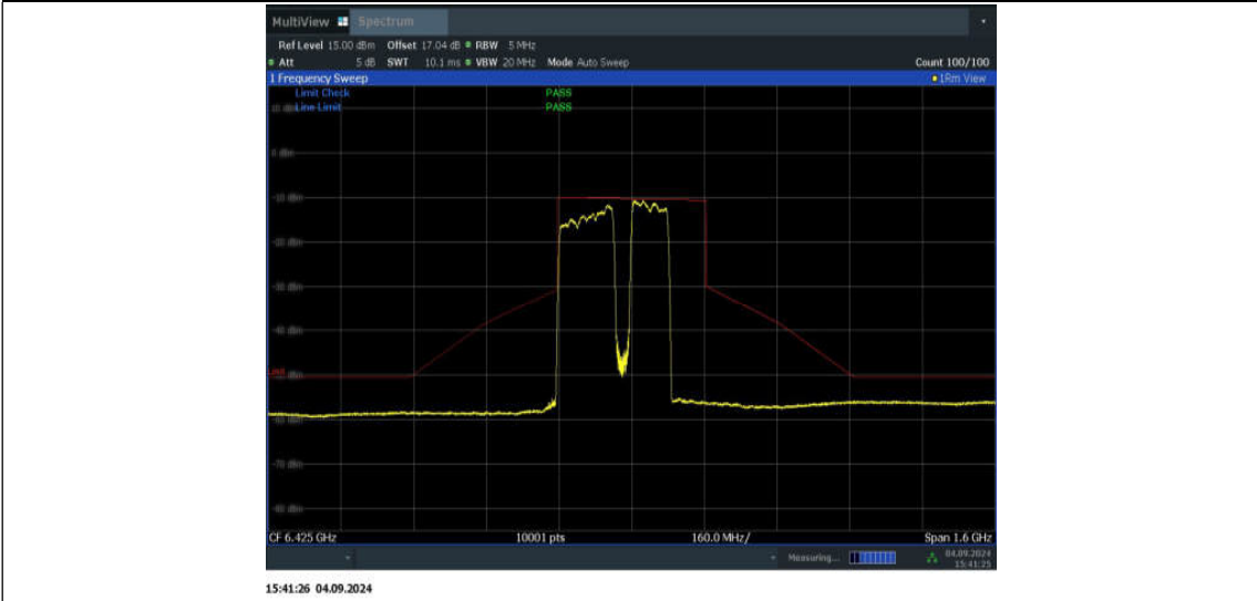
11BE320MIMO_Ant1_6425_2*996+484_Non-OFDMA_5
