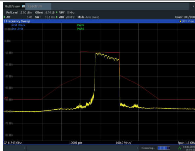
11BE320MIMO_Ant1_6745_2*996+484_Non-OFDMA_7
