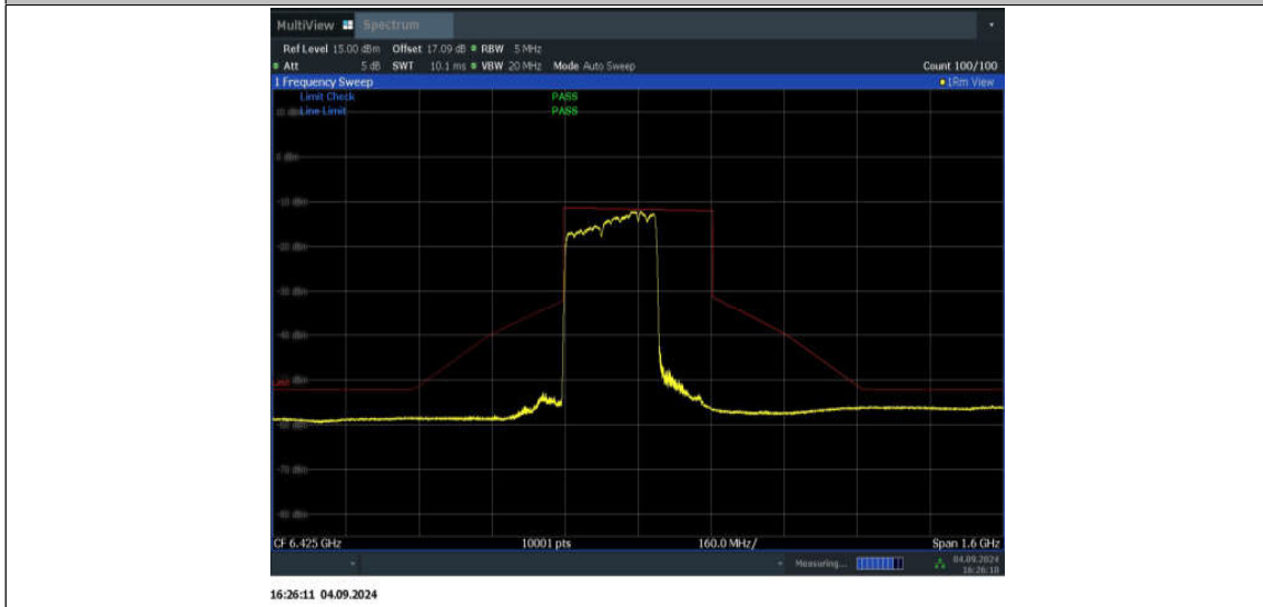
11BE320MIMO_Ant2_6425_2*996+484_Non-OFDMA_7
