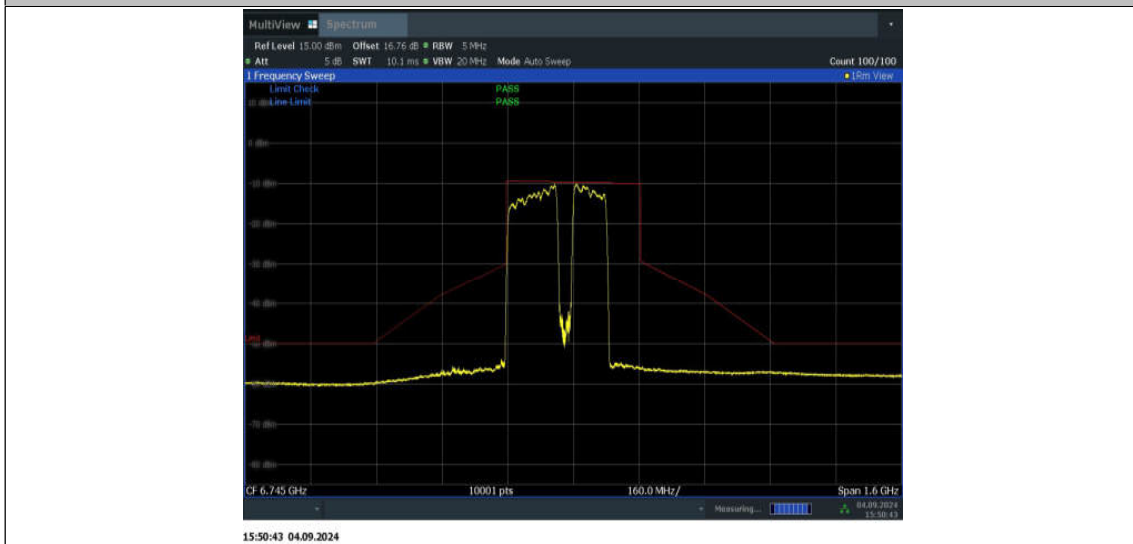
11BE320MIMO_Ant1_6745_2*996+484_Non-OFDMA_5
