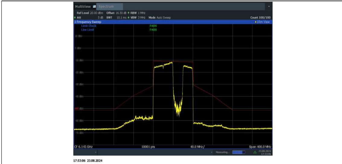
11BE80MIMO_Ant1_6145_484+242_Non-OFDMA_4
