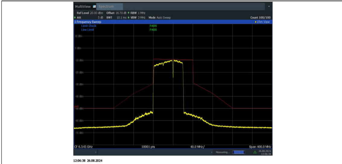
11BE80MIMO_Ant2_6545_484+242_Non-OFDMA_1
