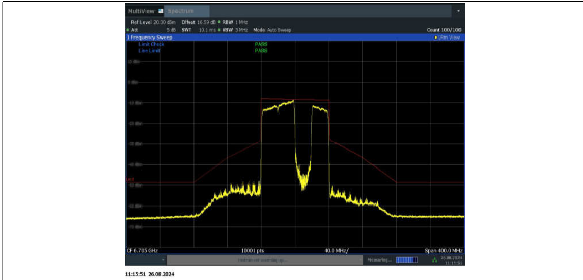
11BE80MIMO_Ant1_6705_484+242_Non-OFDMA_4
