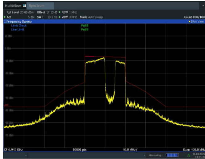
11BE80MIMO_Ant1_6945_484+242_Non-OFDMA_3
