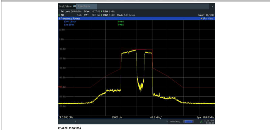
11BE80MIMO_Ant1_5985_484+242_Non-OFDMA_3
