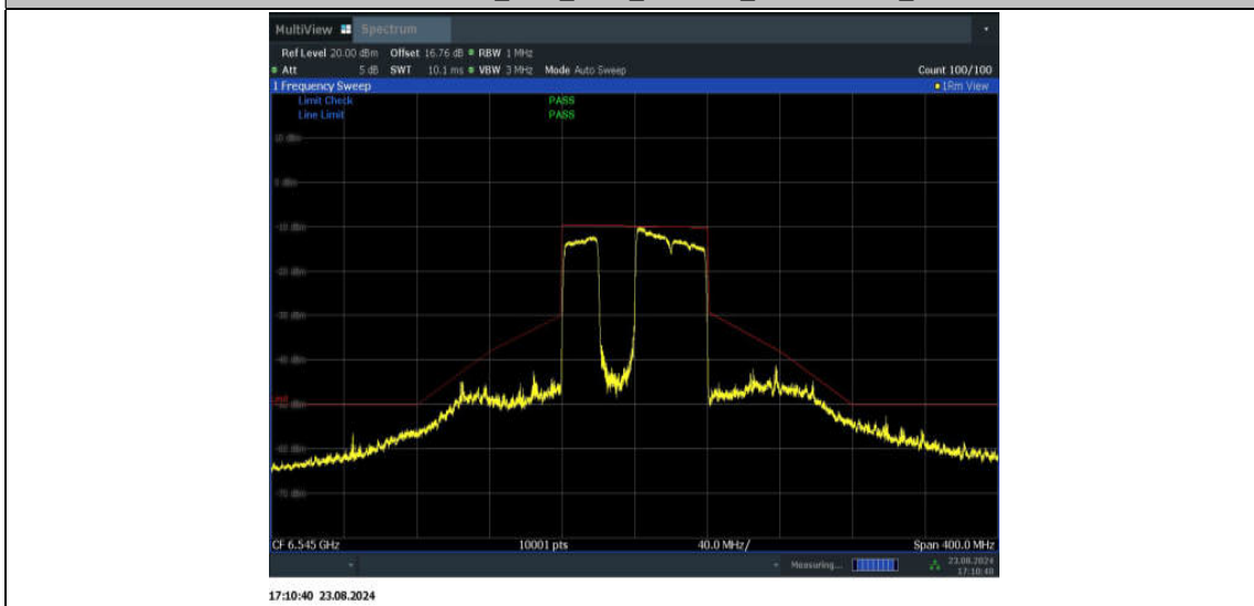
11BE80MIMO_Ant2_6545_484+242_Non-OFDMA_2
