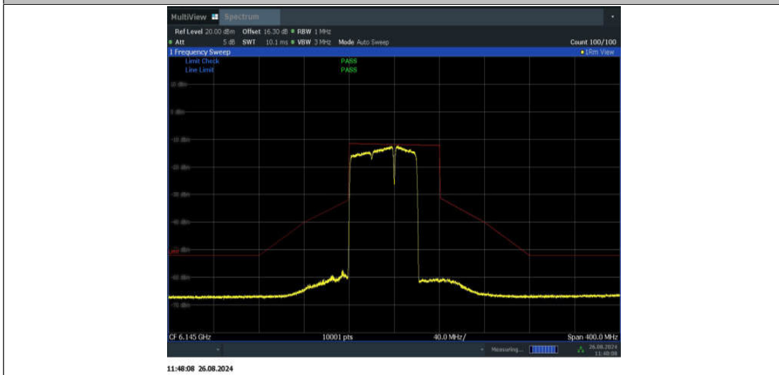
11BE80MIMO_Ant2_6145_484+242_Non-OFDMA_1
