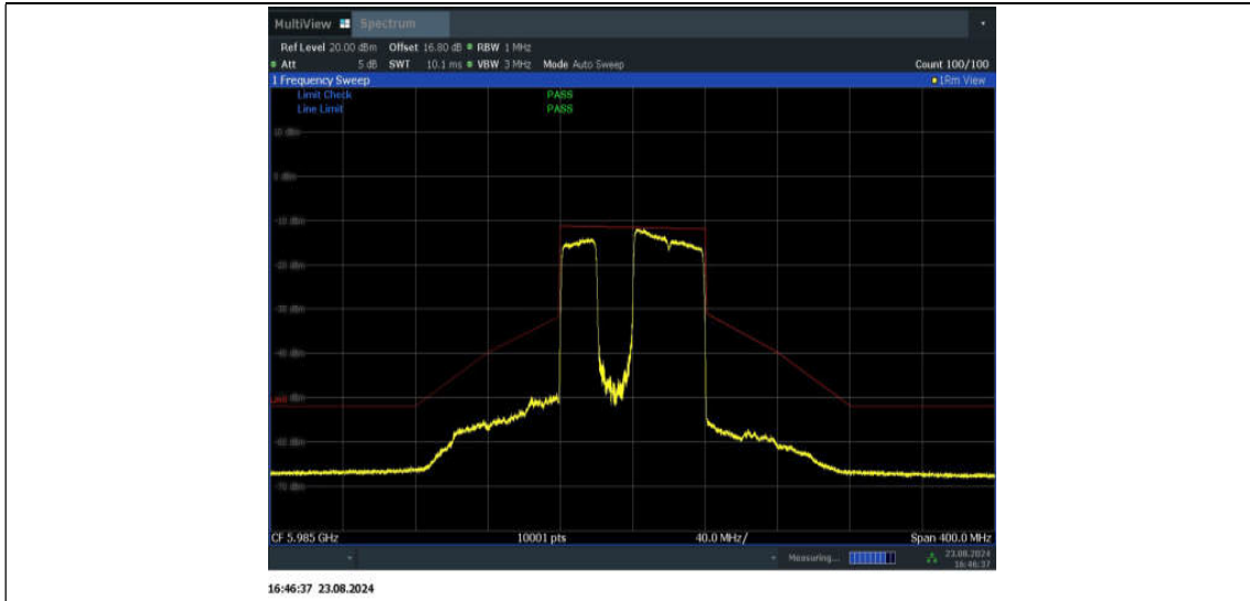
11BE80MIMO_Ant2_5985_484+242_Non-OFDMA_3
