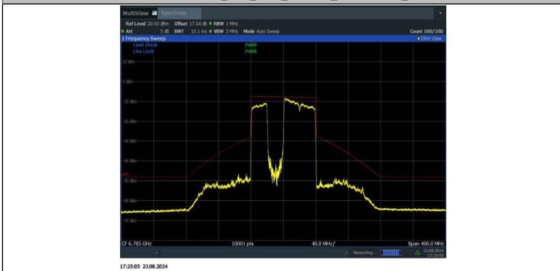
11BE80MIMO_Ant1_6785_484+242_Non-OFDMA_2
