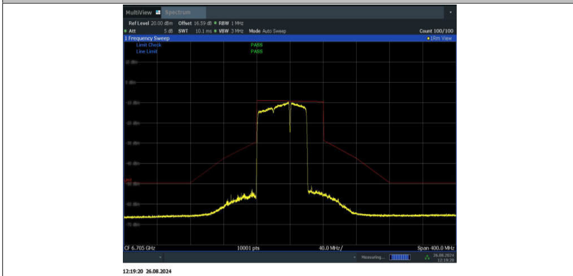
11BE80MIMO_Ant2_6705_484+242_Non-OFDMA_1
