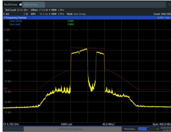
11BE80MIMO_Ant1_6785_484+242_Non-OFDMA_3
