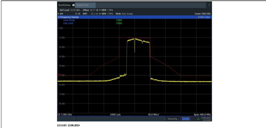
11BE80MIMO_Ant1_5985_484+242_Non-OFDMA_2
