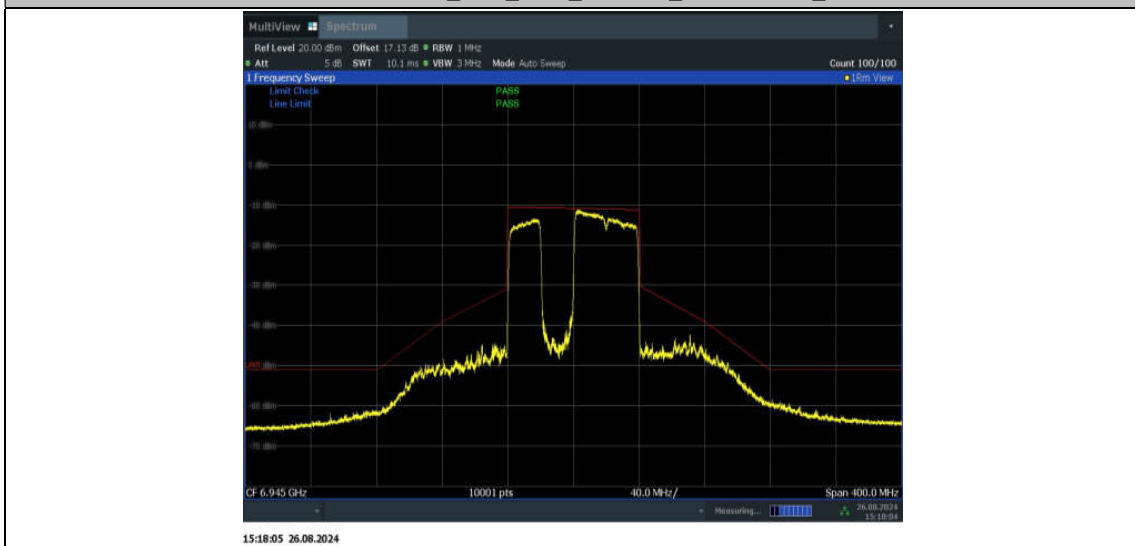
11BE80MIMO_Ant2_6945_484+242_Non-OFDMA_2
