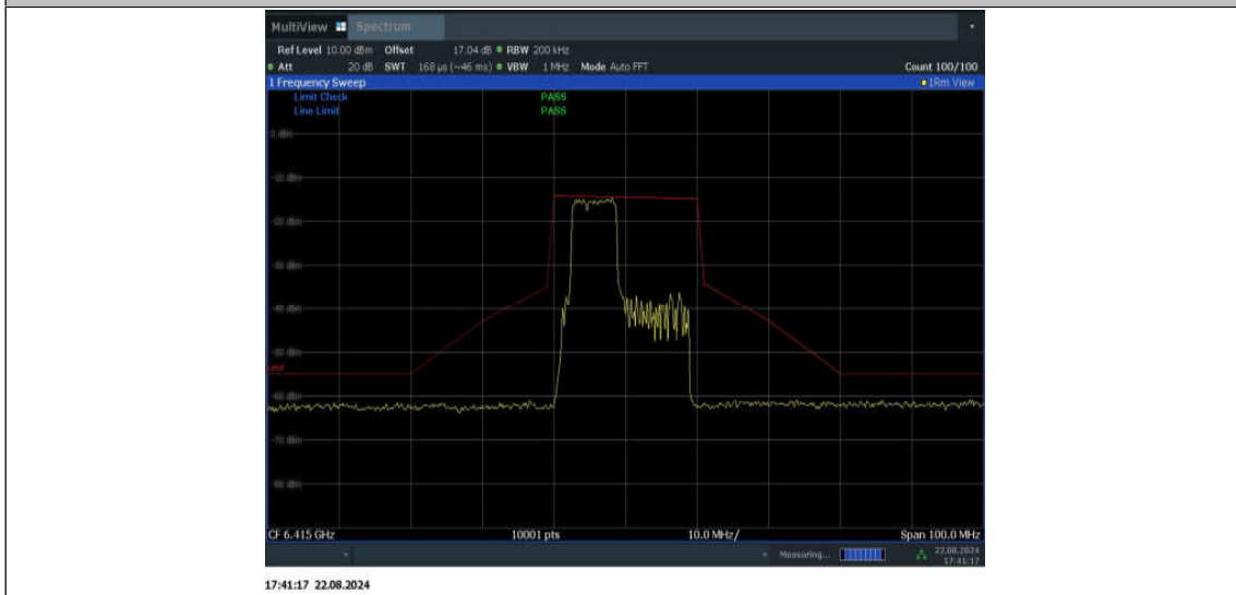
11BE20MIMO_Ant1_6415_106+26_OFDMA_1
