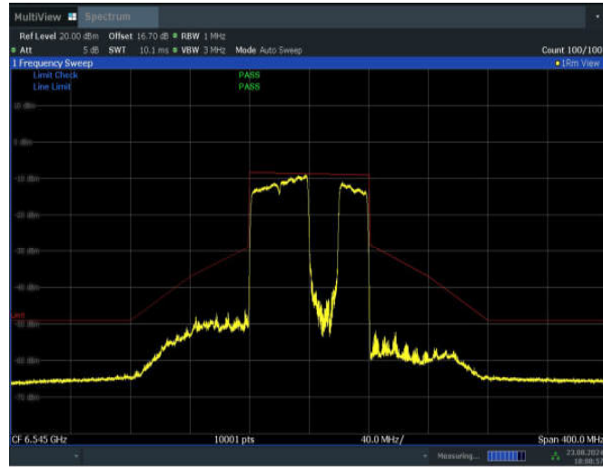
11BE80MIMO_Ant1_6545_484+242_Non-OFDMA_3
