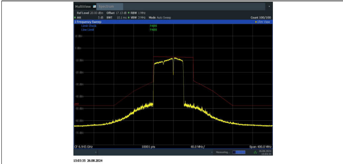
11BE80MIMO_Ant2_6945_484+242_Non-OFDMA_1
