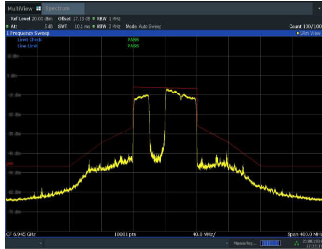
11BE80MIMO_Ant1_6945_484+242_Non-OFDMA_2
