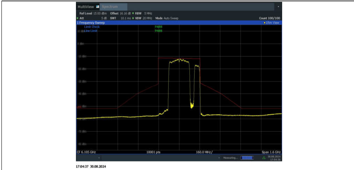
11BE320MIMO_Ant2_6105_2*996+484_Non-OFDMA_12
