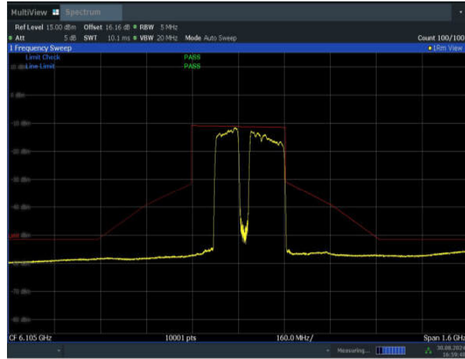
11BE320MIMO_Ant2_6105_2*996+484_Non-OFDMA_9
