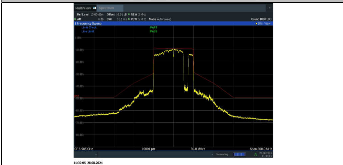
11BE160MIMO_Ant1_6985_996+484+242_Non-OFDMA_7
