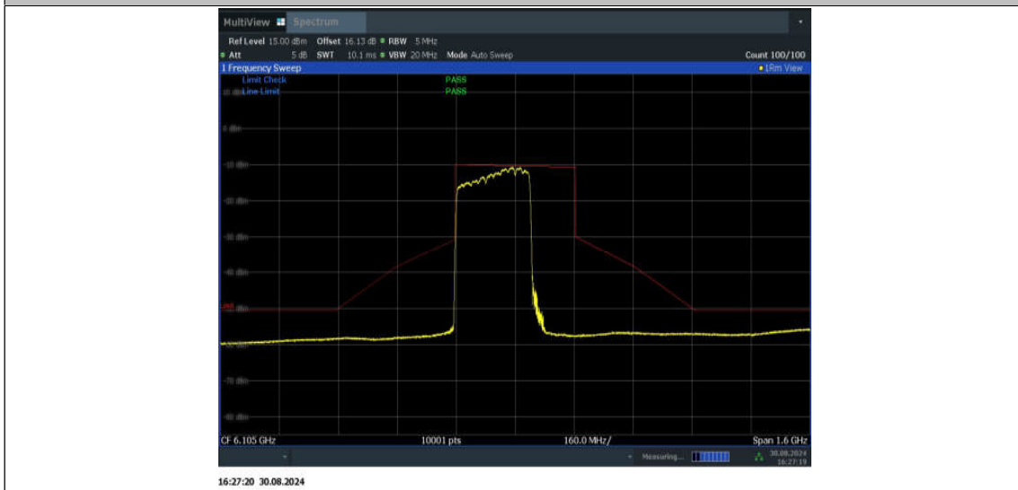
11BE320MIMO_Ant1_6105_2*996+484_Non-OFDMA_7
