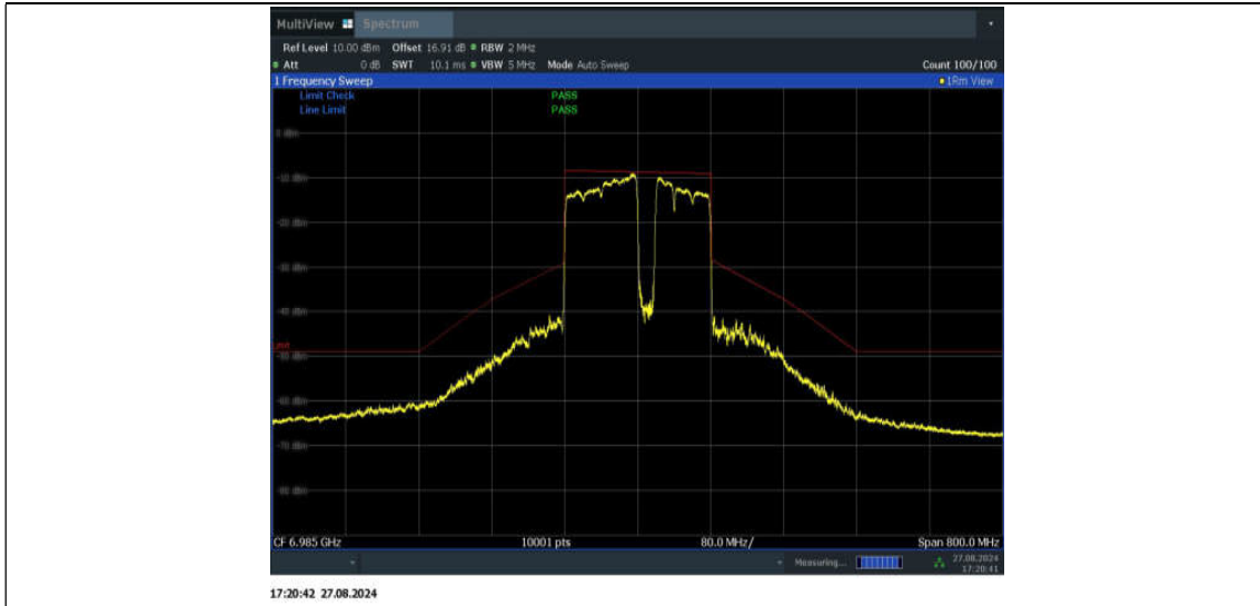
11BE160MIMO_Ant1_6985_996+484+242_Non-OFDMA_6
