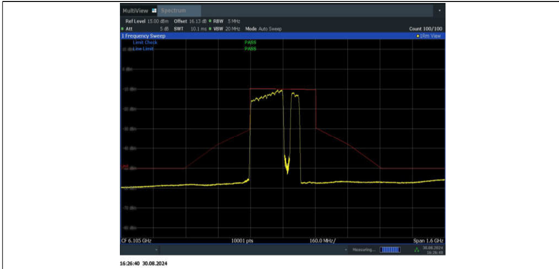
11BE320MIMO_Ant1_6105_2*996+484_Non-OFDMA_6
