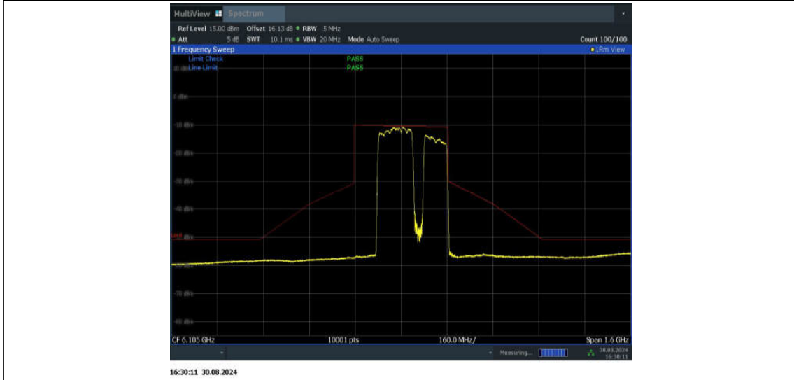
11BE320MIMO_Ant1_6105_2*996+484_Non-OFDMA_11
