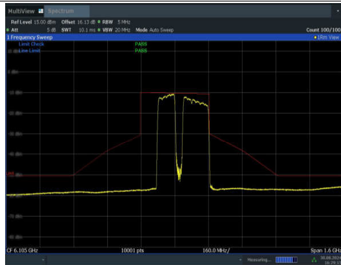
11BE320MIMO_Ant1_6105_2*996+484_Non-OFDMA_9
