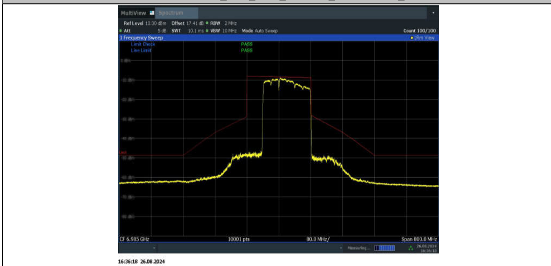
11BE160MIMO_Ant1_6985_996+484_Non-OFDMA_1
