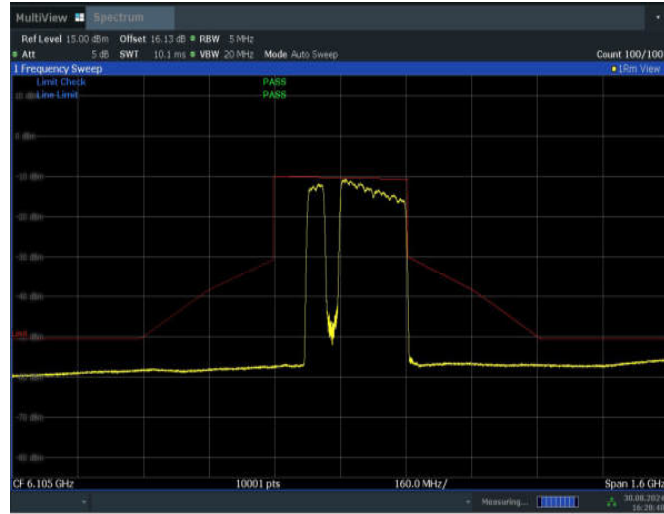
11BE320MIMO_Ant1_6105_2*996+484_Non-OFDMA_8
