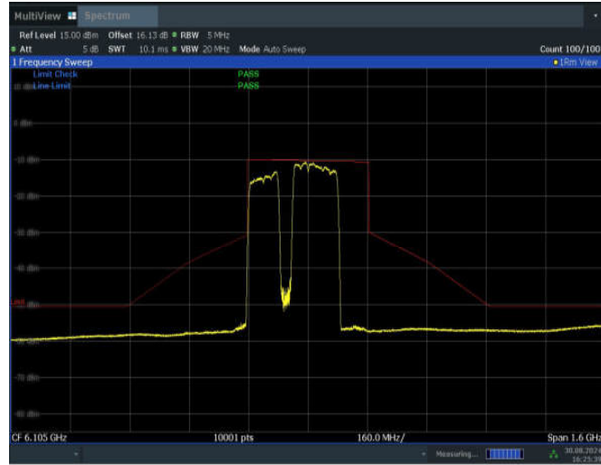
11BE320MIMO_Ant1_6105_2*996+484_Non-OFDMA_3
