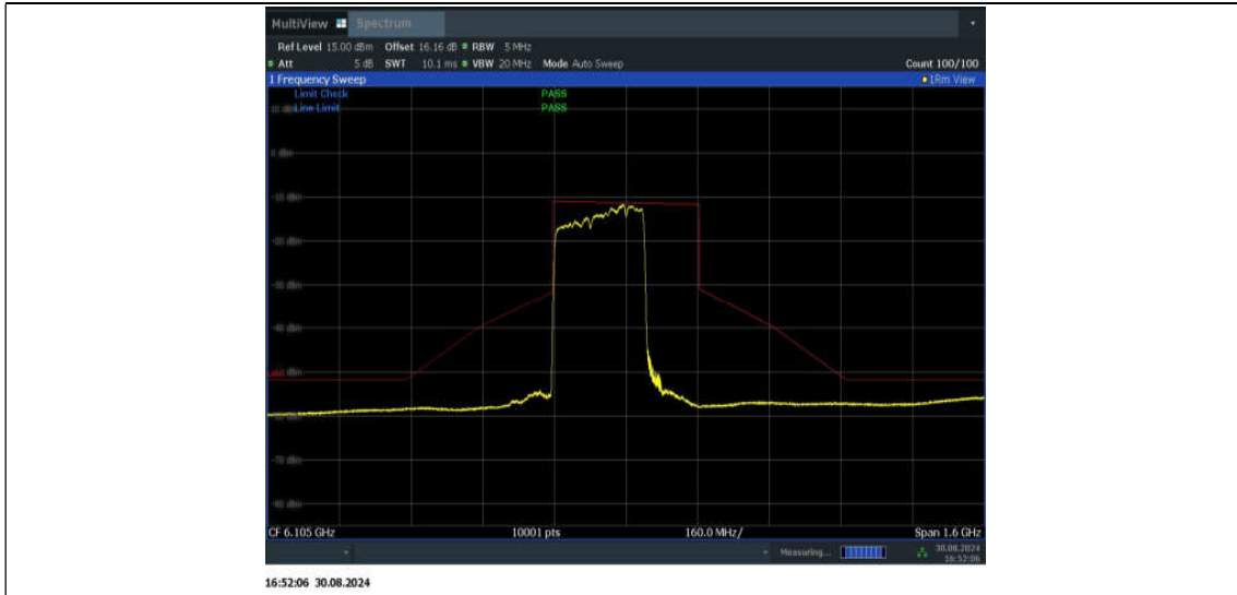
11BE320MIMO_Ant2_6105_2*996+484_Non-OFDMA_7
