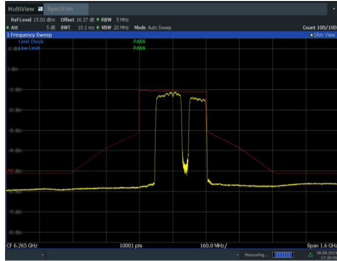
11BE320MIMO_Ant1_6265_2*996+484_Non-OFDMA_10
