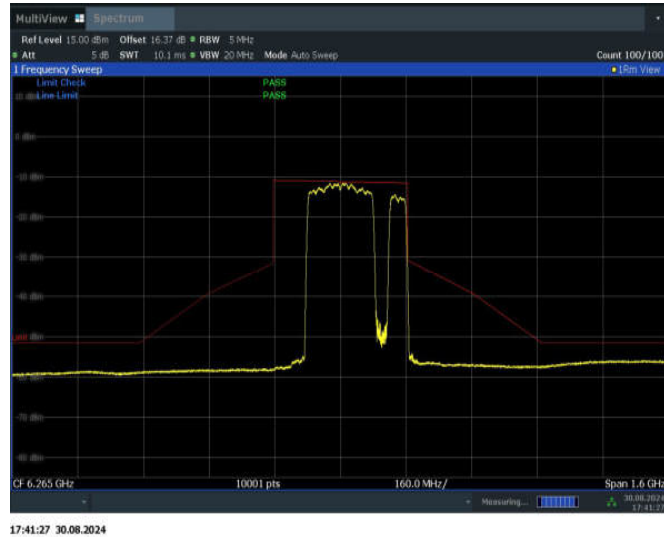
11BE320MIMO_Ant1_6265_2*996+484_Non-OFDMA_12
