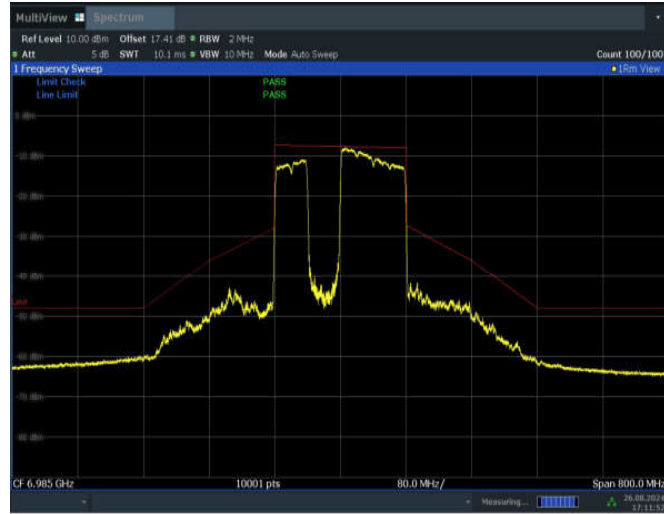
11BE160MIMO_Ant1_6985_996+484_Non-OFDMA_2
