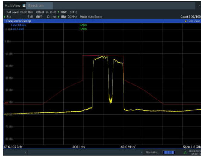
11BE320MIMO_Ant2_6105_2*996+484_Non-OFDMA_10
