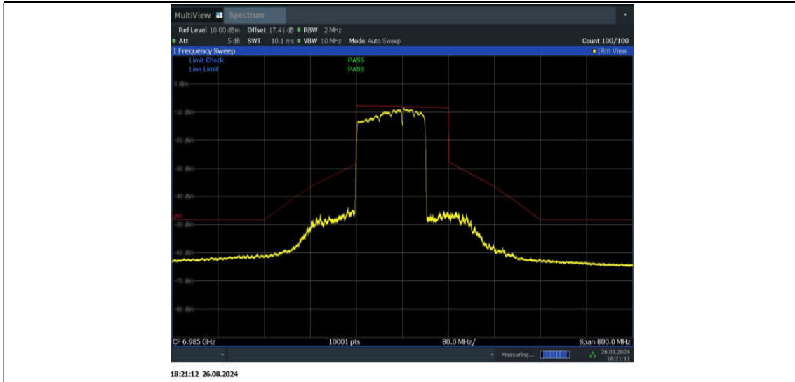
11BE160MIMO_Ant1_6985_996+484+242_Non-OFDMA_1
