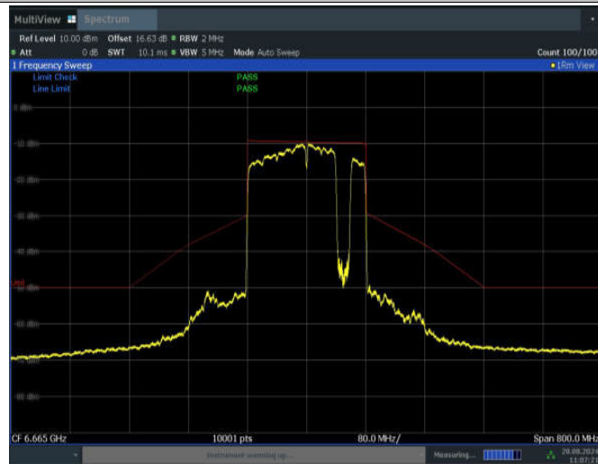
11BE160MIMO_Ant1_6665_996+484+242_Non-OFDMA_7
