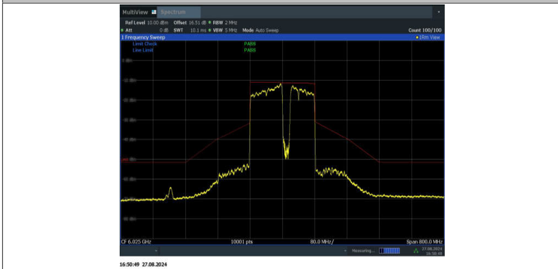
11BE160MIMO_Ant1_6025_996+484+242_Non-OFDMA_6
