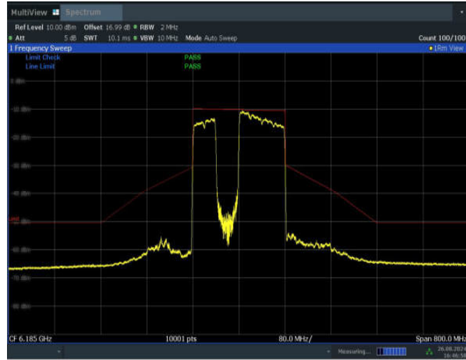
11BE160MIMO_Ant1_6185_996+484_Non-OFDMA_2
