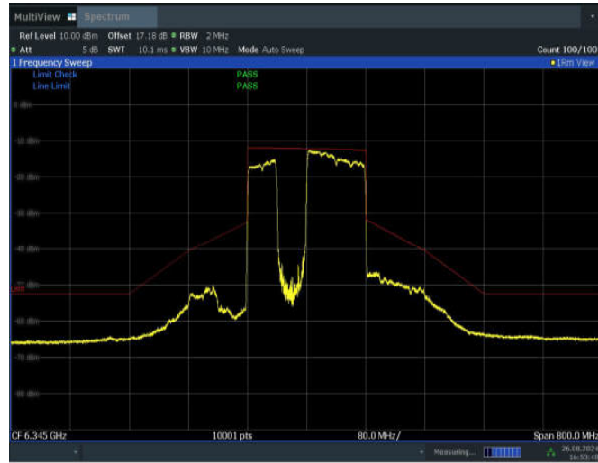
11BE160MIMO_Ant2_6345_996+484_Non-OFDMA_2
