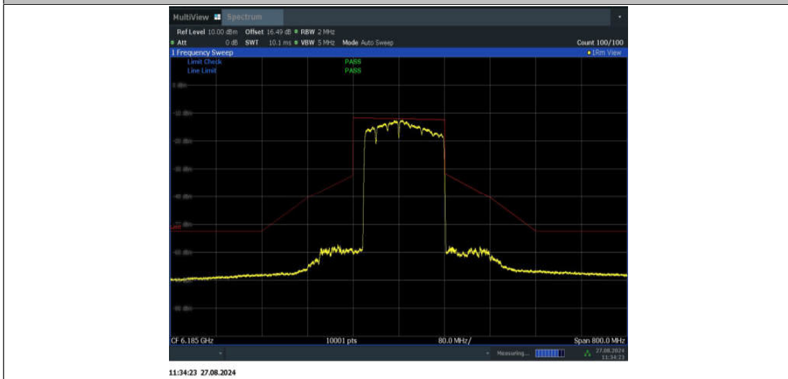
11BE160MIMO_Ant1_6185_996+484+242_Non-OFDMA_2
