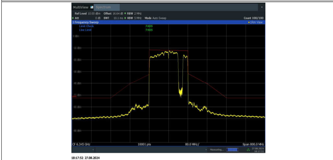
11BE160MIMO_Ant1_6345_996+484+242_Non-OFDMA_8
