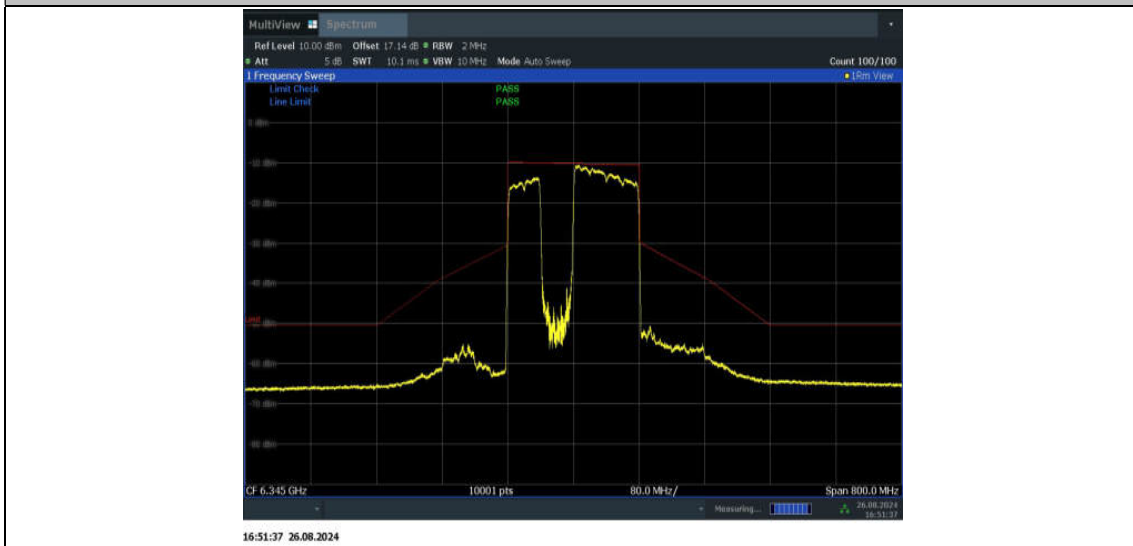
11BE160MIMO_Ant1_6345_996+484_Non-OFDMA_2
