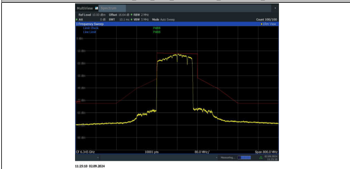
11BE160MIMO_Ant1_6345_996+484+242_Non-OFDMA_8
