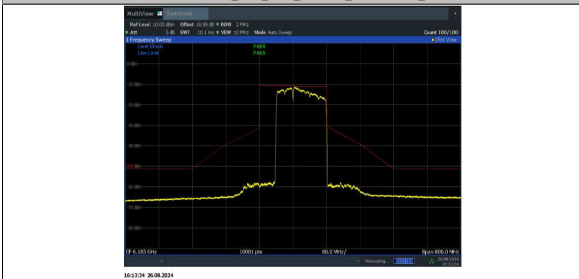
11BE160MIMO_Ant1_6185_996+484_Non-OFDMA_1
