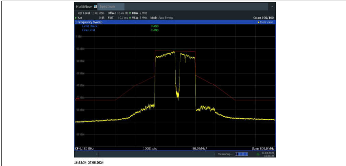
11BE160MIMO_Ant1_6185_996+484+242_Non-OFDMA_6
