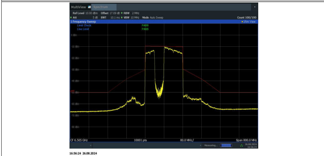
11BE160MIMO_Ant1_6505_996+484_Non-OFDMA_3
