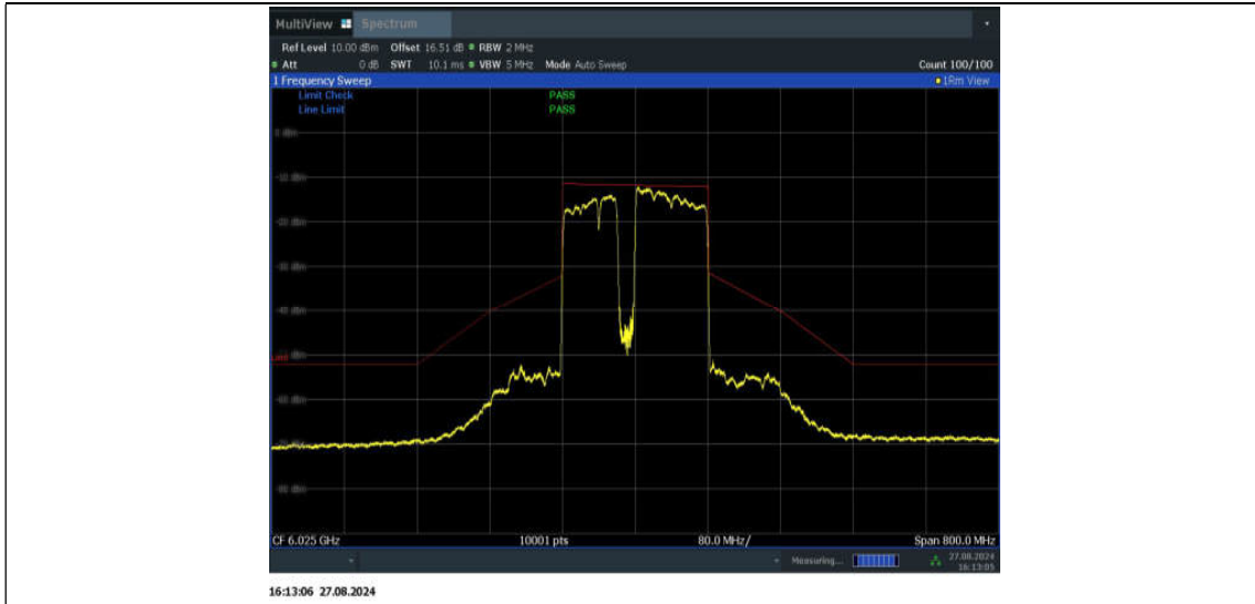
11BE160MIMO_Ant1_6025_996+484+242_Non-OFDMA_5
