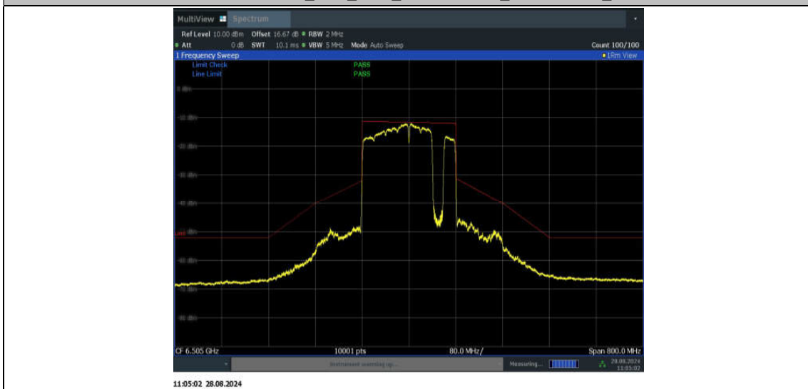
11BE160MIMO_Ant2_6505_996+484+242_Non-OFDMA_7
