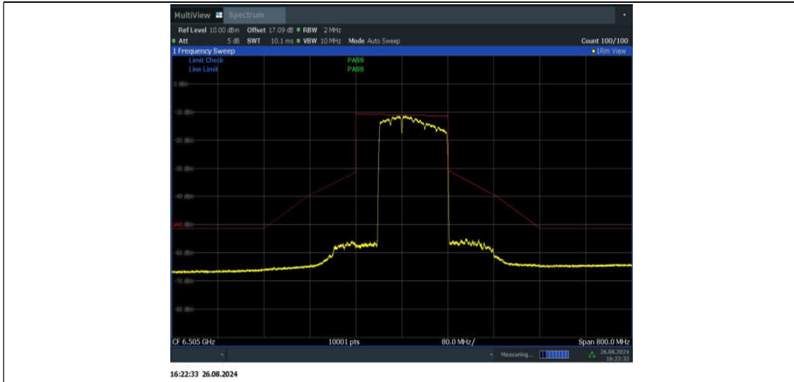
11BE160MIMO_Ant1_6505_996+484_Non-OFDMA_2
