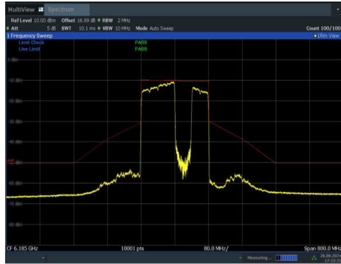
11BE160MIMO_Ant1_6185_996+484_Non-OFDMA_3
