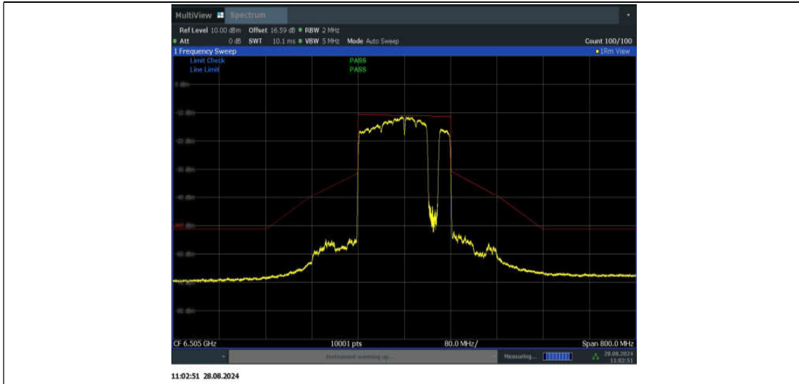
11BE160MIMO_Ant1_6505_996+484+242_Non-OFDMA_8
