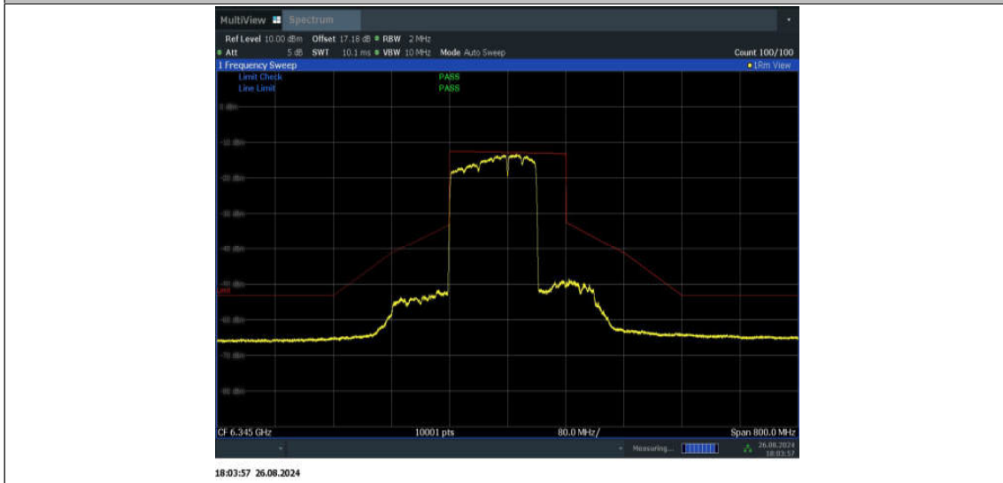
11BE160MIMO_Ant2_6345_996+484+242_Non-OFDMA_1
