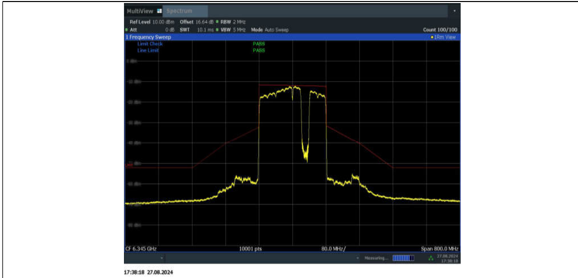
11BE160MIMO_Ant1_6345_996+484+242_Non-OFDMA_7
