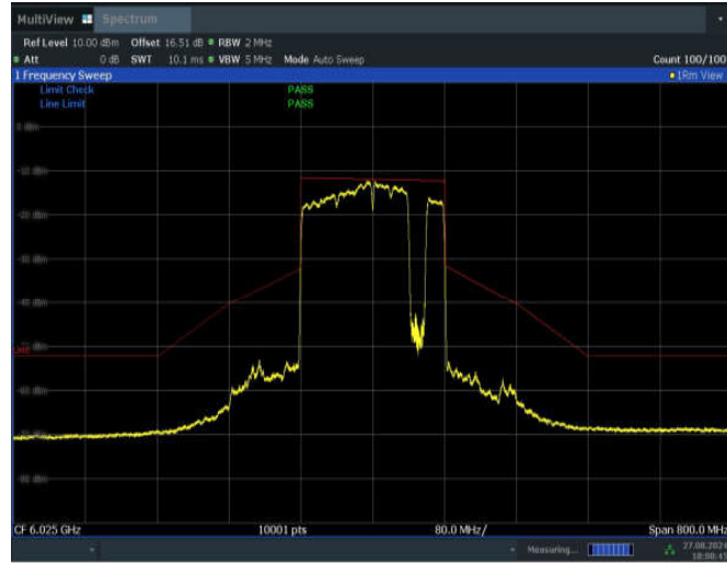
11BE160MIMO_Ant1_6025_996+484+242_Non-OFDMA_7
