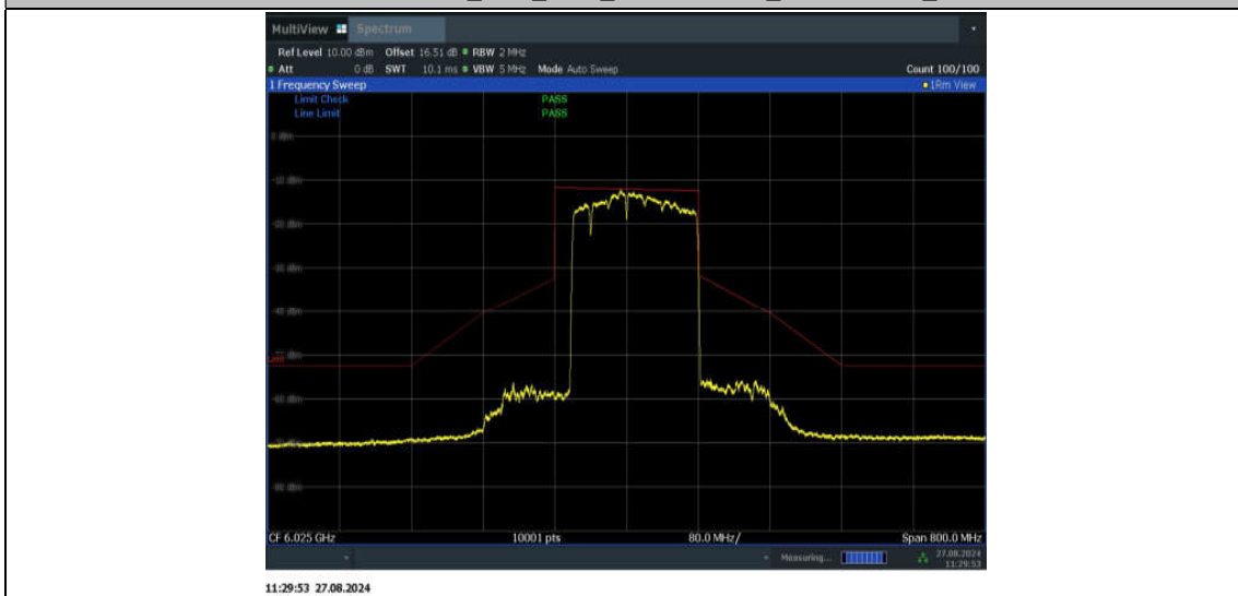
11BE160MIMO_Ant1_6025_996+484+242_Non-OFDMA_1
