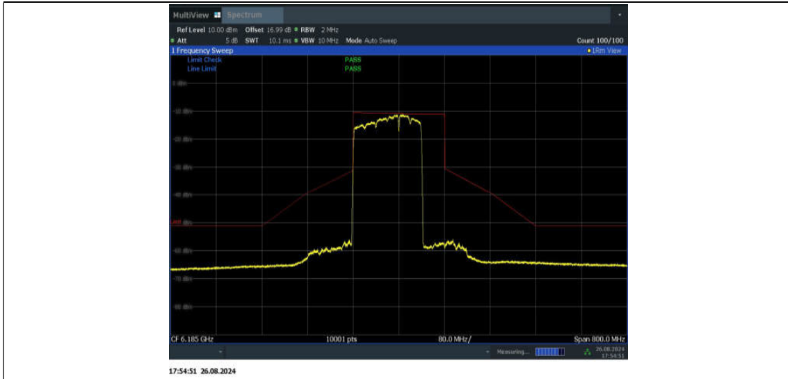
11BE160MIMO_Ant1_6185_996+484+242_Non-OFDMA_1
