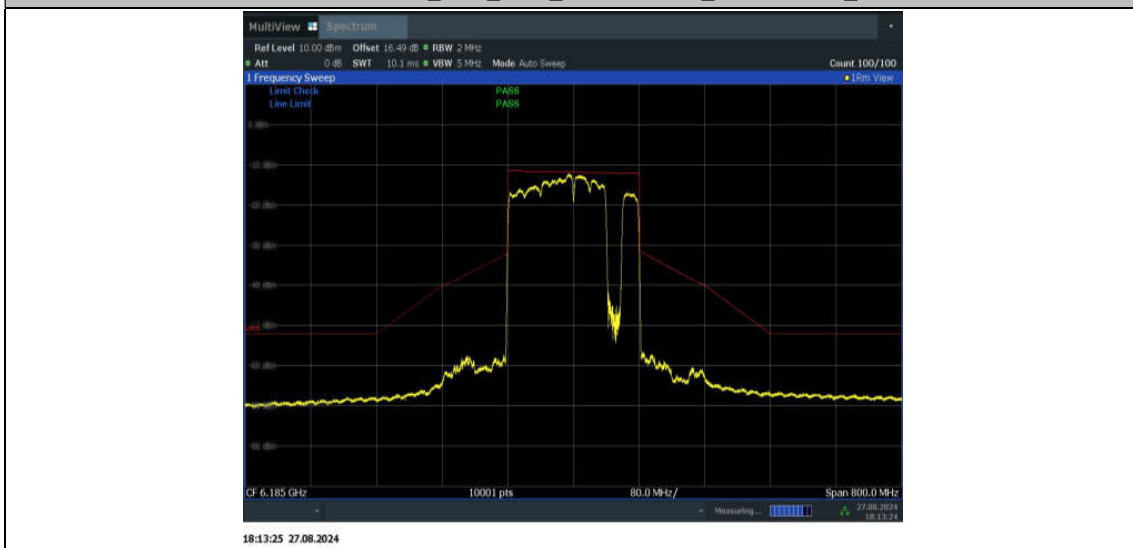
11BE160MIMO_Ant1_6185_996+484+242_Non-OFDMA_7
