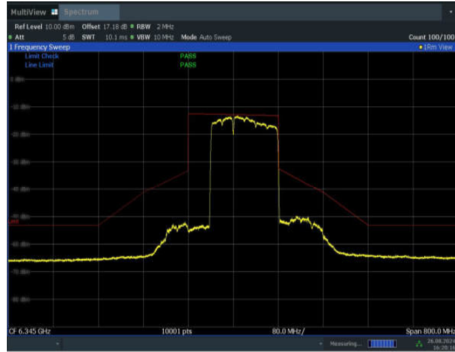
11BE160MIMO_Ant2_6345_996+484_Non-OFDMA_1
