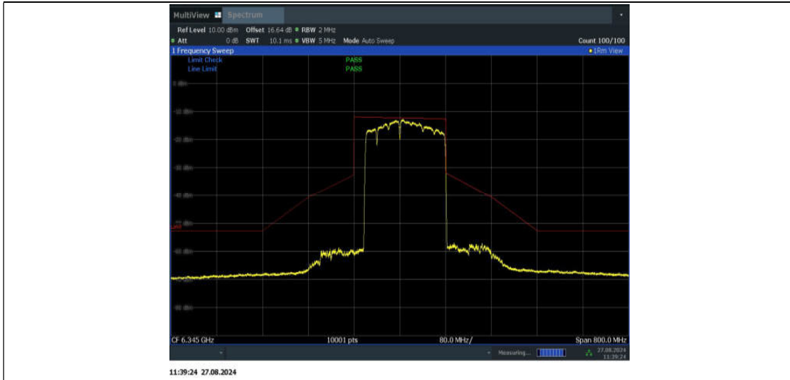
11BE160MIMO_Ant1_6345_996+484+242_Non-OFDMA_2
