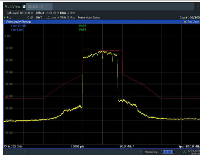
11BE160MIMO_Ant1_6025_996+484+242_Non-OFDMA_8
