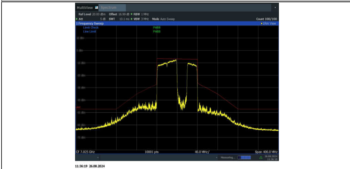
11BE80MIMO_Ant1_7025_484+242_Non-OFDMA_3
