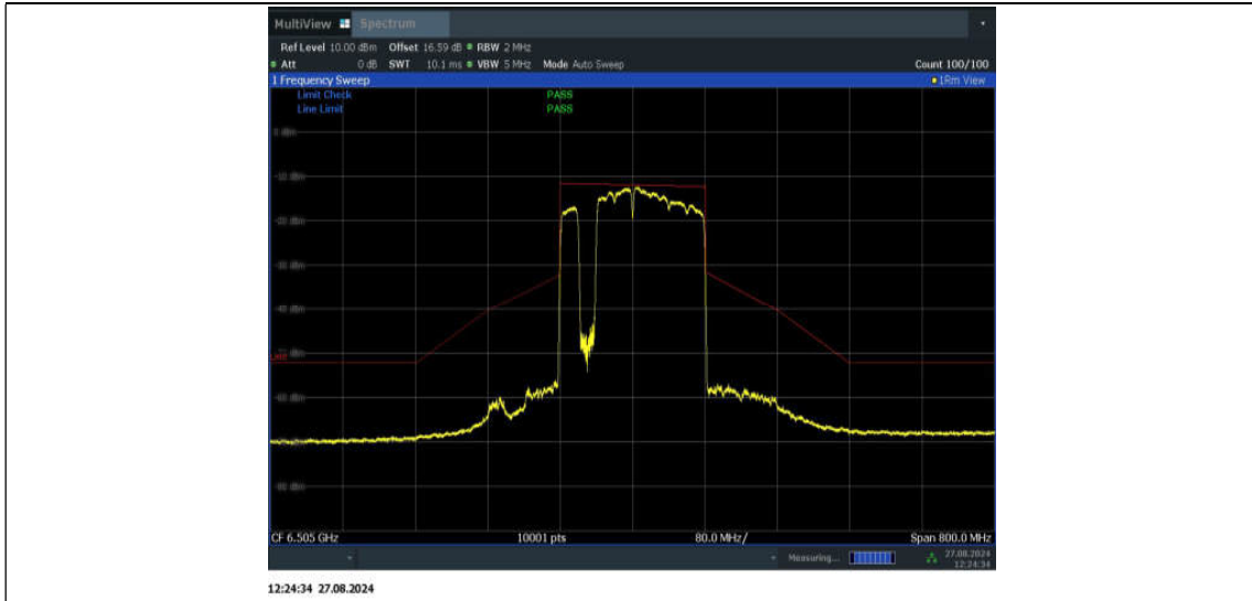
11BE160MIMO_Ant1_6505_996+484+242_Non-OFDMA_3
