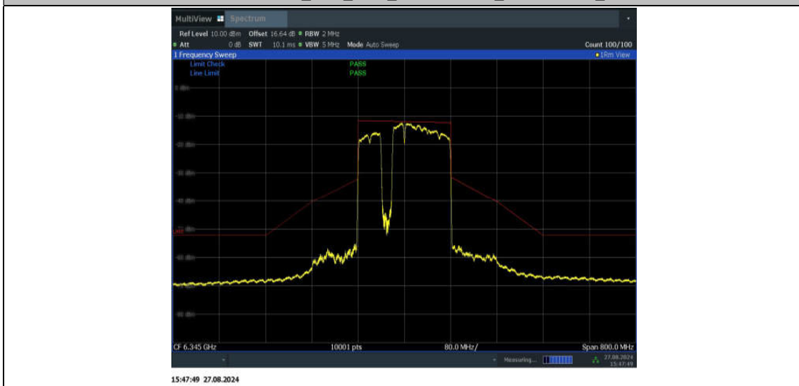
11BE160MIMO_Ant1_6345_996+484+242_Non-OFDMA_3
