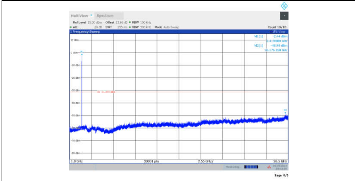
11BE20MIMO_Ant7_2412_106Tone_RU53_0~Reference
