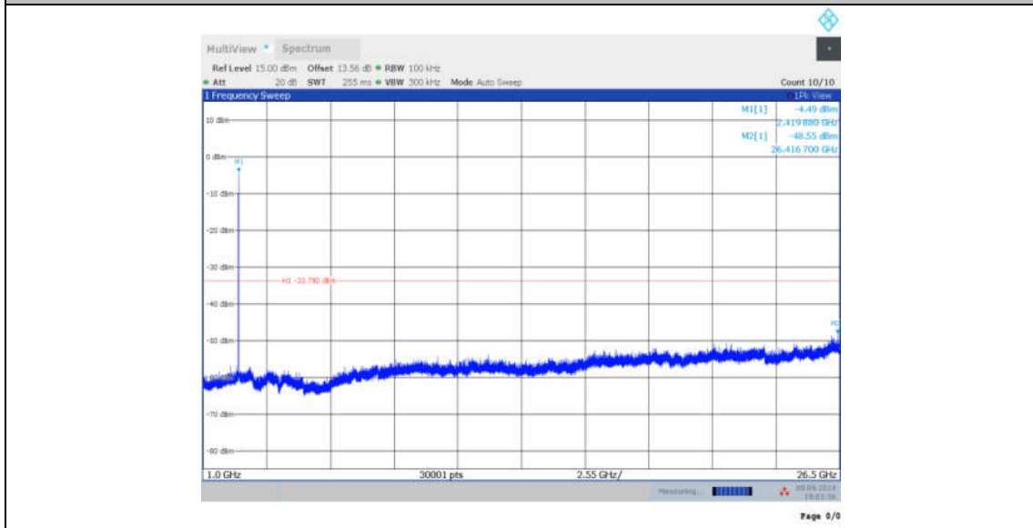
11BE20MIMO_Ant12_2412_106Tone_RU53_0~Reference
