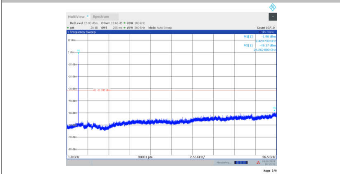
11BE20MIMO_Ant7_2412_52Tone_RU37_0~Reference
