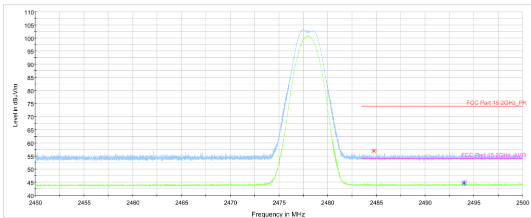
Fig.19. Frequency Band Edges: GFSK, 2478 MHz, Hopping Off, 2.45 GHz - 2.50GHz
