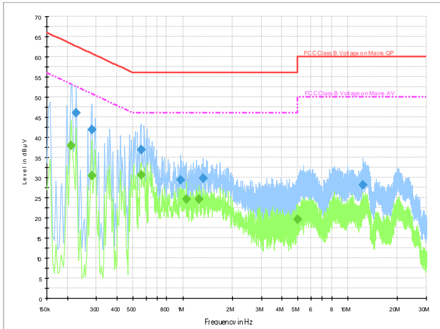
Fig.B.10.1 AC Powerline Conducted Emission-blutetooth
