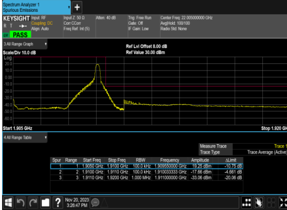
N2(10M)_DFT-s-OFDM_QPSK_Edge_1RB_Right_High_CH
