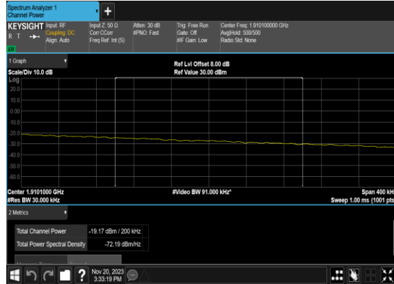
N2(20M)_DFT-s-OFDM_QPSK_Edge_1RB_Right_High_CH_CHP_P ASS
