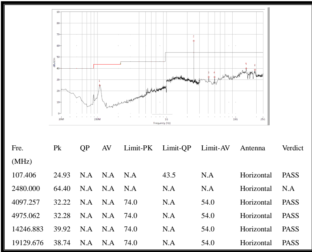
(30MHz to 25GHz, Antenna Horizontal @ GFSK, channel 78)
