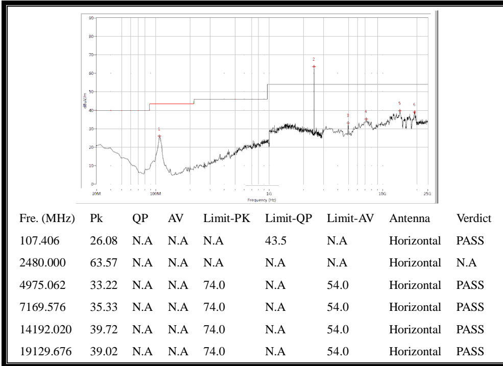
(30MHz to 25GHz, Antenna Horizontal @ \pi/4 -DQPSK, channel 78)
