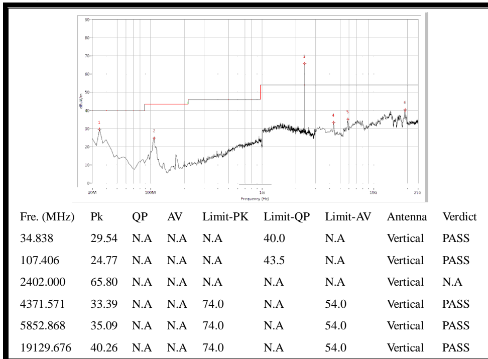
(30MHz to 25GHz, Antenna Vertical @ □/4-DQPSK, channel 0)
