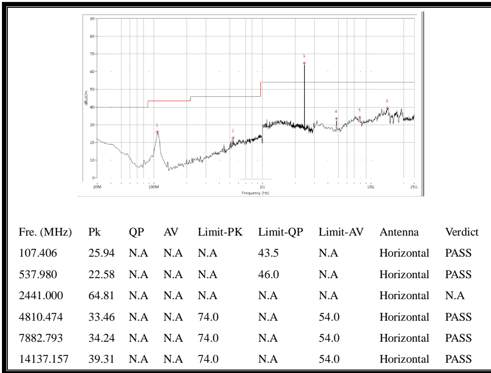
(30MHz to 25GHz, Antenna Horizontal @ \pi/4 -DQPSK, channel 39)
