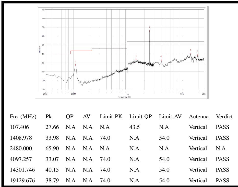
(30MHz to 25GHz, Antenna Vertical @ GFSK, channel 78)
