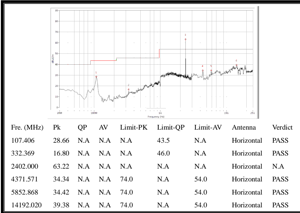
(30MHz to 25GHz, Antenna Horizontal @ □/4-DQPSK, channel 0)
