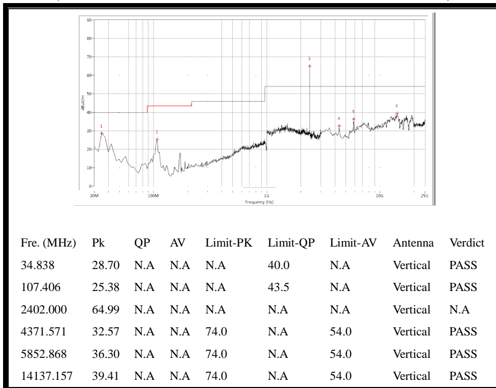
(30MHz to 25GHz, Antenna Vertical @ GFSK, channel 0)
