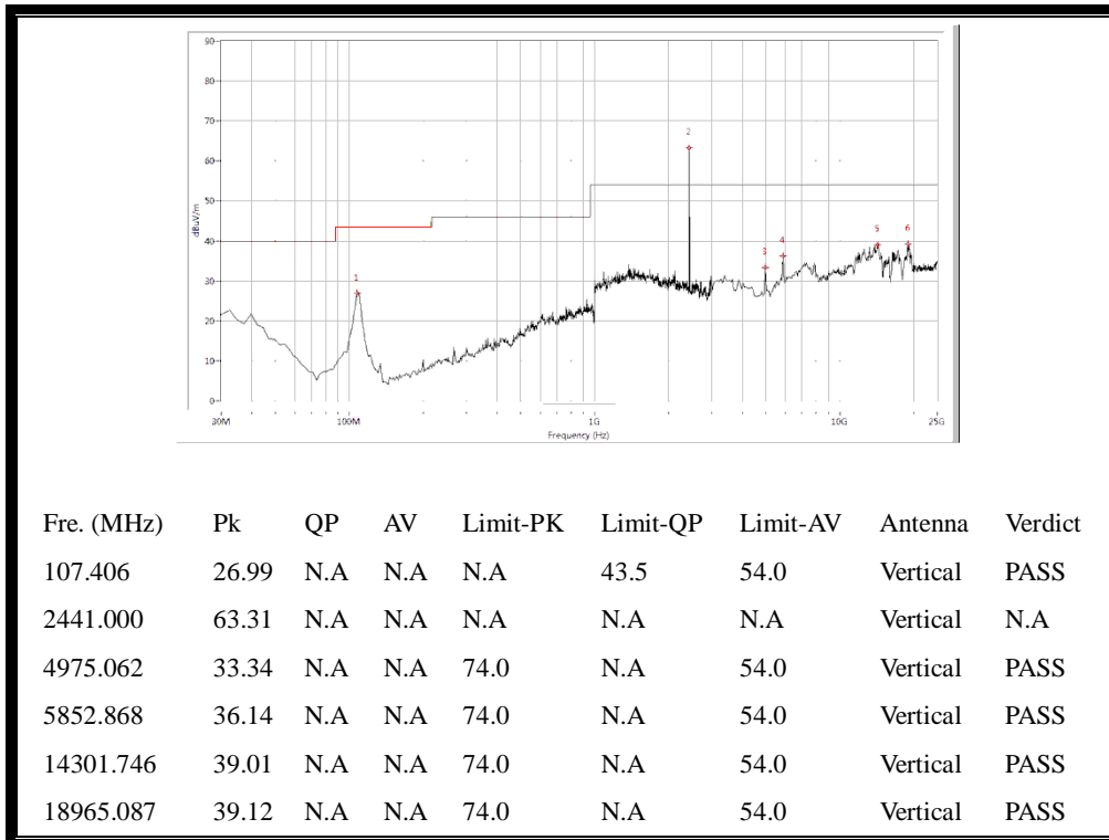
(30MHz to 25GHz, Antenna Vertical @ GFSK, channel 39)
