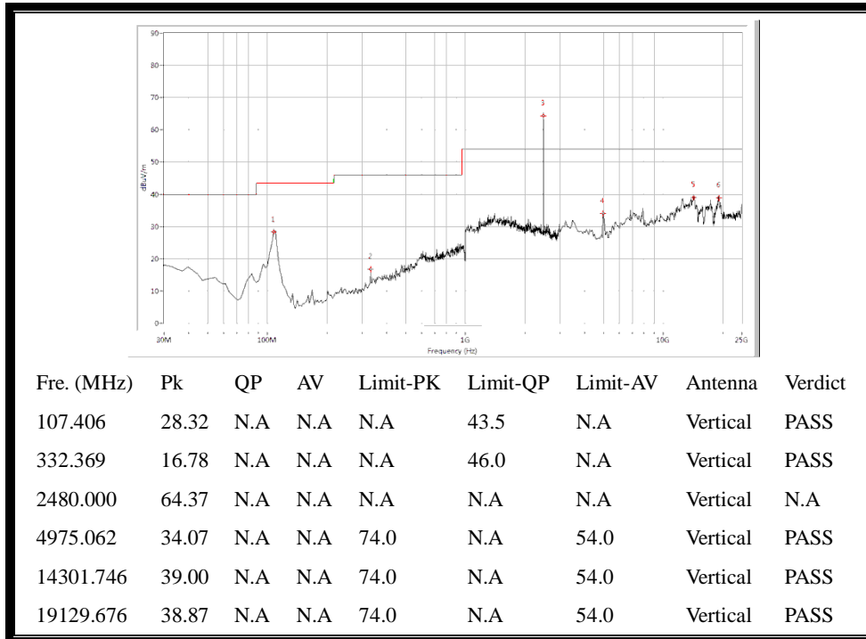
(30MHz to 25GHz, Antenna Vertical @ \pi/4 -DQPSK, channel 78)
