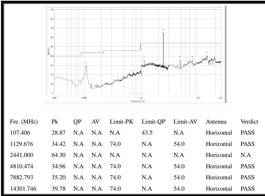
(30MHz to 25GHz, Antenna Horizontal @ GFSK, channel 39)
