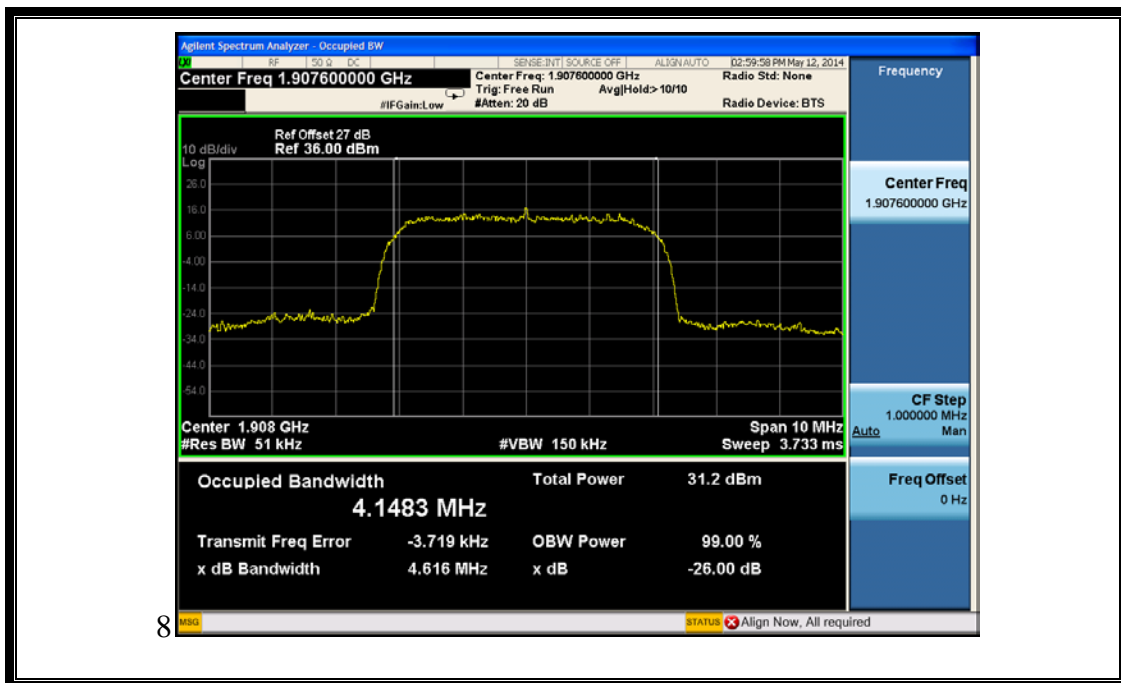
(Plot X: HSPA1900 MHz Channel = 9538)
