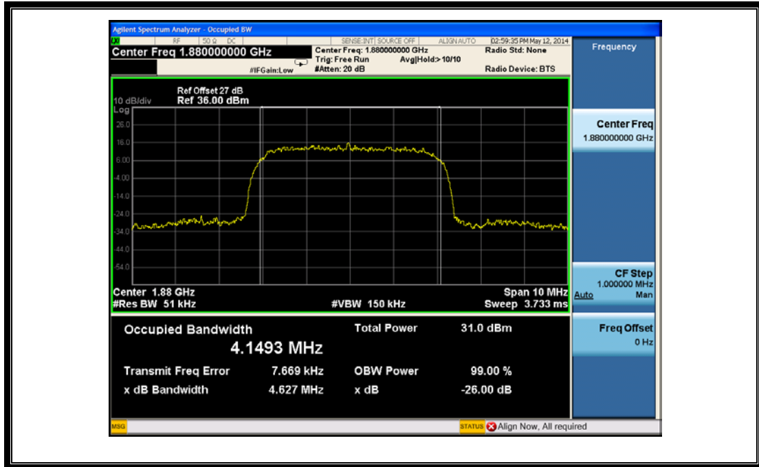
(Plot W: HSPA1900 MHz Channel = 9400)
