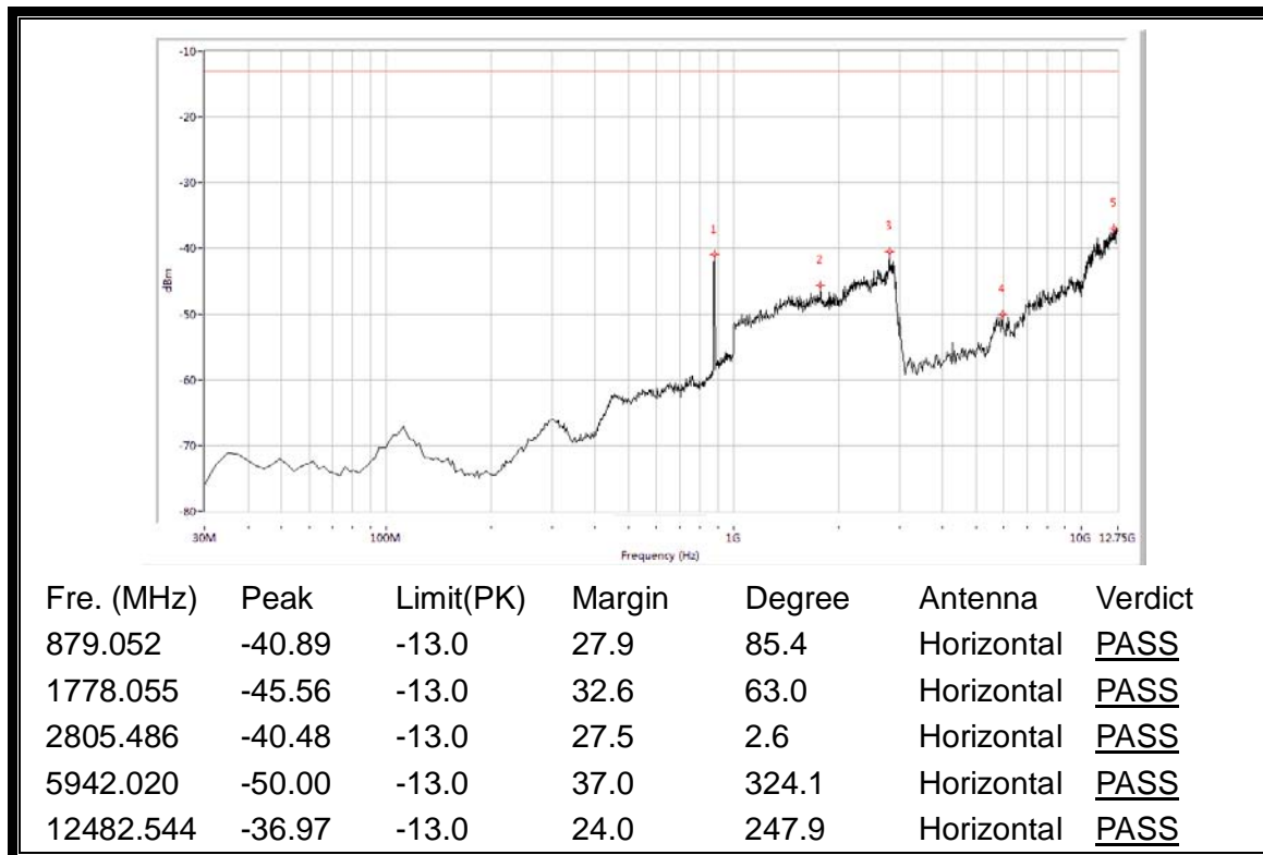
(Plot E.3: WCDMA 850MHz Channel = 4175, Test Antenna Horizontal)
