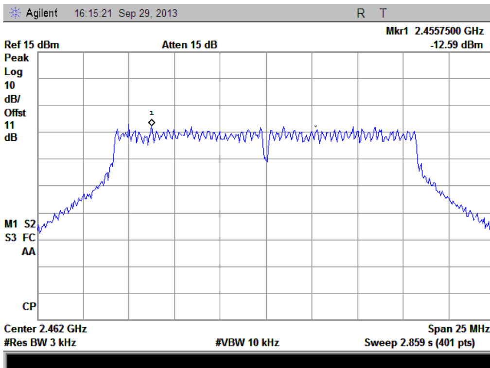
(Plot I: Channel = 11 @ 802.11g)
