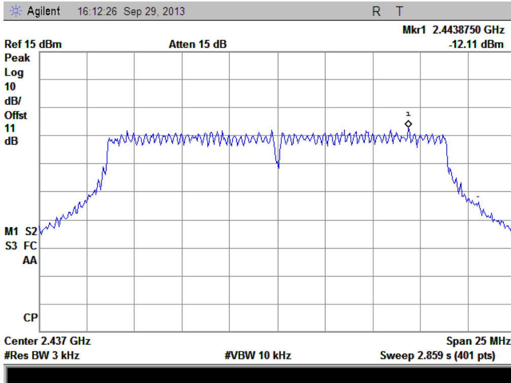
(Plot K: Channel = 6 @ 802.11n-20MHz)
