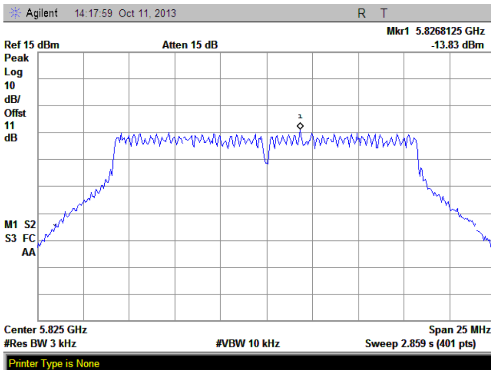
(Plot C: Channel = 165 @ 802.11a)
