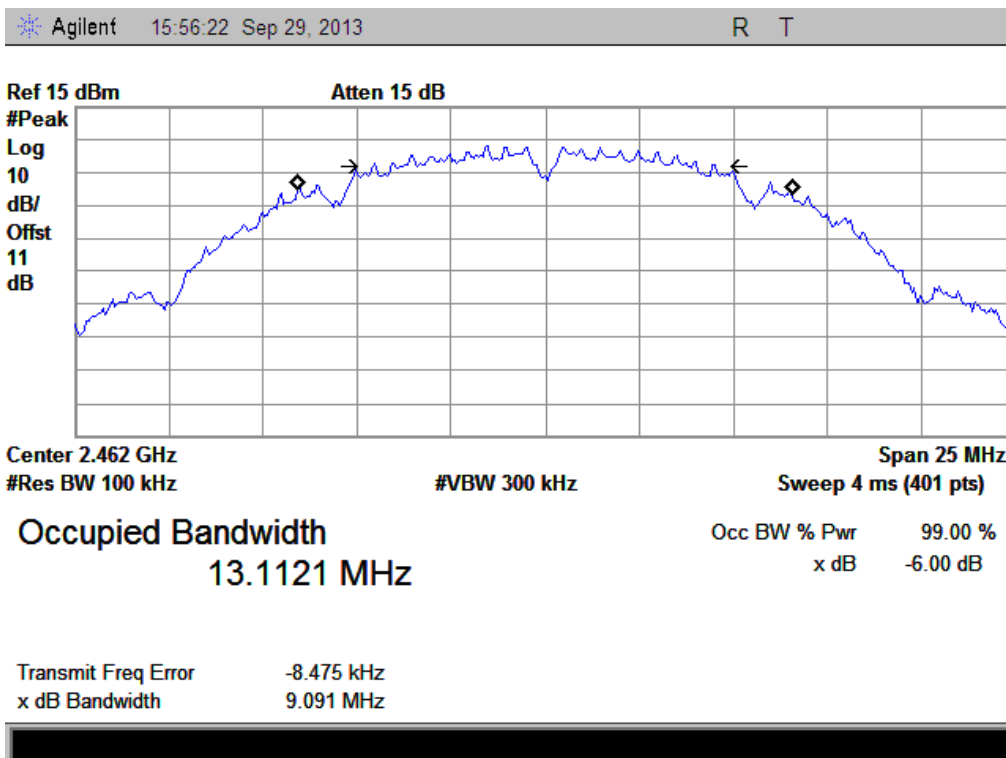
(Plot F: Channel 11: 2462MHz @ 802.11b)
