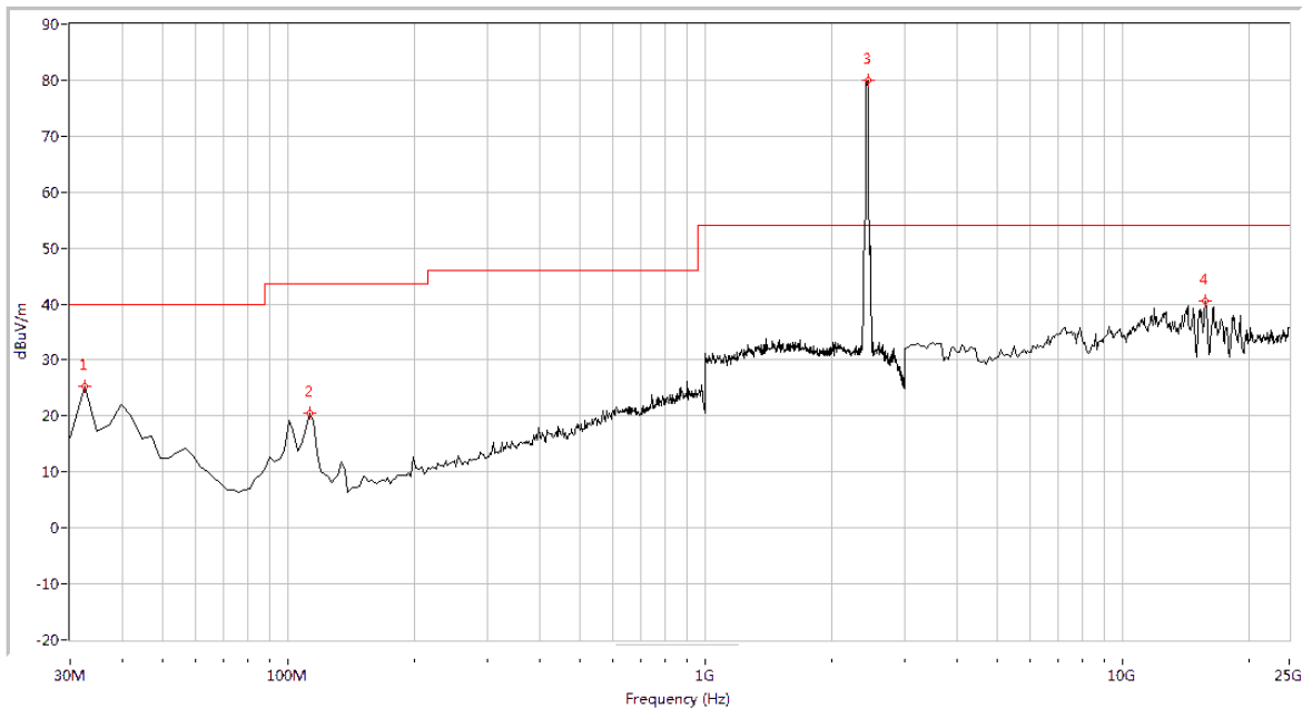
(Plot Q.2: Antenna Horizontal, 30MHz to 25GHz)
