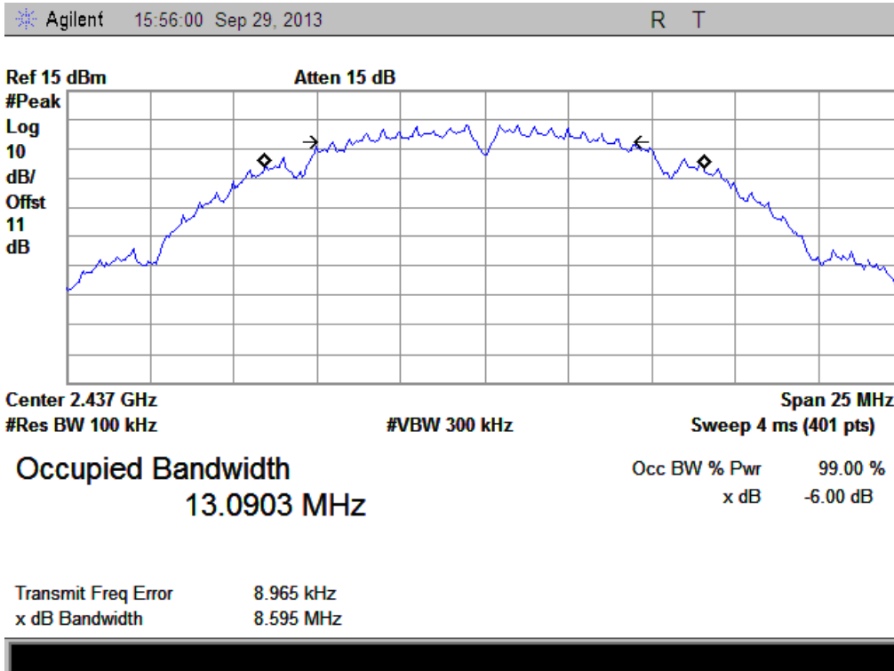
(Plot E: Channel 6: 2437 MHz @ 802.11b)
