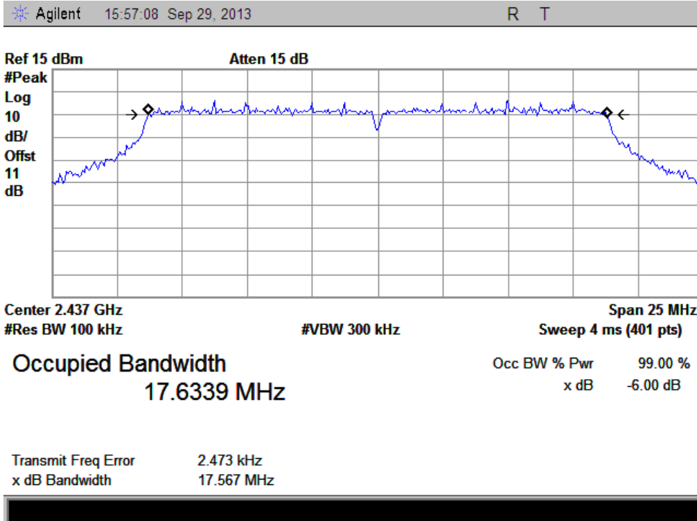
(Plot K: Channel 6: 2437MHz @ 802.11n-20)
