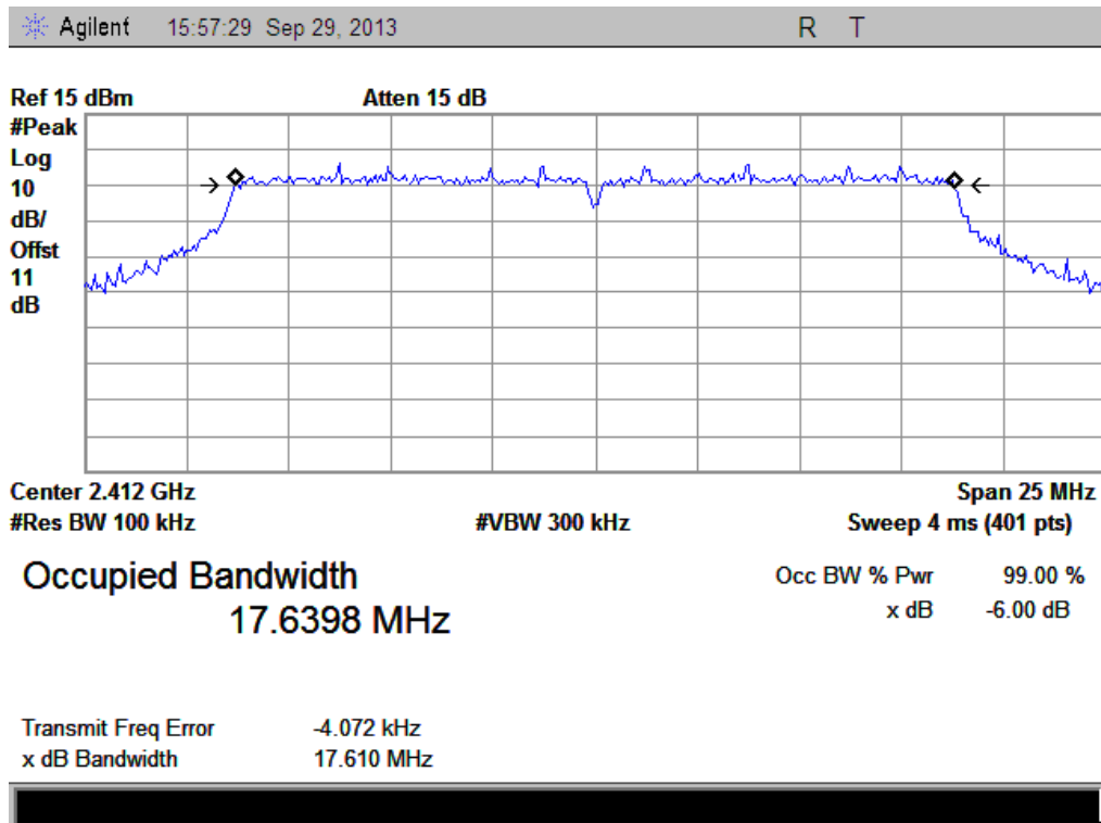
(Plot J: Channel 1: 2412MHz @ 802.11n-20)
