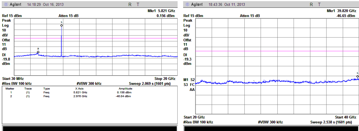
(Plot O.1: Channel = 165, 30MHz to 40GHz)
