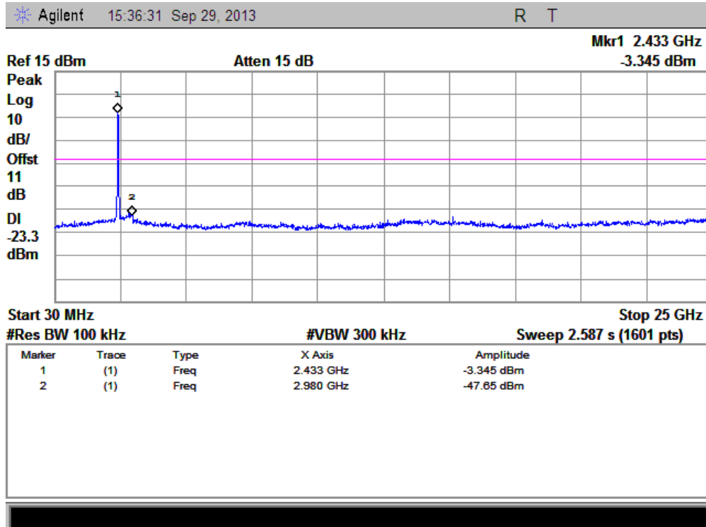
(Plot Q.1: Channel = 6, 30MHz to 25GHz)
