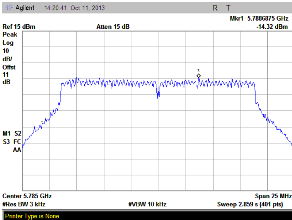
(Plot N: Channel = 157 @ 802.11n-20MHz)
