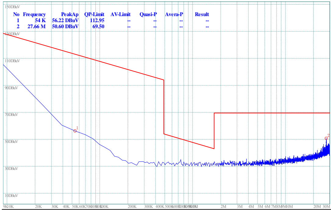
(Plot G.1: 9kHz to 30MHz)
