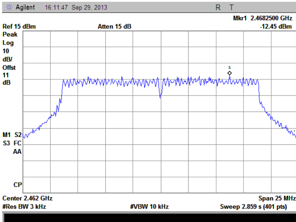
(Plot L: Channel = 11 @ 802.11n-20MHz)
