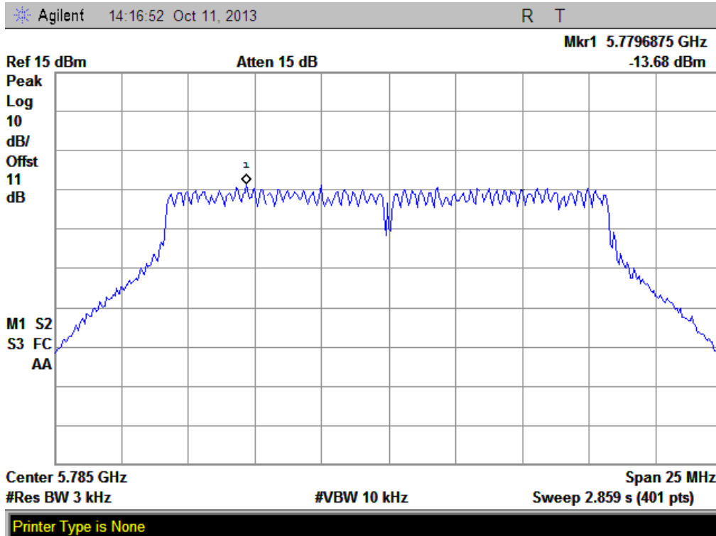
(Plot B: Channel = 157 @ 802.11a)
