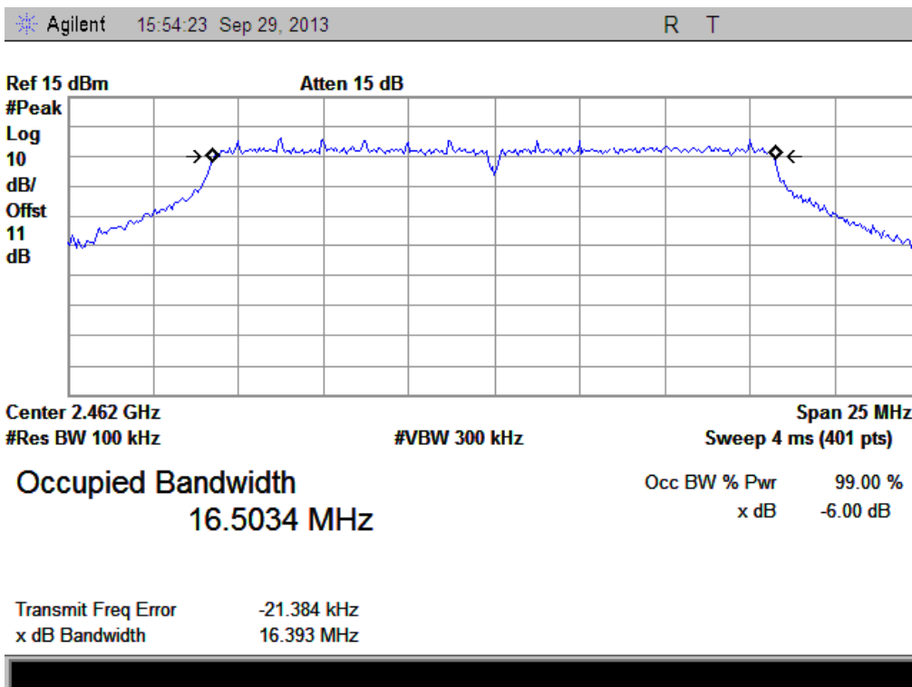
(Plot I: Channel 11: 2462MHz @ 802.11g)
