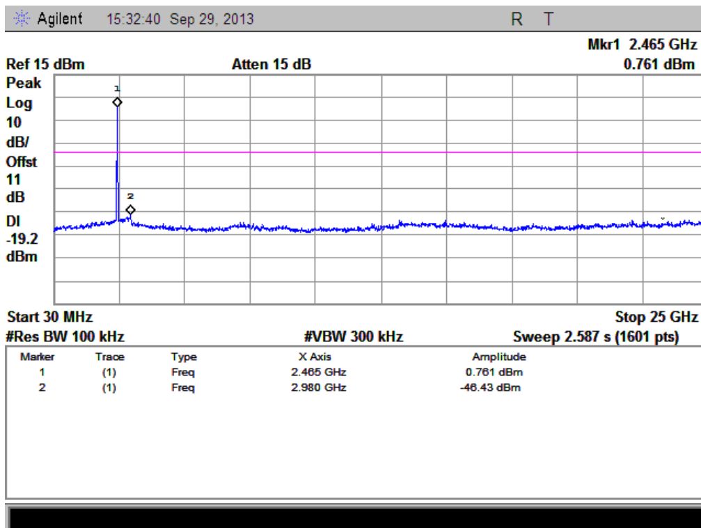
(Plot L.1: Channel = 11, 30MHz to 25GHz)\
