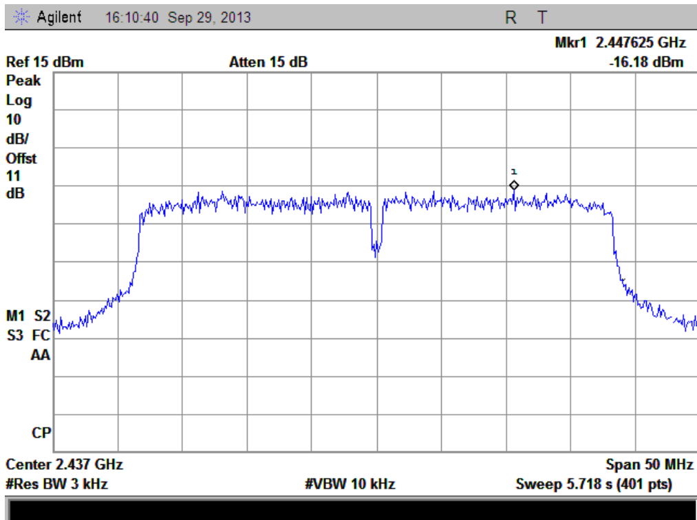
(Plot Q: Channel = 6 @ 802.11n-40MHz)
