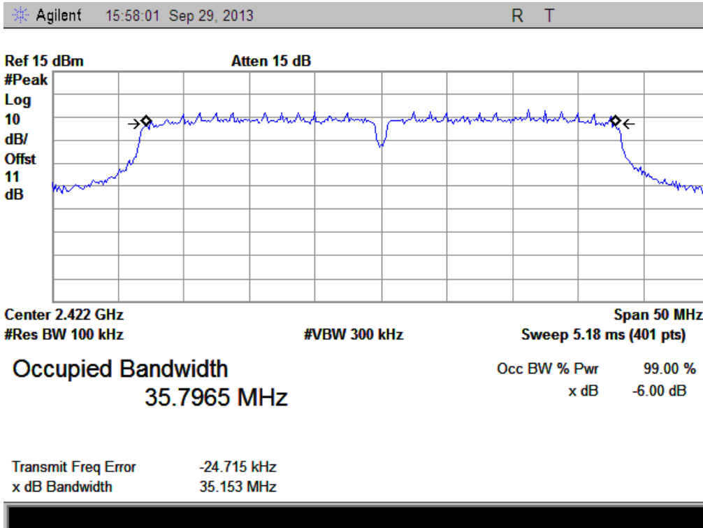
(Plot P: Channel 1: 2422MHz @ 802.11n-40)
