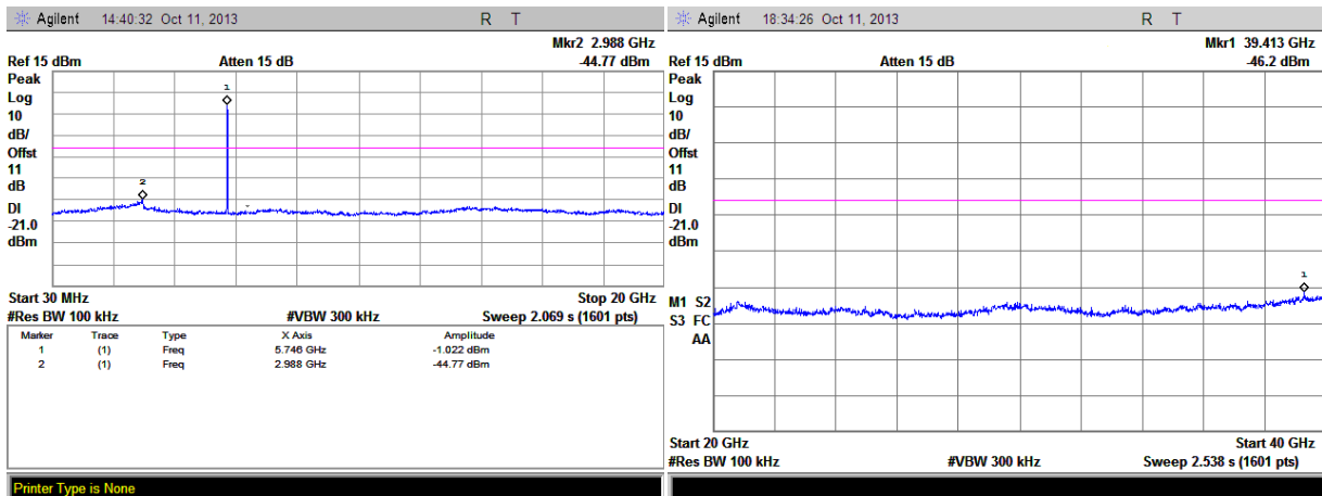
(Plot A.1: Channel = 149, 30MHz to 40GHz)
