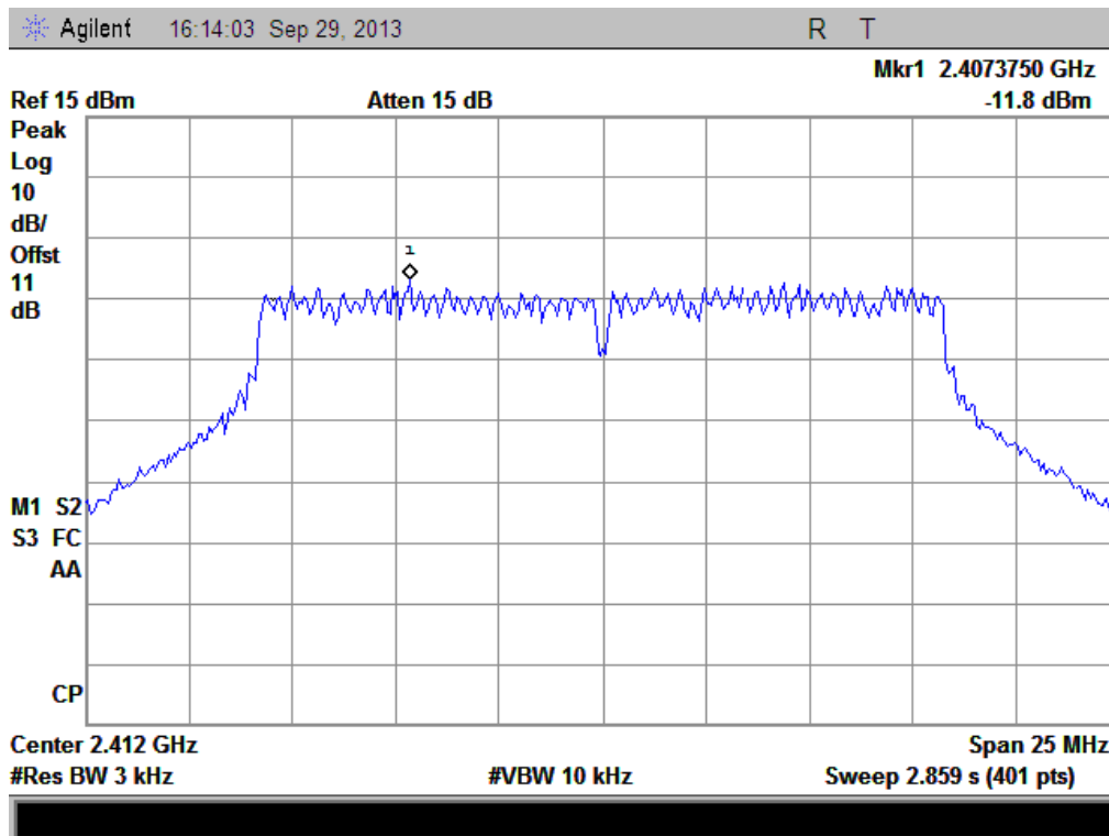
(Plot G: Channel = 1 @ 802.11g)
