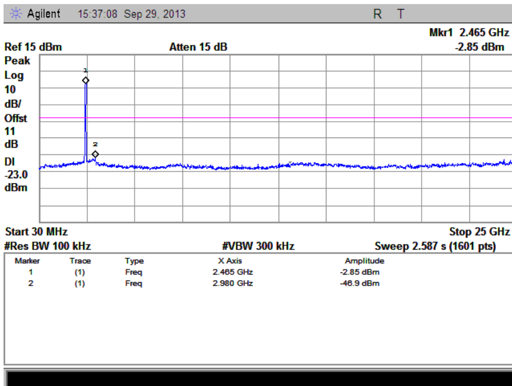
(Plot R.1: Channel = 9, 30MHz to 25GHz)
