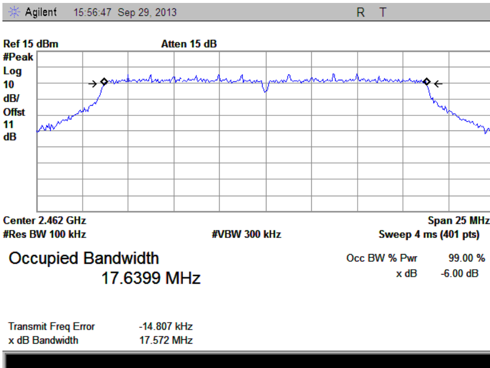
(Plot L: Channel 11: 2462MHz @ 802.11n-20)
