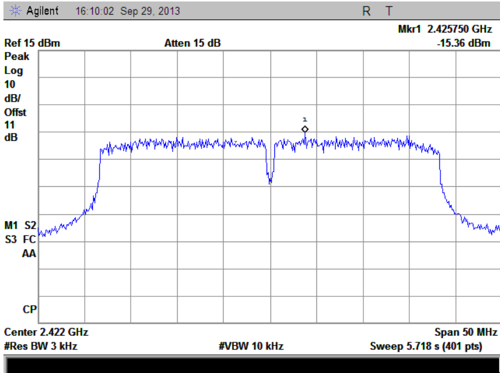
(Plot P: Channel = 3 @ 802.11n-40MHz)
