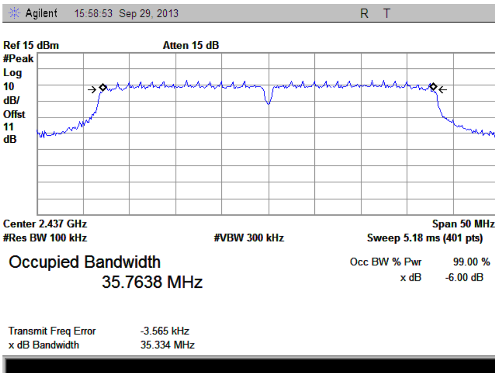
(Plot Q: Channel 6: 2437MHz @ 802.11n-40)
