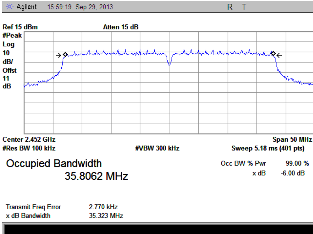
(Plot R: Channel 11: 2452MHz @ 802.11n-40)
