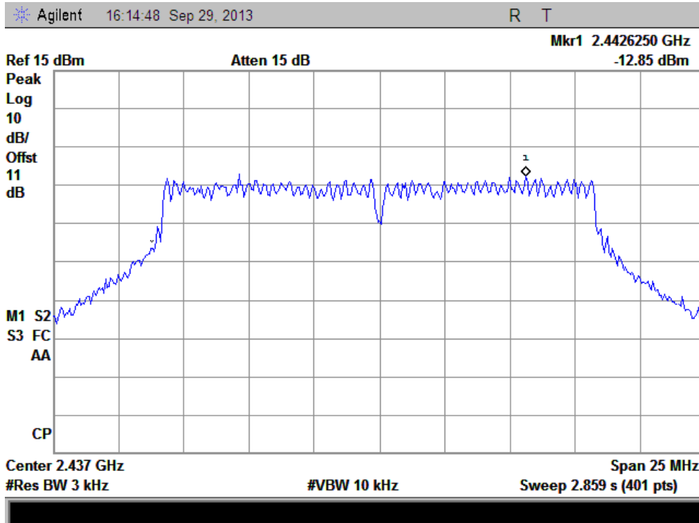
(Plot H: Channel = 6 @ 802.11g)
