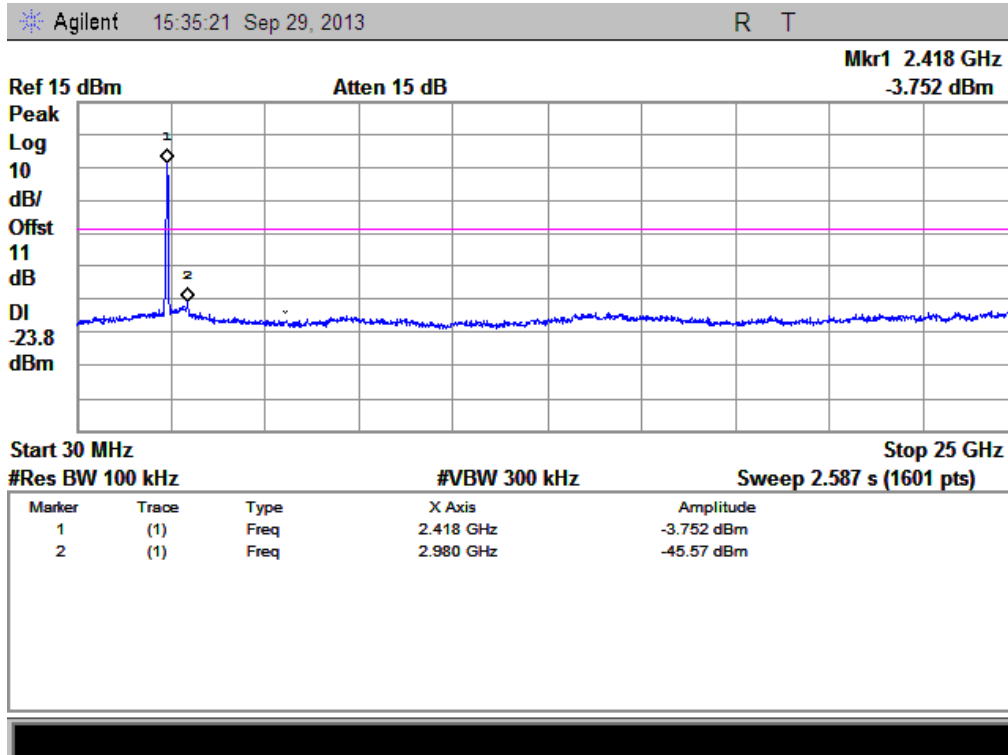
(Plot P.1: Channel = 3, 30MHz to 25GHz)
