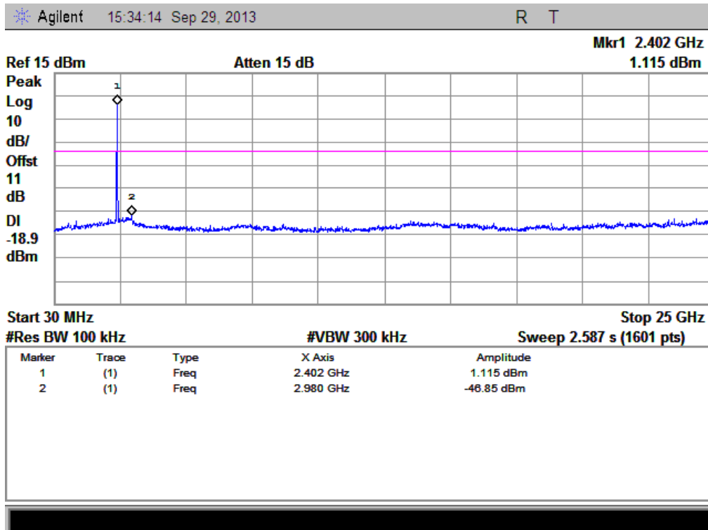
(Plot J.1: Channel = 1, 30MHz to 25GHz)
