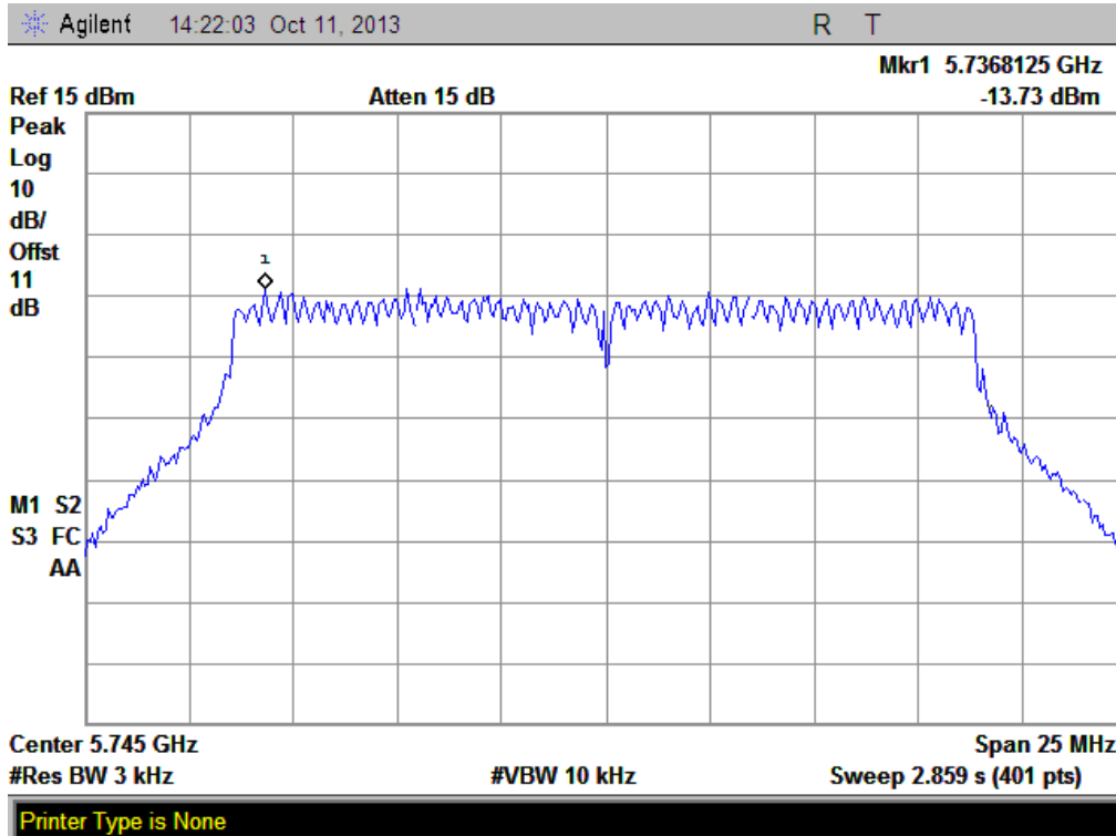
(Plot M: Channel = 149 @802.11n-20MHz)
