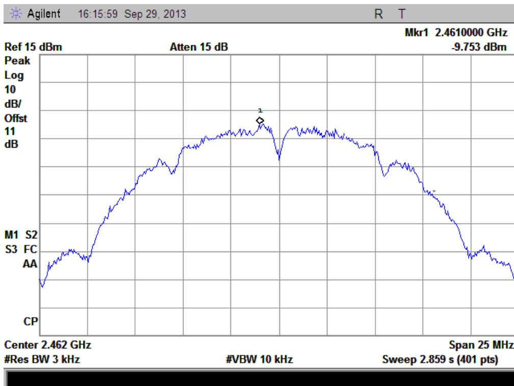
(Plot F: Channel = 11 @ 802.11b)
