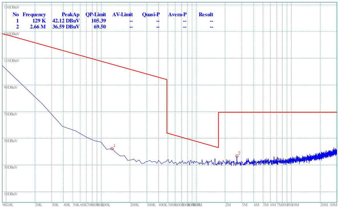
(Plot O.1: 9kHz to 30MHz)
