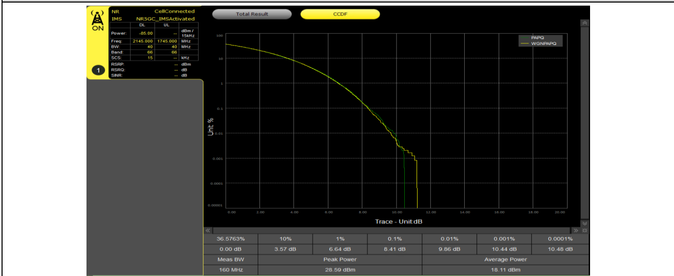
1-N66-PC3-15-40-M-2-CP-256QAM-Outer_Full-216@0-Ant3-8.41-100%-0.00-8.41-PASS-≤13
