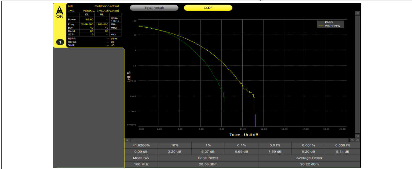
1-N66-PC3-15-40-H-1-DFT-256QAM-Outer_Full-216@0-Ant3-6.65-100%-0.00-6.65-PASS-≤13
