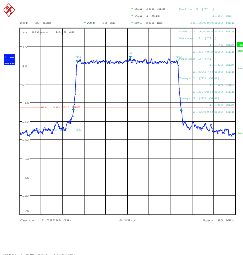
1-N41-PC2-30-30-M-9-CP-256QAM-Outer_Full-78@0-Ant3-27.9-30.000-≤30-PASS
