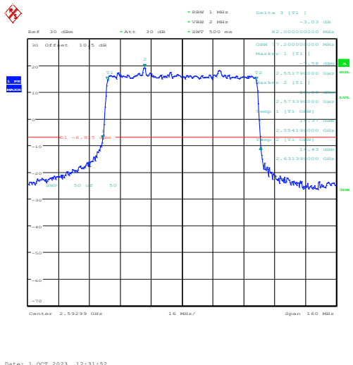
1-N41-PC2-30-80-M-1-DFT-PI2BPSK-Outer_Full-216@0-Ant3-77.2-82.000-≤80-PASS
