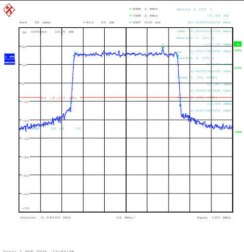
1-N41-PC2-30-80-M-2-DFT-QPSK-Outer_Full-216@0-Ant3-77.6-82.000-≤80-PASS
