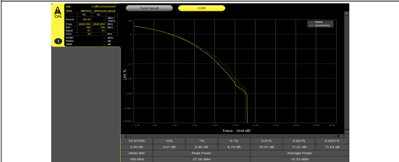
1-N41-PC2-30-100-H-2-CP-256QAM-Outer_Full-273@0-Ant3-8.79-100%-0.00-8.79-PASS-≤13
