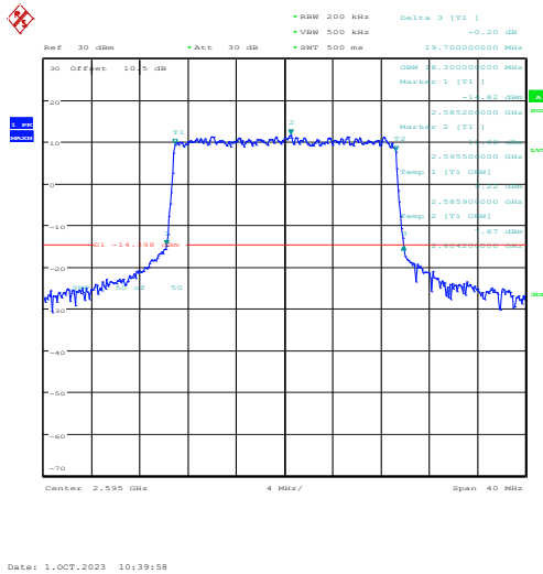
1-N38-PC3-30-20-M-7-CP-16QAM-Outer_Full-51@0-Ant3-18.3-19.700-≤20-PASS
