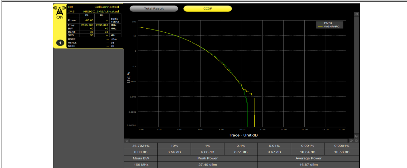
1-N38-PC3-30-40-M-2-CP-256QAM-Outer_Full-106@0-Ant3-8.51-100%-0.00-8.51-PASS-≤13
