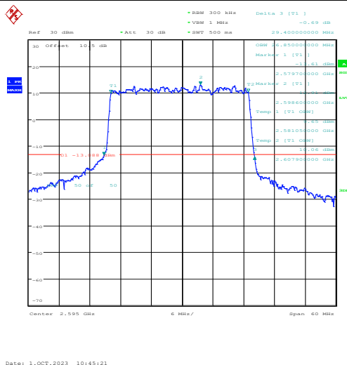
1-N38-PC3-30-30-M-5-DFT-256QAM-Outer_Full-75@0-Ant3-26.85-29.400-≤30-PASS
