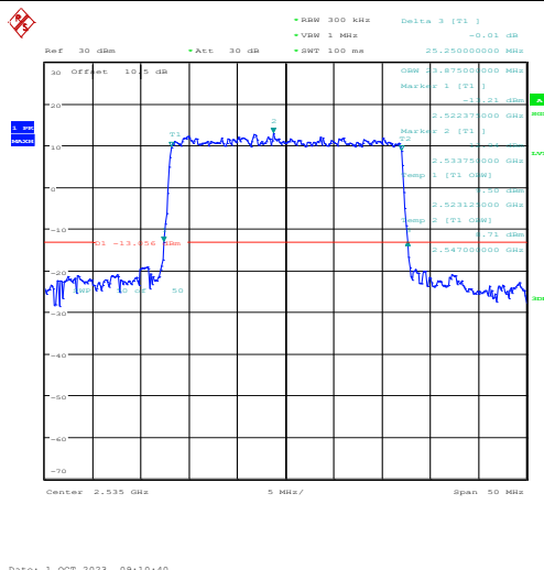
1-N7-PC3-15-25-M-6-CP-QPSK-Outer_Full-133@0-Ant3-23.875-25.250-≤25-PASS
