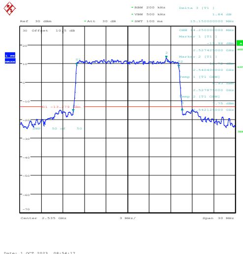
1-N7-PC3-15-15-M-9-CP-256QAM-Outer_Full-79@0-Ant3-14.25-15.150-<math>\leq 15</math>-PASS
