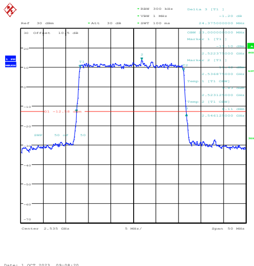
1-N7-PC3-15-25-M-5-DFT-256QAM-Outer_Full-128@0-Ant3-23-24.375-≤25-PASS
