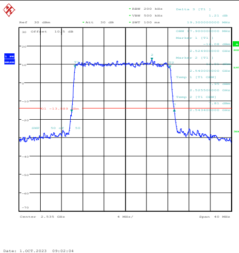
1-N7-PC3-15-20-M-5-DFT-256QAM-Outer_Full-100@0-Ant3-17.9-19.300-≤20-PASS
