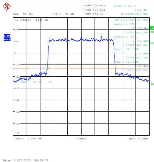
1-N7-PC3-15-15-M-8-CP-64QAM-Outer_Full-79@0-Ant3-14.175-15.150-≤15-PASS
