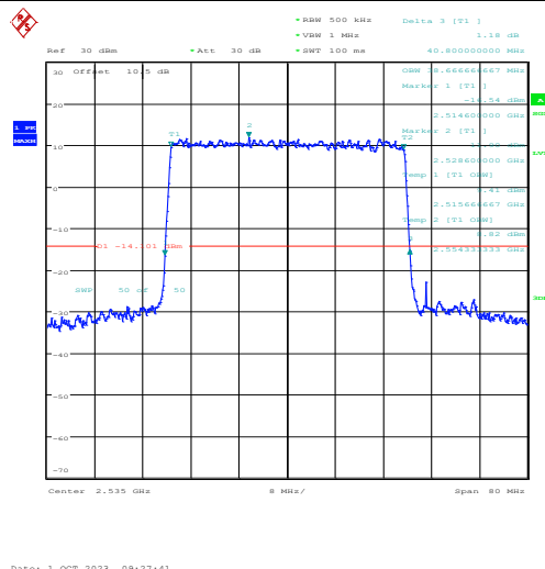
1-N7-PC3-15-40-M-4-DFT-64QAM-Outer_Full-216@0-Ant3-38.667-40.800-≤40-PASS
