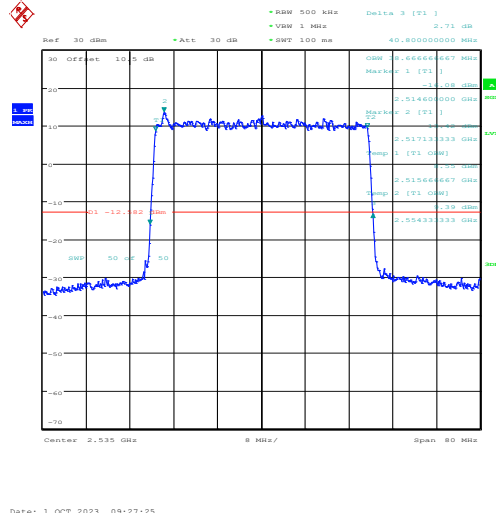
1-N7-PC3-15-40-M-3-DFT-16QAM-Outer_Full-216@0-Ant3-38.667-40.800-≤40-PASS
