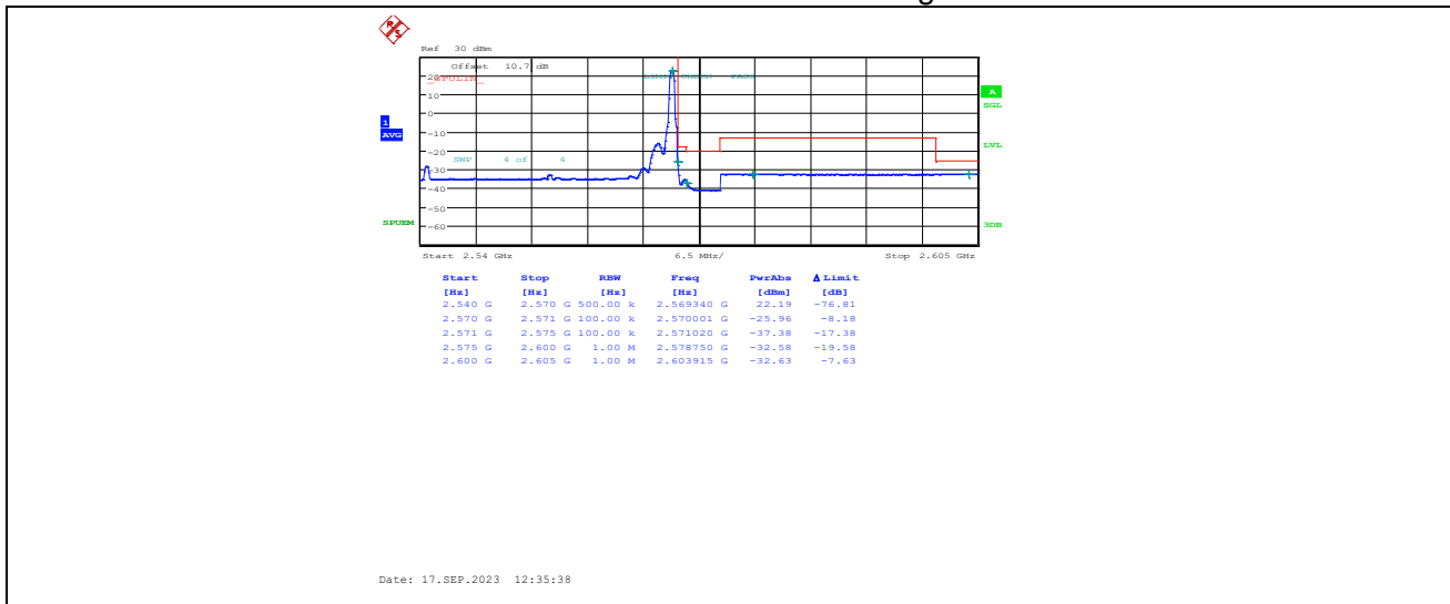
1-N7-PC3-15-30-H-2-DFT-PI2BPSK-Edge_1RB_Right-1@159-Ant3-PASS
