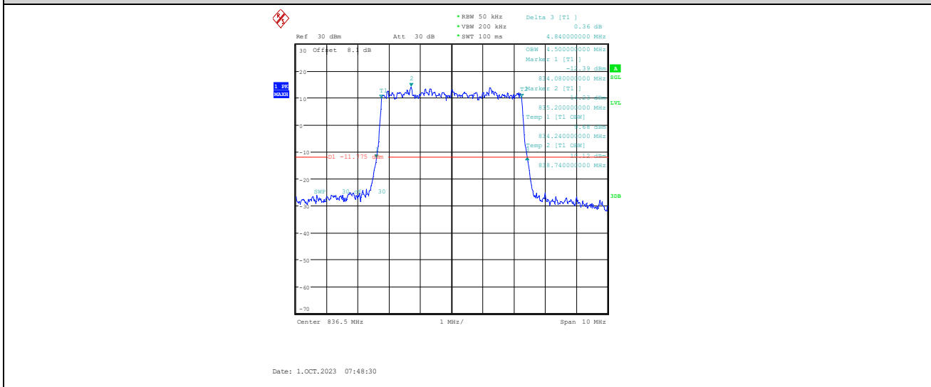
1-N5-PC3-15-5-M-4-DFT-64QAM-Outer_Full-25@0-Ant1-4.5-4.840-≤5-PASS
