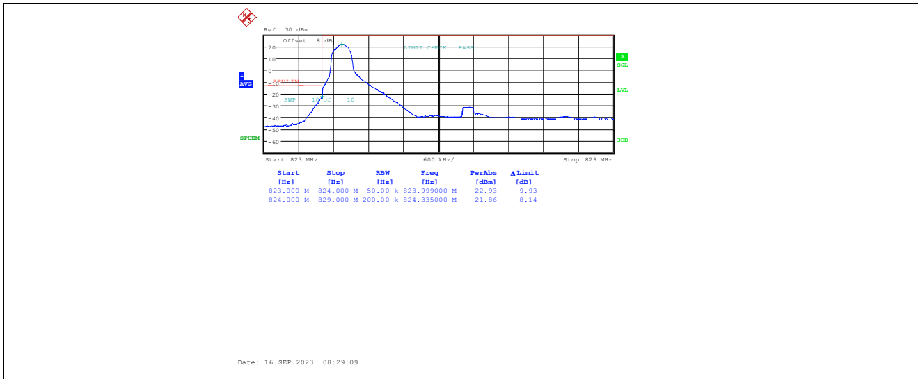
1-N5-PC3-15-5-L-1-DFT-PI2BPSK-Edge_1RB_Left-1@0-Ant1-PASS
