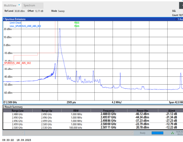
7-7-10MHz-20MHz-QPSK-QPSK-20805-20949-50RB#0-100RB#0
