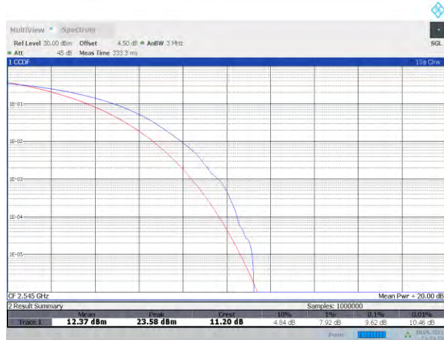
Band41-20MHz-QPSK-40140-100RB#0
