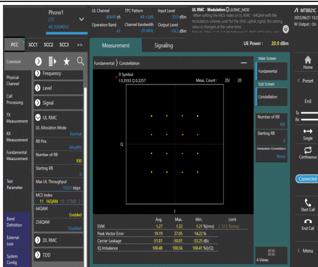
Band41-20MHz-16QAM-40640-100RB#0
