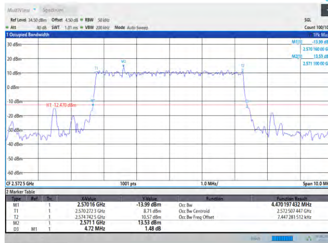
Band38-5MHz-QPSK-38000-25RB#0
