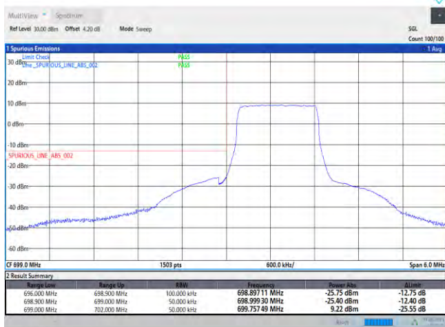
Band12-1.4MHz-QPSK-23017-6RB#0
