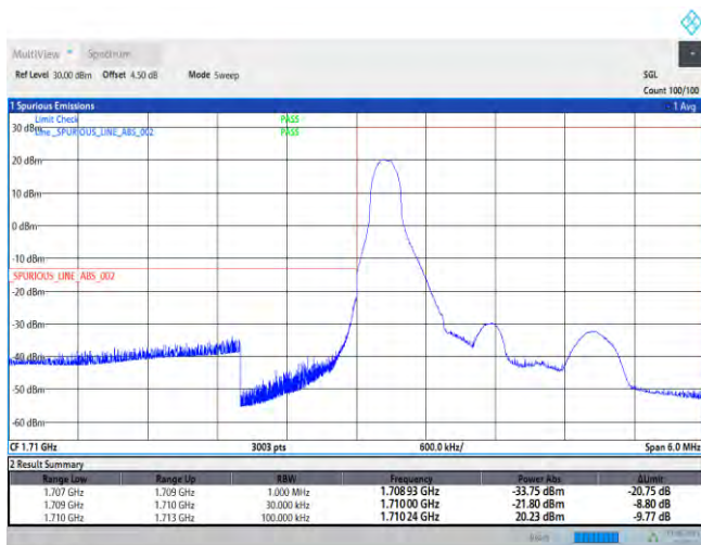
Band4-1.4MHz-QPSK-19957-1RB#0
