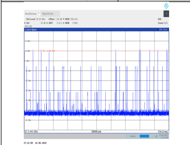
3DH5-Ant2-Hop
