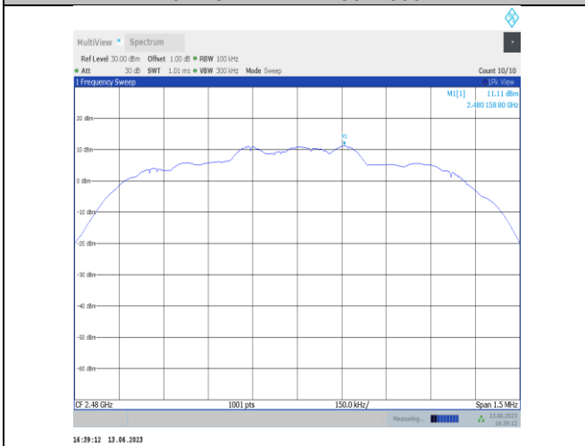
3DH5-Ant2-2480-0~Reference
