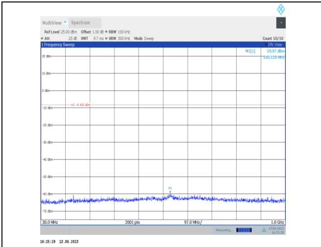
DH5-Ant2-2441-30~1000
