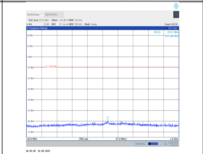
2DH5-Ant2-2441-30~1000
