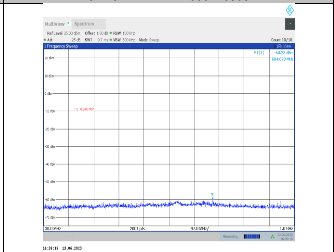
3DH5-Ant2-2480-30~1000
