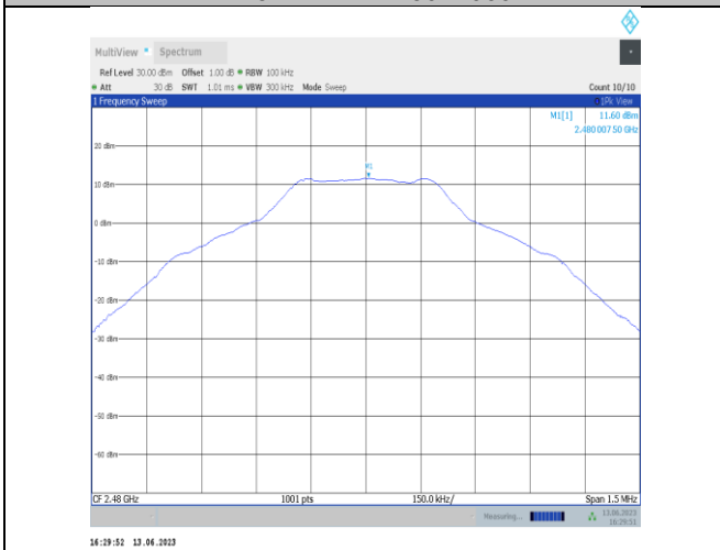
DH5-Ant2-2480-0~Reference
