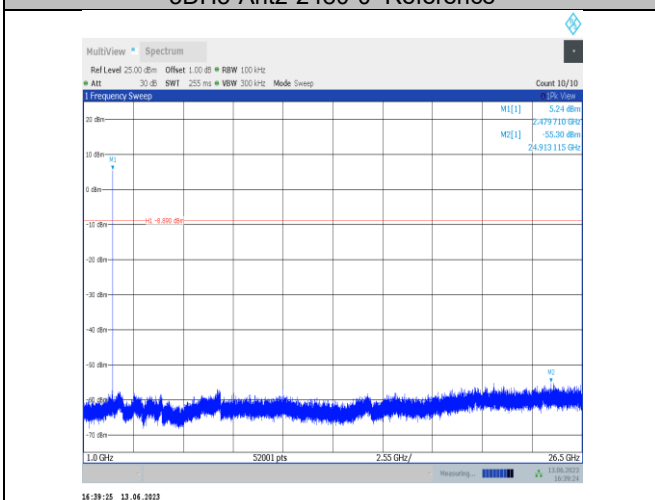
3DH5-Ant2-2480-1000~26500
