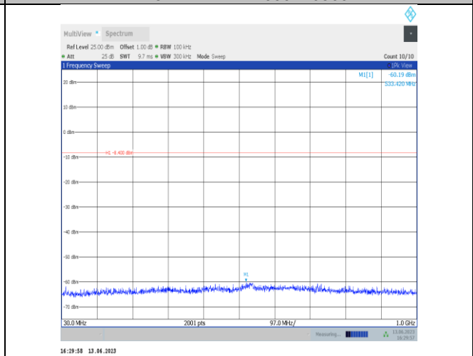
DH5-Ant2-2480-30~1000
