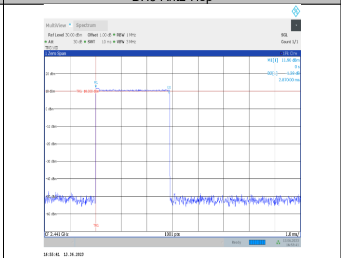
2DH5-Ant2-Hop
