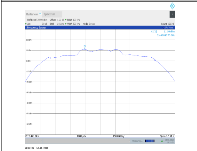
2DH5-Ant2-2441-0~Reference
