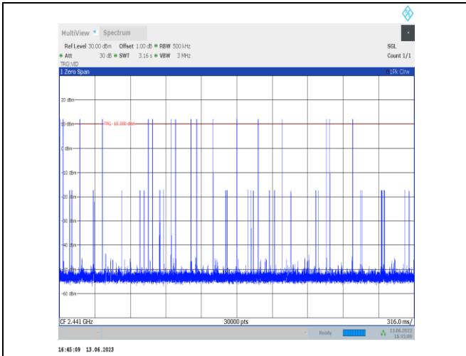
DH3-Ant2-Hop
