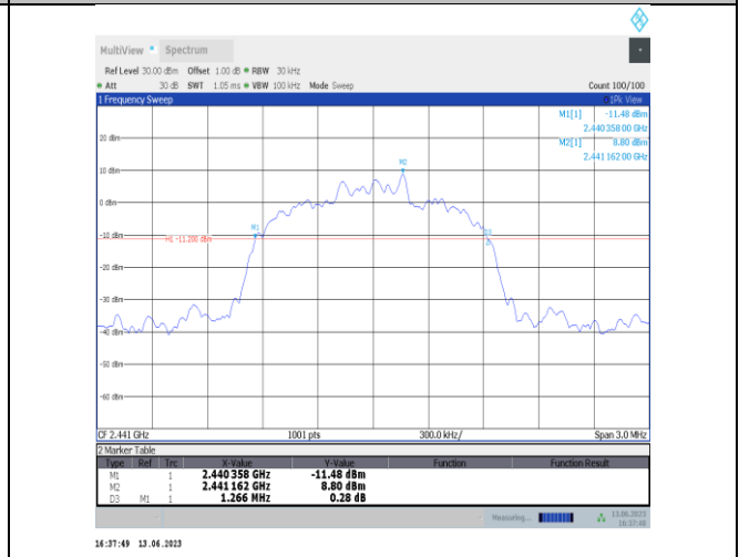
3DH5-Ant2-2441
