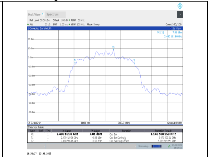
2DH5-Ant2-2480
