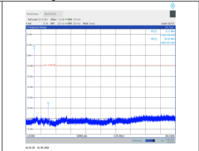
2DH5-Ant2-2402-1000~26500
