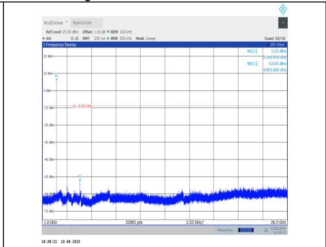
3DH5-Ant2-2441-1000~26500
