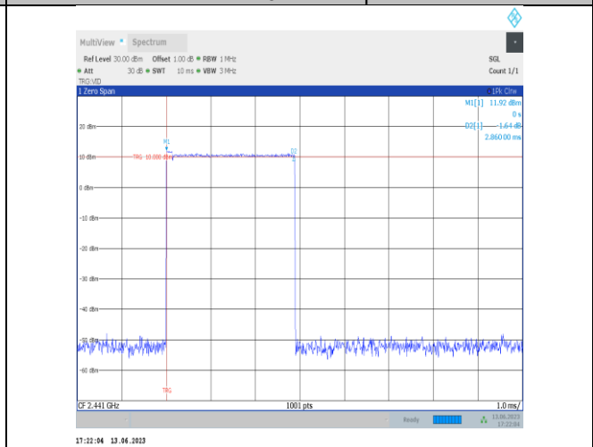
3DH5-Ant2-Hop
