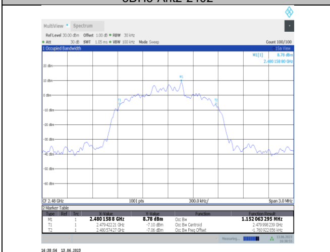
3DH5-Ant2-2480
