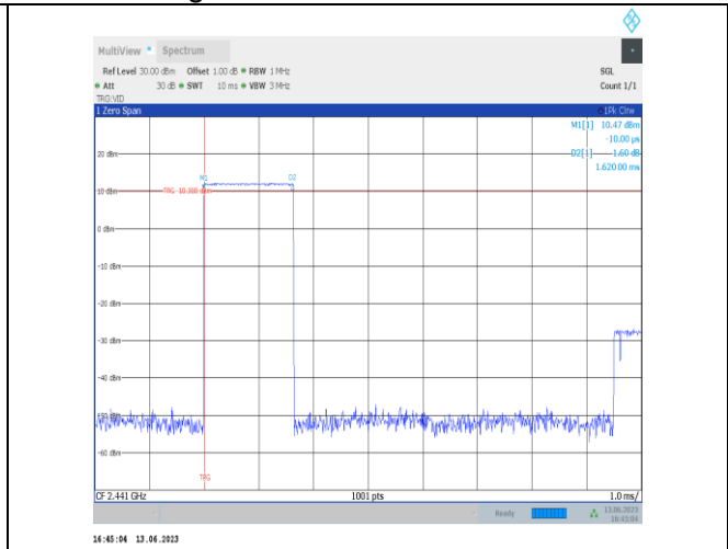
DH3-Ant2-Hop
