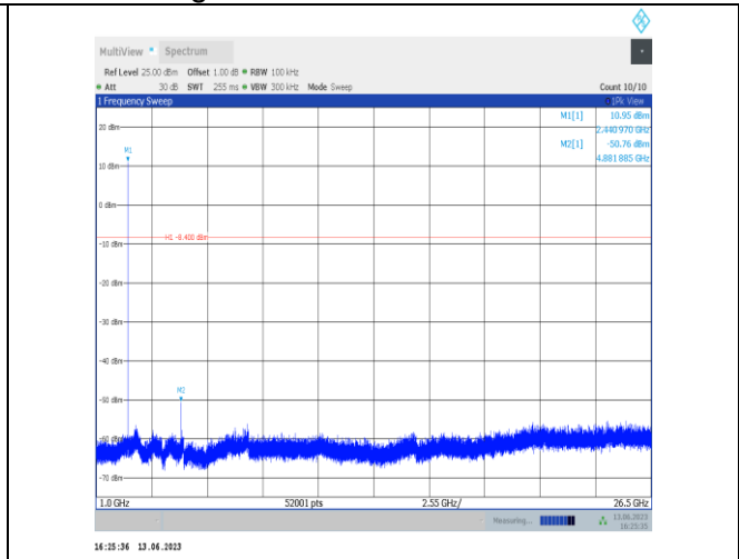
DH5-Ant2-2441-1000~26500
