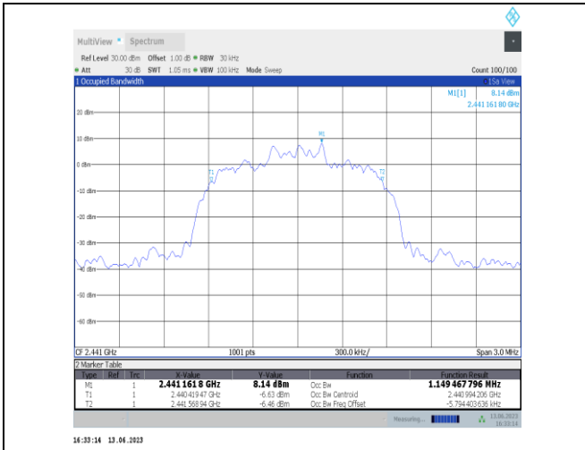
2DH5-Ant2-2441
