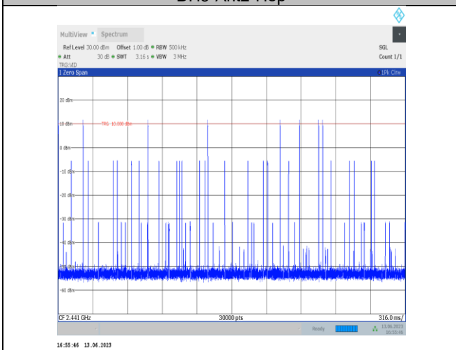
2DH5-Ant2-Hop
