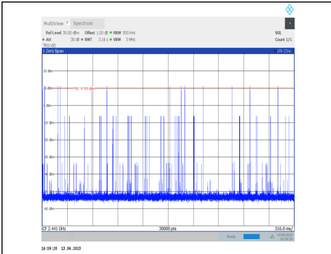
2DH3-Ant2-Hop
