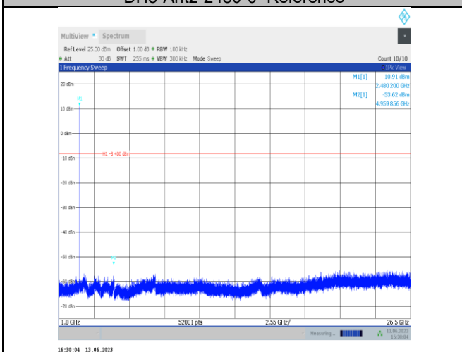
DH5-Ant2-2480-1000~26500
