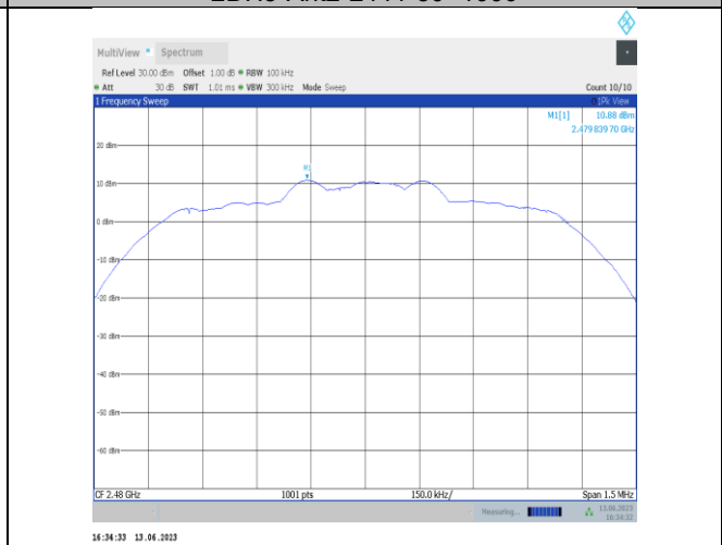
2DH5-Ant2-2480-0~Reference
