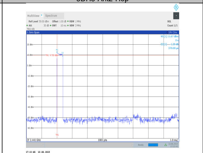
3DH1-Ant2-Hop
