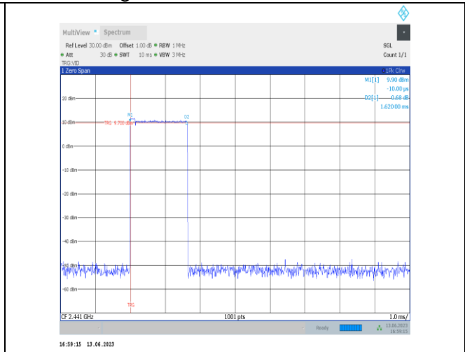
2DH3-Ant2-Hop
