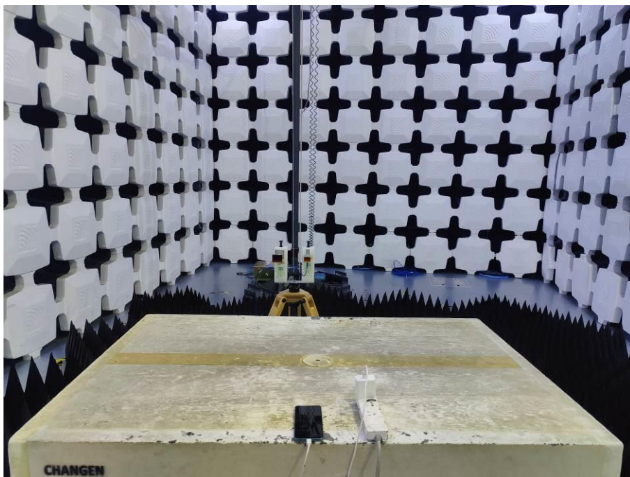
8. Radiated Emissions (Part 15B, Camera/Video Player/GSM receiver/WCDMA receiver/LTE receiver, 26.5GHz-40GHz)
