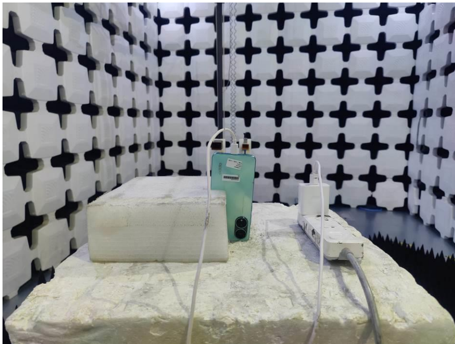
8. Radiated Emissions (Part 22/24/27, 26.5GHz-40GHz)
