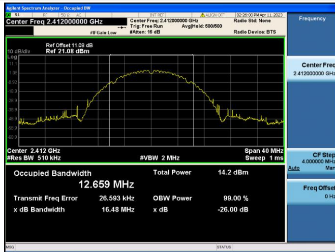
802.11b CHANNEL 1
